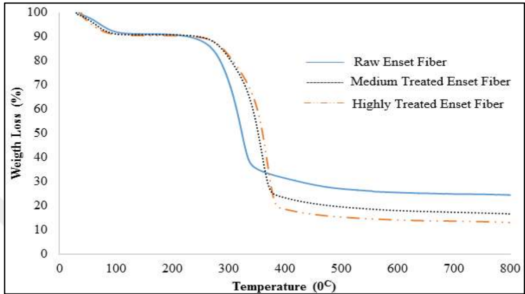
Figure 4. 6. TGA curves of raw, medium and highly treated enset fibers
