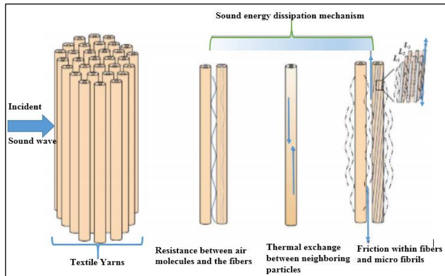
Figure 2.20. Sound energy dissipation mechanism of porous textile material (Jichun et al. 2018)
