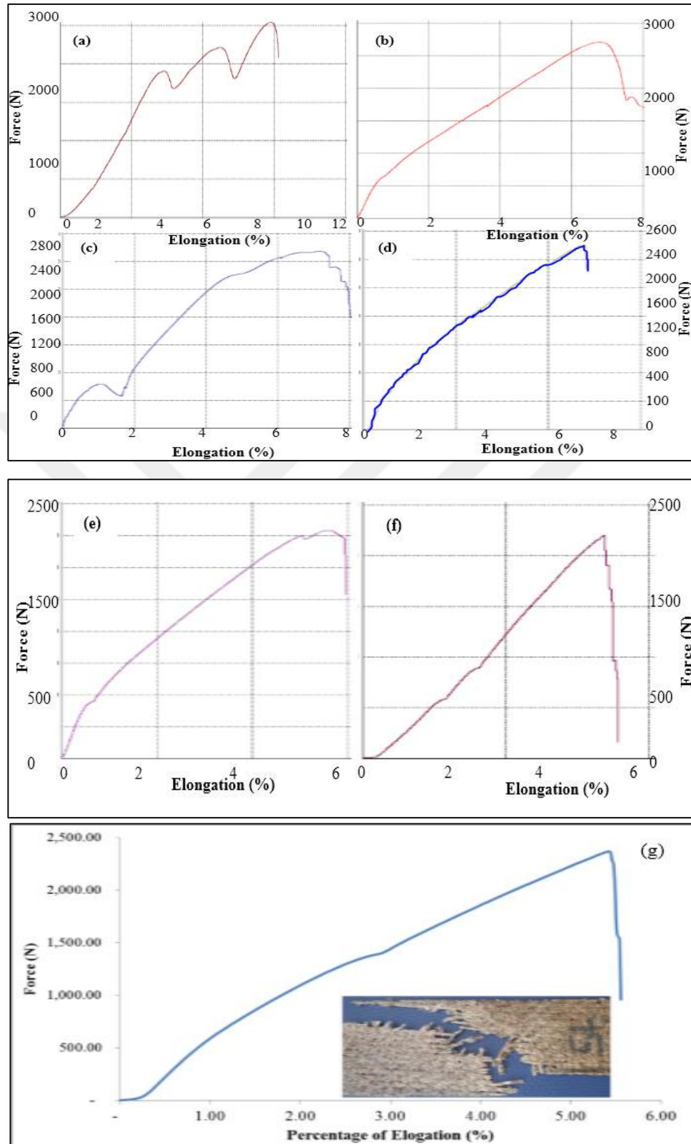
Figure 4.8. Single layer enset fabric reinforced green composite via acacia to frankincense bio resin mixing ratio (%) a) 75:25 b) 70:30 c) 65: 35 d) 60:40 e) 55:45 f and g) 50:50
