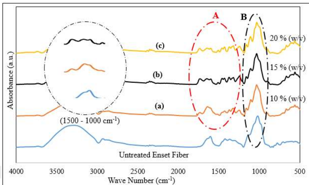
Figure 4.5. FTIR gradual wiped-out of hemicellulose and lignin from enset fiber with \alpha -amylase enzyme treatment and mechanical hammering a) 10% (w/v) \alpha -amylase enzyme treated b) 15% (w/v) \alpha -amylase enzyme treated c) 20% (w/v) \alpha -amylase enzyme treated enset fiber
