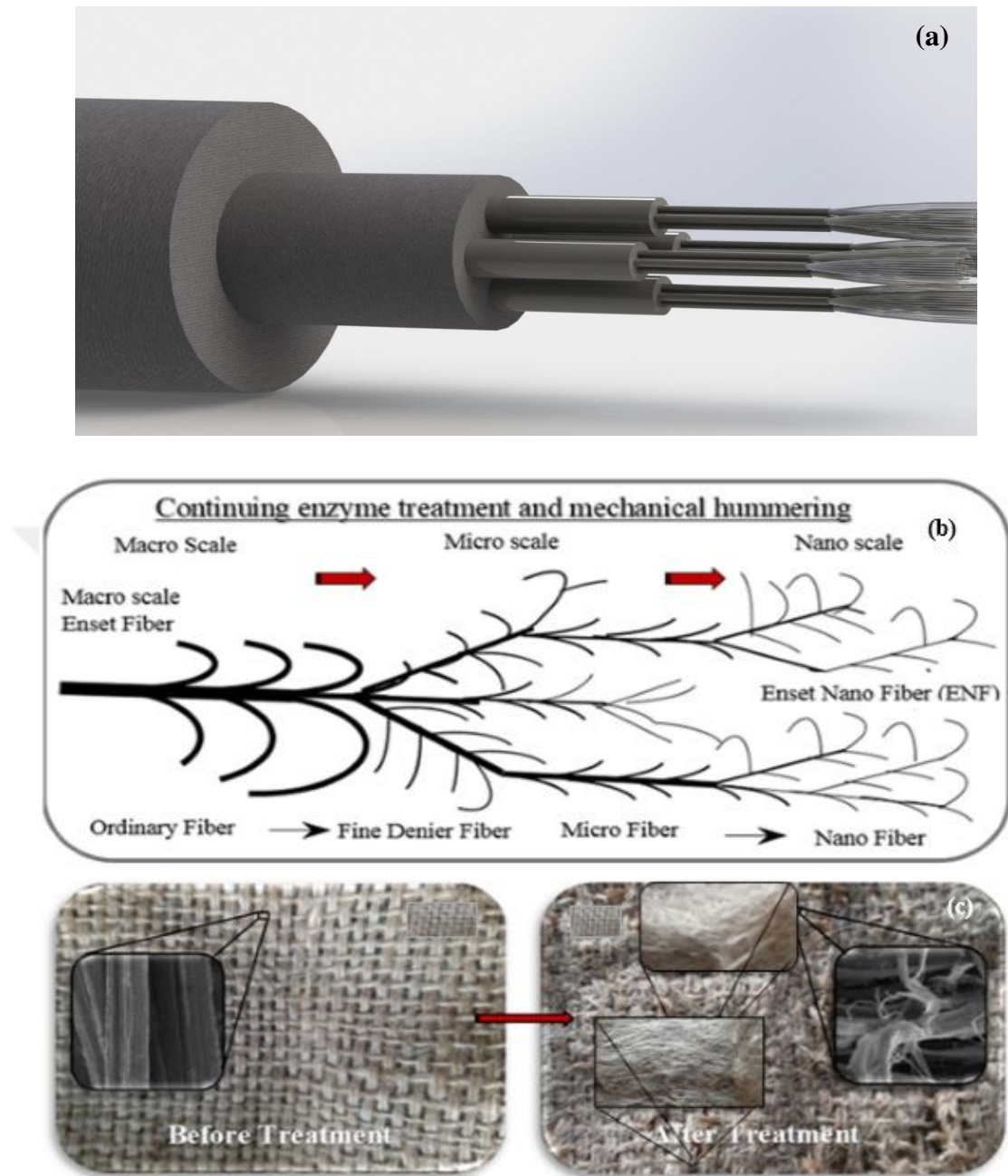
Figure 3.14. a) Auto CAD simulation b) Schematic illustration of micro and nano enset fiber preparation c) Micro and nano enset fiber preparation by \alpha -amylase enzyme treatment and mechanical hammering
