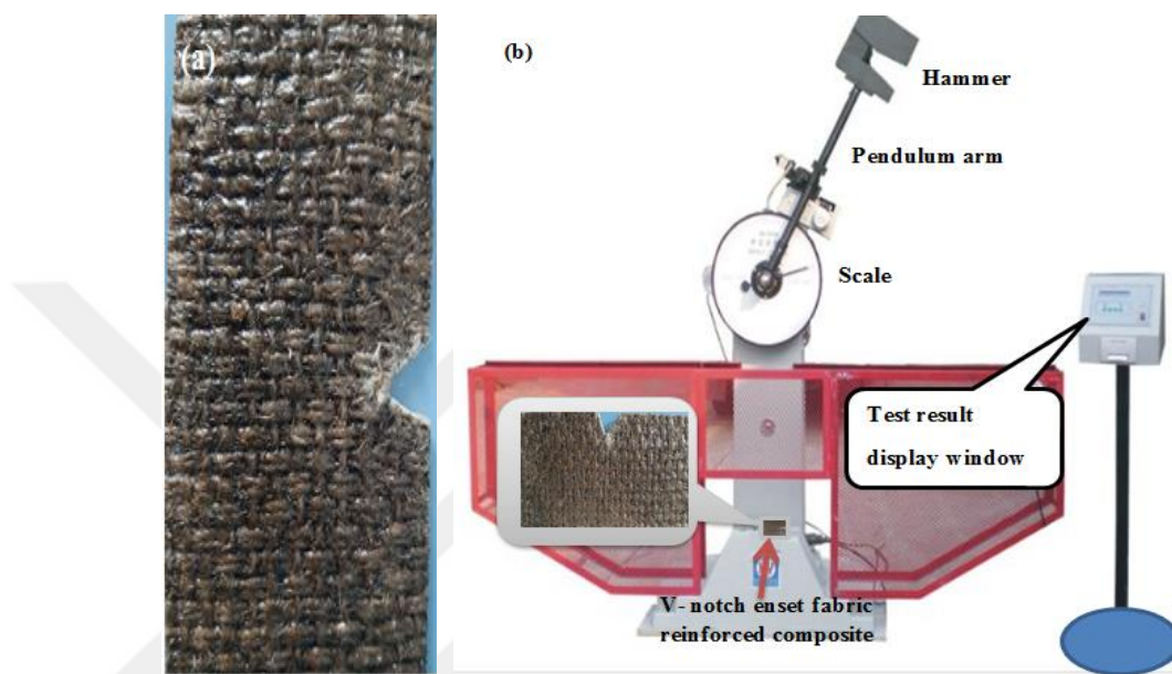
Figure 3.13. a) V- notch sample for impact strength testing b) JBW-300 computer display pendulum impact strength testing device
