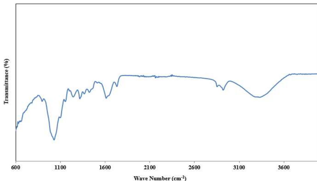
Figure 3.3. FTIR adsorption bands of enset fiber 11
