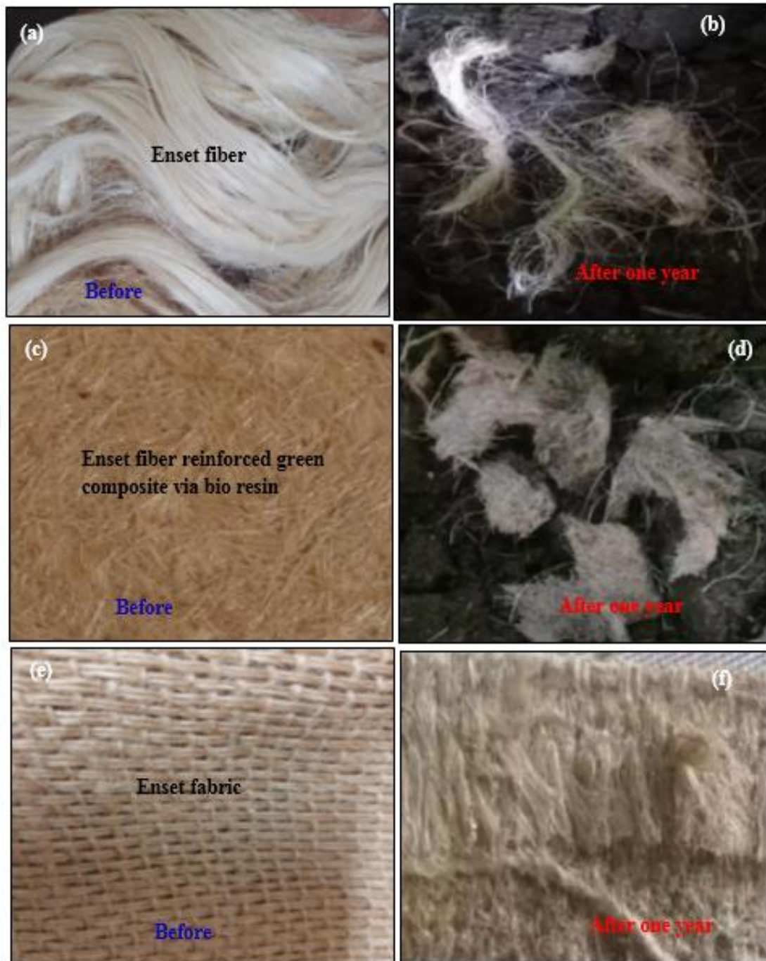
Figure 4.24. Biodegradability test of enset textile materials kept in in soil for one year a) Neat enset fiber b) Enset fiber after one year c) Fiber reinforced green composite d) Green composite after one year e) Neat enset fabric f) Enset fabric after one year
