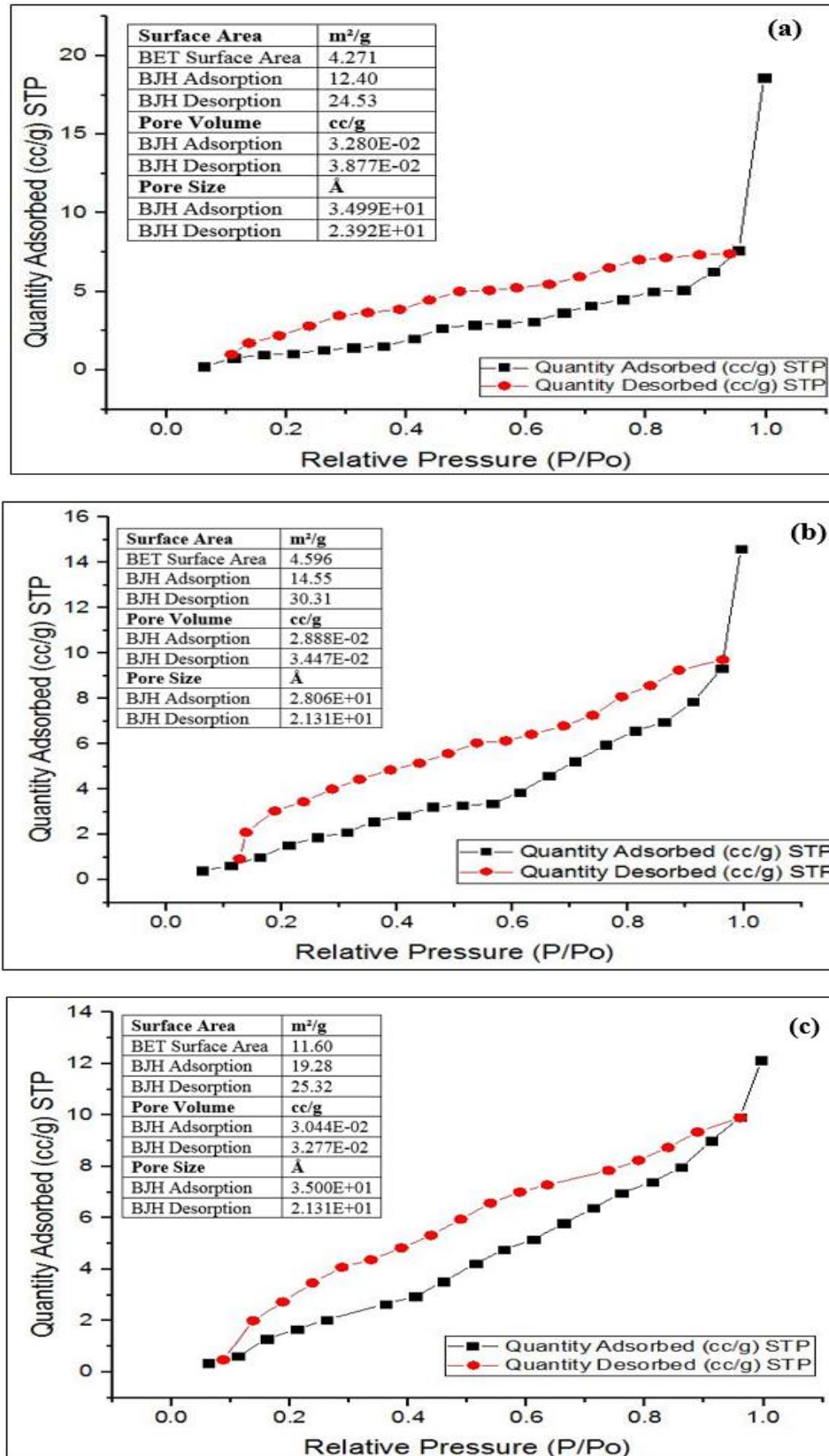
Figure 4.4. BET curve-surface area analysis of treated enset fiber a) 10 % w/v b) 15% w/v and c) 20% w/v concentration of \alpha -amylase enzyme
