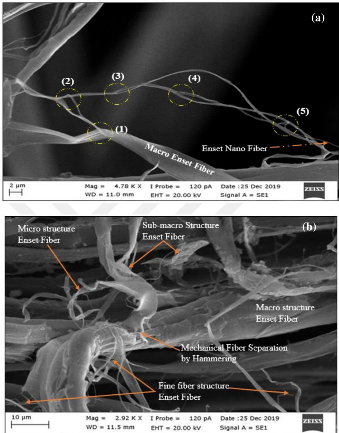
Figure 4.3. SEM views: a) Hierarchical defibrillation of macro-scale enset fiber into enset nano fiber b) Gradually removal of hemicellulose and lignin from the macro structure of enset fiber by mechanical hammering
