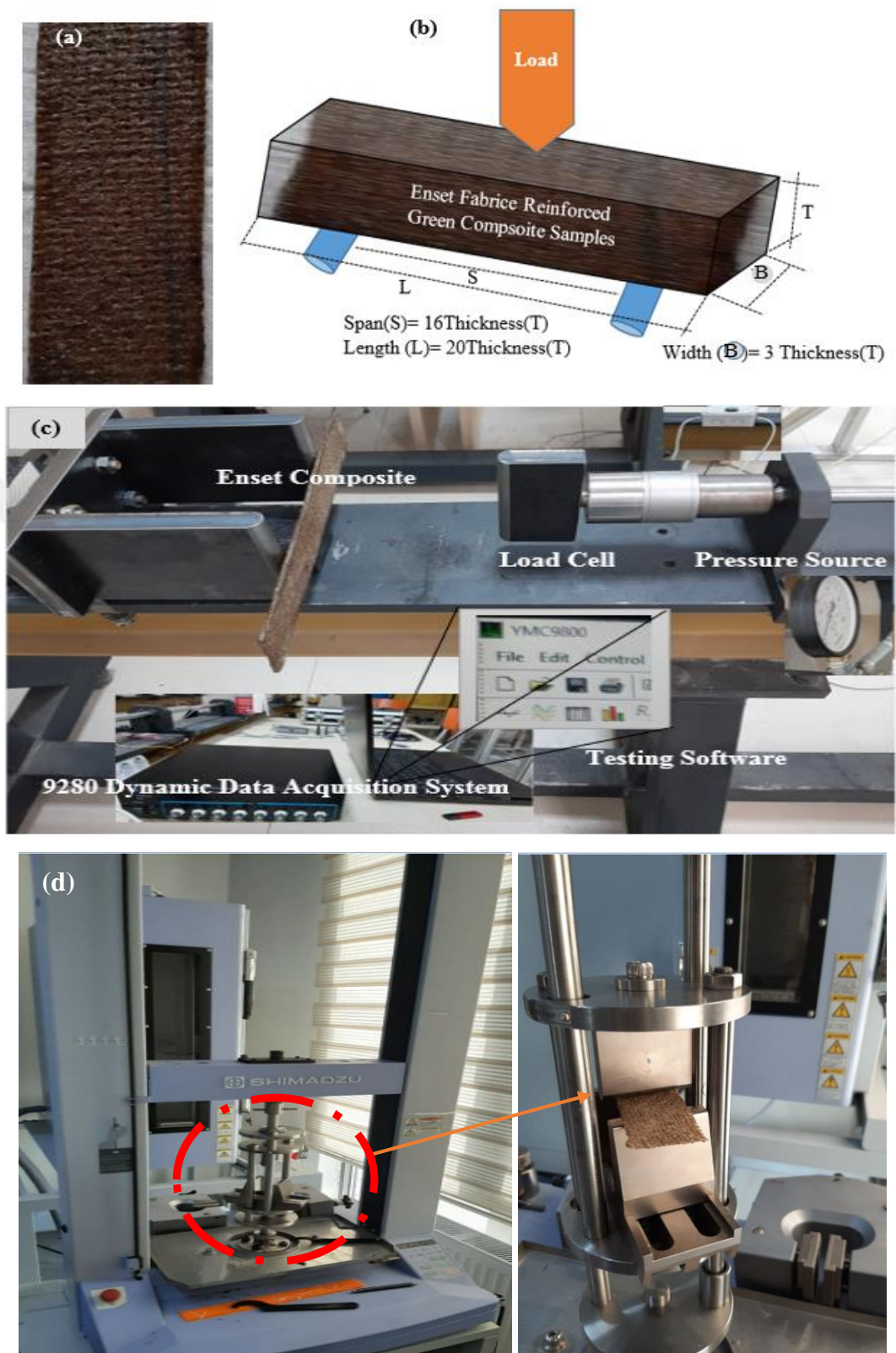
Figure 3.11. a) Enset fabric reinforced composite specimens b) Schematic illustration of 3 point bending flexural test c) Dynamic flexural strength tester d) Shimadzu strength tester
