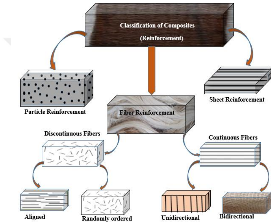
Figure 2.9. Classification of composite based on reinforcing material (Rajak et al. 2019)
