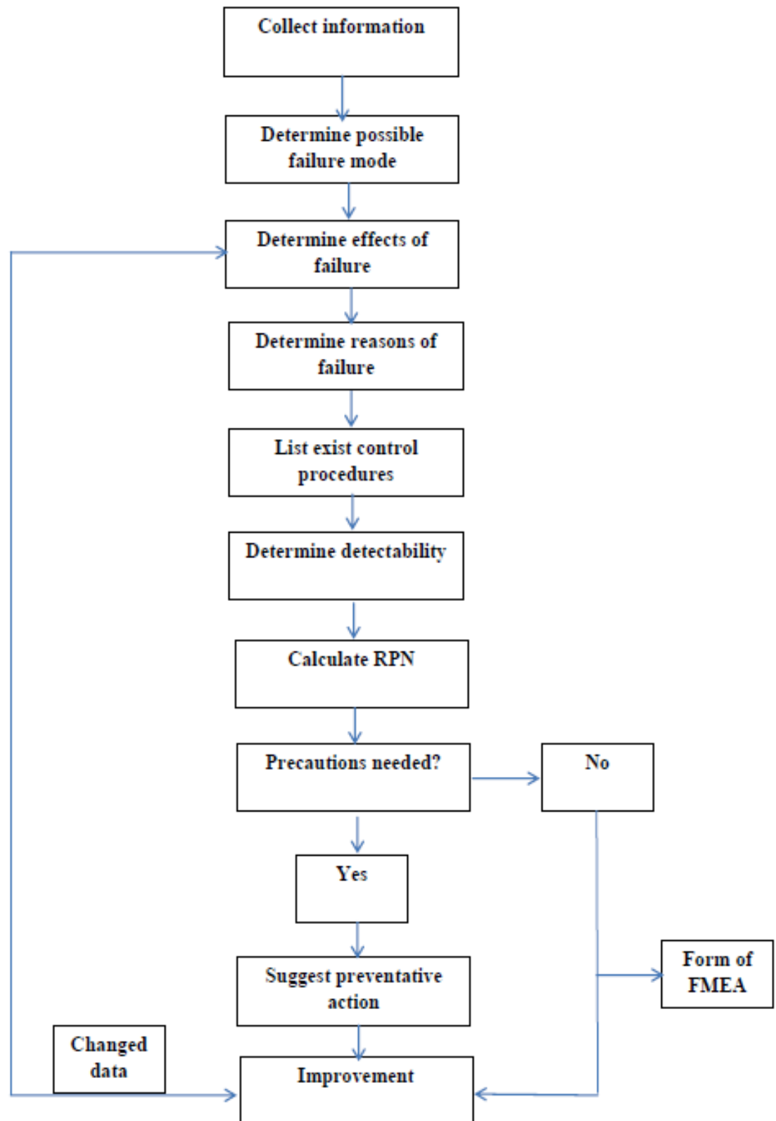
Figure 2.8 FMEA process
