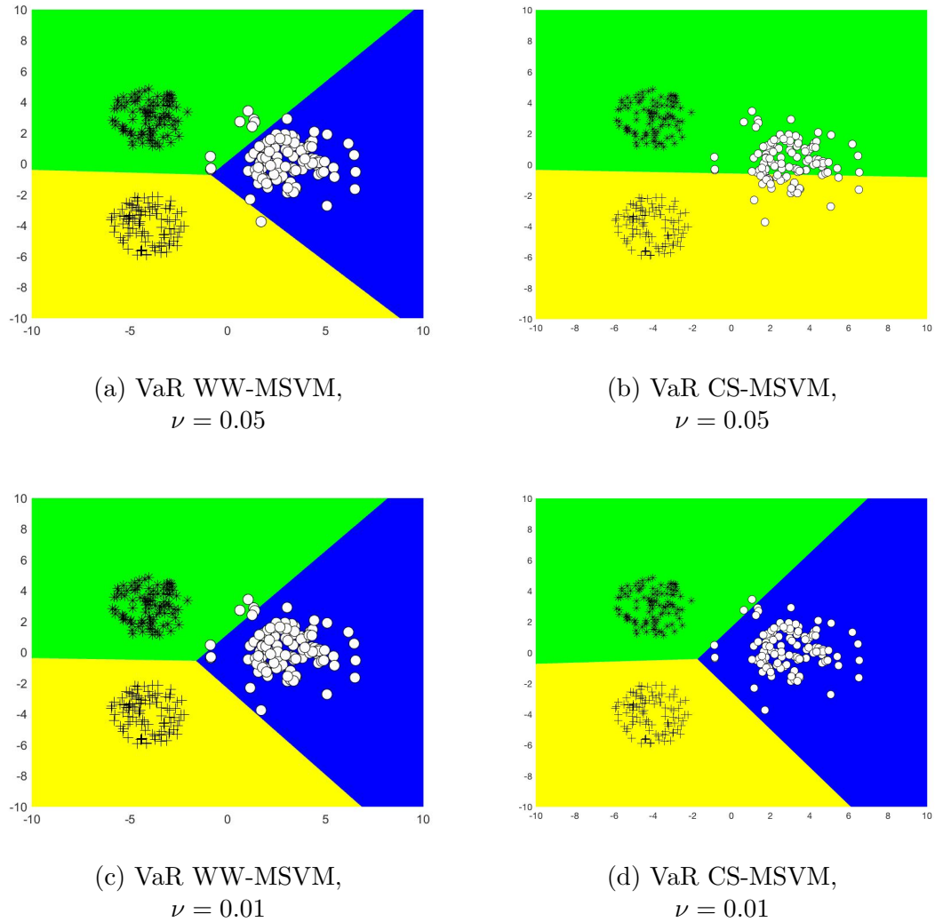
Figure 5.21: Comparison of VaR WW-MSVM and VaR CS-MSVM with different \nu values under 0.05 class 1 probability for Outlier 3 dataset.
