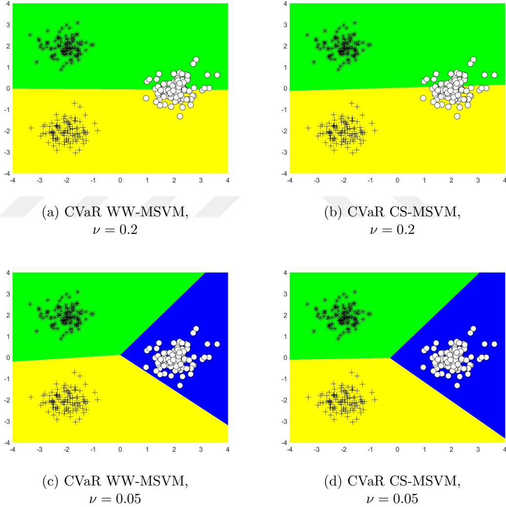
Figure 5.6: Comparison of CVaR WW-MSVM and CVaR CS-MSVM with different \nu values under 0.01 class 1 probability for Ratio 1 dataset.
