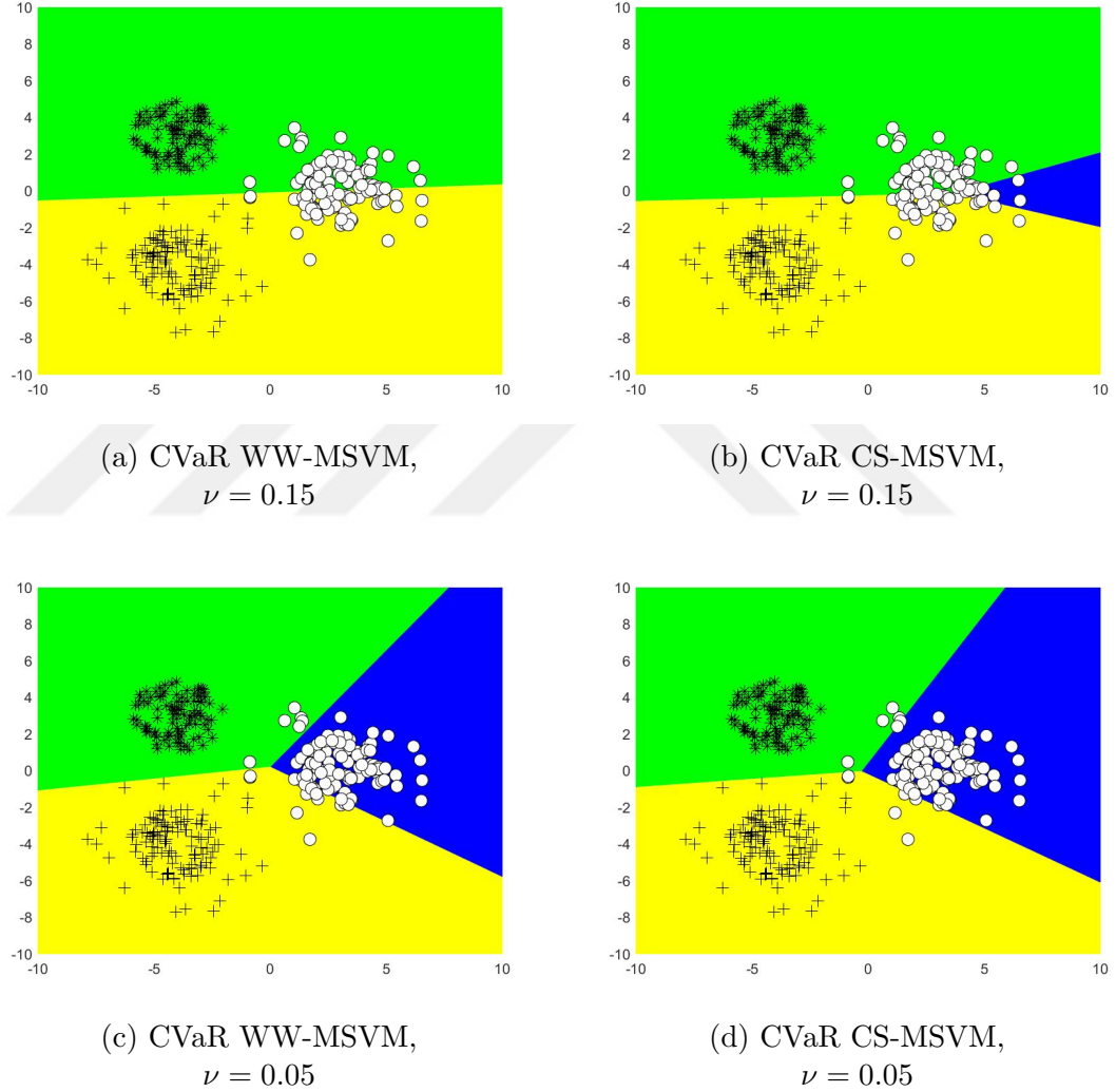
Figure 5.12: Comparison of CVaR WW-MSVM and CVaR CS-MSVM with different \nu values under 0.01 class 1 probability for Outlier 2 dataset.
