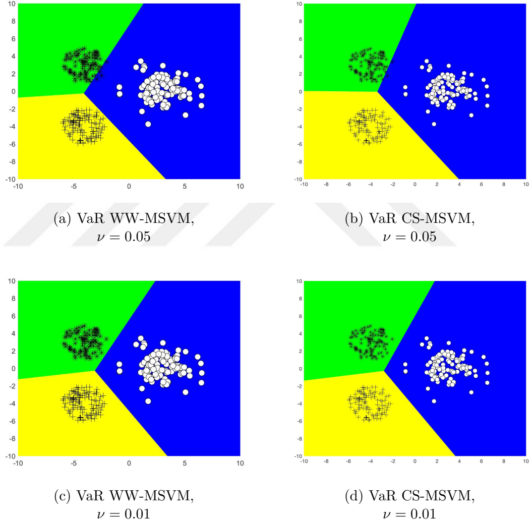
Figure 5.22: Comparison of VaR WW-MSVM and VaR CS-MSVM with different \nu values under 0.88 class 1 probability for Outlier 3 dataset.
