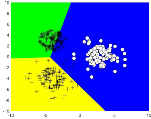
(a) CVaR WW-MSVM, \nu = 0.15
