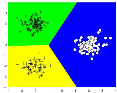
(h) CVaR WW-MSVM, 0.88 class 1 probability
