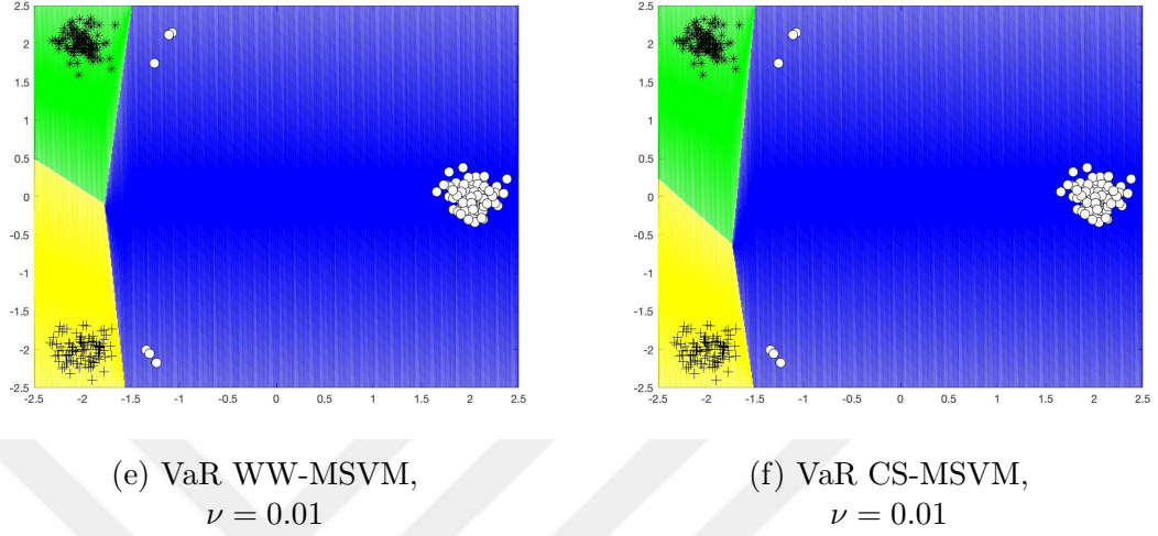
Figure 5.19: Comparison of VaR WW-MSVM and VaR CS-MSVM with different \nu values under 0.88 class 1 probability for Noise 2 dataset.
