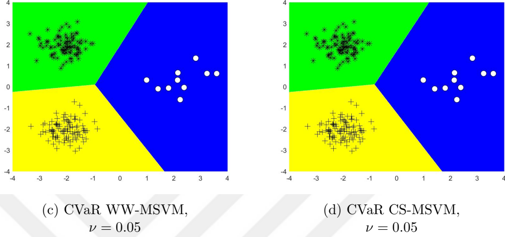
Figure 5.8: Comparison of CVaR WW-MSVM and CVaR CS-MSVM with different \nu values under 0.88 class 1 probability for Ratio 6 dataset.
