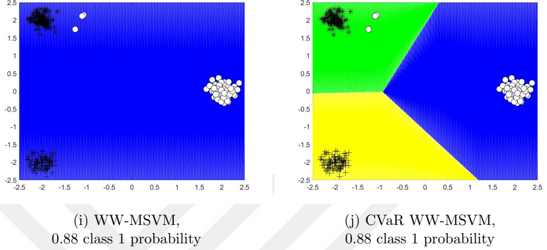
Figure 5.4: Comparison of WW-MSVM and CVaR WW-MSVM with \nu = 0.1 under different class 1 probabilities for Noise 1 dataset.
