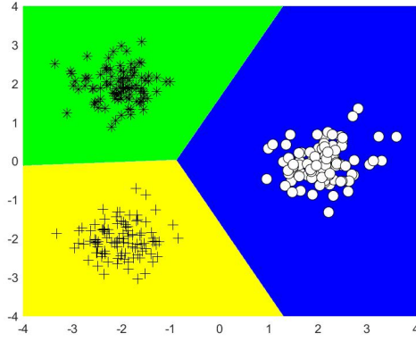
(c) CVaR CS-MSVM, 0.88 class 1 probability
