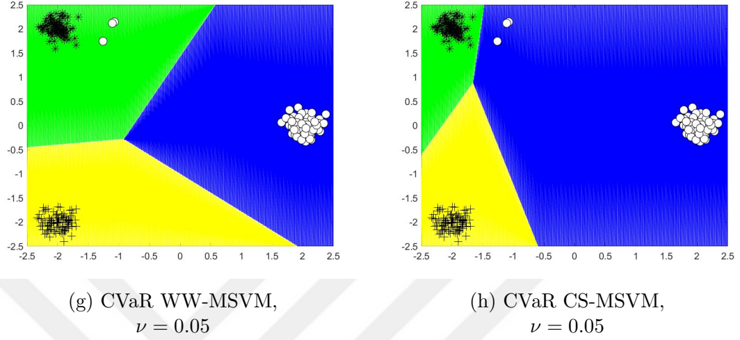
Figure 5.9: Comparison of CVaR WW-MSVM and CVaR CS-MSVM with different \nu values under 0.88 class 1 probability for Noise 1 dataset.
