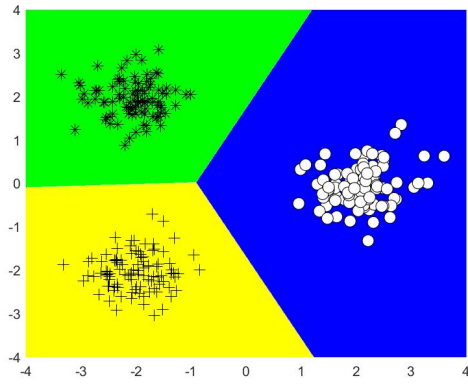
(c) CVaR WW-MSVM, \nu = 0.05
