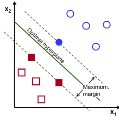
(b) Maximum margin hyperplane constructed by SVM
