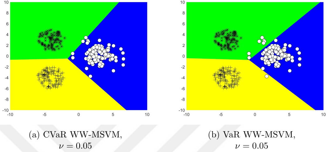
Figure 5.17: Comparison of CVaR WW-MSVM and VaR WW-MSVM with different \nu values under 0.05 class 1 probability for Outlier 3 dataset.
