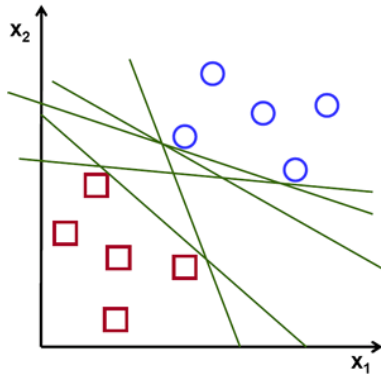
(a) Separating hyperplanes for binary classification problem
