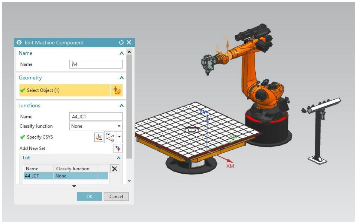
Figure 7-6: Fourth axis
