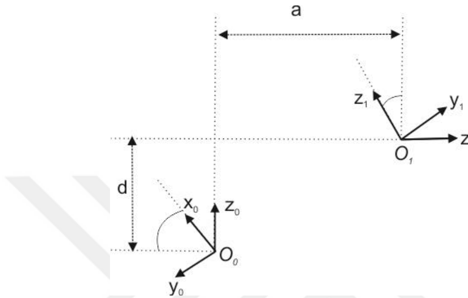
Figure 2-2: Homogenous transformation O_0 to O_1
