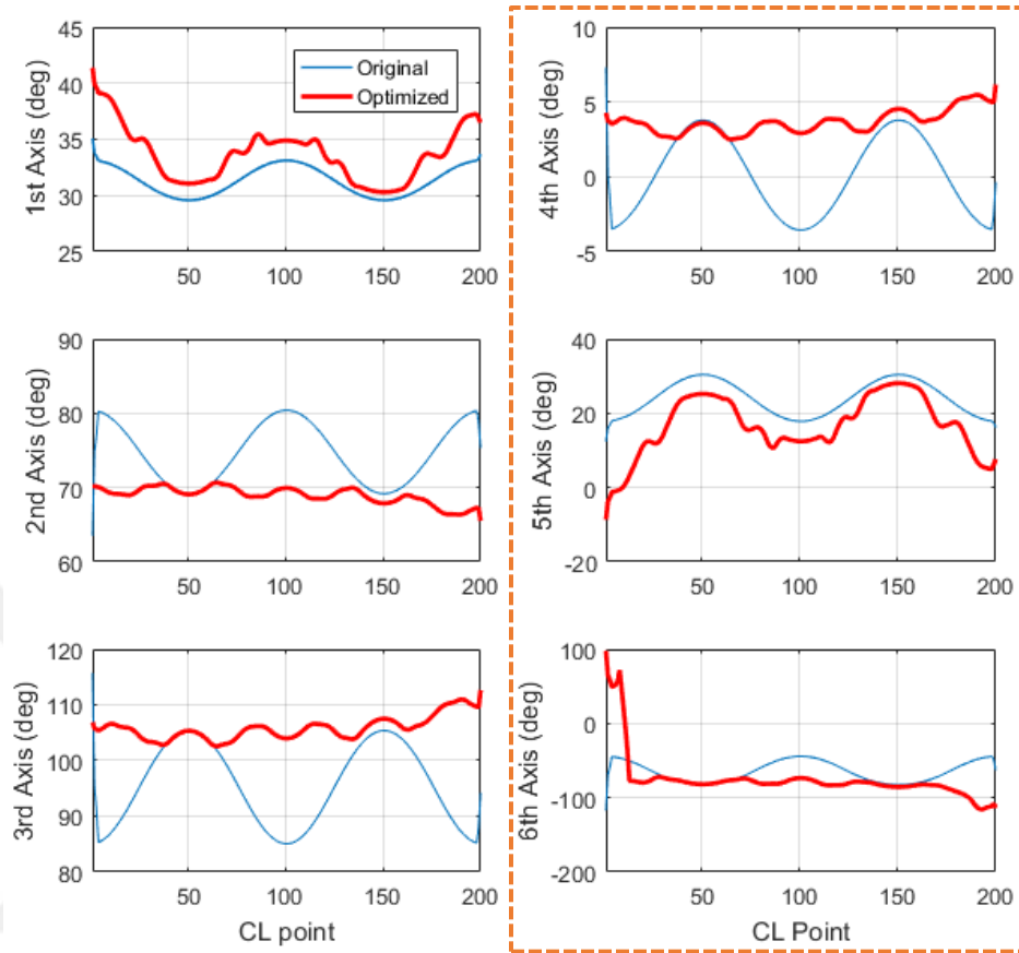
Figure 3-13: Optimized angles wrt last three axes (Case 2)
