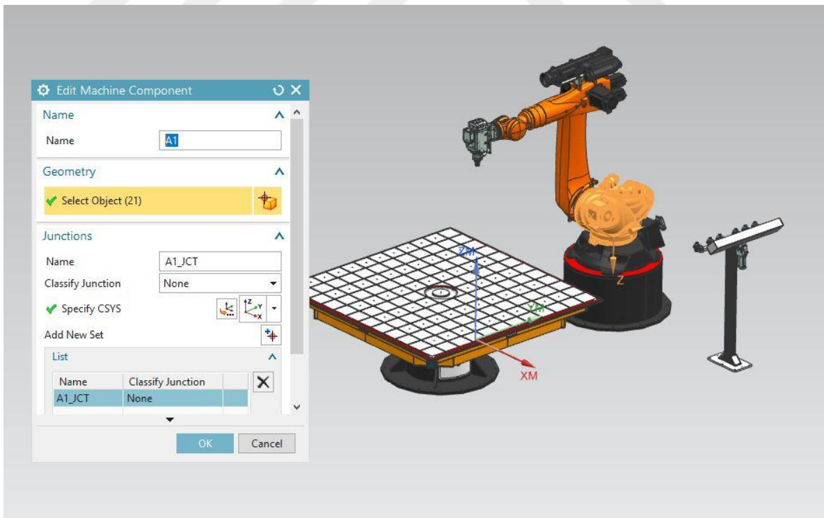
Figure 7-2: Robot base
