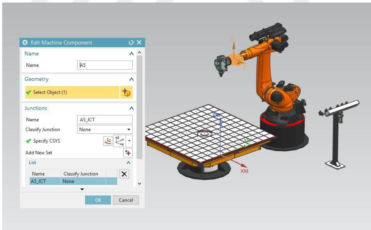
Figure 7-7: Fifth axis
