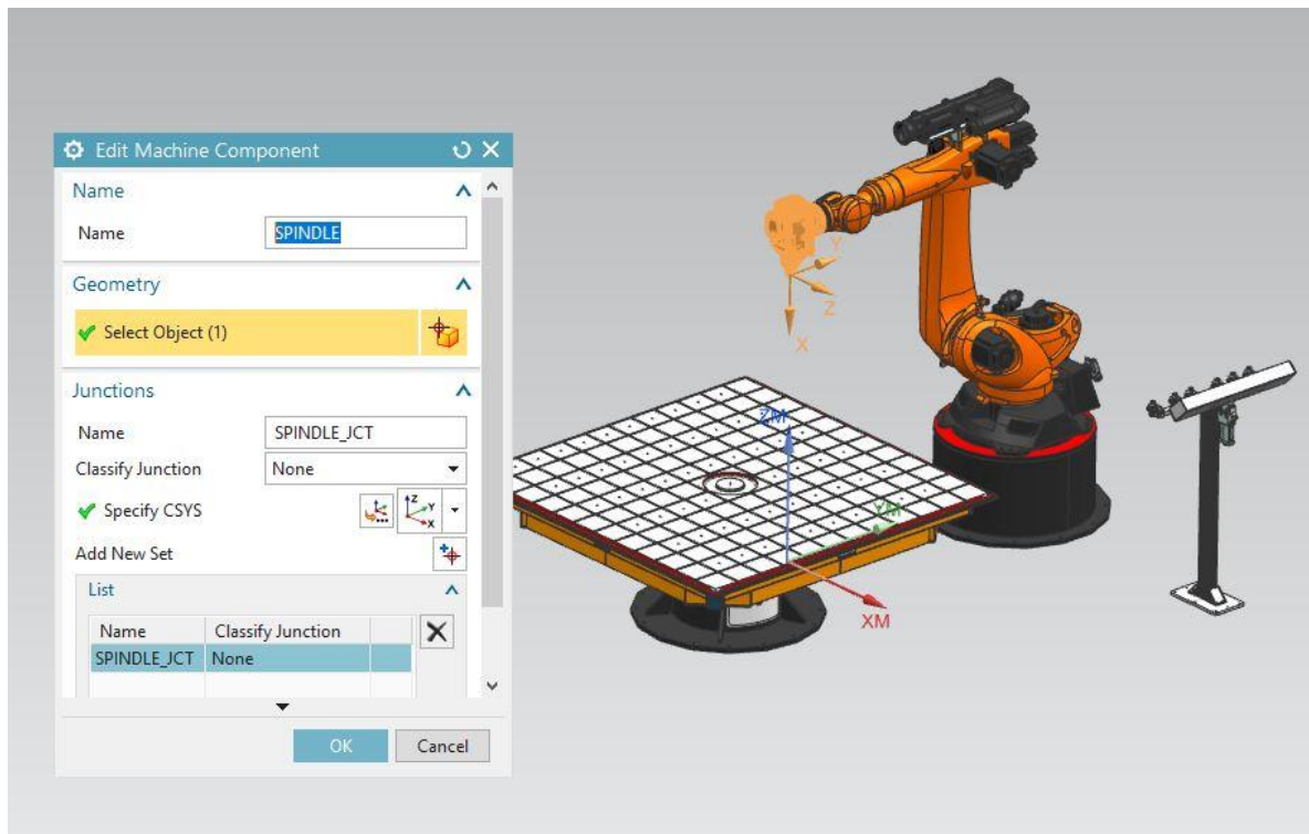
Figure 7-9: Spindle
