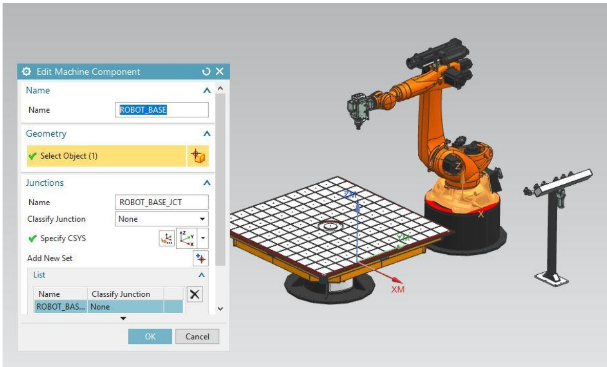
Figure 7-2: Robot base
