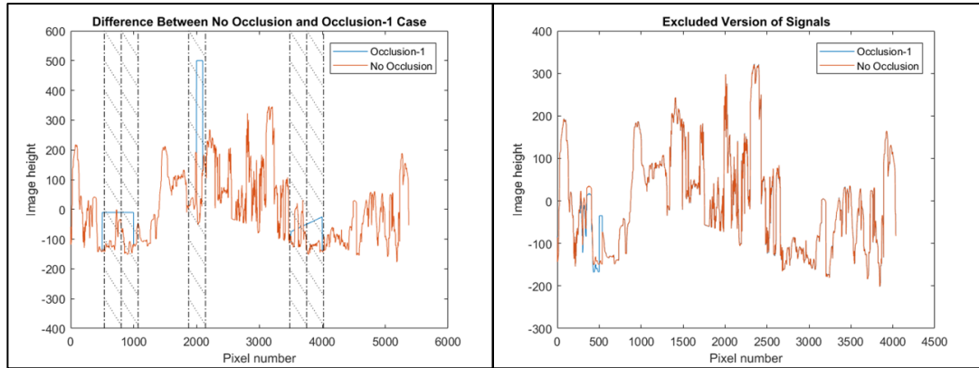
Figure 5.37. Occlusion-1 and Excluded Version of Skyline Signal
