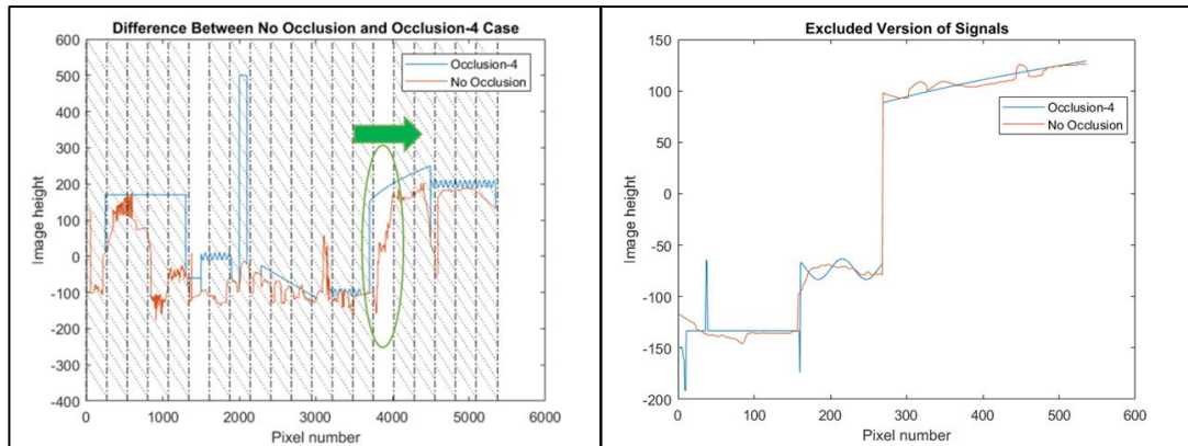
Figure 5.29. Occlusion-4 and Excluded Version of Skyline Signal “K(Diag1,5,Leaves-Sunrise)”
