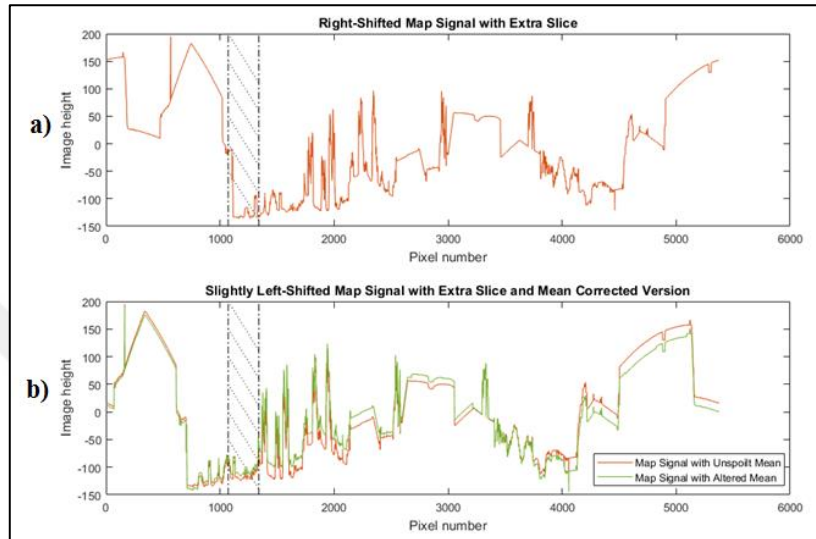
Figure 4.16. a) Map Signal Shifted Certain Amounts
