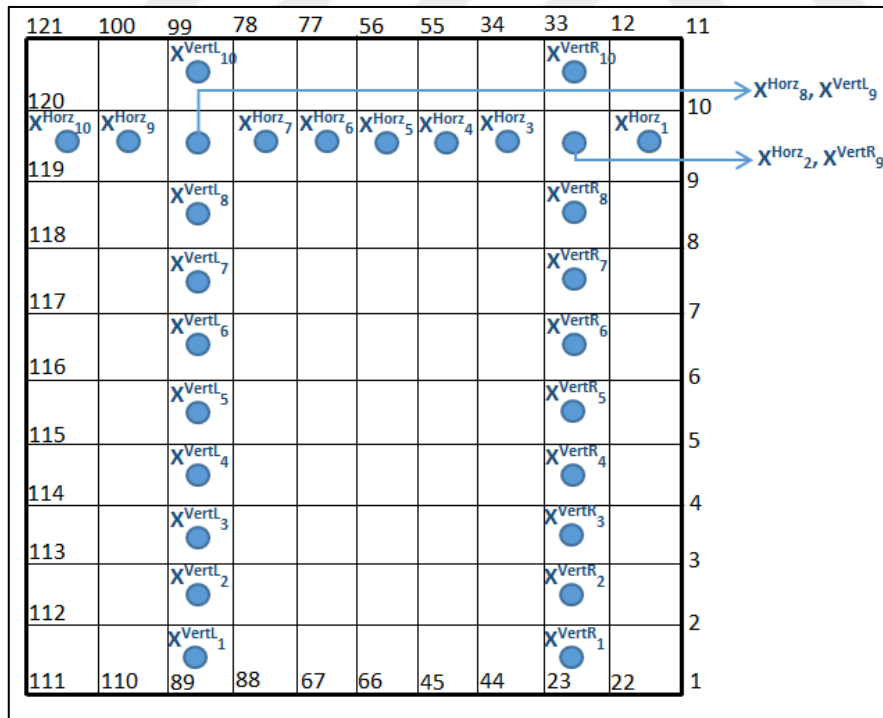
Figure 5.6. Points of Test Areas “Horz”, “VertL” and “VertR”
