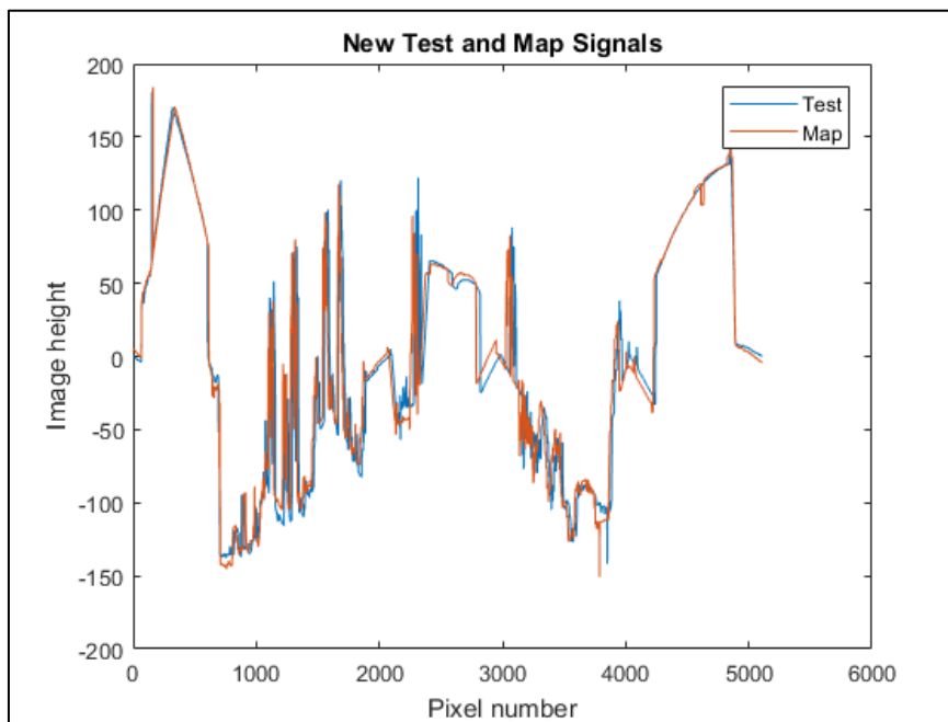
Figure 4.19. New Test and Map Signals to Obtain a Similarity Value
