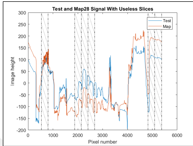
Figure 5.40. Skyline Signals of "K(VertR,5,Leaves-Cloudy)" and "K(Map,28,Leaves-Sunrise)"
