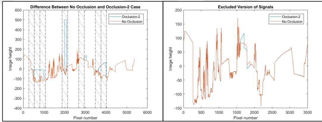
Figure 5.33. Occlusion-2 and Excluded Version of Skyline Signal “T(Diag1,5,NoLeaves-Noon)”
