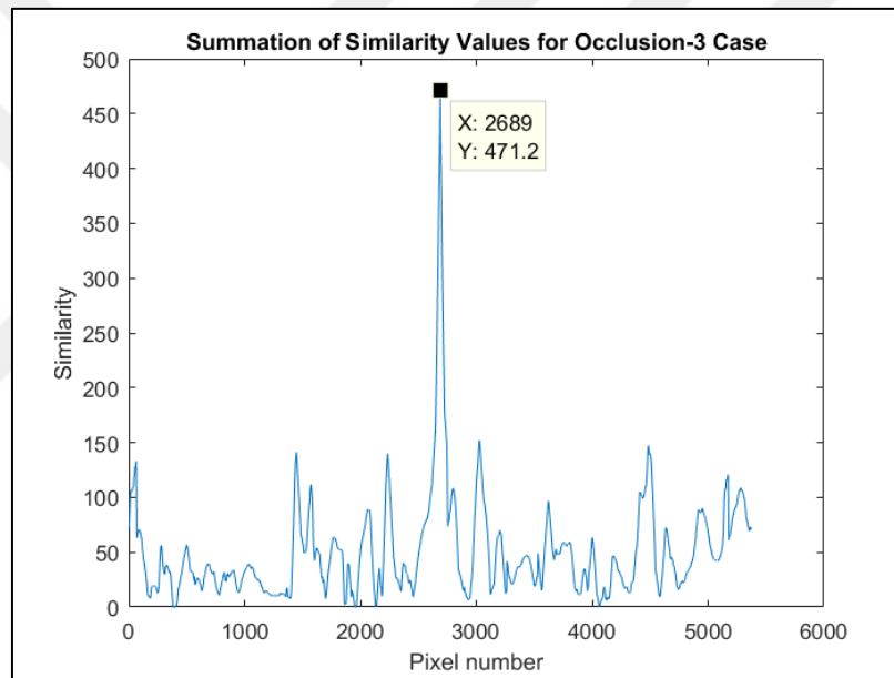
Figure 5.30. Summation of Similarity Values for “K(Diag1,5,Leaves-Sunrise)” Occlusion-3 Case
