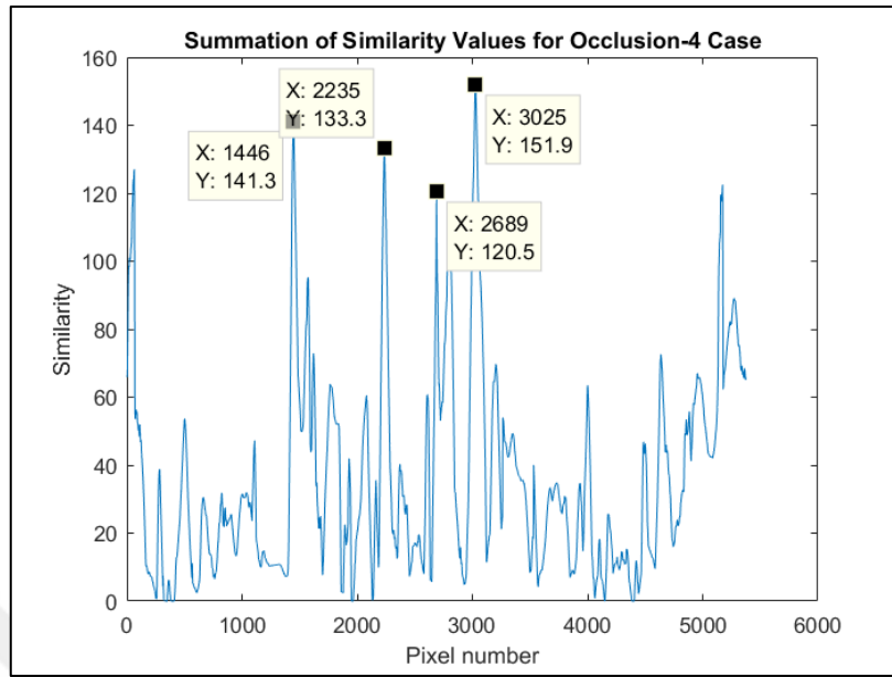
Figure 5.31. Summation of Similarity Values for “K(Diag1,5,Leaves-Sunrise)” Occlusion-4 Case
