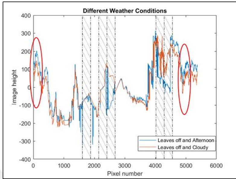
Figure 5.9. Skyline Signals of “B(Diag1,5,NoLeaves-Afternoon)” and “B(Diag1,5,NoLeaves-DarkClouds)”
