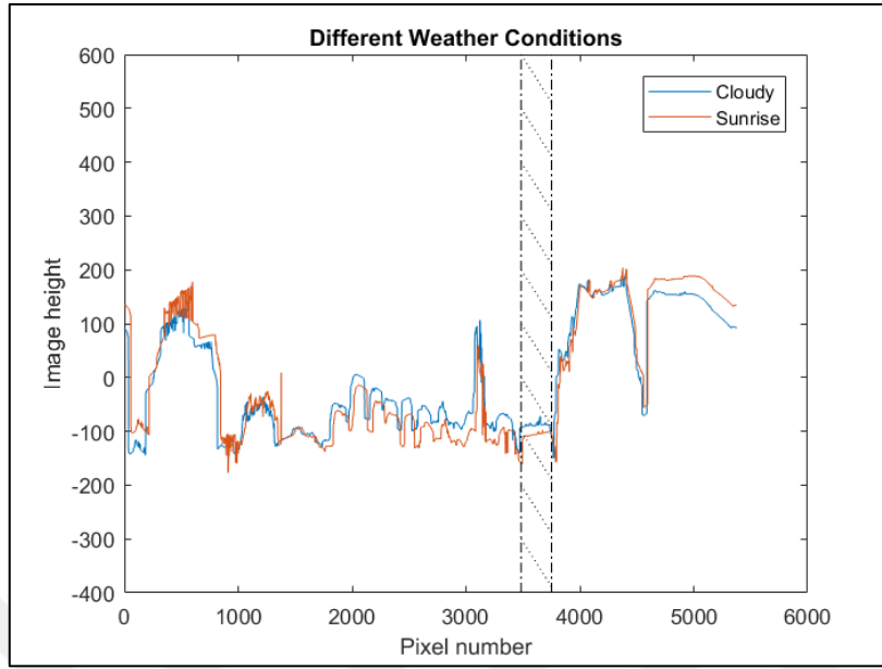
Figure 5.13. Skyline Signal of Photographs Captured at Different Conditions for Test Location “K”, “K(Diag1,5,Leaves-Sunrise)” and “K(Diag1,5,Leaves-Cloudy)”
