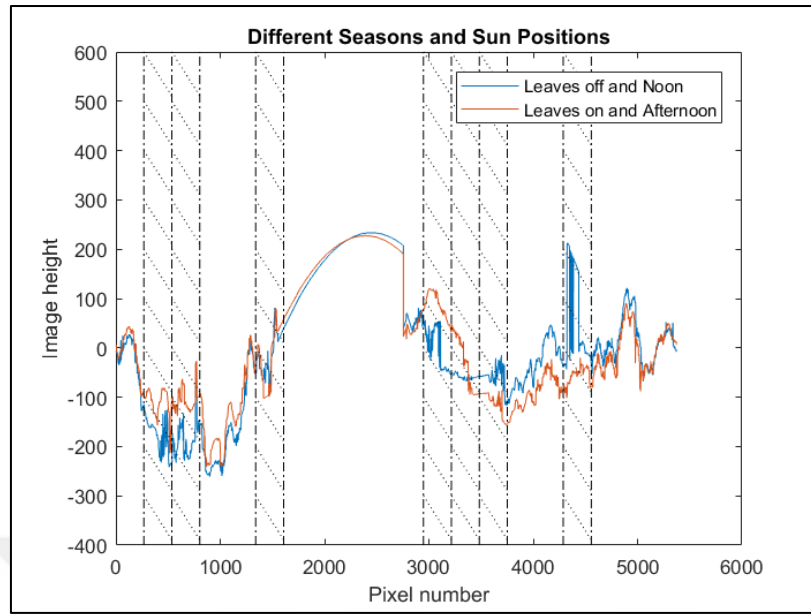
a) “G(Diag1,5,Leaves-Afternoon)” and “G(Diag1,5,NoLeaves-Noon)”
