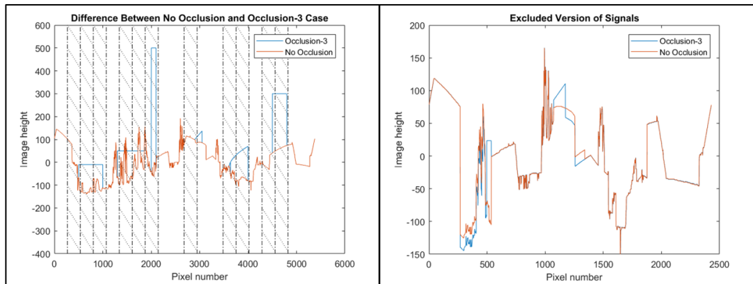
Figure 5.34. Occlusion-3 and Excluded Version of Skyline Signal “T(Diag1,5,NoLeaves-Noon)”
