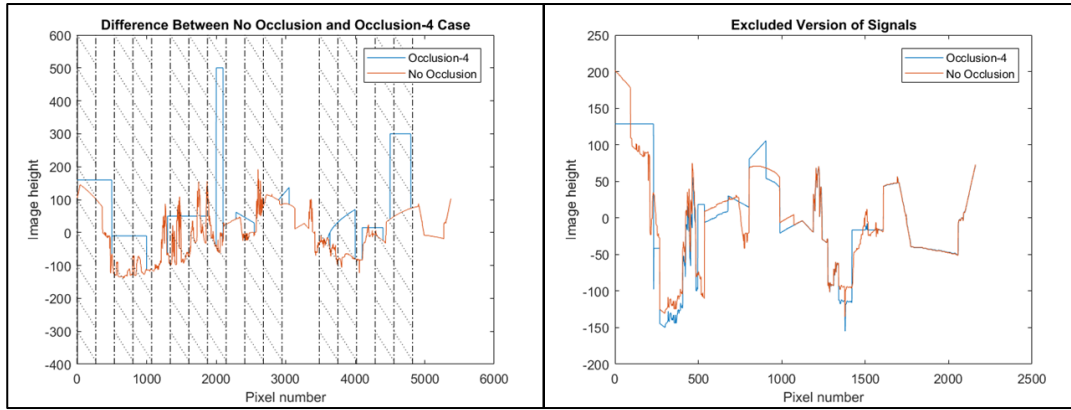
Figure 5.35. Occlusion-4 and Excluded Version of Skyline Signal
