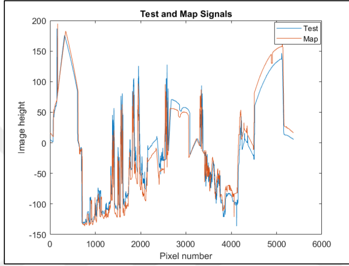
Figure 4.6. Test and Map Skyline Signals
