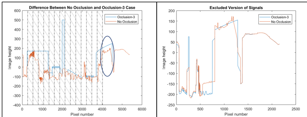
Figure 5.28. Occlusion-3 and Excluded Version of Skyline Signal “K(Diag1,5,Leaves-Sunrise)”
