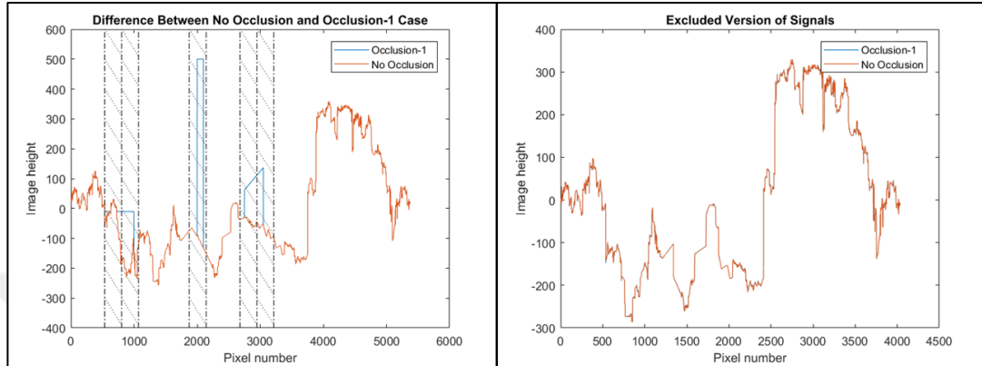
Figure 5.23. Occlusion and Excluded Version of Skyline Signal “B(Diag1,5,NoLeaves-Noon)”
