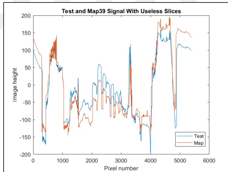
Figure 5.41. Skyline Signals of "K(VertR,5,Leaves-Cloudy)" and "K(Map,39,Leaves-Sunrise)"
