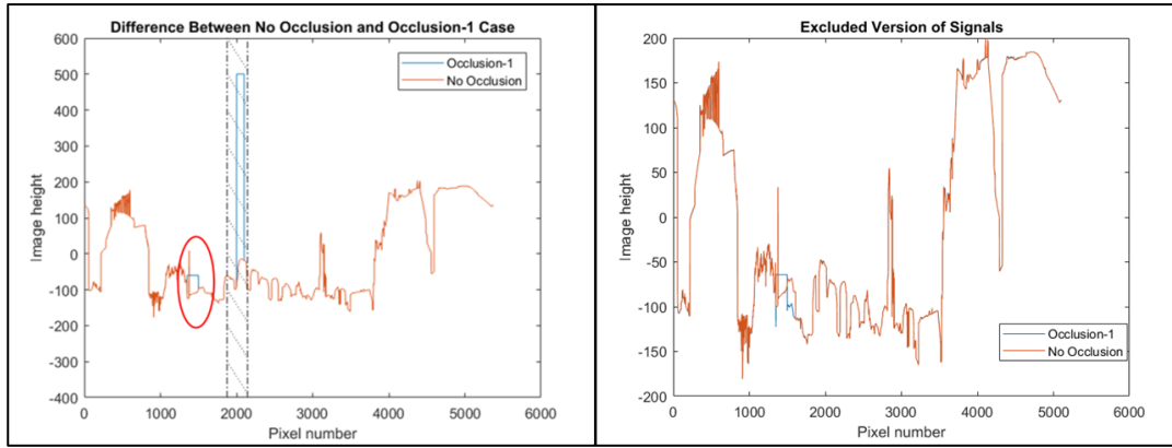
Figure 5.26. Occlusion-1 and Excluded Version of Skyline Signal “K(Diag1,5,Leaves-Sunrise)”
