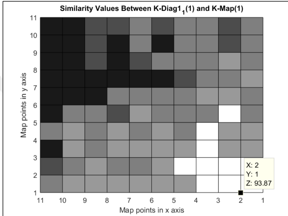
Figure 5.42. Localization of “K(Diag1,1,Leaves-Sunrise)” with “K(Map,Leaves-Sunrise)”
