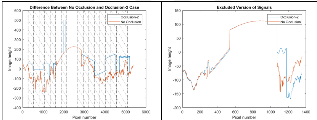
Figure 5.25. Occlusion-2 and Excluded Version of Skyline Signal “G(Diag1,5,Leaves-Afternoon)”
