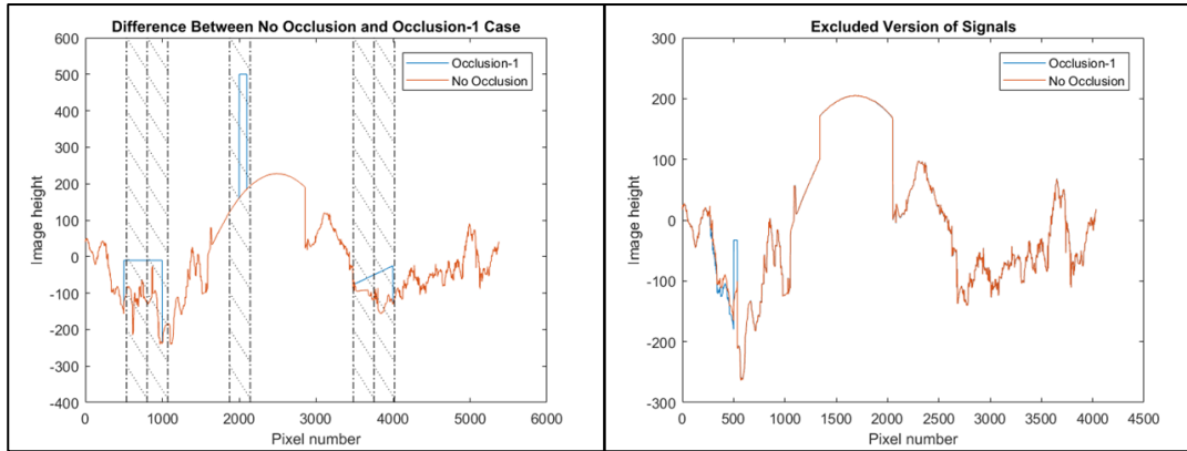
Figure 5.24. Occlusion-1 and Excluded Version of Skyline Signal “G(Diag1,5,Leaves-Afternoon)”
