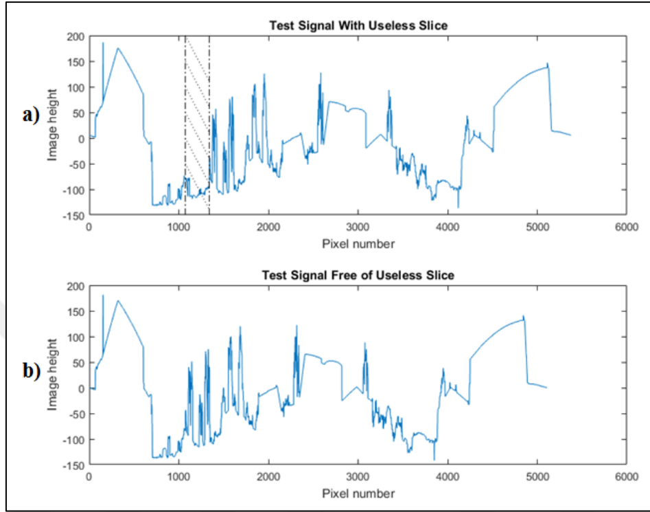
Figure 4.15. a) Test Signal with Soon-to-be Eliminated Unusable Slice b) Test Signal without the Unusable Slice
