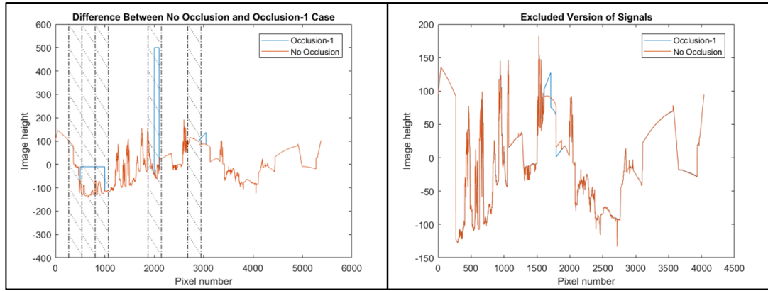
Figure 5.32. Occlusion-1 and Excluded Version of Skyline Signal “T(Diag1,5,NoLeaves-Noon)”
