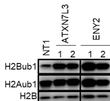
Figure 3.11. Western blot image showing H2Bub and H2Aub protein levels after ATXN7L3 or ENY2 knockouts in fibroblasts. H2B was used as a loading control.
