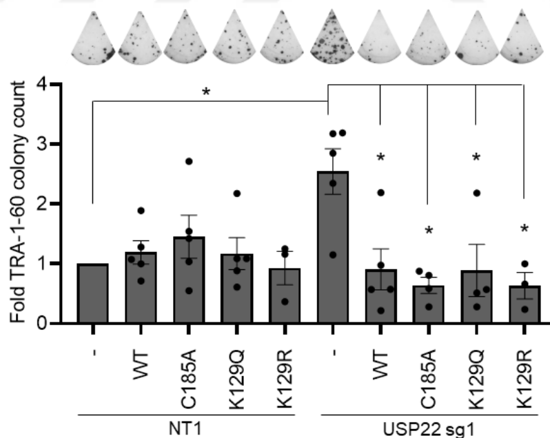
Figure 3.9. Fold change in reprogramming efficiency upon USP22 overexpression in both wild-type and USP22 knockout background. Error bars indicate the error of mean. n=3, independent experiments for KR mutations, n=4 for CA and KQ mutations in USP22 knockout background and n=5 for other comparisons. * Stand for p<0.05.
