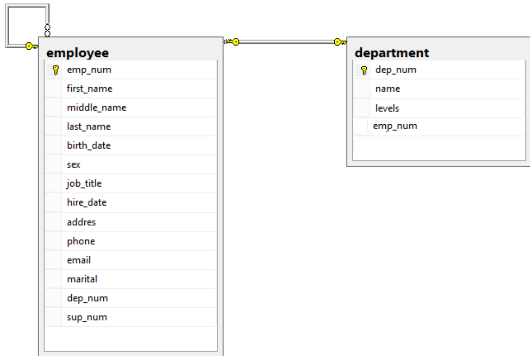
Figure 9 Relational mapping
