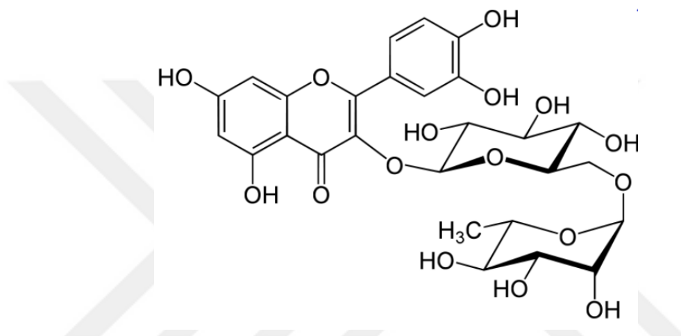
Figure 2.7. Molecular structure of Rutin
