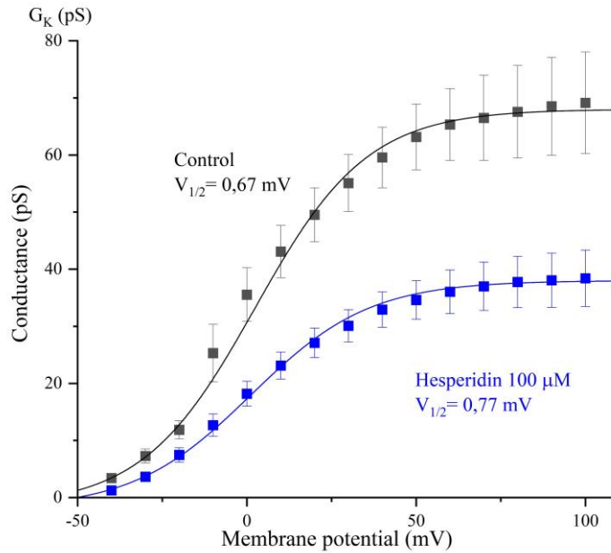
Figure 4.19. K^+ channels conductance in relation to membrane potential and from control DRG cells and after application of 100 \mu M of hesperidin showing 50% reduction in maximum conductance ( n= 10 ; P<0.05 ). and non-significant shift in the V_{1/2} value ( n= 10 ; P>0.05 ). Data are represented as mean values \pm S.E.M. ( n= 10 ; P>0.05 ).
