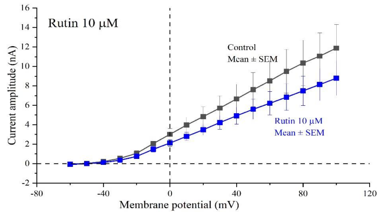
Figure 4.5. Graphic representation of mean values \pm SEM of the relation between membrane (mV) and outward K^+ current amplitudes (nA), from control cell and after application of 10 \mu M of rutin, with data showing 23% decrease of K^+ currents densities relatively to membrane potential, ( n = 6 ; P < 0.05 ).
