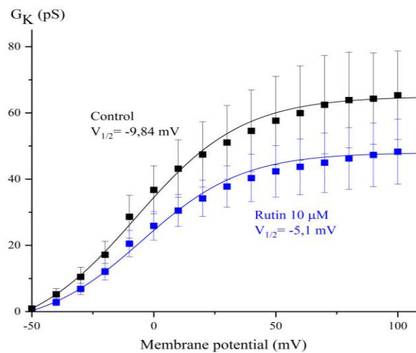
Figure 4.6. K^+ channels conductance in relation to membrane potential and from control DRG cells and after application of 10 \mu M of rutin showing 25% reduction in maximum conductance. ( n = 6 ; P < 0.05 ). and non-significant shift in the V_{1/2} value ( P > 0.05 ). Data are represented as mean values \pm S.E.M.
