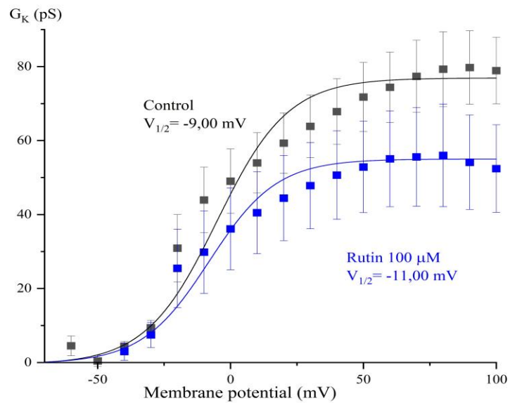
Figure 4.9. K^+ channels conductance in relation to membrane potential and from control DRG cells and after application of 100 \mu M of rutin showing 30% reduction in maximum conductance ( n=6 ; P<0.05 ). and non-significant shift in the V_{1/2} value ( P>0.05 ), Data are represented as mean values \pm S.E.M.
