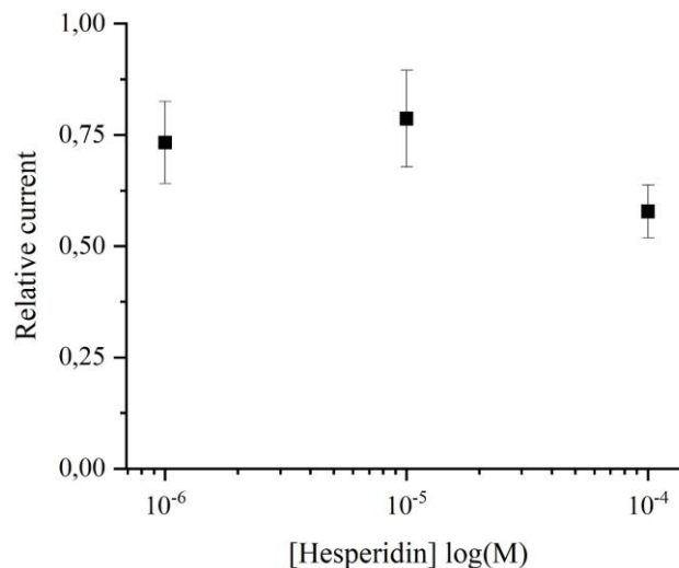
Figure 4.20. Dose related effect of hesperidin on relative K^+ current showing no dose related effect between the 3 doses of hesperidin (1 \mu M, 10 \mu M, 100 \mu M) investigated in the study.
