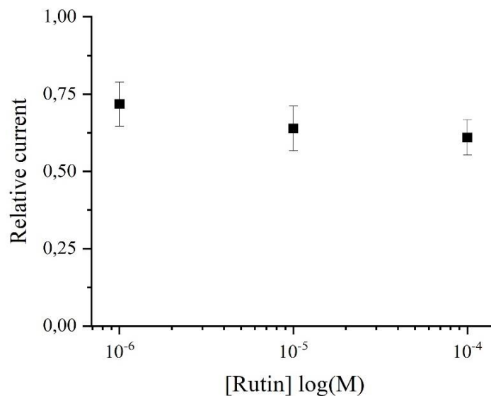
Figure 4.10. Dose related effect of rutin on relative K^+ current showing no dose related between the 3 doses of rutin (1 \mu M, 10 \mu M, 100 \mu M) investigated in the study.
