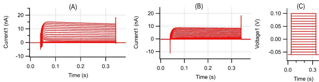
Figure 4.4. K^+ currents densities recorded from control cell (A) after injection of incremental depolarizing voltage steps (C), and K^+ currents densities after application of 10 \mu M dose of rutin (B) and execution of the same voltage protocol (C).
