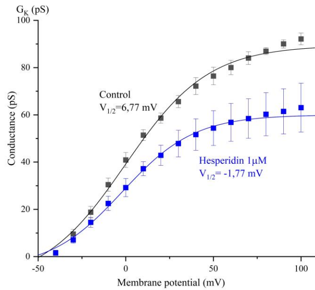
Figure 4.13. K^+ channels conductance in relation to membrane potential and from control cells and after application of 1 \mu M of hesperidin showing 36% reduction in maximum conductance ( n=5 , P<0.05 ), and significant shift in the V_{1/2} value ( n=5 ; P<0.05 ), Data are represented as mean values \pm S.E.M.
