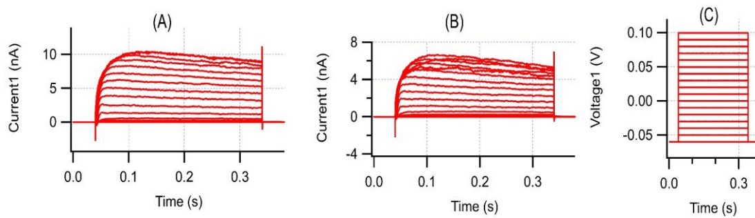
Figure 4.27. K^+ currents densities recorded from control cell (A) after injection of incremental depolarizing voltage steps (C), and K^+ currents densities after application of 100 \mu M dose of CGA (B) and execution of the same voltage protocol (C).
