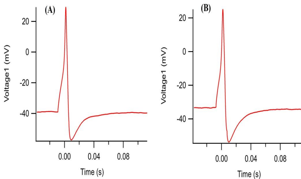
Figure 4.35. Control recording of elicited AP before (A) and after application of hesperidin at 100 \mu M dose (B).
