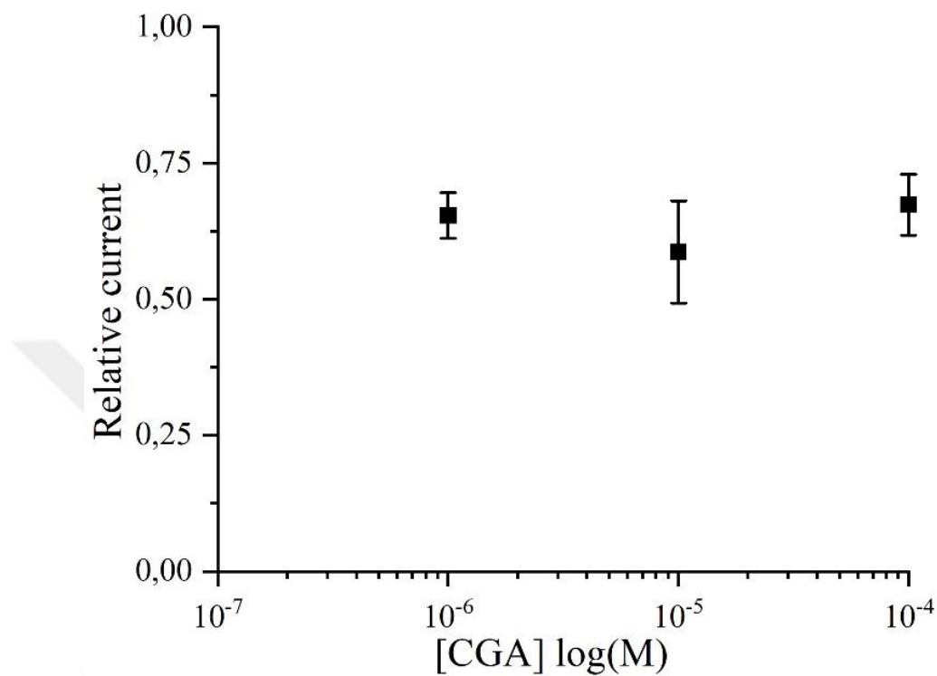
Figure 4.30. Dose related effect of CGA on relative K^+ current showing no dose related effect between the 3 doses of CGA (1 \mu M, 10 \mu M, 100 \mu M) investigated in the study.
