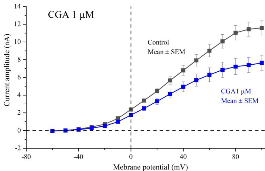
Figure 4.22. Graphic representation of mean values \pm SEM of the relation between membrane (mV) and outward \text{K}^+ current amplitudes (nA), from control cell and after application of 1 \mu\text{M} of CGA, with data showing 26% decrease of \text{K}^+ currents densities relatively to membrane potential. Data are represented as mean values \pm S.E.M. ( n = 6 ; P < 0.05 ).
