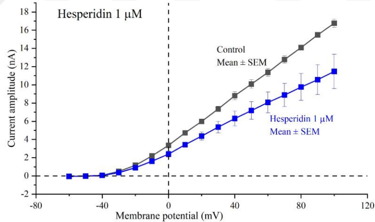
Figure 4.12. Graphic representation of mean values \pm SEM of the relation between membrane (mV) and outward \text{K}^+ current amplitudes (nA), from control cell and after application of 1 \mu\text{M} of hesperidin, with data showing 28% decrease of \text{K}^+ currents densities relatively to membrane potential. ( n = 5 ; P < 0.05 ).
