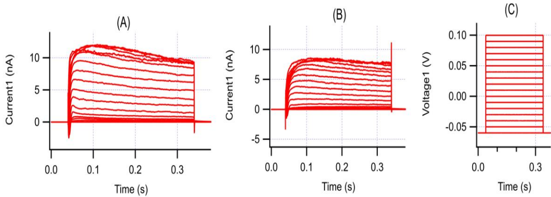
Figure 4.21. \text{K}^+ currents densities recorded from control cell (A) after injection of incremental depolarizing voltage steps (C), and \text{K}^+ currents densities after application of 1 \mu\text{M} dose of CGA (B) and execution of the same voltage protocol (C).
