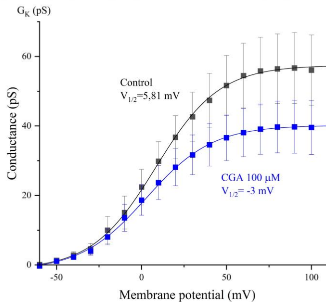
Figure 4.29. K^+ channels conductance in relation to membrane potential and from control DRG cells and after application of 100 \mu M of CGA showing 33% reduction in maximum conductance ( n=10 ; P>0.05 ) and non-significant shift in the V_{1/2} value ( n=10 ; P>0.05 ). Data are represented as mean values \pm S.E.M.).
