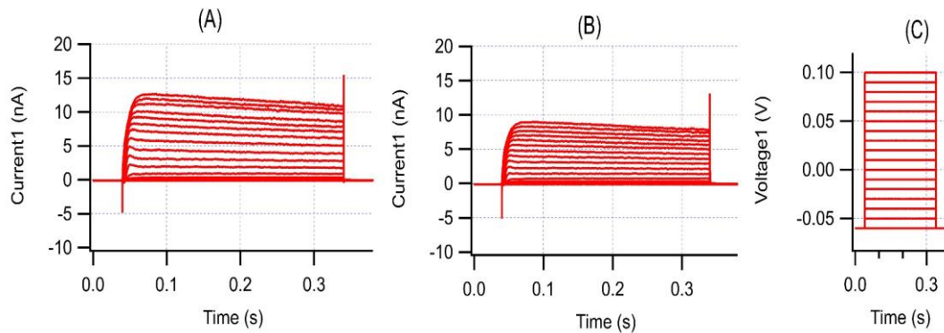
Figure 4.14. K^+ currents densities recorded from control cell (A) after injection of incremental depolarizing voltage steps (C), and K^+ currents densities after application of 10 \mu M dose of hesperidin (B) and execution of the same voltage protocol (C).
