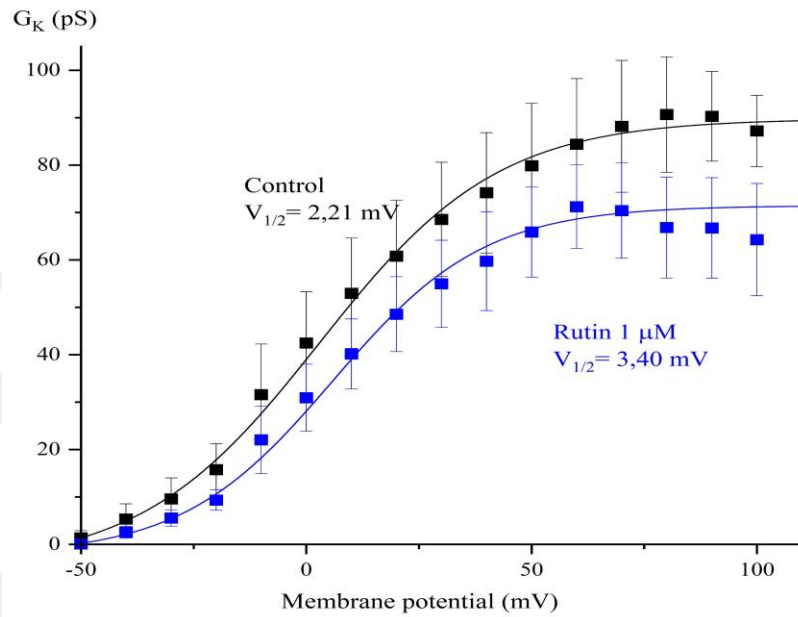
Figure 4.3. K^+ channels conductance in relation to membrane potential and from control DRG cells and after application of 1 \mu M of rutin showing 23% reduction in maximum conductance and non-significant shift in the V_{1/2} value ( n=5 ; P>0.05 ). Data are represented as mean values \pm S.E.M.
