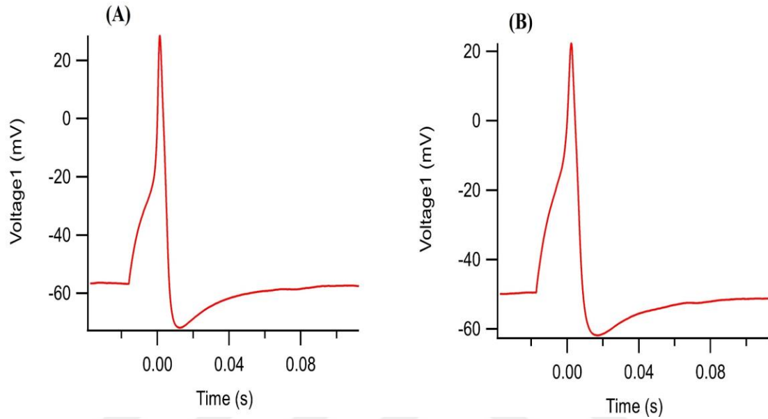
Figure 4.31. Control recording of elicited AP before (A) and after application of rutin at 1 \mu M dose (B).
