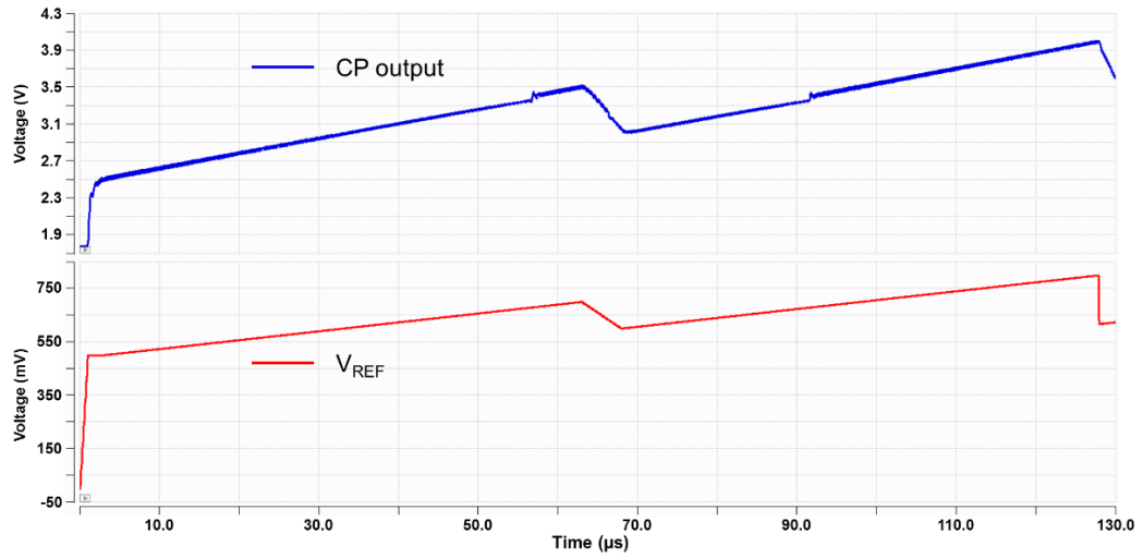
Figure 3.10. Transient simulation showing the regulation of the converter
