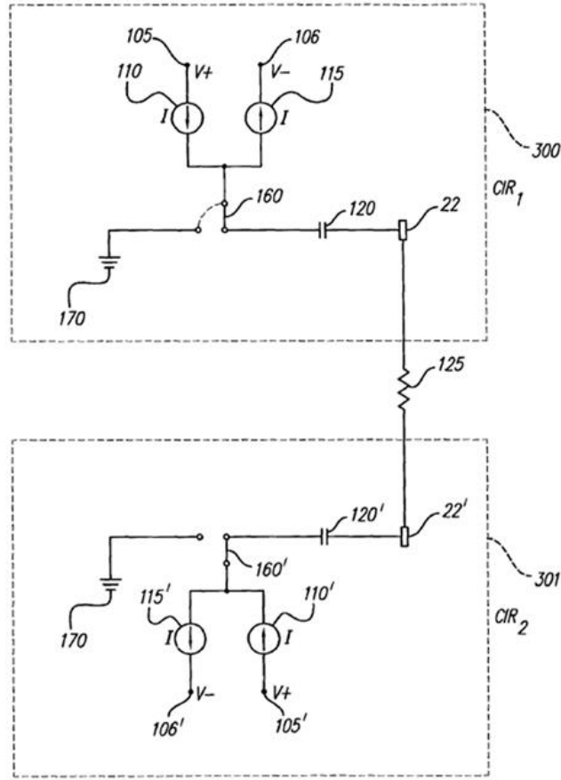
Figure 1.7. Schematic figure for the method presented in [32]
