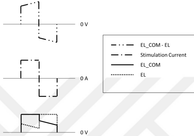
Figure 3.15. Example waveforms to stimulation current and electrode voltages
