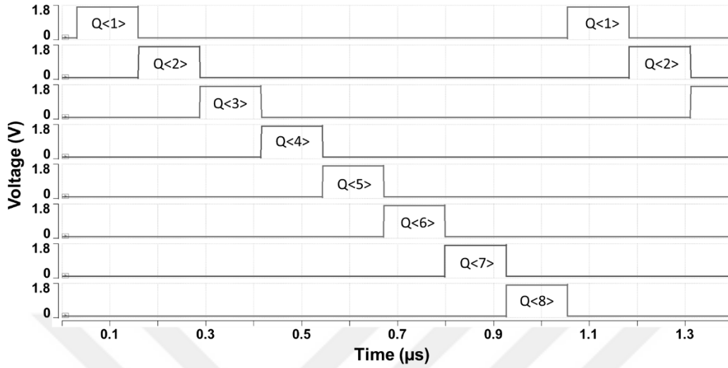
Figure 3.30. Simulation result showing operation of shift register
