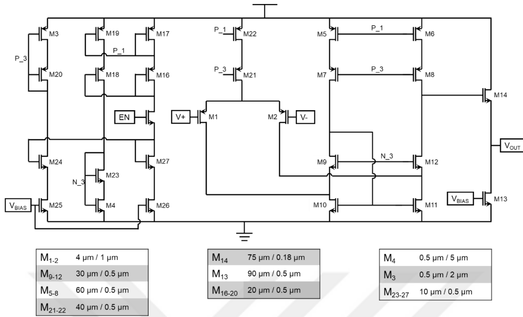
Figure 3.19. Folded cascode utilized as difference amplifier
