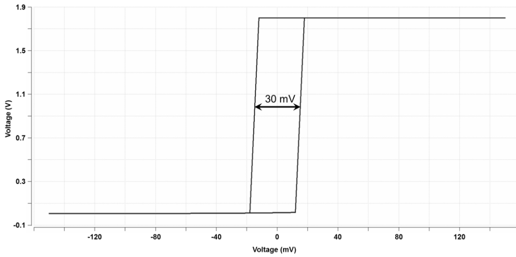
Figure 3.27. DC sweep simulation result of the hysteresis comparator for all corners
