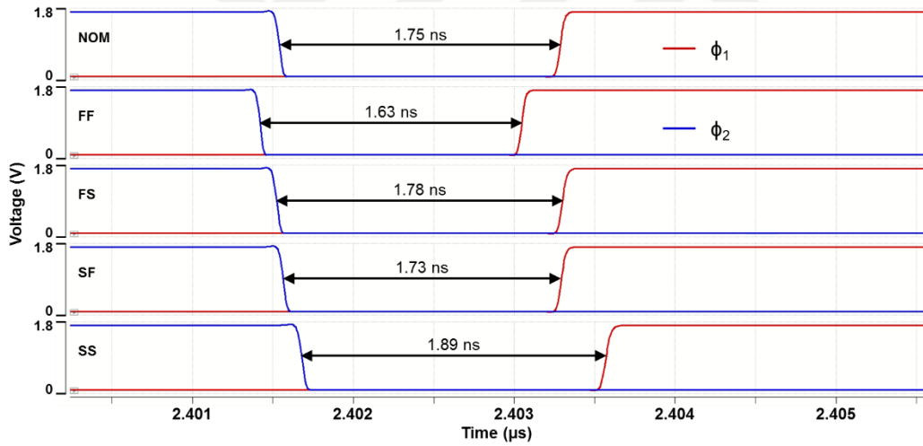
Figure 3.4. Dead-time variation with different corners for non-overlapping phases
