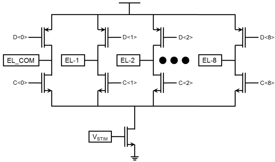
Figure 3.28. Schematic diagram of H-bridge used for biphasic pulse
