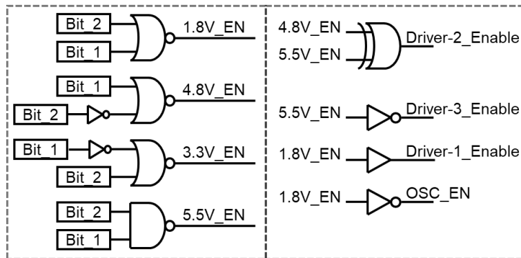
Figure 3.7. Simple logic used to control switched M1-4 and drivers
