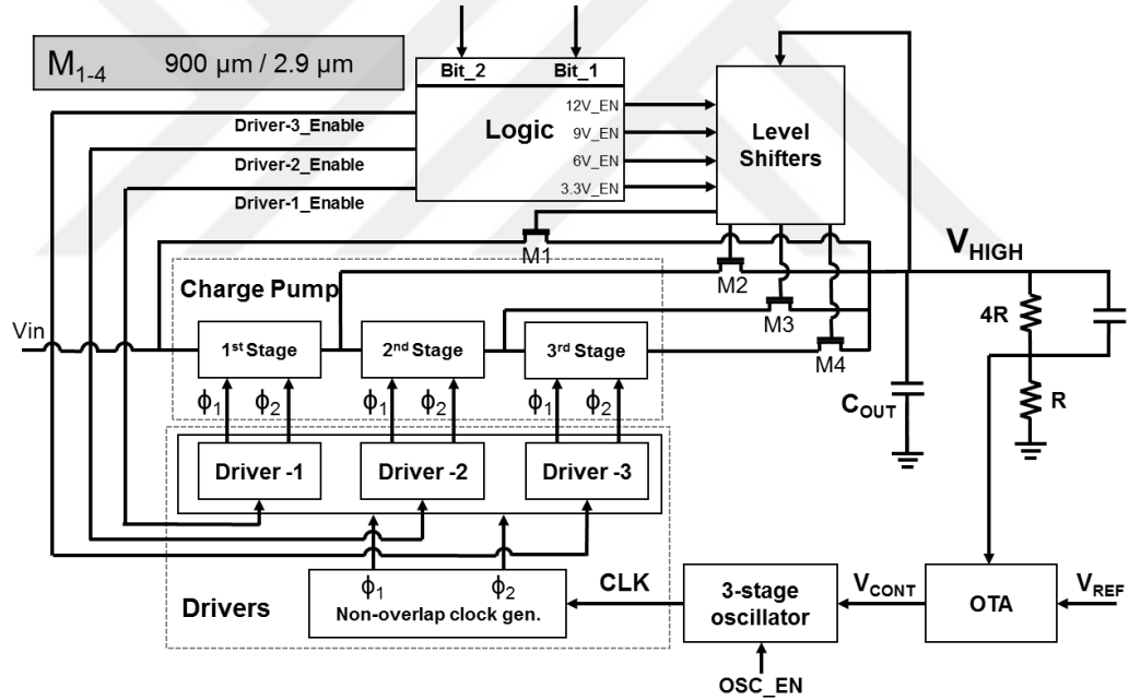
Figure 2.7. Block diagram of the converter
