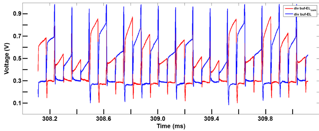
Figure 3.37. Scaled electrode voltages
