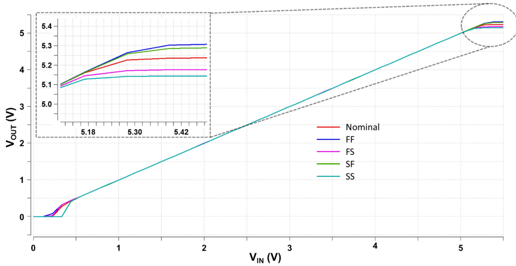
Figure 3.13. DC sweep simulation results of the HV buffer for all corners
