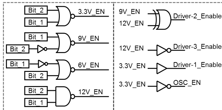
Figure 2.9. Simple logic used to control switched M1-4 and drivers
