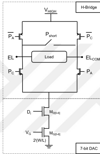
Figure 2.14. Schematic diagram of H-bridge and 7-bit DAC
