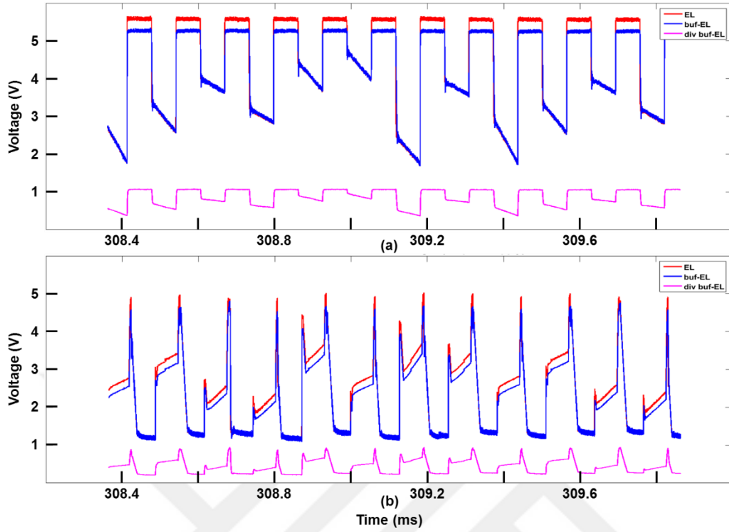
Figure 3.35. Input and output waveforms for HV buffers (EL - #) and after resistive division for (a) constant 5.5 V supply (b) adaptive supply
