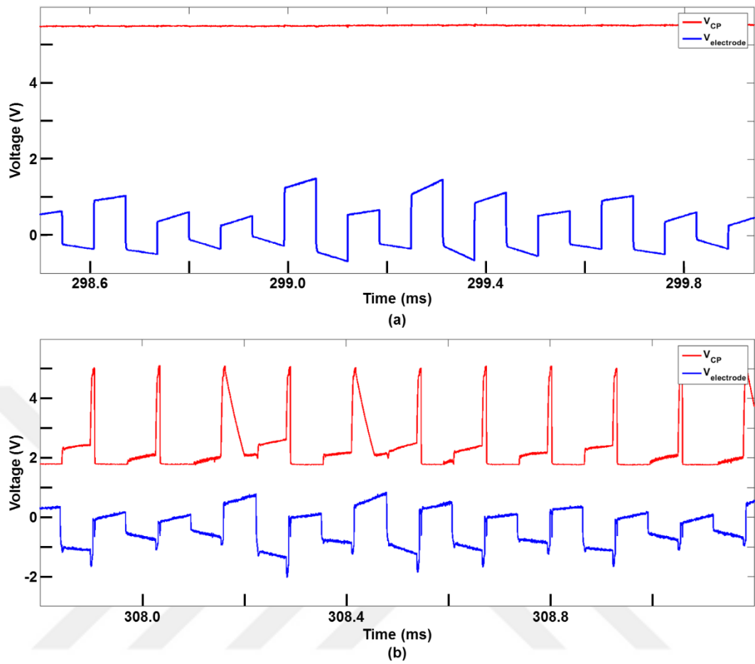
Figure 3.43. Electrode voltages and CP output for 140 \mu A stimulation current and loads in Table 3.2
