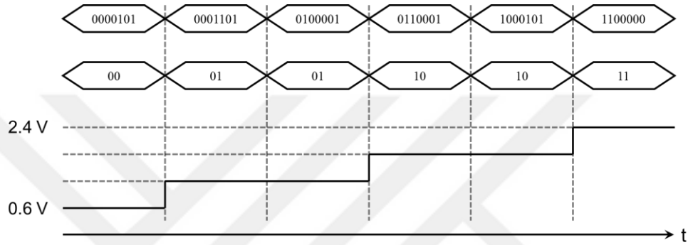
Figure 2.19. Illustration for the generation of the reference voltage
