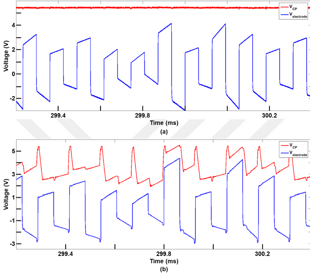
Figure 3.40. Electrode voltages and CP output for 450 \mu A and loads in Table 3.2 (a) constant mode (b) adaptive mode
