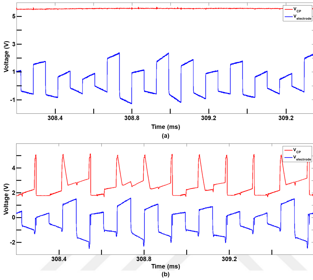
Figure 3.42. Electrode voltages and CP output for 230 \mu A and loads in Table 3.2 (a) constant mode (b) adaptive mode
