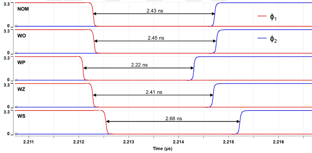
Figure 2.11. Dead-time variation with different corners for non-overlapping phases
