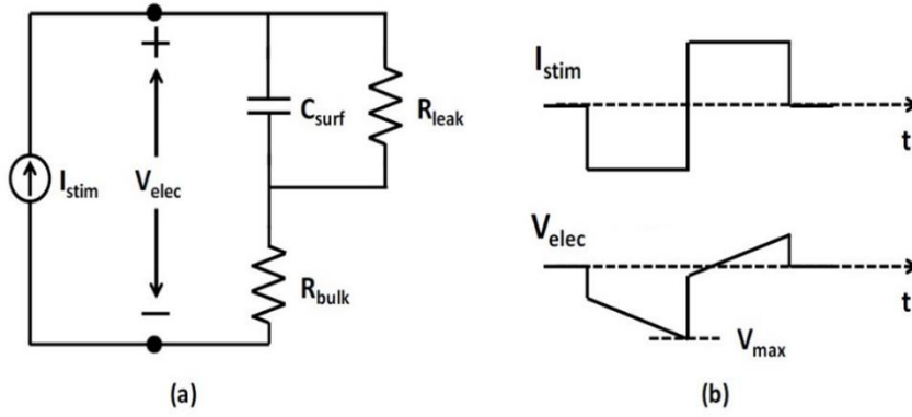
Figure 1.3. (a) Electrode impedance model (b) example stimulation current and resulting electrode potential difference
