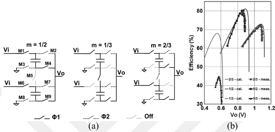
Figure 2.5. (a) Changing of converter topology in [40] (b) corresponding efficiency change
