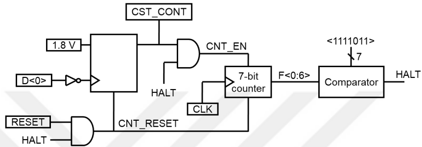
Figure 3.23. Circuitry used to generate CST_CONT
