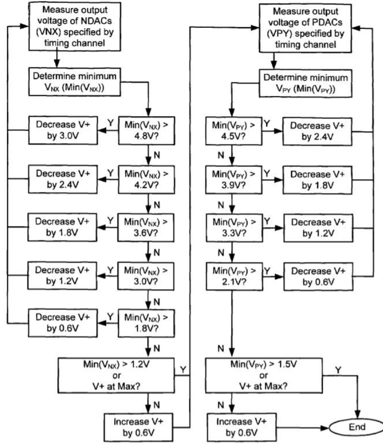
Figure 1.8. An example algorithm from the work in [49]
