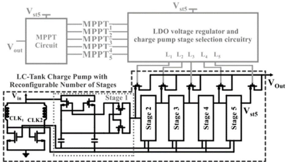
Figure 2.6. Charge pump structure in [50]
