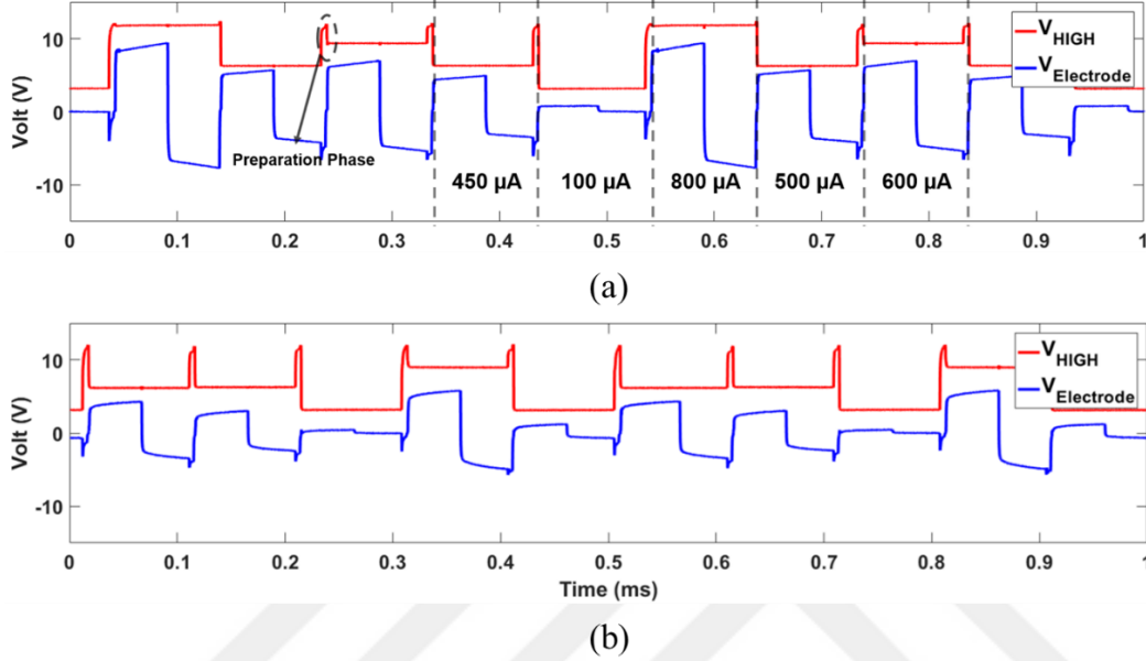
Figure 2.21. Electrode voltages and adaptive converter output for (a) artificial load (b) in-vitro
