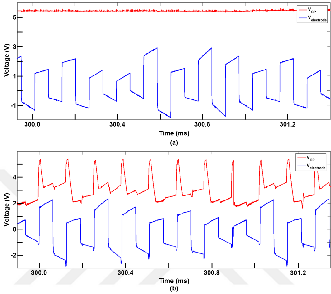
Figure 3.41. Electrode voltages and CP output for 300 \mu A and loads in Table 3.2 (a) constant mode (b) adaptive mode
