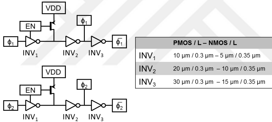
Figure 2.8. Schematic diagram of the drivers
