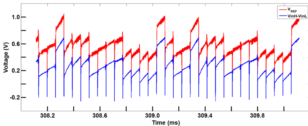
Figure 3.39. Input and output of difference amplifier
