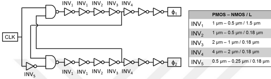
Figure 3.3. Schematic of the non-overlapping clock generator
