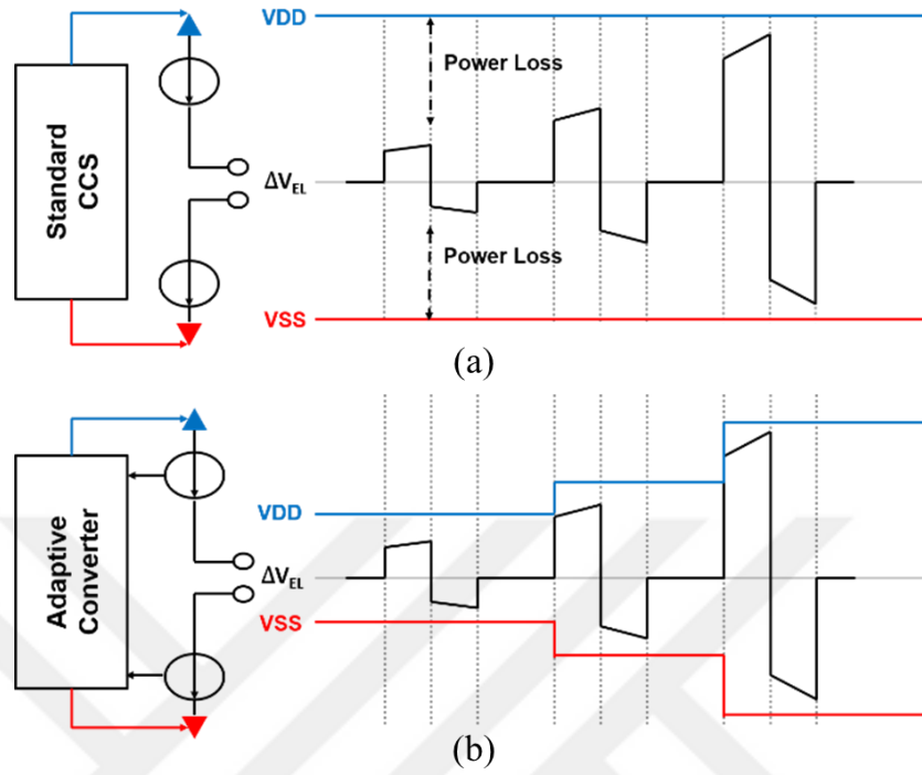
Figure 1.4. Example waveforms for constant current stimulator and (a) constant supply voltage (b) changing supply voltage
