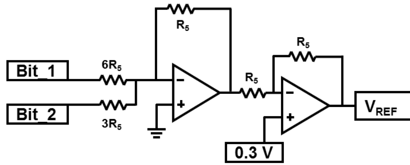
Figure 2.15. 2-bit DAC structure
