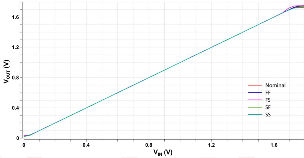
Figure 3.18. DC sweep simulation results of the LV buffer for all corners
