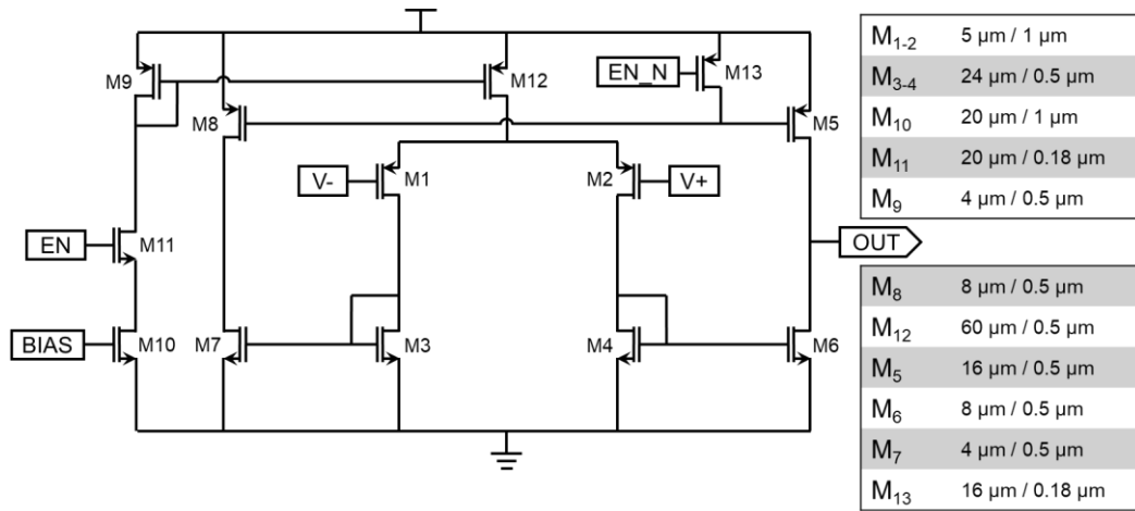
Figure 3.9. OTA used in PFM
