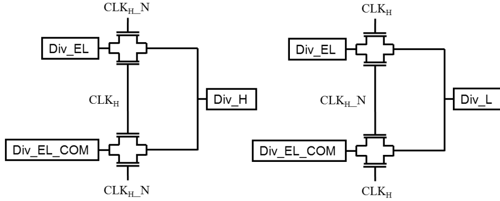
Figure 3.16. Circuitry to arrange magnitudes of electrodes
