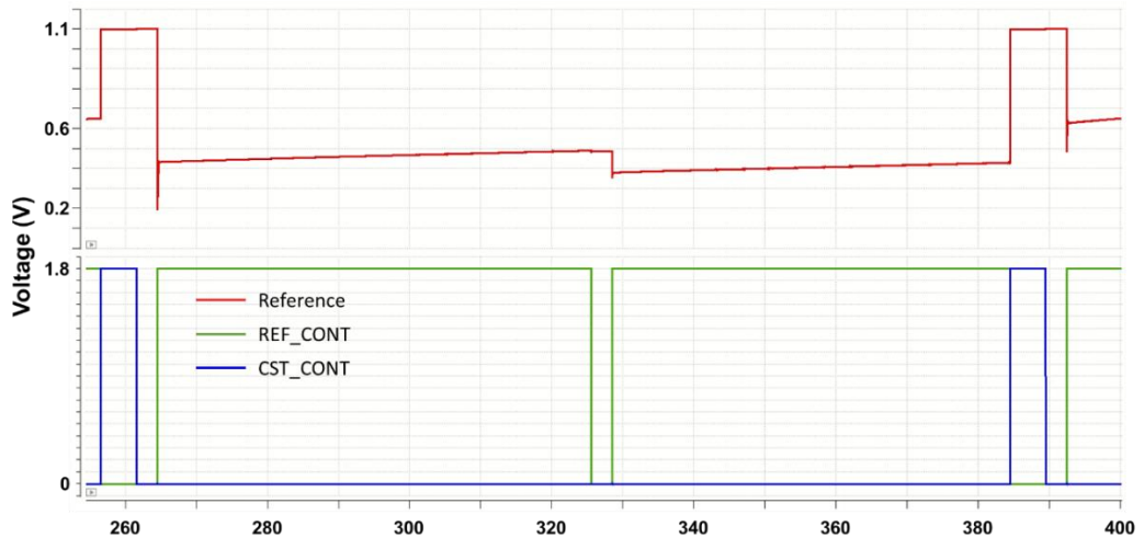
Figure 3.24. CST_CONT, REF_CONT and obtained reference voltage for the charge pump
