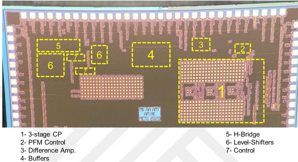
Figure 3.32. Micrograph of the design
