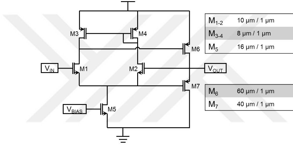
Figure 3.12. Schematic diagram of the HV buffer utilized to isolate the electrodes
