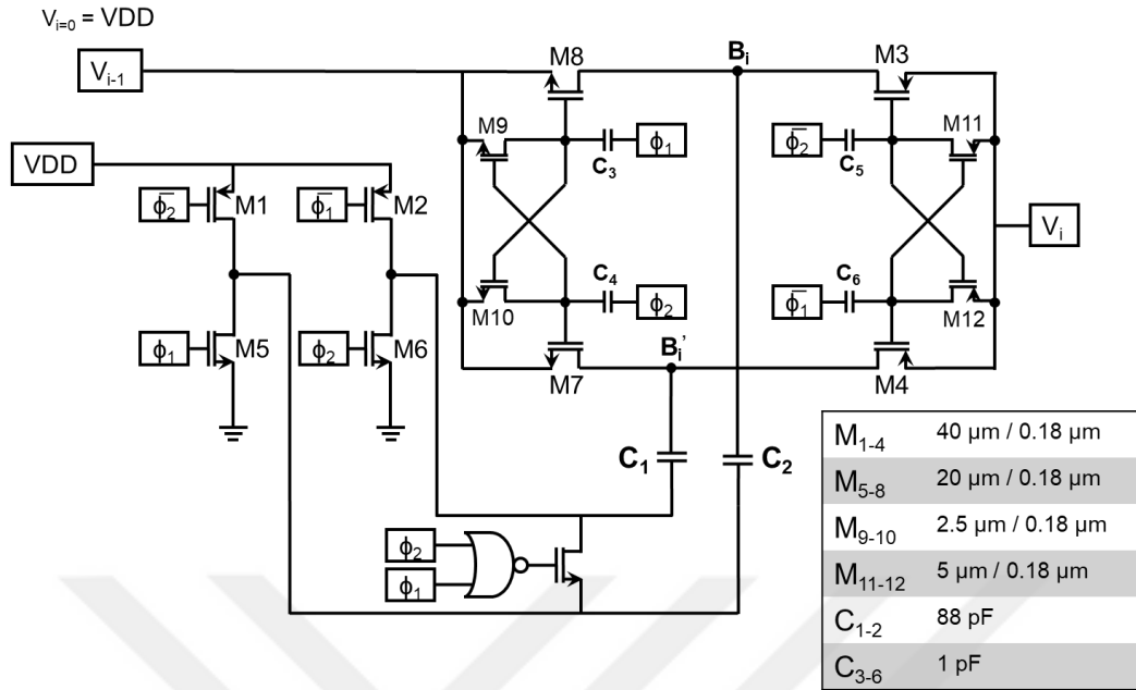
Figure 3.6. 1-stage charge pump schematic diagram
