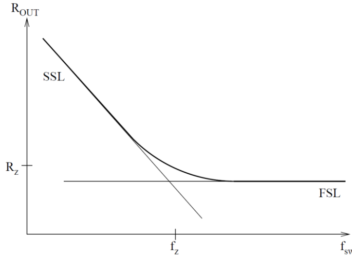
Figure 2.3. Graphical representation of the SC converter output resistance and its components
