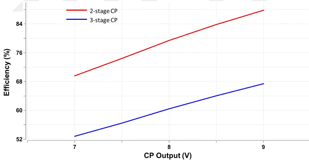
Figure 2.4. Efficiency values for simulated 2-stage and 3-stage charge pumps
