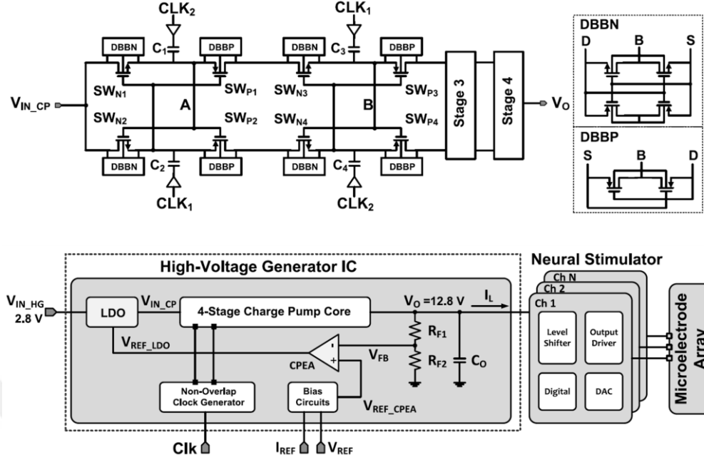
Figure 1.2. Charge pump and block diagram of the system in [13]
