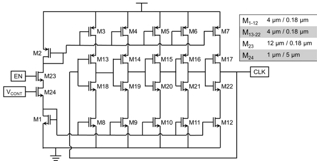
Figure 3.2. Schematic diagram of the 5-stage current starved VCO
