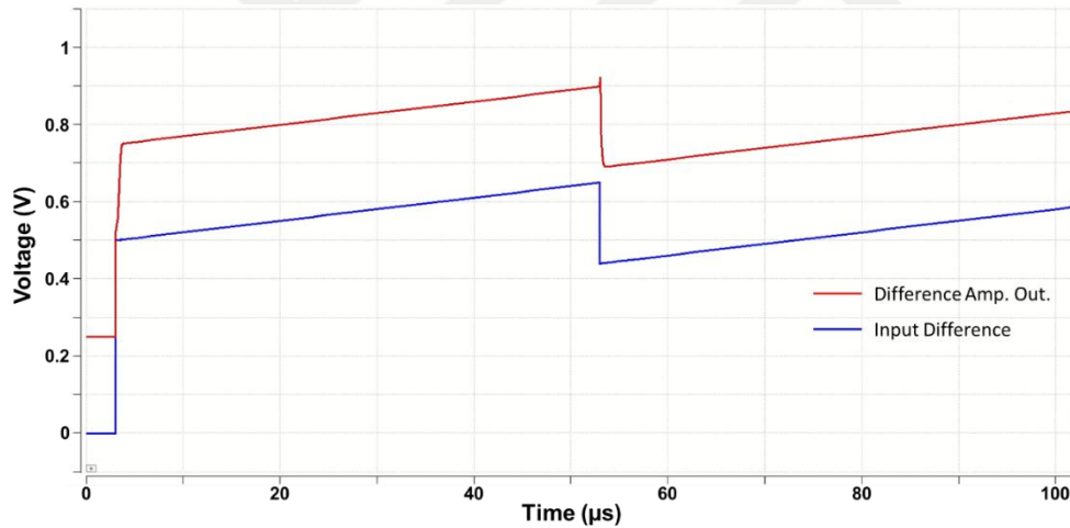
Figure 3.20. Difference amplifier input and output with offset
