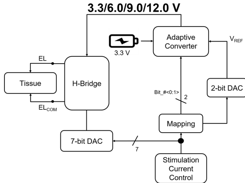
Figure 2.13. Adaptive converter system block diagram
