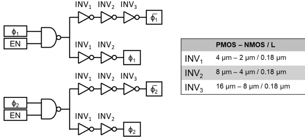
Figure 3.5. Schematic diagram of clock drivers
