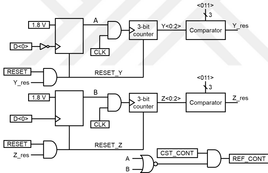
Figure 3.22. Circuitry used to generate REF_CONT
