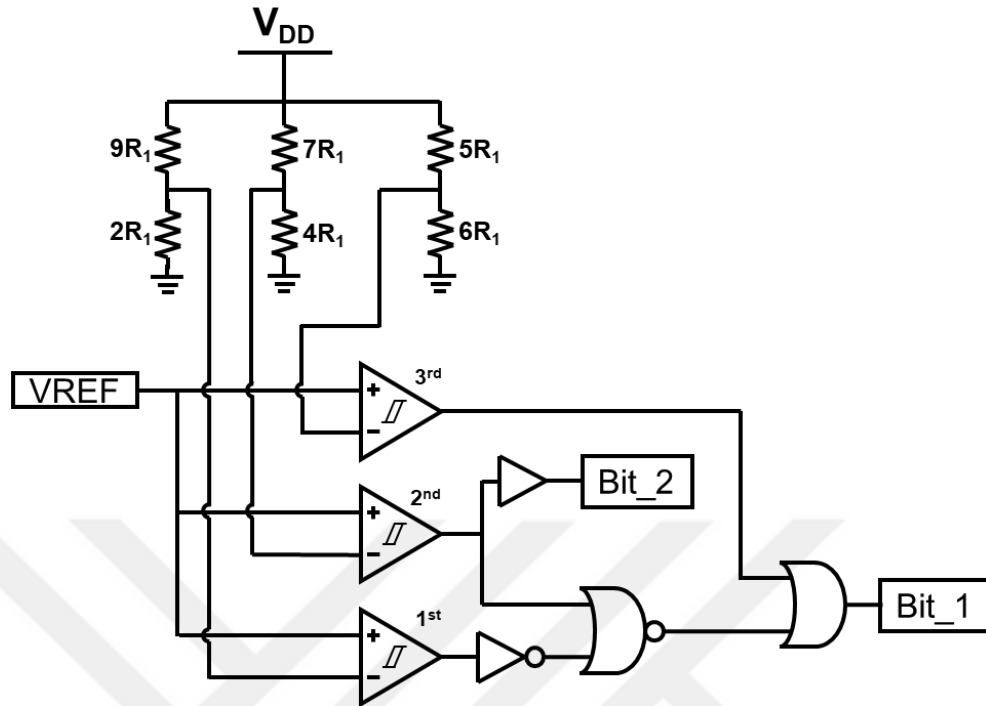
Figure 3.25. Flash ADC and creation of Bit_1 and Bit_2
