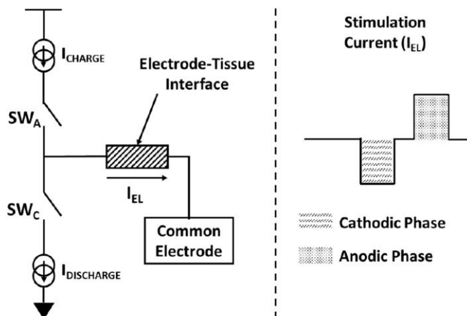
Figure 1.1. Simple illustration of CCS method [6]
