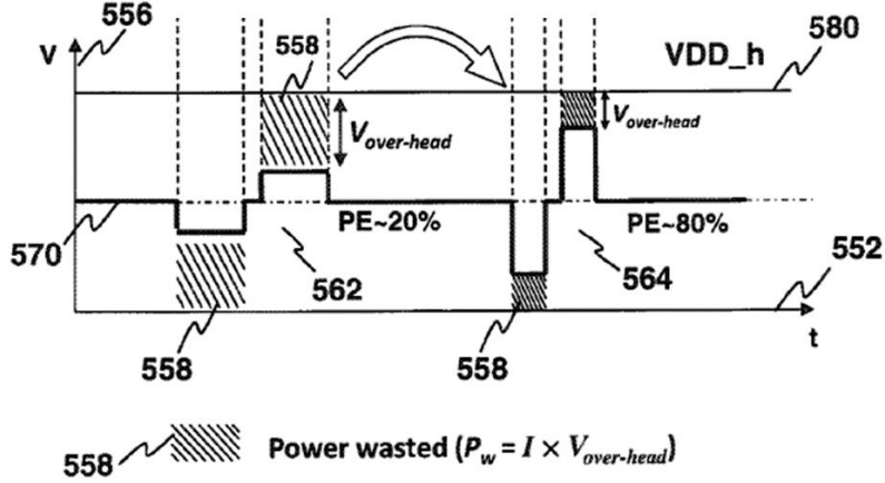
Figure 1.9. Example waveforms to modification performed on the stimulation current in [1]
