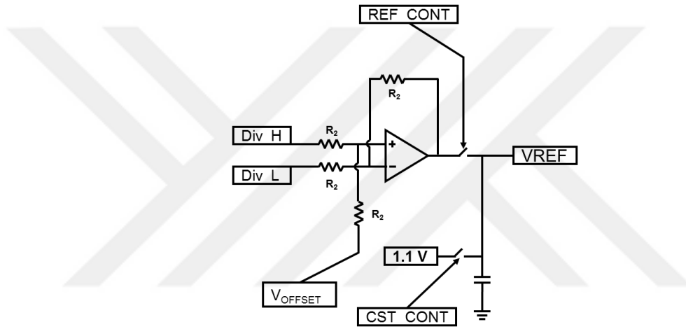
Figure 3.21. Circuit used to perform subtraction operation
