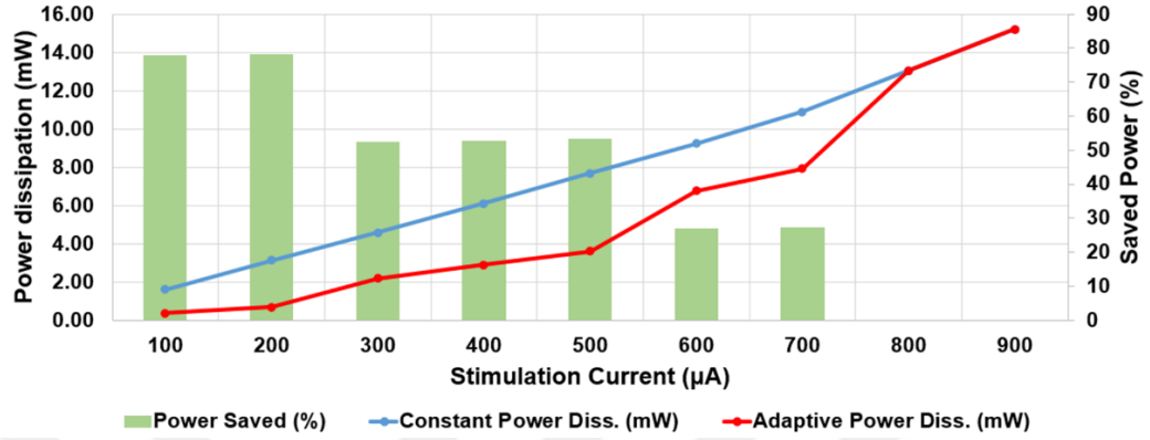
Figure 2.22. Power dissipation for constant and adaptive output configuration
