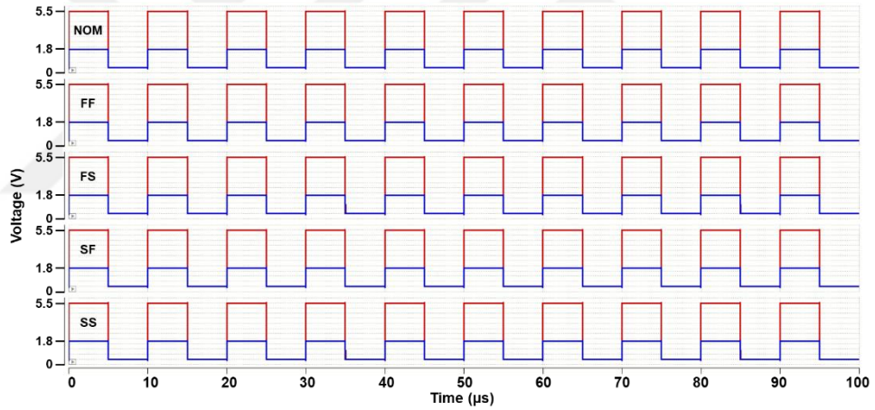
Figure 3.8. Level shifters operation for switches M1-4 for 1.8 V and 5.5 V supply
