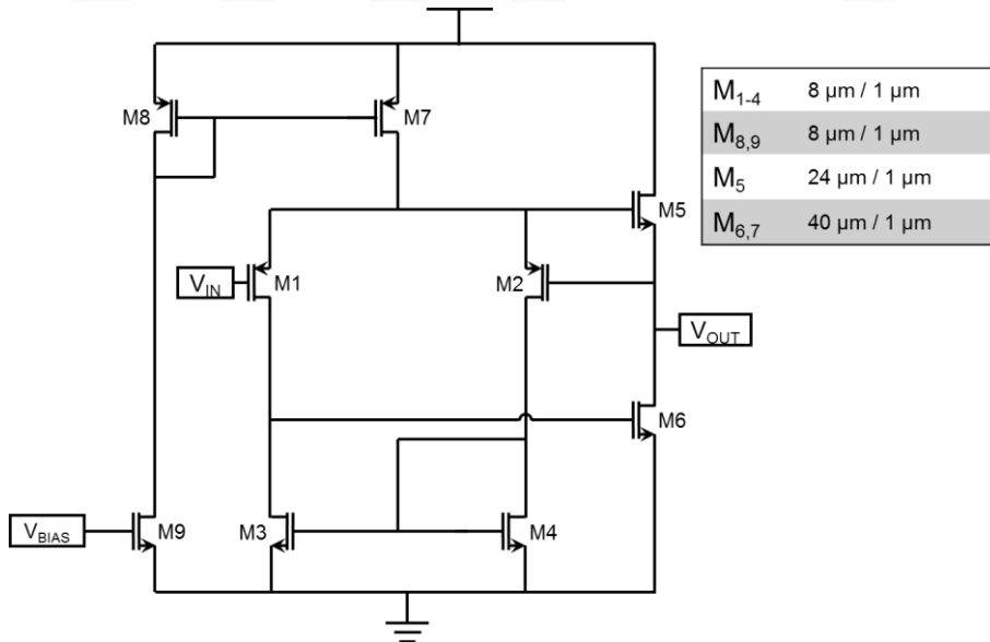
Figure 3.17. Schematic diagram of the used LV buffer
