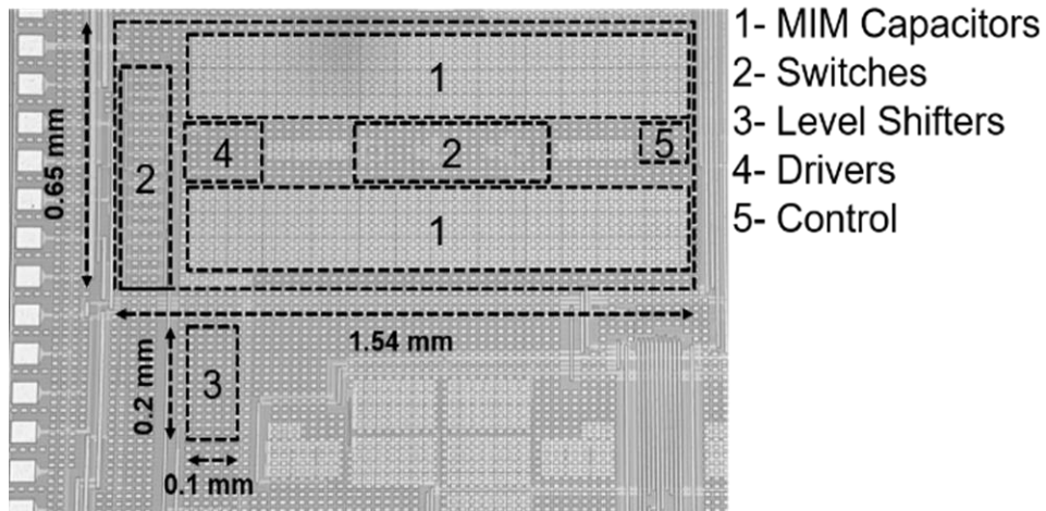
Figure 2.16. Die micrograph of the converter
