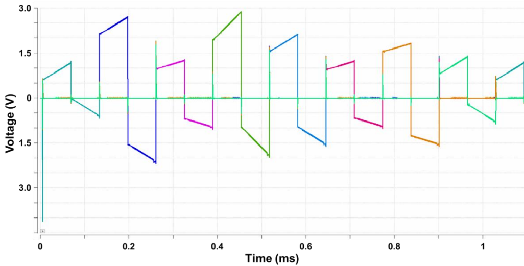
Figure 3.31. Example waveforms for a sequence of 8 stimulation electrodes
