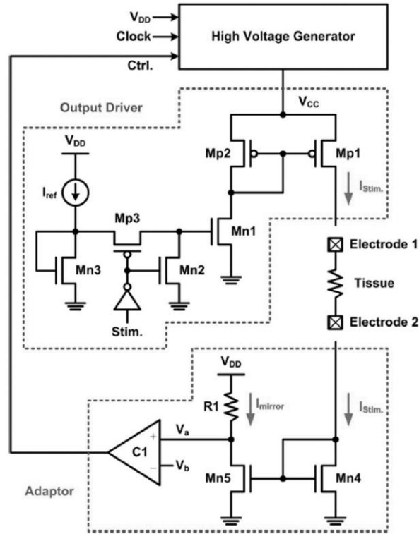
Figure 1.5. Block diagram of the system in [20]
