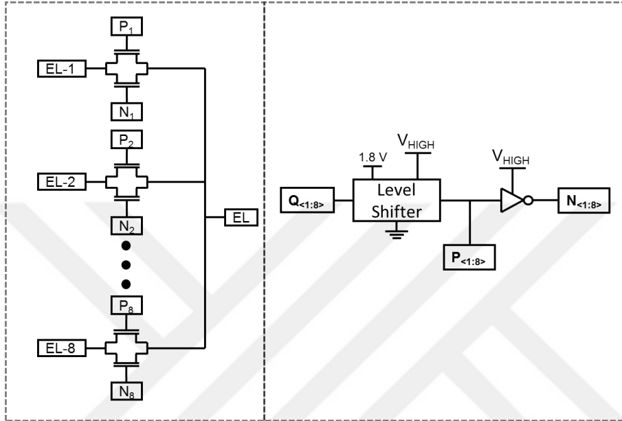
Figure 3.14. Switch matrix utilized to use one buffer with EL-1 to EL-8
