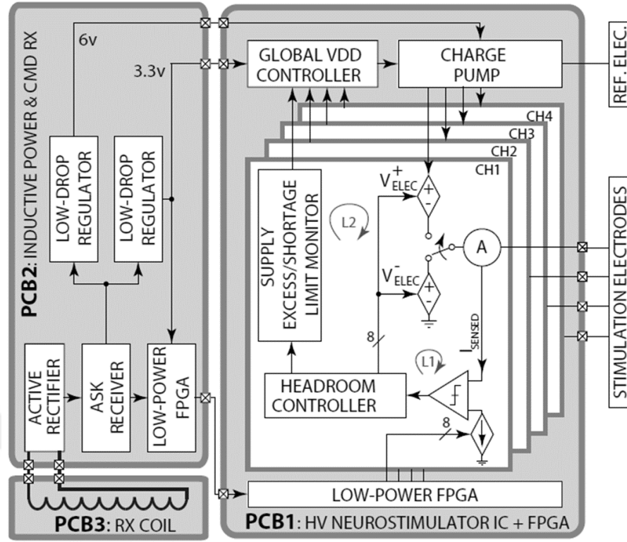
Figure 1.6. Block diagram of the system in [31]
