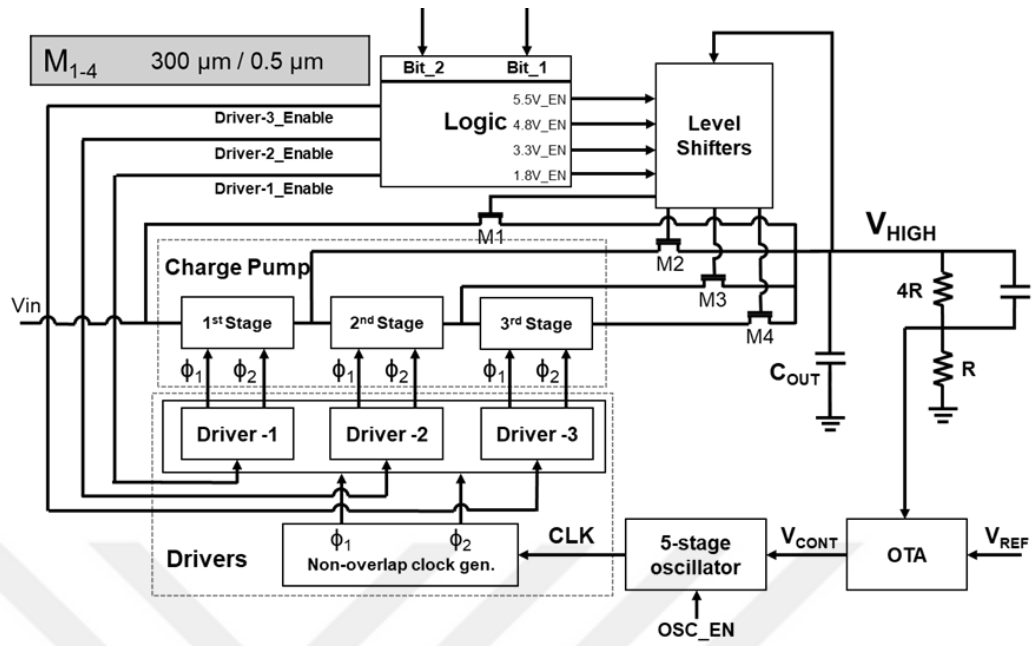
Figure 3.1. Block diagram of the charge pump side of the system
