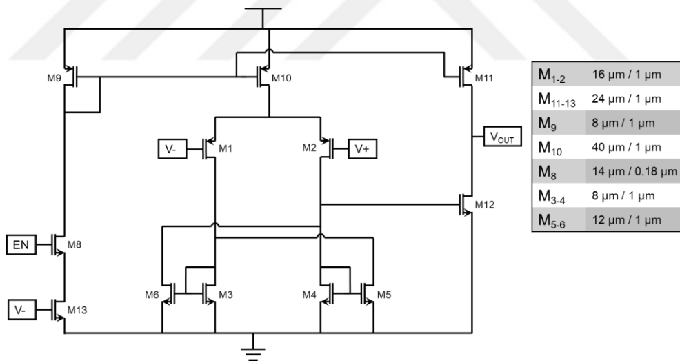
Figure 3.26. Hysteresis comparator used in the flash ADC
