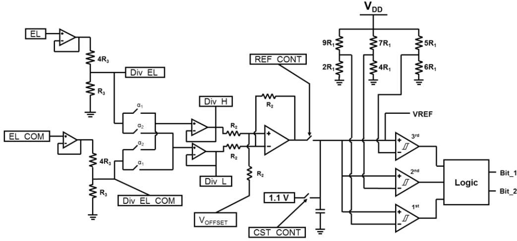
Figure 3.11. Block diagram of the voltage tracking circuitry
