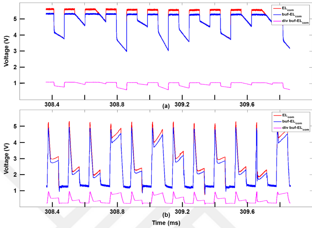
Figure 3.36. Input and output waveforms for HV buffers ( EL_{COM} ) and after resistive division for (a) constant 5.5 V supply (b) adaptive supply
