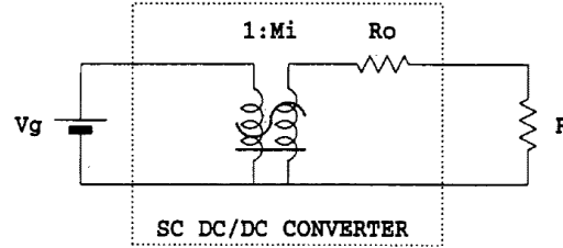
Figure 2.2. Model of switched-capacitor converter [41]
