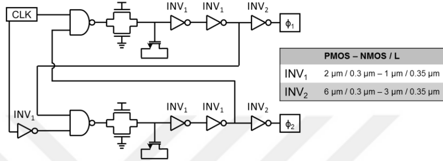
Figure 2.10. Schematic diagram of the non-overlapping clock generator
