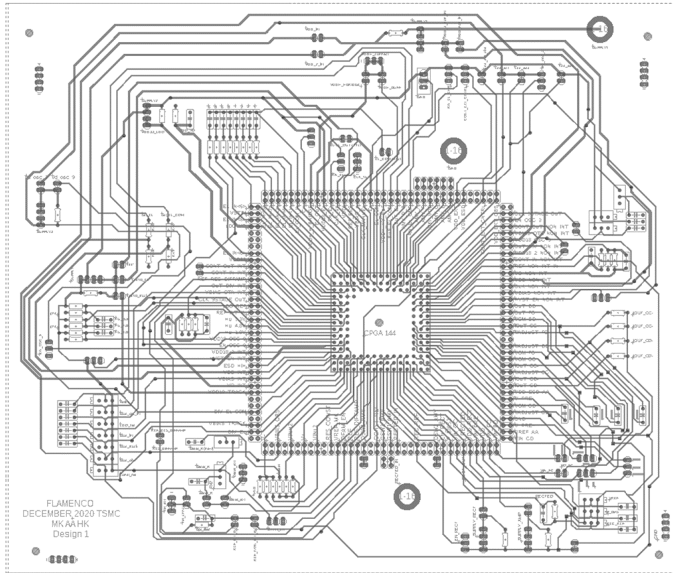
Figure 3.33. Adaptive converter test PCB
