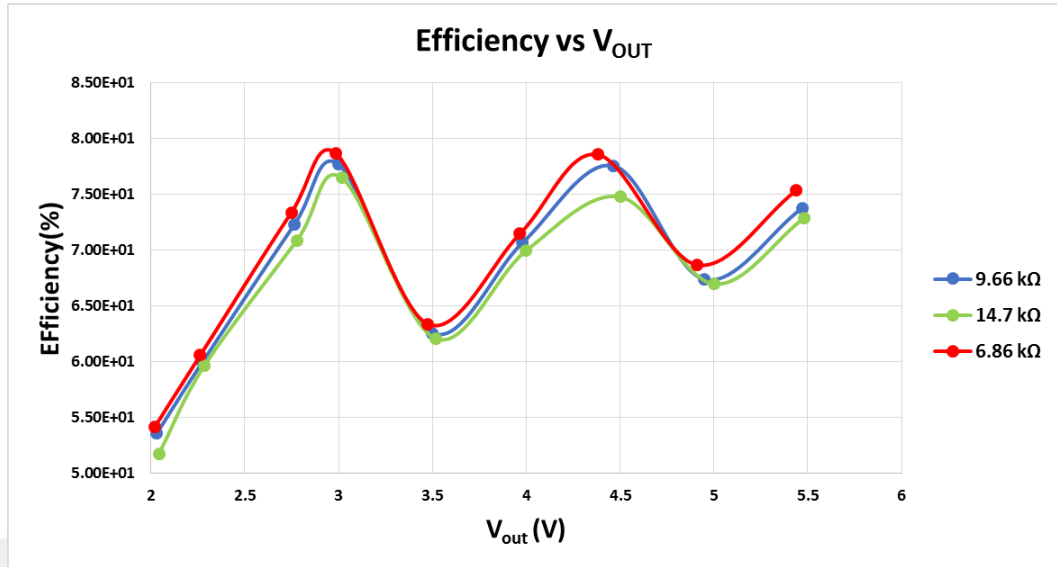
Figure 3.34. Efficiency of the step-up converter vs V_{OUT} and varying loads
