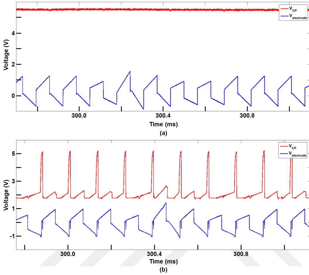
Figure 3.44. Electrode voltages and CP output for 470 \mu A and loads in Table 3.3 (a) constant mode (b) adaptive mode
