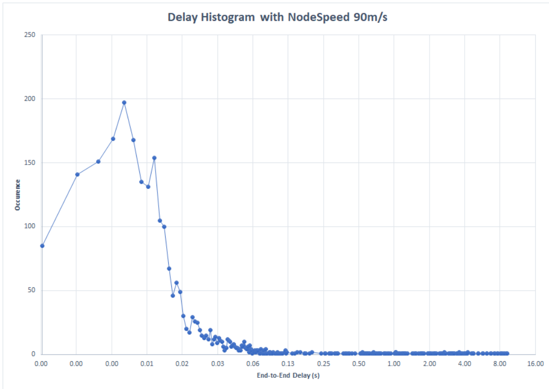
(a) Scenario-II Results: DelayHistogram when Node Speed is 90m/s
