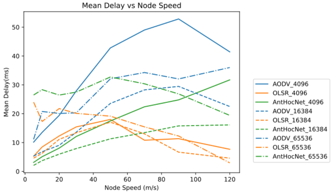
Figure 29: Scenario-II Results: End-to-End Delay vs Node Speed (EGM)
