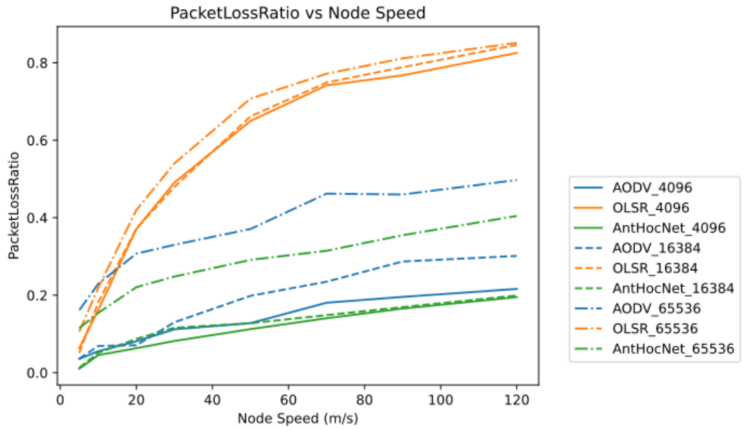
Figure 24: Scenario-II Results: Packet Loss Rate vs. Node Speed (PPRZM)
