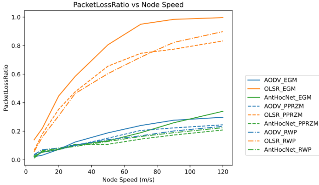
Figure 18: Scenario-I Results: Packet Loss Rate vs. Node Speed
