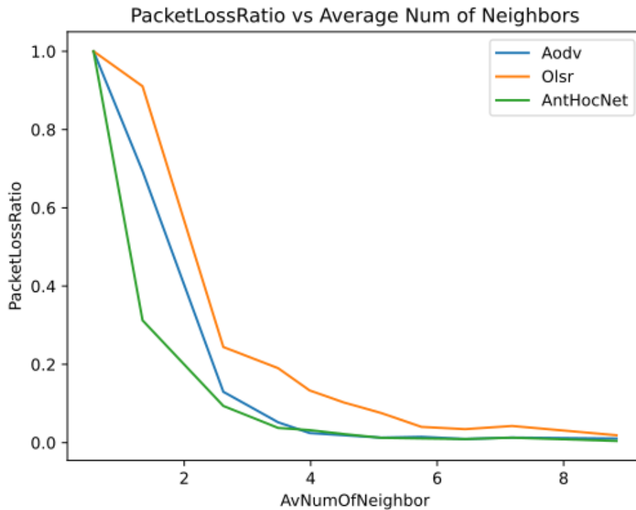
Figure 4: Packet Loss Ratio vs Average Number Of Neighbors, Node Speed = 5 m/s
