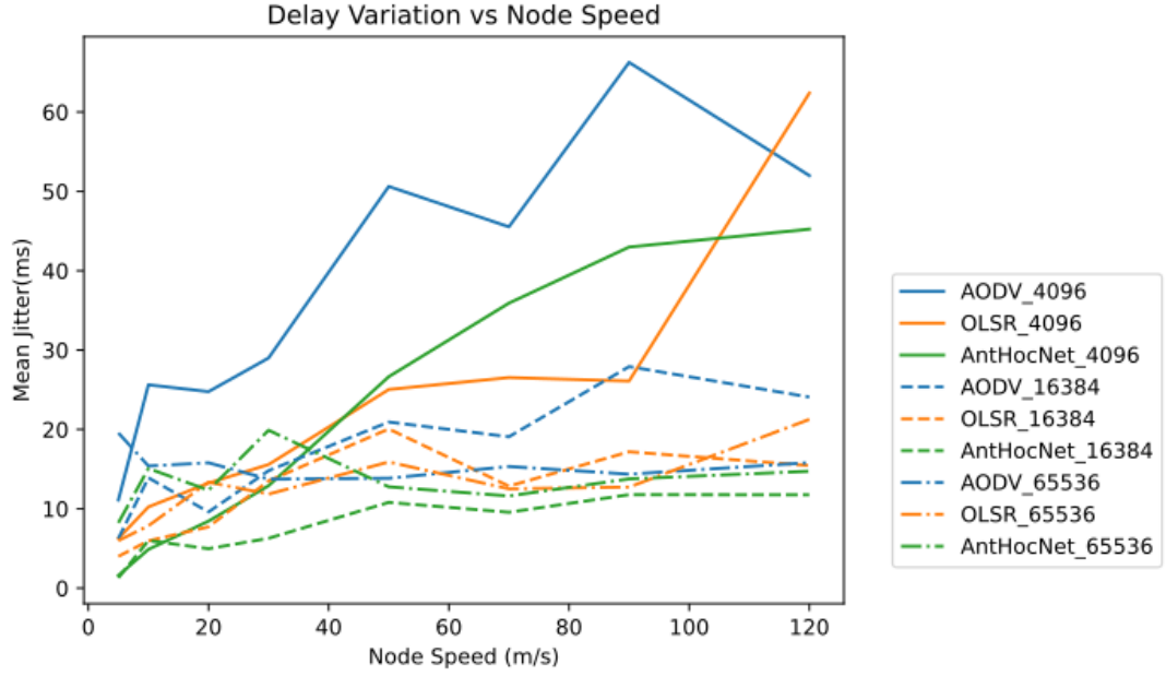
Figure 35: Scenario-II Results: End-to-End Delay Variation vs Node Speed (RWP)
