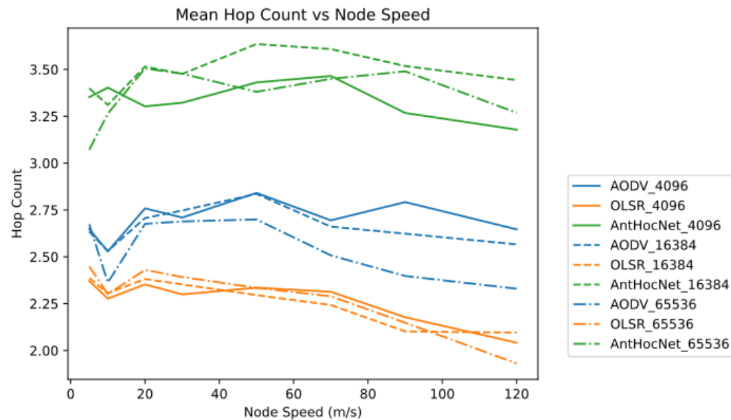
Figure 27: Scenario-II Results: Mean Hop Count vs Node Speed (PPRZM)
