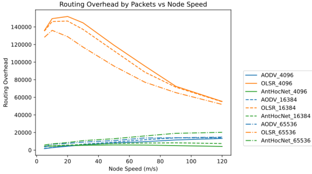
Figure 36: Scenario-II Results: Routing Overhead vs Node Speed (EGM)
