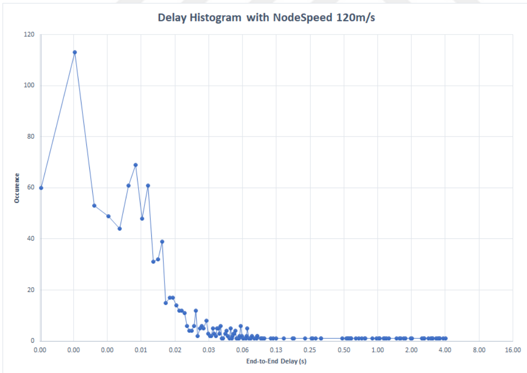
(b) Scenario-II Results: DelayHistogram when Node Speed is 120m/s
