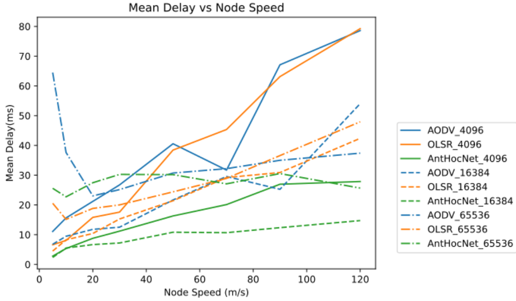
Figure 30: Scenario-II Results: End-to-End Delay vs Node Speed (PPRZM)
