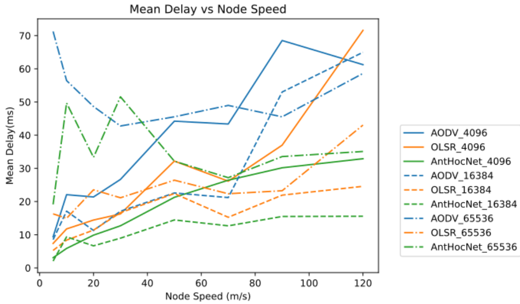
Figure 31: Scenario-II Results: End-to-End Delay vs Node Speed (RWP)
