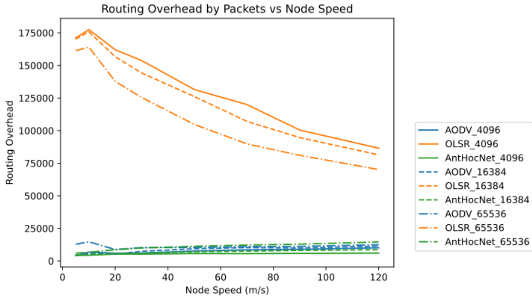
Figure 37: Scenario-II Results: Routing Overhead vs Node Speed (PPRZM)
