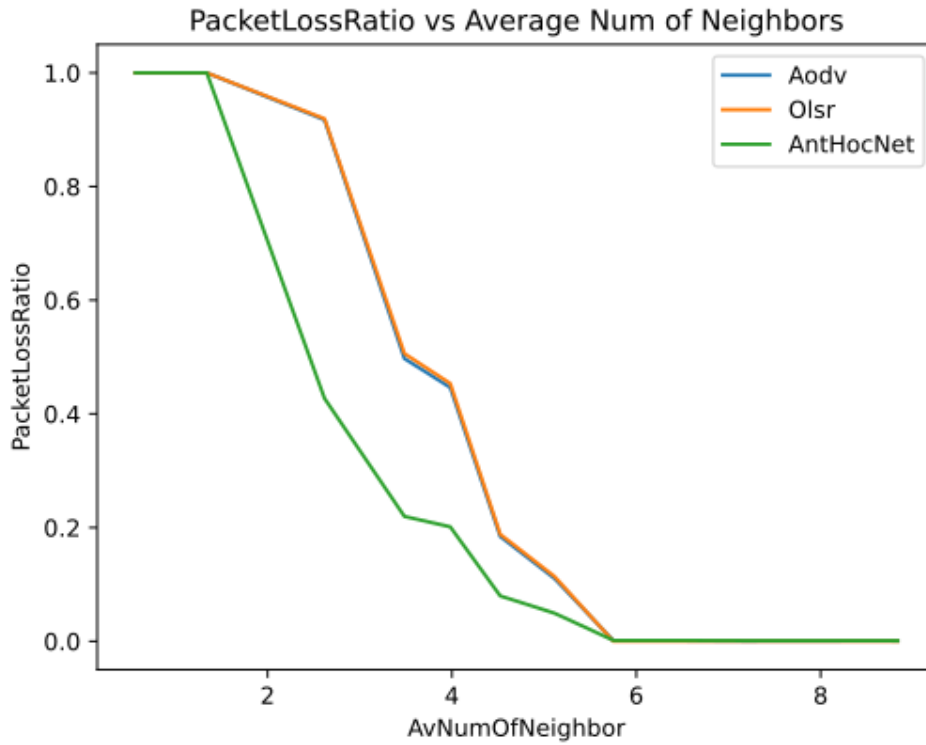
Figure 3: Packet Loss Ratio vs Average Number Of Neighbors, Node Speed = 0 m/s
