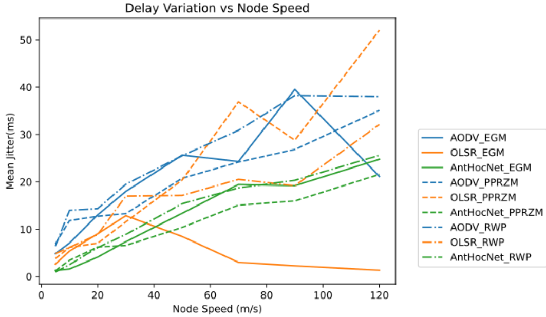
Figure 21: Scenario-I Results: Jitter vs. Node Speed
