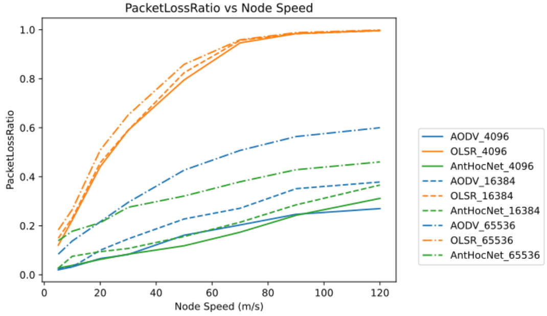
Figure 23: Scenario-II Results: Packet Loss Rate vs. Node Speed (EGM)
