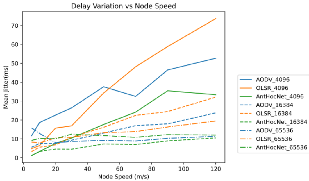
Figure 34: Scenario-II Results: End-to-End Delay Variation vs Node Speed (PPRZM)
