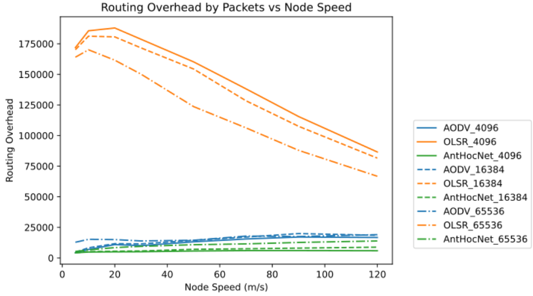
Figure 38: Scenario-II Results: Routing Overhead vs Node Speed (RWP)
