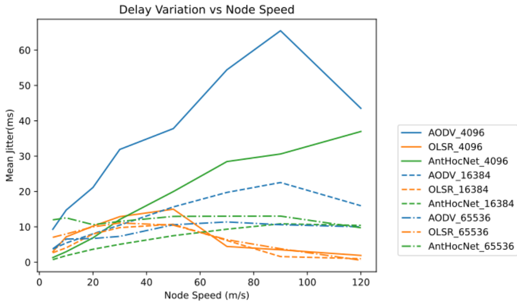
Figure 33: Scenario-II Results: End-to-End Delay Variation vs Node Speed (EGM)
