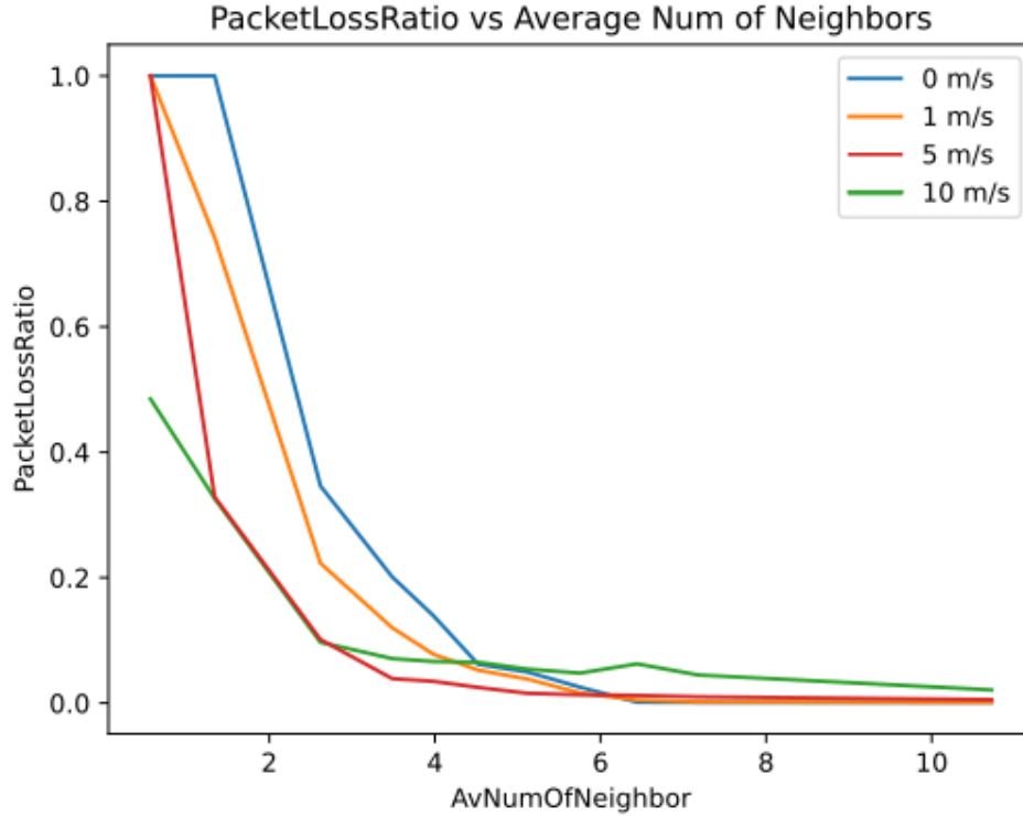
Figure 5: Packet Loss Ratio vs Average Number Of Neighbors, AntHocNet
