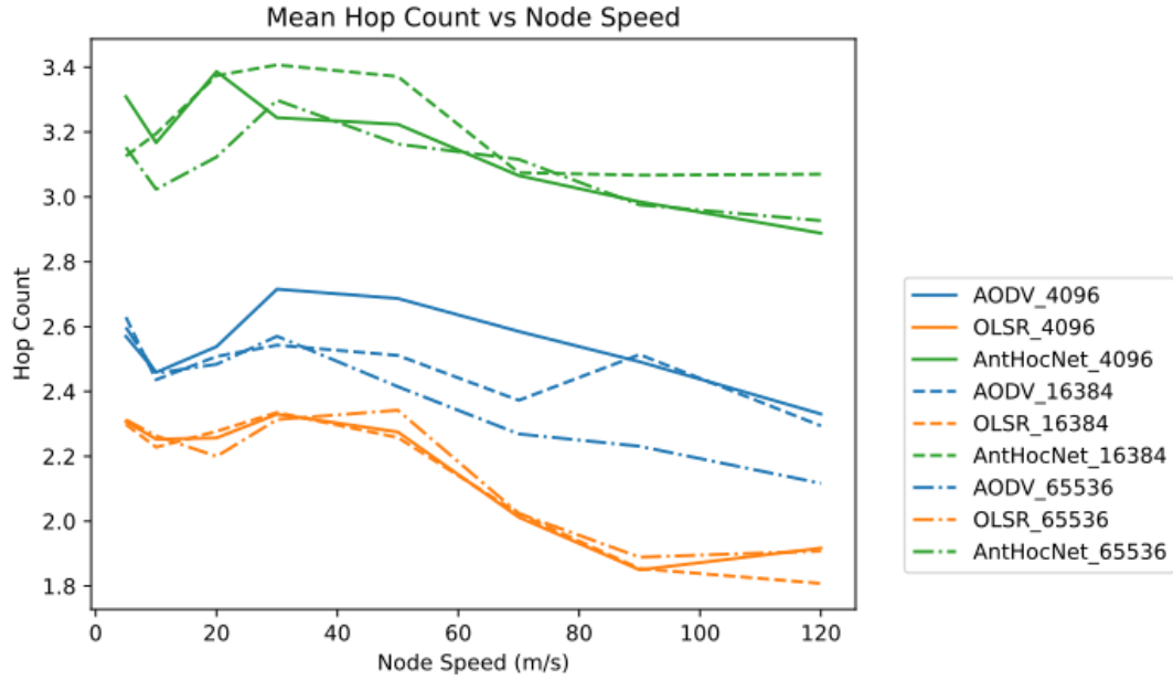
Figure 28: Scenario-II Results: Mean Hop Count vs Node Speed (RWP)
