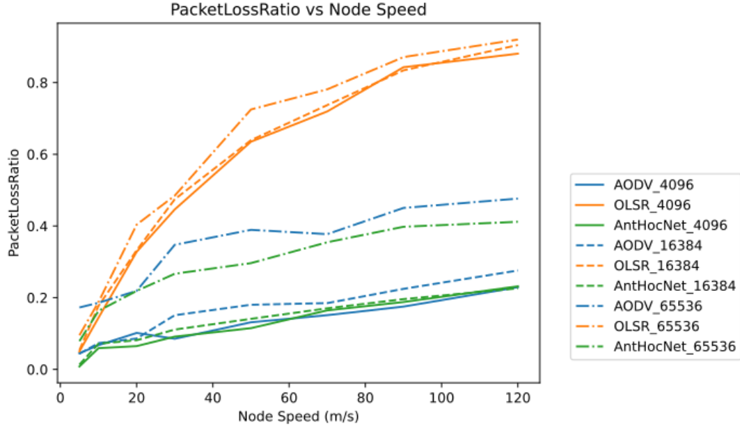
Figure 25: Scenario-II Results: Packet Loss Rate vs. Node Speed (RWP)
