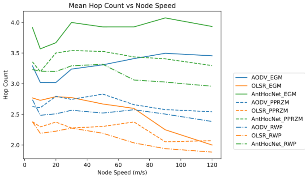
Figure 19: Scenario-I Results: Mean Hop Count vs. Node Speed
