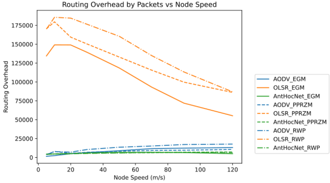
Figure 22: Scenario-I Results: Routing Overhead vs. Node Speed
