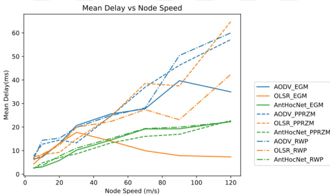
Figure 20: Scenario-I Results: Mean End-to-end Delay vs. Node Speed
