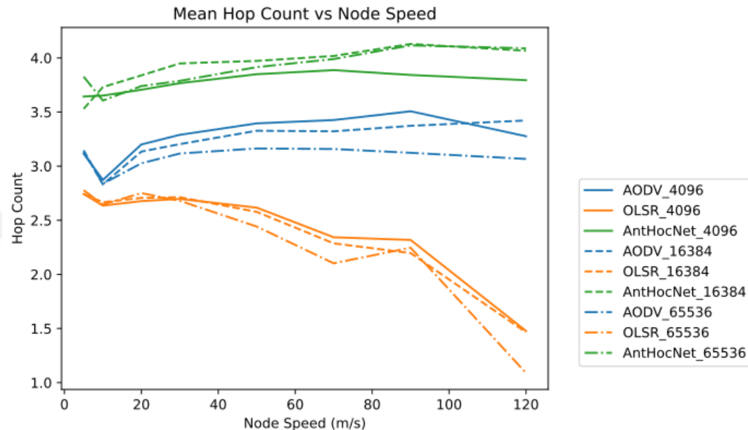
Figure 26: Scenario-II Results: Mean Hop Count vs Node Speed (EGM)
