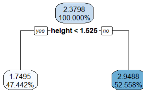
Figure 4.2: Decision Tree of REEMtree Model
