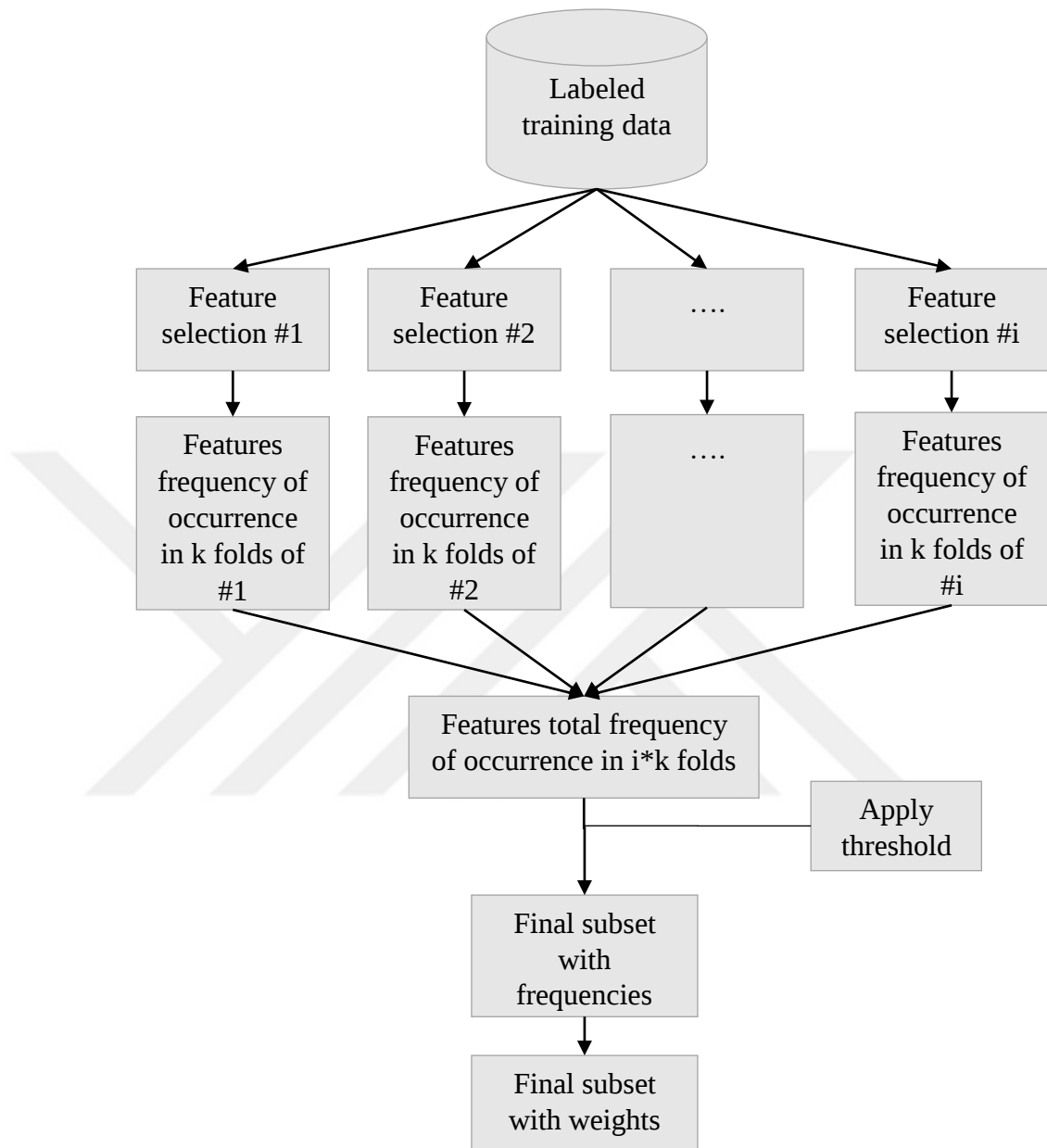
Figure 3.8: Ensemble feature selection approach
