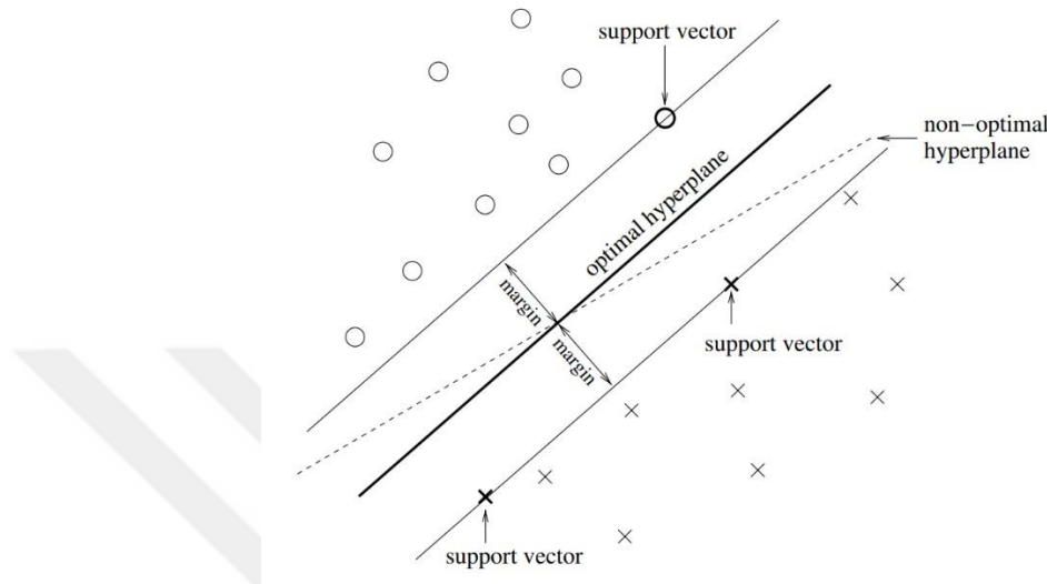
Figure 3.5: SVM optimal hyperplane [59]
