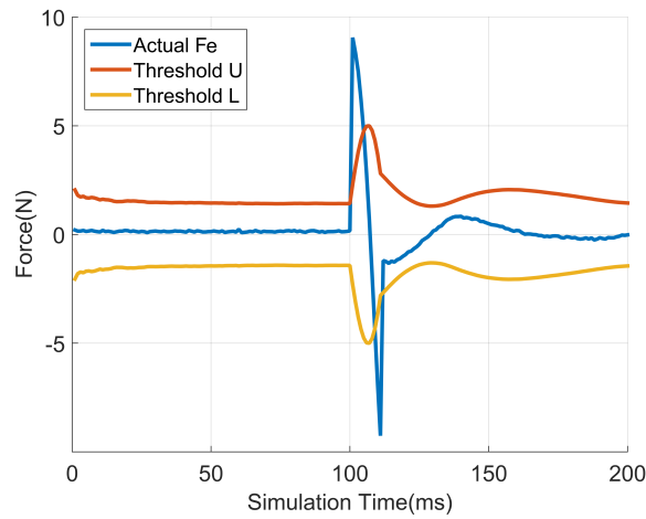
Figure 3.12: Upper(U) and lower(L) threshold vs. estimated impact force
