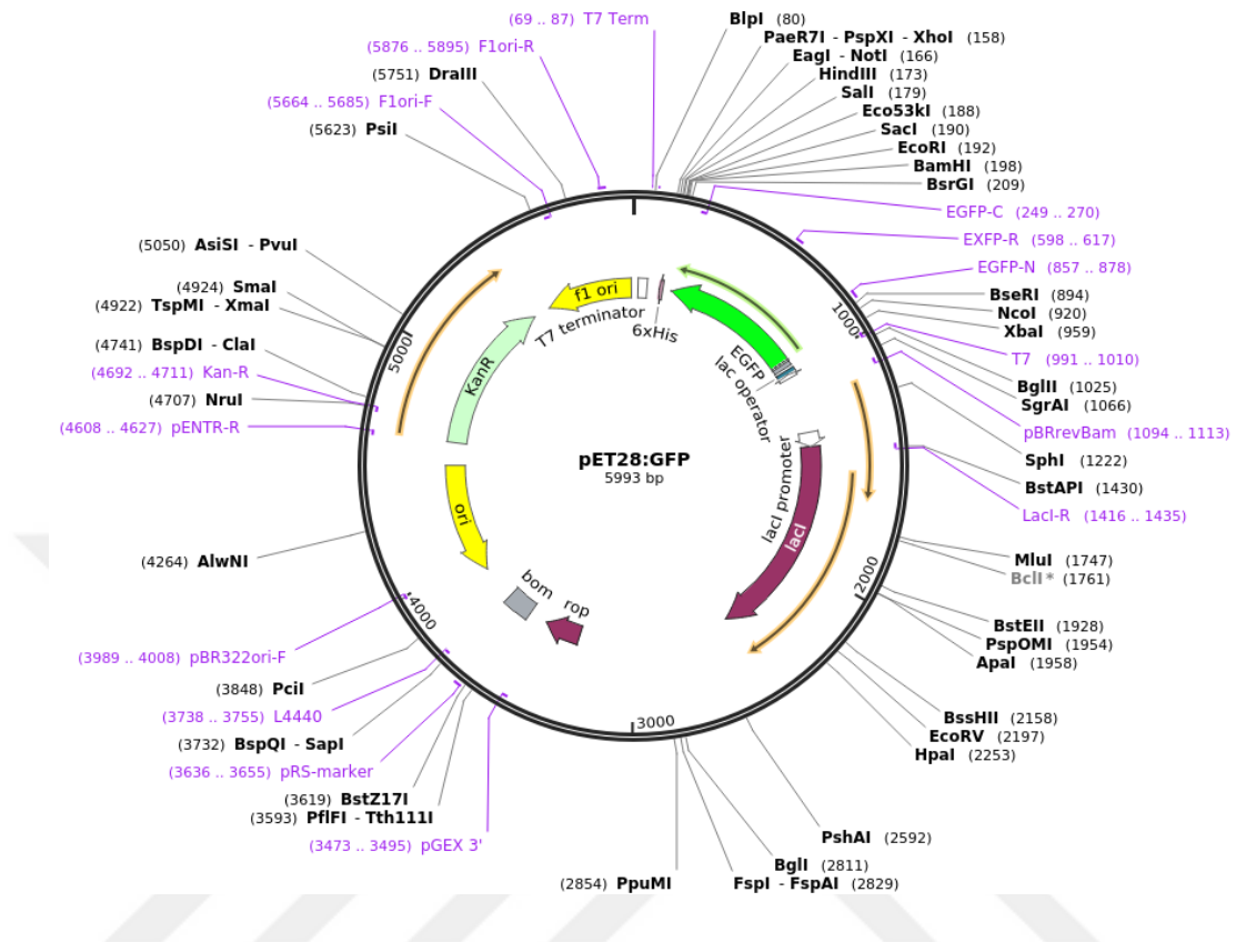
Figure 2.6. pET28a: GFP plasmid vector's genetic map (Addgene plasmid # 60733 ; http://n2t.net/addgene:60733 ; RRID:Addgene_60733)
