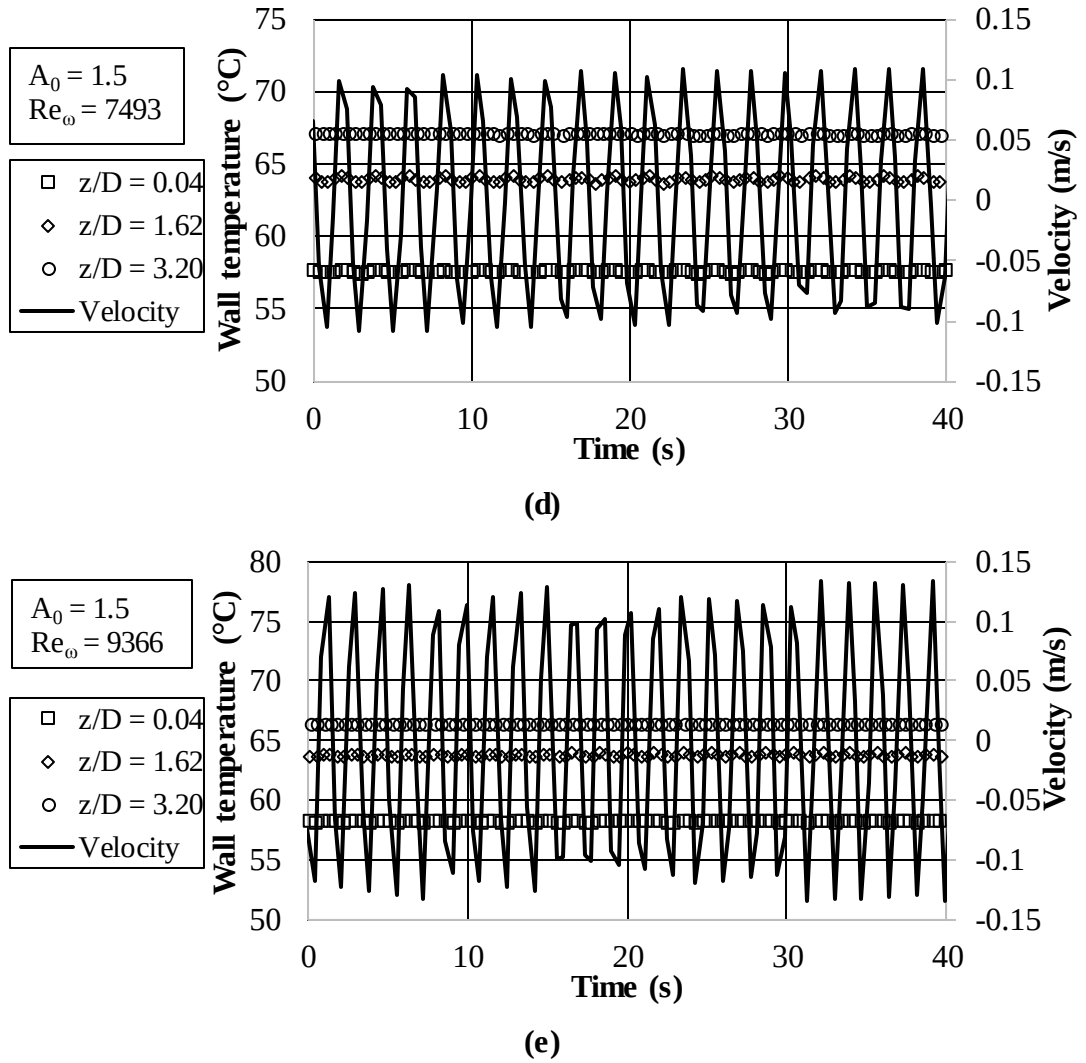
Figure 4.14 (continued) : Wall temperature and flow velocity as functions of time for fluid displacement A_0 = 1.5 for (a) Re_\omega = 1873 , (b) Re_\omega = 3746 , (c) Re_\omega = 5619 , (d) Re_\omega = 7493 and (e) Re_\omega = 9366 .
