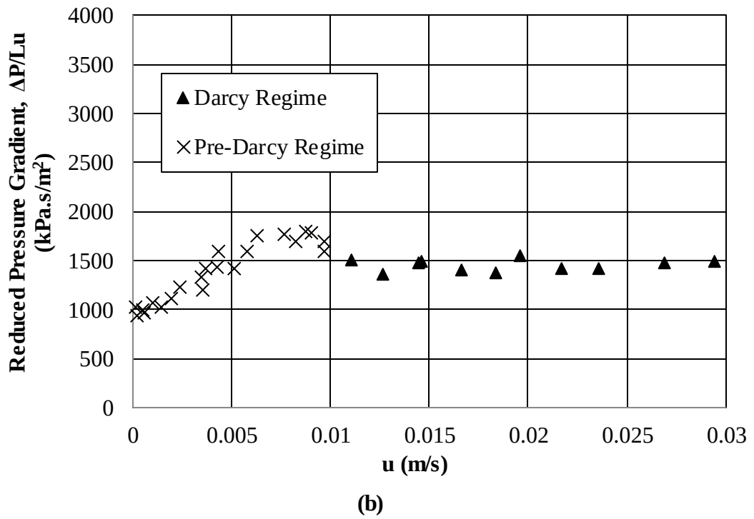
Figure 3.6 : Reduced pressure gradients versus average velocity for 1-mm spheres. Uncertainty in reduced pressure drop is 1.11% in the pre-Darcy regime and 0.70% in all other regimes: (a) Complete velocity range (b) Darcy and pre-Darcy regimes only.
