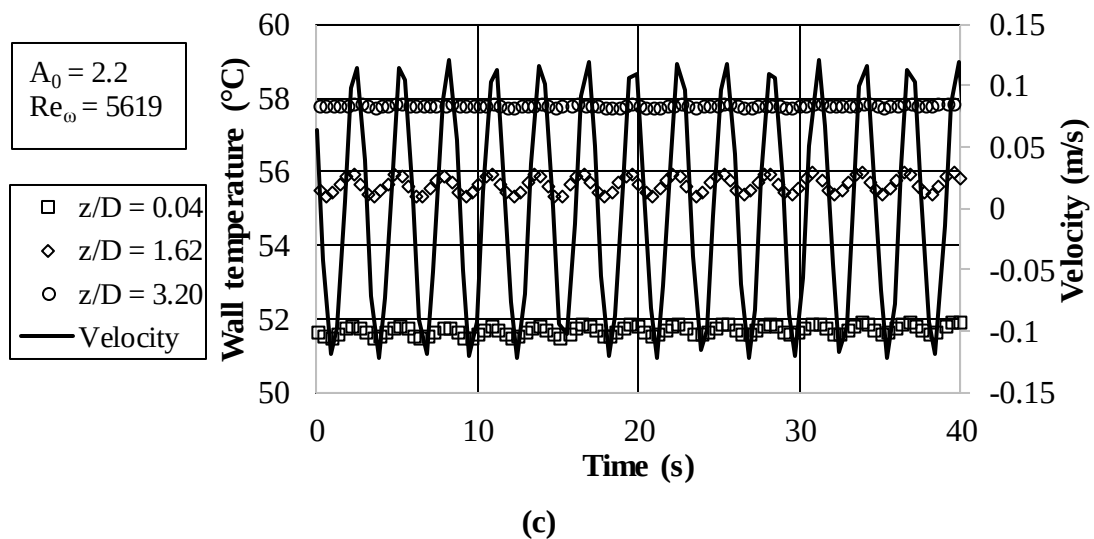
Figure 4.16 : Wall temperature and flow velocity as functions of time for fluid displacement A_0 = 2.2 for (a) Re_\omega = 1873 , (b) Re_\omega = 3746 and (c) Re_\omega = 5619 .
