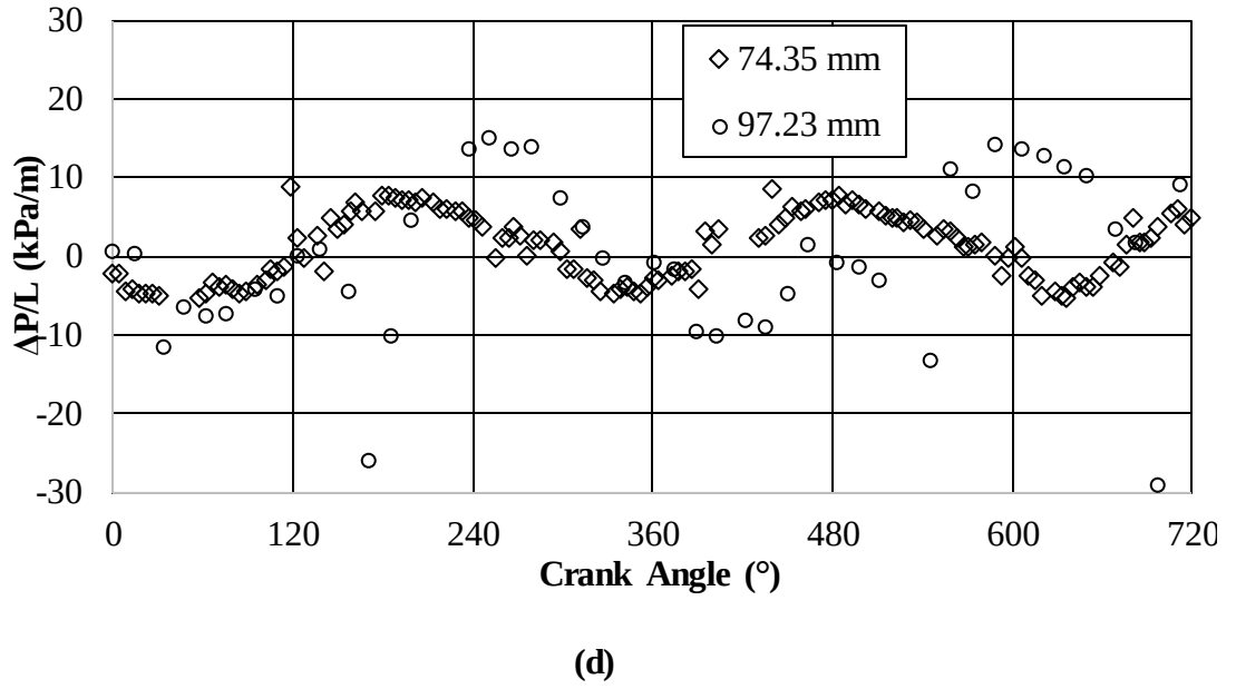
Figure 3.28 (continued) : Pressure gradient as a function of crank angle – effect of displacement: (a) \omega = 0.116 Hz, (b) \omega = 0.232 Hz, (c) \omega = 0.348 Hz and (d) \omega = 0.580 Hz.
