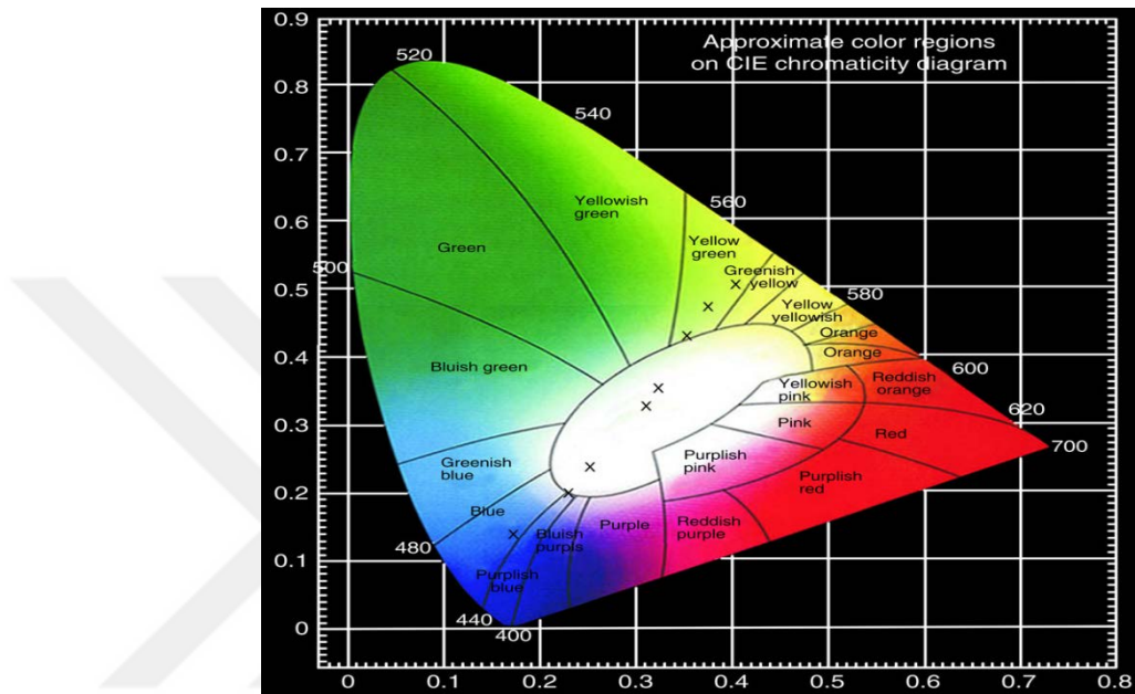
Figure 10. The CIE chromaticity diagram
