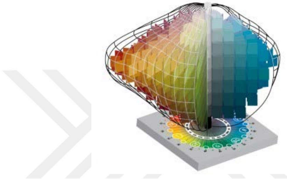
Figure 5. Geometrical framework showing hue, value and chroma in Munsell Colour System.
