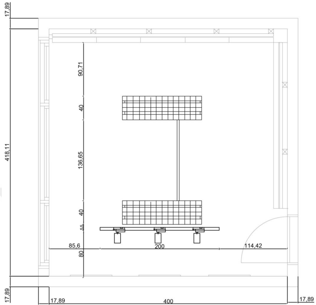
Figure 7. Reflected ceiling plan of the experiment room
