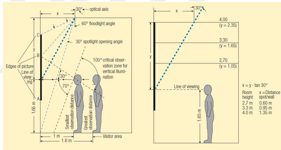
Figure 12. A diagram showing the optimal positioning of the luminaire and observation distance
