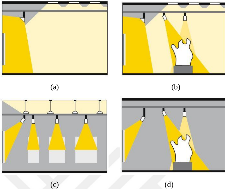
Figure 4. a) Diffuse lighting for the room, directional lighting for the wall b) Supplementary directional lighting for objects in the room c) Indirect and direct illumination d) Directional Lighting (Source: http://en.licht.de/fileadmin/Publications/licht-wissen/0703_lw18_E_light_museums_galleries_web.pdf )
