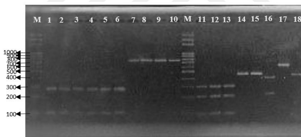
Figure 3.5. Gel image of PCR products cut with HaeIII restriction enzyme
