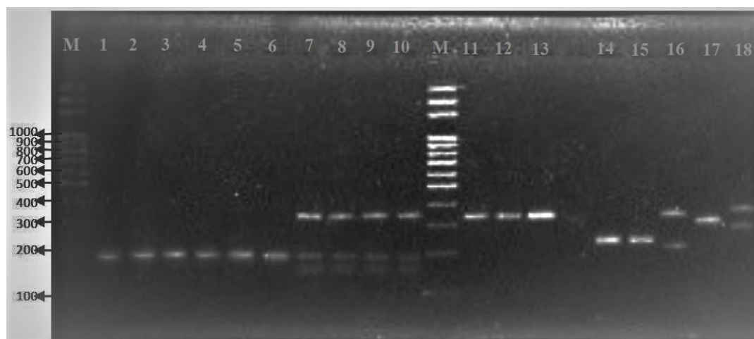
Figure 3.4. Gel image of PCR products cut with HinfI restriction enzyme M, 100bp Marker; 1, reference strain M. pulcherrima (DSMZ); 2- M. pulcherrima (D1D2)/ M. sinensis (ITS) D3 (DA 0CM NS3); 3, M. pulcherrima B10 (BB 0CM NS2); 4, M. aff. pulcherrima B11 (BB 0CM NS3); 5, M. fructicola D15 (DB 4CM NS3); 6, M. aff. fructicola B33 (BB 4CM NS8); 7, reference strain H. uvarum (DSMZ); 8, H. guilliermondii K1 (KA 0CM NS1); 9, H. opuntiae K2 (KA 0CM NS2); 10, H. uvarum K13 (KA 4CM NS3); 11, reference strain L. thermotolerans (DSMZ); 12, L. thermotolerans O9 (OB 4CM NS4); 13, L. thermotolerans O16 (OA 0CM NS7); 14, reference strain Candida spp.(DSMZ); 15, Candida zemplinina ( Starmerella bacillaris ) D10 (DA 4CM NS2); 16, Rhodotorula mucilaginosa K9 (KB 0CM NS4); 17, Wickerhamomyces anomalus K41 (KA 0CM S1); 18, Solicoccozyma aerea B4 (BA 0CM NS4)
