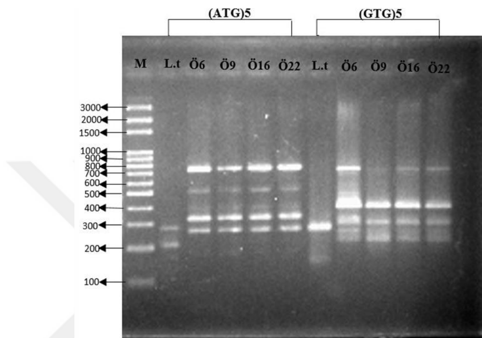
Figure 3.9. The amplification product of L. thermotolerans using (ATG) 5 and (GTG) 5 microsatellite primers
