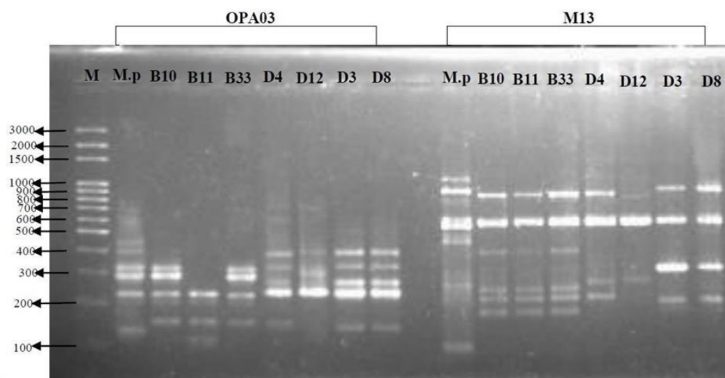
Figure 3.18. The amplification product of M. pulcherrima strains using OPA-03 and M13 primers
