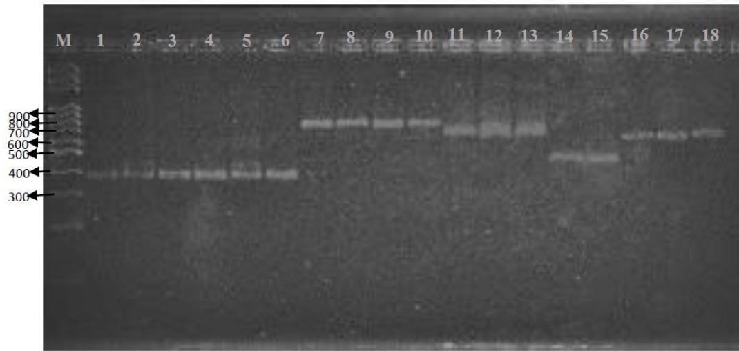
Figure 3.2. Non-Saccharomyces species PCR results
