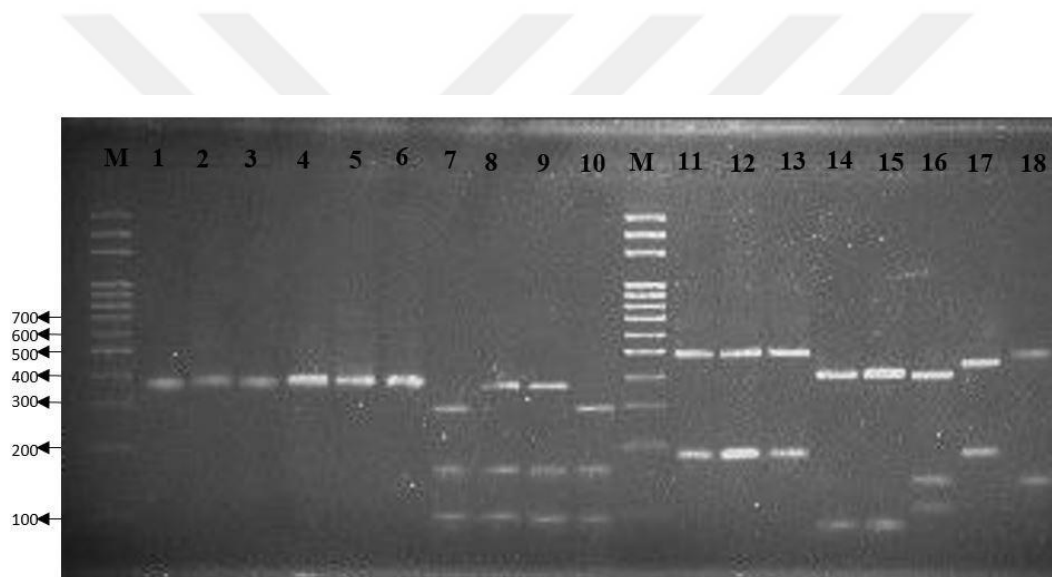
Figure 3.6. Gel image of PCR products cut with DdeI restriction enzyme M, 100bp Marker; 1, reference strain M. pulcherrima (DSMZ); 2, M. pulcherrima (D1D2)/ M. sinensis (ITS) D3 (DA 0CM NS3); 3, M. pulcherrima B10 (BB 0CM NS2); 4, M. aff. pulcherrima B11 (BB 0CM NS3); 5, M. fructicola D15 (DB 4CM NS3); 6, M. aff. fructicola B33 (BB 4CM NS8); 7, reference strain H. uvarum (DSMZ); 8, H. guilliermondii K1 (KA 0CM NS1); 9, H. opuntiae K2 (KA 0CM NS2); 10, H. uvarum K13 (KA 4CM NS3); 11, reference strain L. thermotolerans (DSMZ); 12, L. thermotolerans O9 (OB 4CM NS4); 13, L. thermotolerans O16 (OA 0CM NS7); 14, reference strain candida spp.(DSMZ); 15, Candida zemplinina ( Starmerella bacillaris ) D10 (DA 4CM NS2); 16, Rhodotorula mucilaginosa K9 (KB 0CM NS4); 17, Wickerhamomyces anomalus K41 (KA 0CM S1); 18, Solicoccozyma aeria B4 (BA 0CM NS4)
