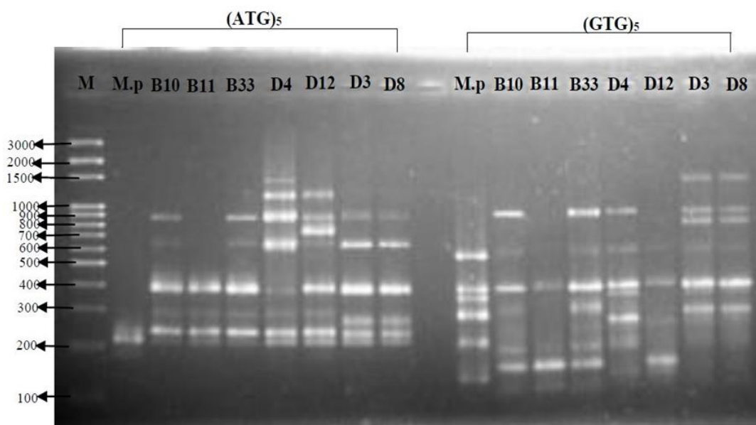
Figure 3.19. The amplification product of M. pulcherrima strains using (ATG) 5 and (GTG) 5 microsatellite primers
