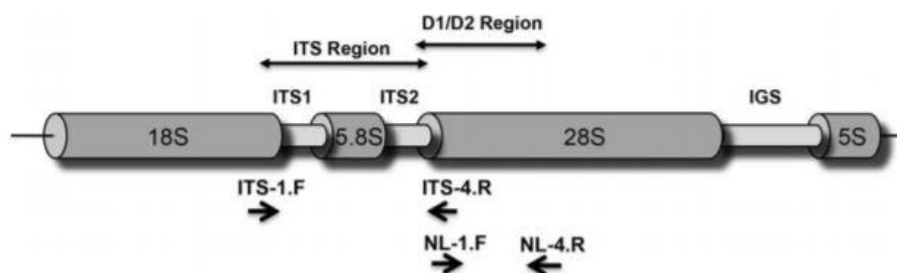
Figure 1.3. The location of D1/D2 variable domains inside the 28S ribosomal subunit, and ITS region flanking 5.8S subunit and related primers (Romanelli et al., 2014)
