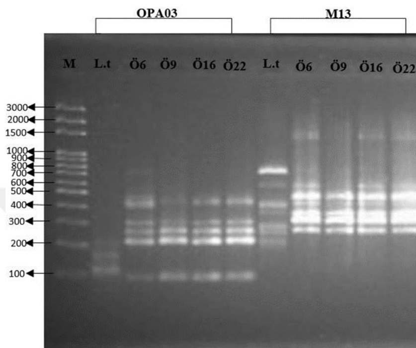
Figure 3.8. The amplification product of L. thermotolerans using primers OPA-03 and M13
