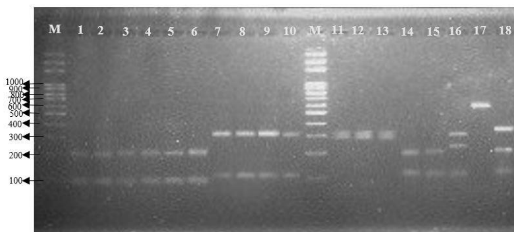
Figure 3.3. Gel image of PCR products cut with HhaI ( CfoI ) restriction enzyme M, 100bp Marker; 1, reference strain M. pulcherrima (DSMZ); 2, M. pulcherrima (D1D2)/ M. sinensis (ITS) D3 (DA 0CM NS3); 3, M. pulcherrima B10 (BB 0CM NS2); 4, M. aff. pulcherrima B11 (BB 0CM NS3); 5, M. fructicola D15 (DB 4CM NS3); 6, M. aff. fructicola B33 (BB 4CM NS8); 7, reference strain H. uvarum (DSMZ); 8, H. guilliermondii K1 (KA 0CM NS1); 9, H. opuntiae K2 (KA 0CM NS2); 10, H. uvarum K13 (KA 4CM NS3); 11, reference strain L. thermotolerans (DSMZ); 12, L. thermotolerans O9 (OB 4CM NS4); 13, L. thermotolerans O16 (OA 0CM NS7); 14, reference strain Candida spp.(DSMZ); 15, Candida zemplinina ( Starmerella bacillaris ) D10 (DA 4CM NS2); 16, Rhodotorula mucilaginosa K9 (KB 0CM NS4); 17, Wickerhamomyces anomalus K41 (KA 0CM S1); 18, Solicoccozyma aerea B4 (BA 0CM NS4)
