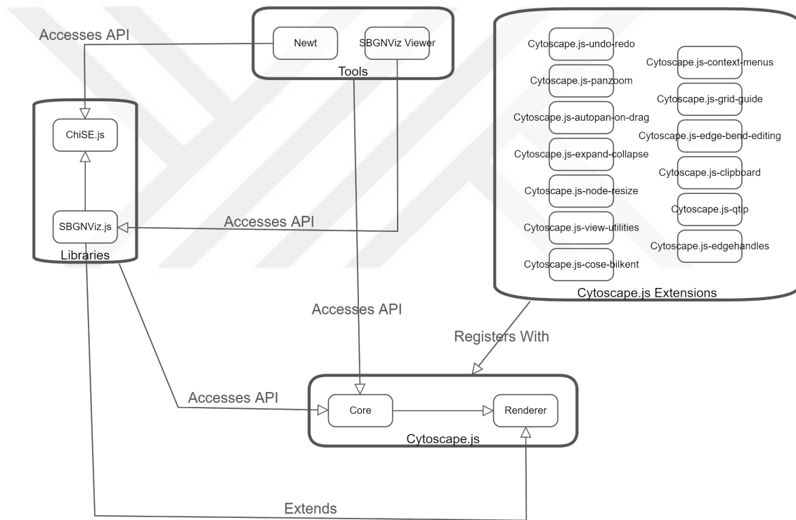
Figure 3.21: Overall System Architecture
