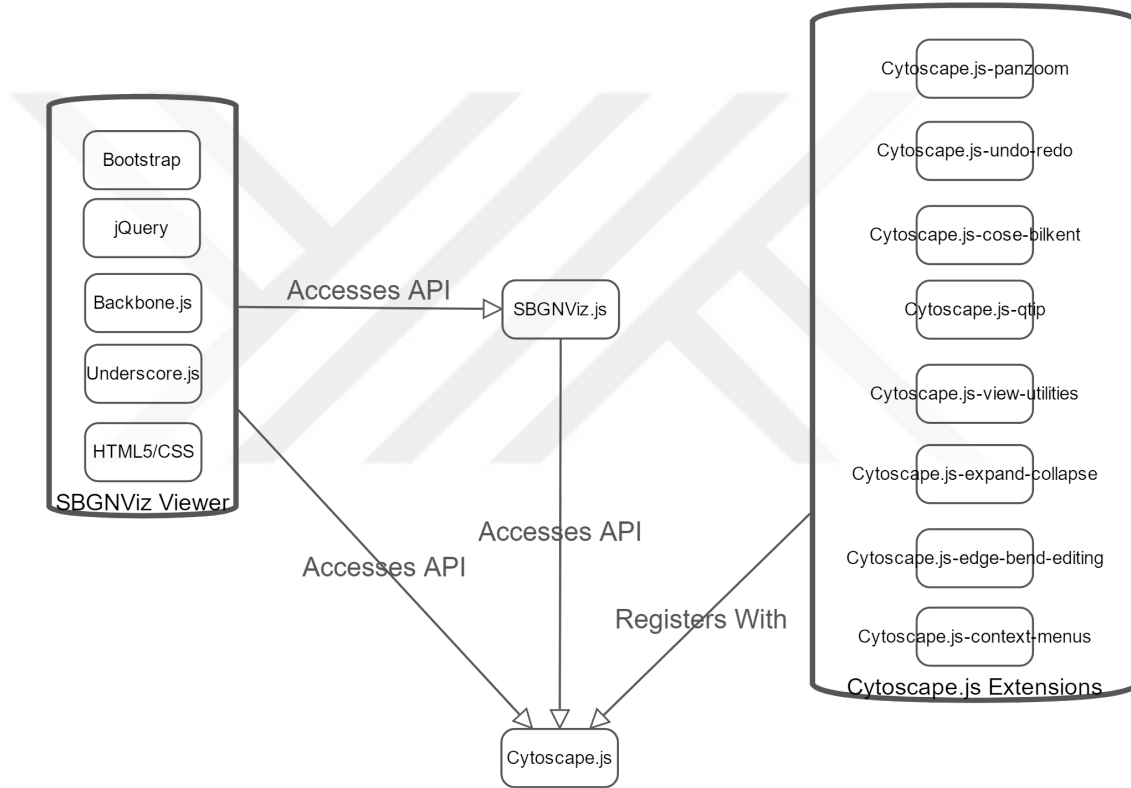
Figure 3.14: SBGNViz Viewer Architecture
