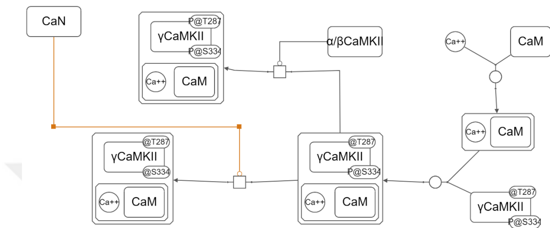
Figure 3.11: Visualization of a graph that includes many edge bend points in SBGNViz Viewer. The bend point positions of the selected edge are highlighted.
