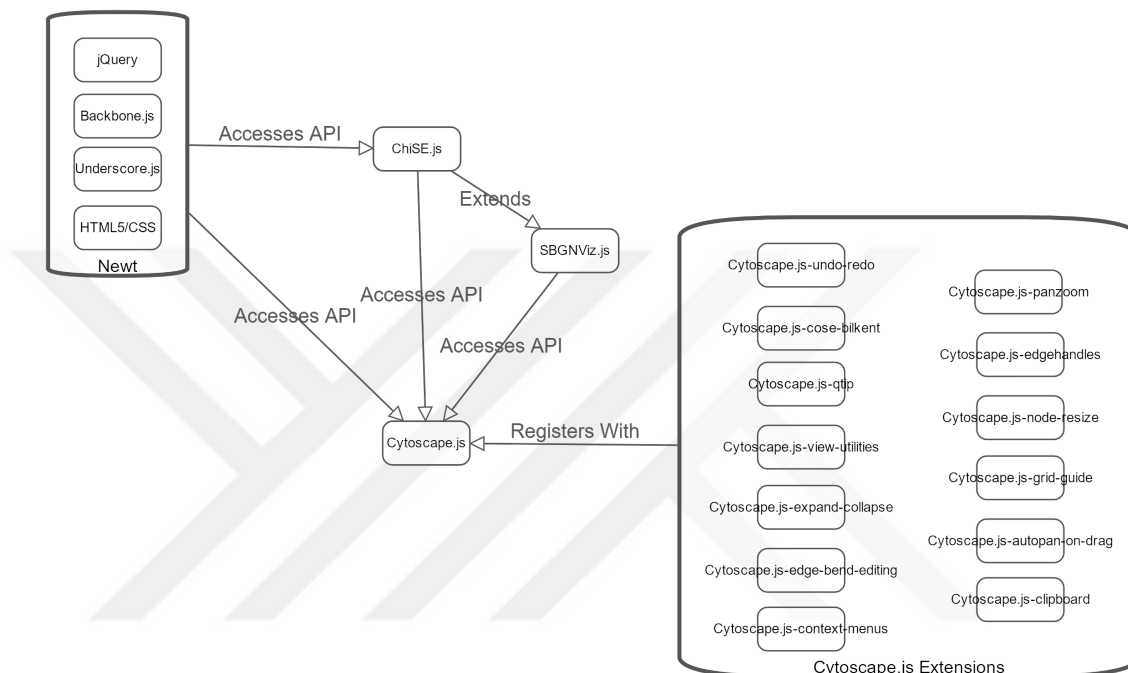
Figure 3.20: Newt Architecture
