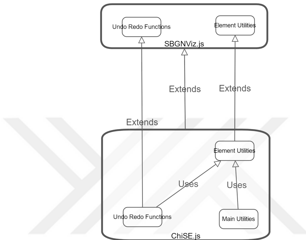
Figure 3.9: ChiSE.js Architecture
