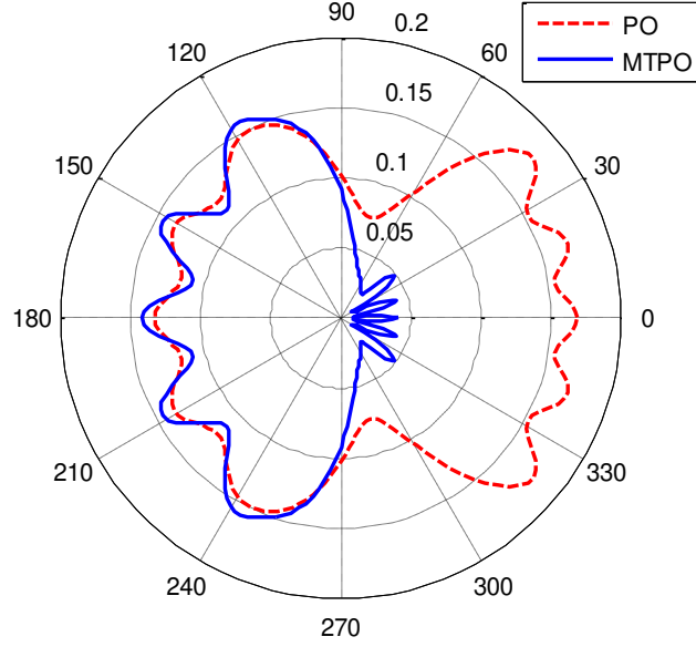
Figure 18 Reflected scattered fields by the hyperbolic reflector at \phi_0 = 60^\circ
