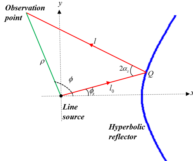
Figure 10 Reflection geometry at the stationary phase point
