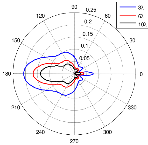
Figure 21 Reflected fields for different observation distances at \phi = 30^\circ
