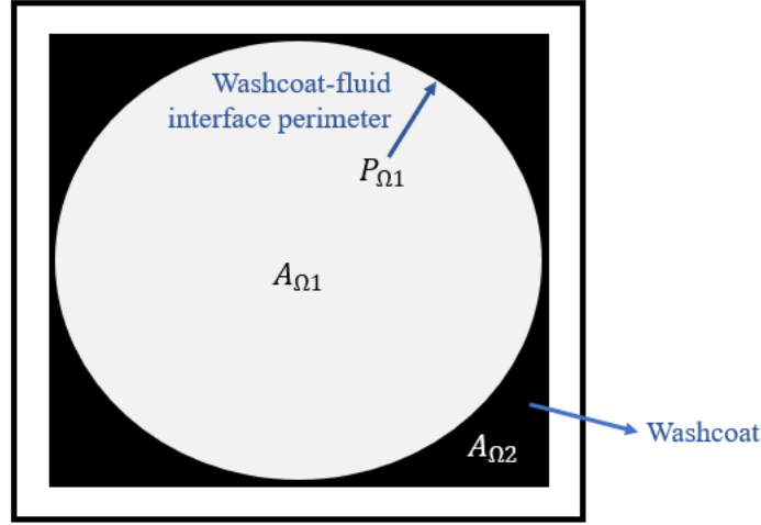
Figure 3.4. Washcoat-fluid interface perimeter ( P_{\Omega 1} ), reactive channel cross-sectional area ( A_{\Omega 1} ) and washcoat cross-sectional area ( A_{\Omega 2} )
