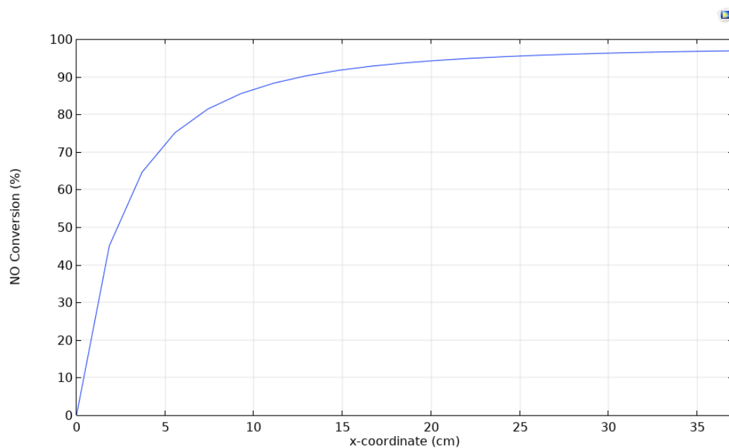
Figure 7.1. NO conversion along the monolith channel direction for Case 1 (SCR unit diameter: 20 cm, NO conversion target at the end of the channel: 98%)
