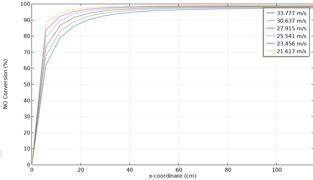
Figure 4.7. NO Conversion along the monolith channel direction for Case 4 at different inlet velocities arising from different diameters (from 20 cm up to 25 cm)
