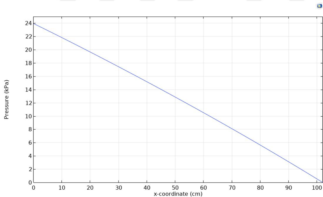
Figure 7.6. Pressure drop along the monolith channel direction for Case 3 (SCR unit diameter: 20 cm, NO conversion target at the end of the channel: 98%)
