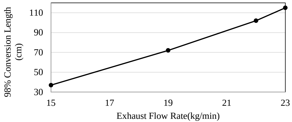
Figure 4.2. Variation of the length where 98% conversion achieved with the increasing engine exhaust mass flow rate
