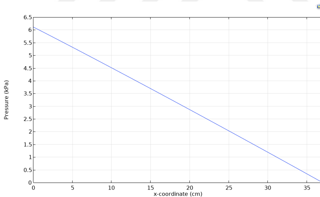
Figure 7.2. Pressure drop along the monolith channel direction for Case 1 (SCR unit diameter: 20 cm, NO conversion target at the end of the channel: 98%)
