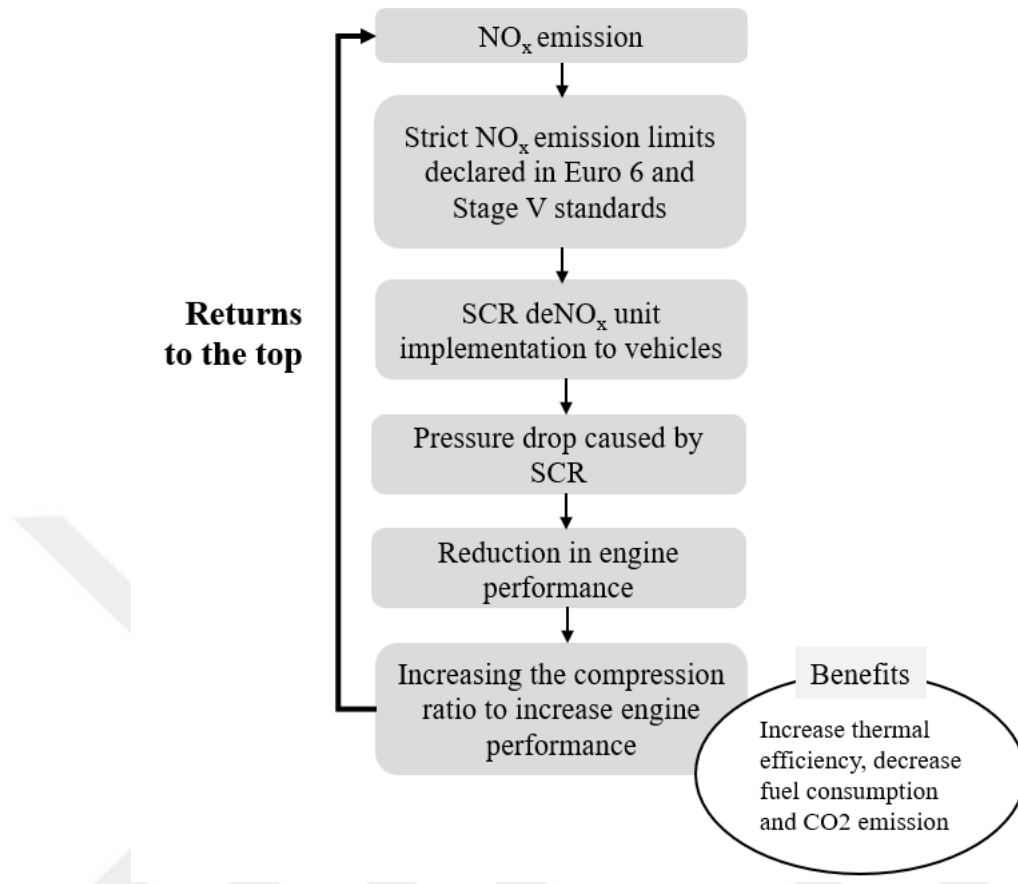
Figure 1.3. Relation between NO x emission, backpressure caused by SCR and engine performance
