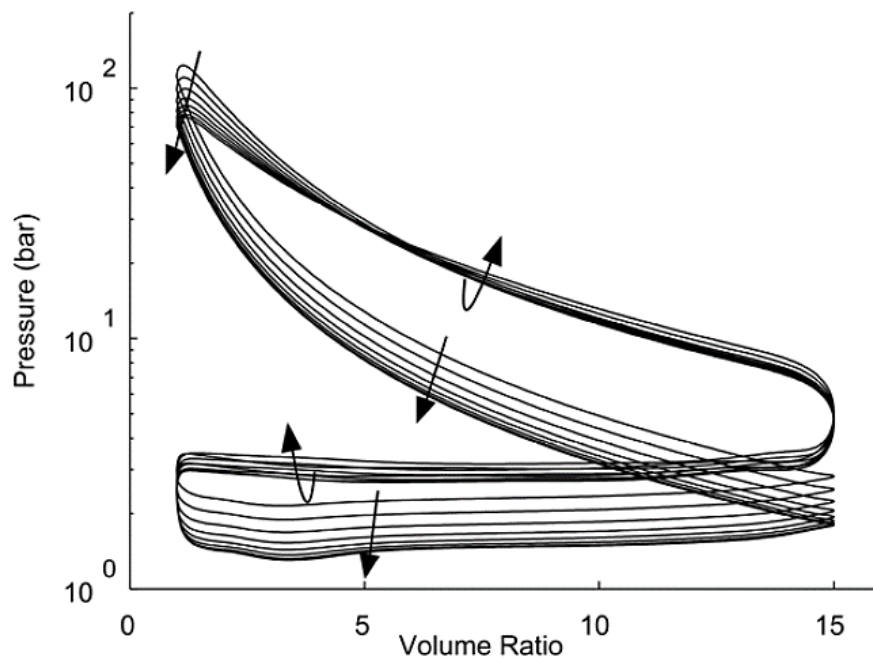
Figure 2.11. Actual PV diagram of a Diesel engine. Arrow directions represent the change with increasing backpressure [49]
