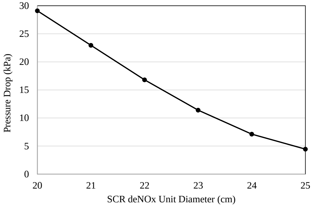
Figure 4.10. Pressure drop variation for Case 4 with increasing SCR unit diameter
