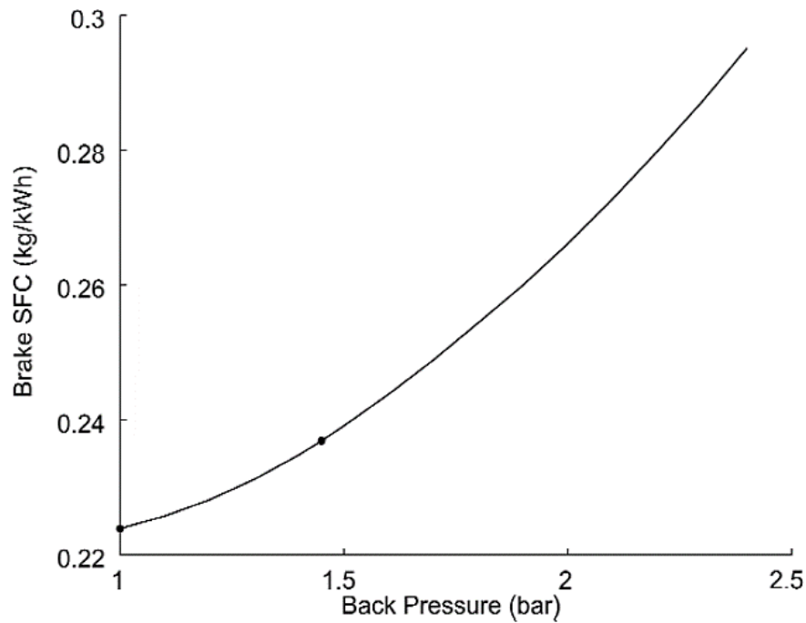
Figure 2.12. BSFC change with increasing backpressure [49]
