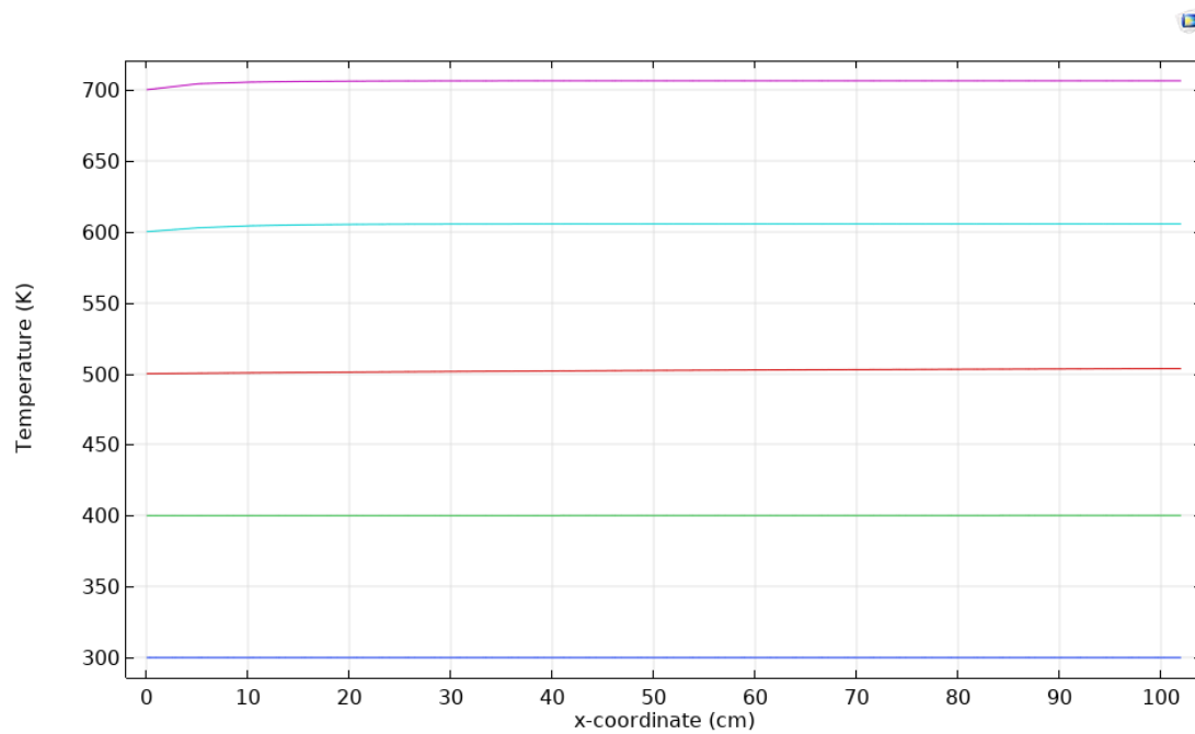
Figure 4.14. Temperature along the monolith channel direction by using exhaust mass flow rate of Case 4
