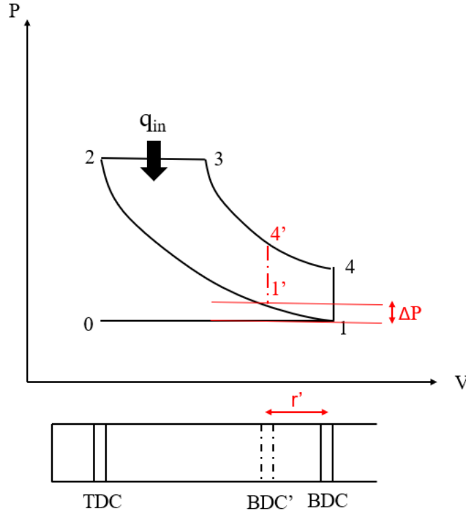
Figure 3.9. Ideal Diesel cycle PV diagram
