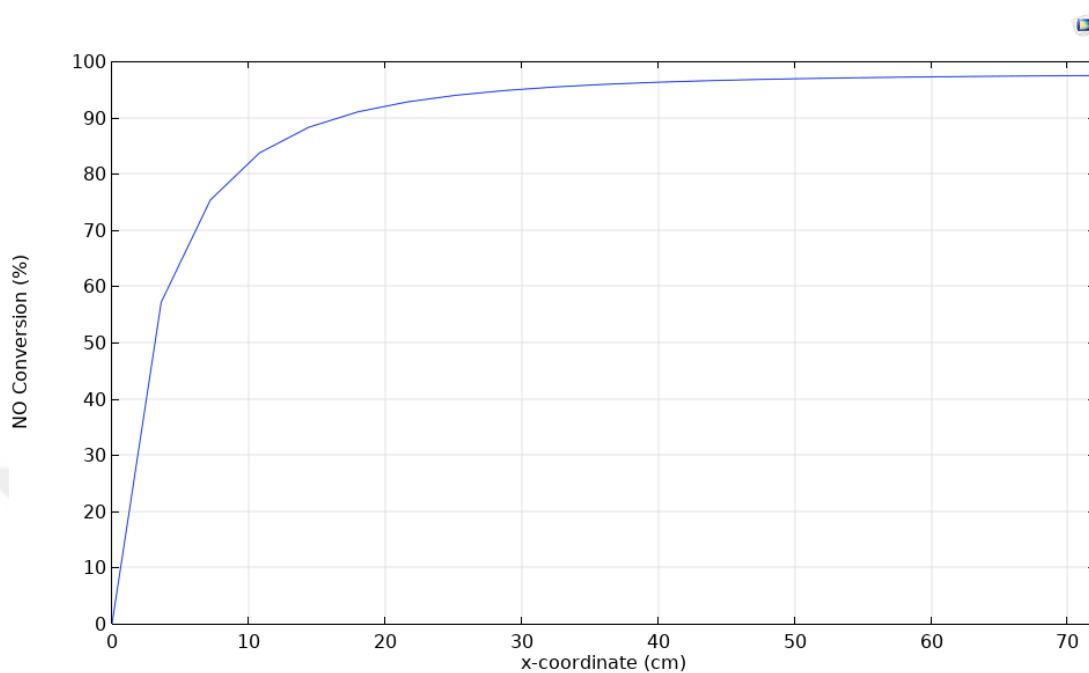
Figure 7.3. NO conversion along the monolith channel direction for Case 2 (SCR unit diameter: 20 cm, NO conversion target at the end of the channel: 98%)
