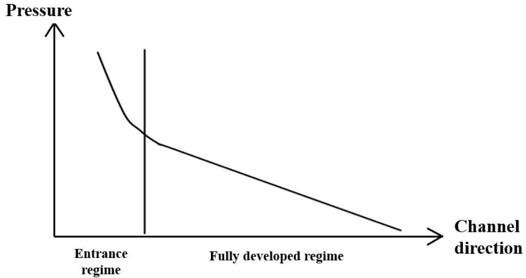
Figure 2.5. Laminar flow pressure profile along the channel direction [55] Copyright © 2003 SAE International, Copyright © 2003 Society of Automotive Engineers of Japan, Inc.
