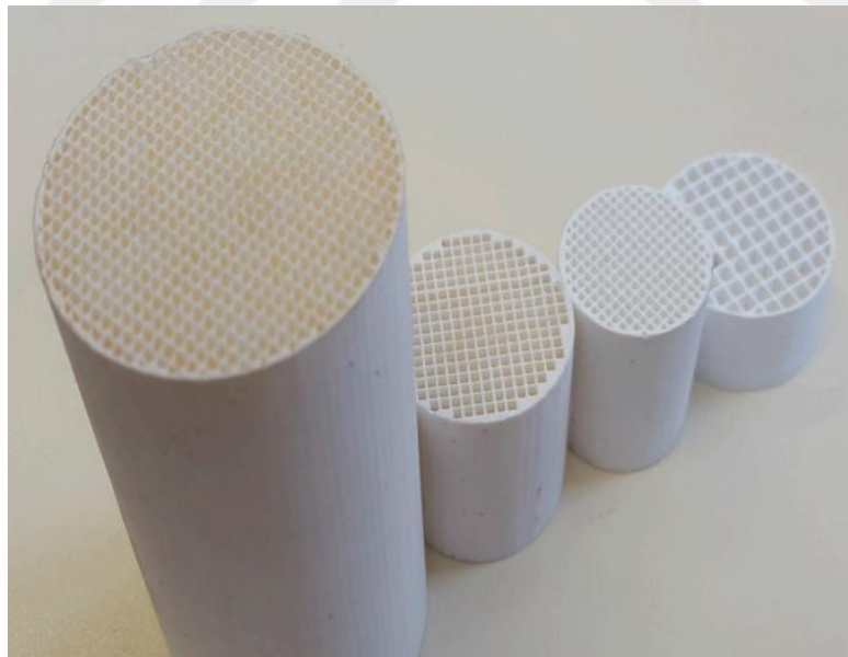
Figure 2.4. Ceramic monoliths at various diameters, lengths and cell densities [35]
