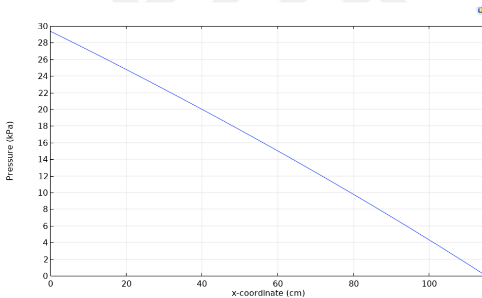
Figure 4.5. Pressure drop along the monolith channel direction for Case 4 (SCR unit diameter: 20 cm, NO conversion target at the end of the channel: 98%)
