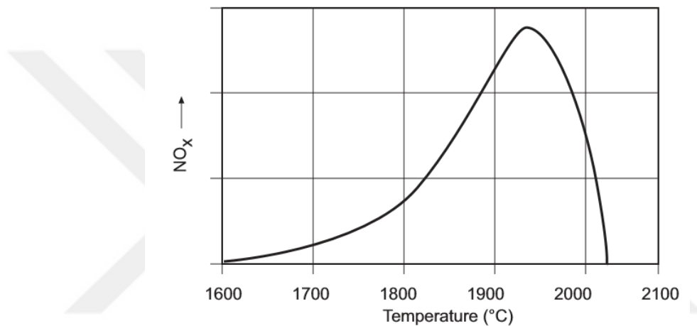
Figure 1.1. Relation between temperature and thermal \text{NO}_x formation [8]
