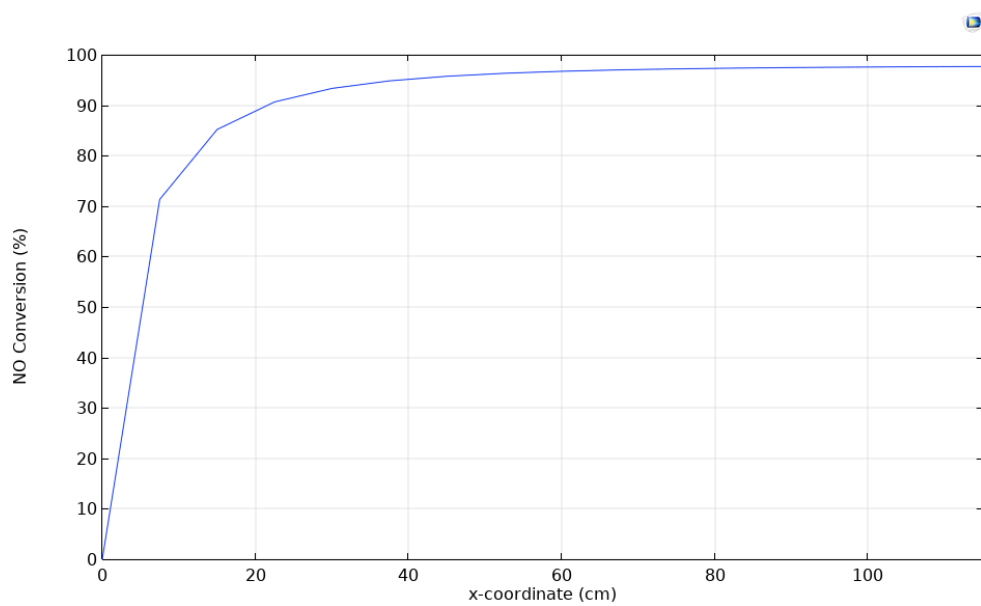
Figure 4.4. NO conversion along the monolith channel direction for Case 4 (SCR unit diameter: 20 cm, NO conversion target at the end of the channel: 98%)
