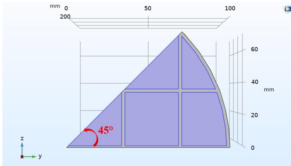
Figure 3.2. 1/8 of the complete monolith reactor (20 cm diameter)
