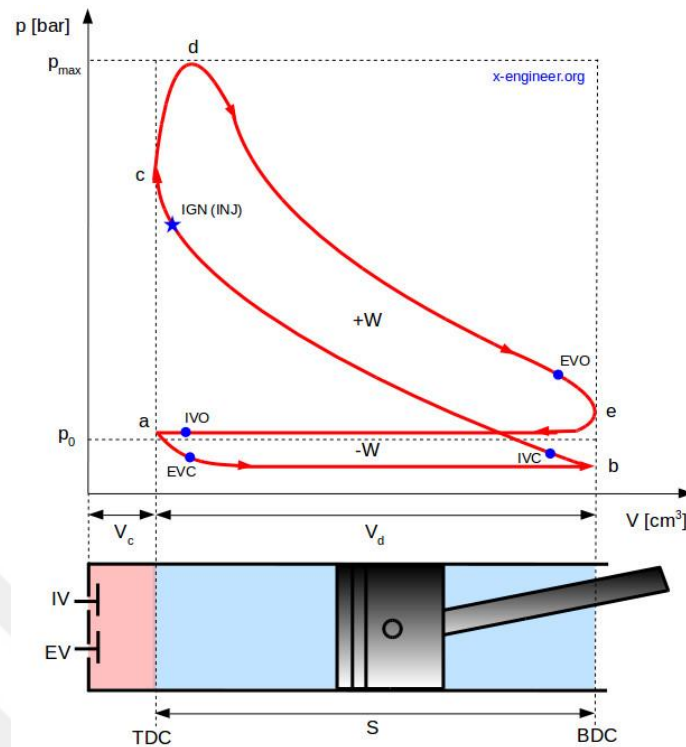
Figure 3.8. An internal combustion engine actual PV diagram [5]
