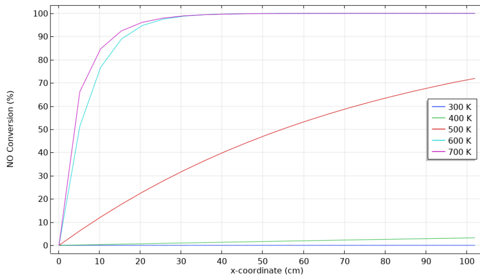
Figure 4.11. NO Conversion along the monolith channel direction by using exhaust mass flow rate of Case 4
