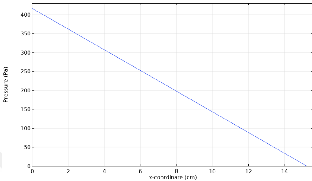
Figure 4.1. Pressure along the monolith channel direction by using the experimental conditions in Ref [14]
