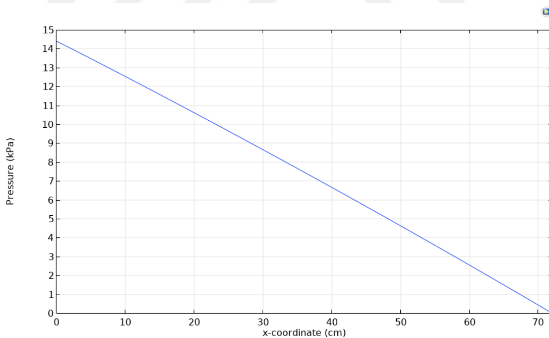
Figure 7.4. Pressure drop along the monolith channel direction for Case 2 (SCR unit diameter: 20 cm, NO conversion target at the end of the channel: 98%)
