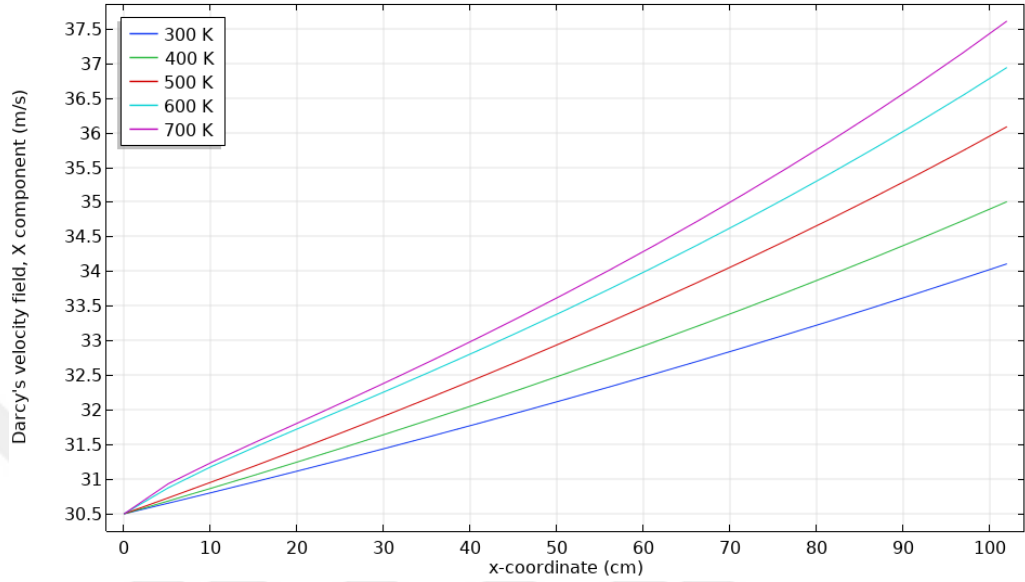
Figure 4.13. Darcy velocity along the monolith channel direction by using exhaust mass flow rate of Case 4
