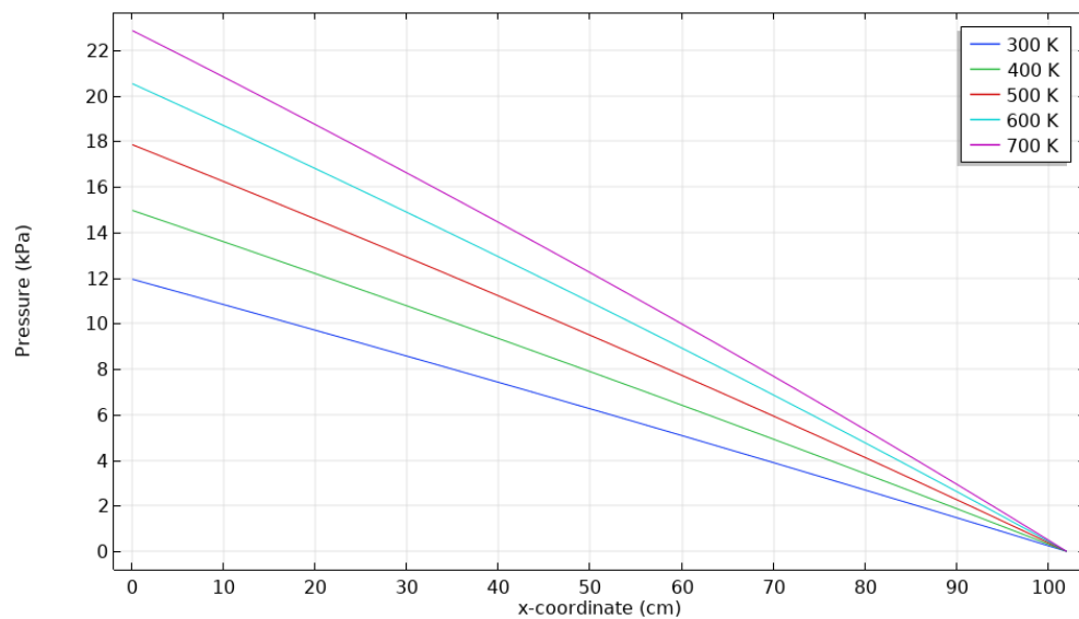
Figure 4.12. Pressure drop along the monolith channel direction by using exhaust mass flow rate of Case 4
