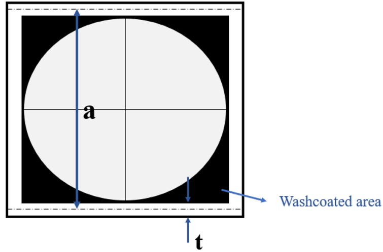
Figure 3.1. A single reactive channel cell spacing ( a ), wall thickness ( t ) and washcoated area (area shaded with black)
