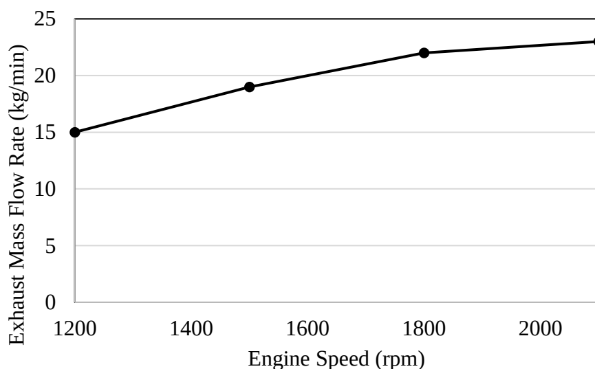
Figure 2.6. Exhaust mass flow rate data of a 9-liter SCANIA industrial engine varying with the engine speed [10].
