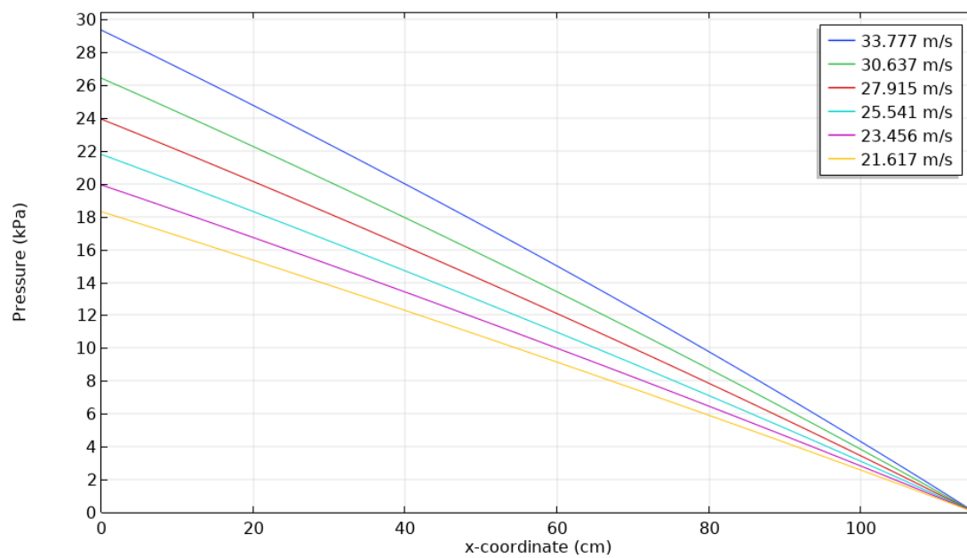
Figure 4.8. Pressure along the monolith channel direction for Case 4 at different inlet velocities arising from different diameters (from 20 cm up to 25 cm)
