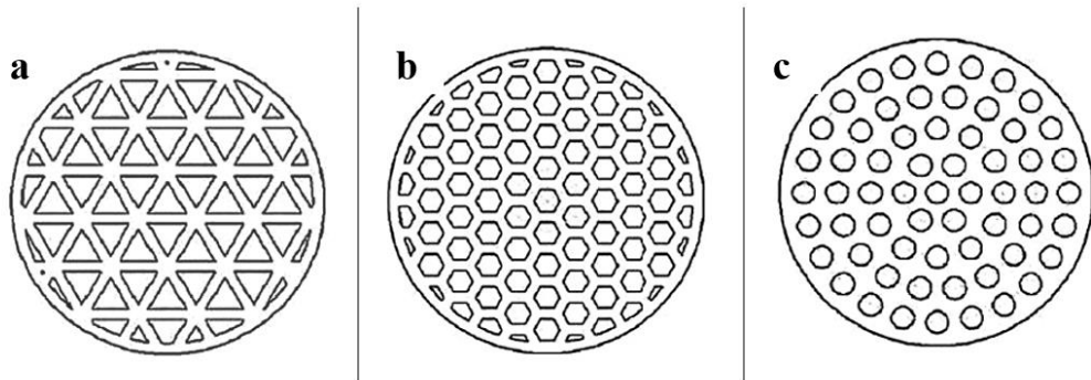
Figure 2.3. Various channel arrangements in a monolith. a.Triangular channels b.Hexagonal channels c. Circular channels [23]
