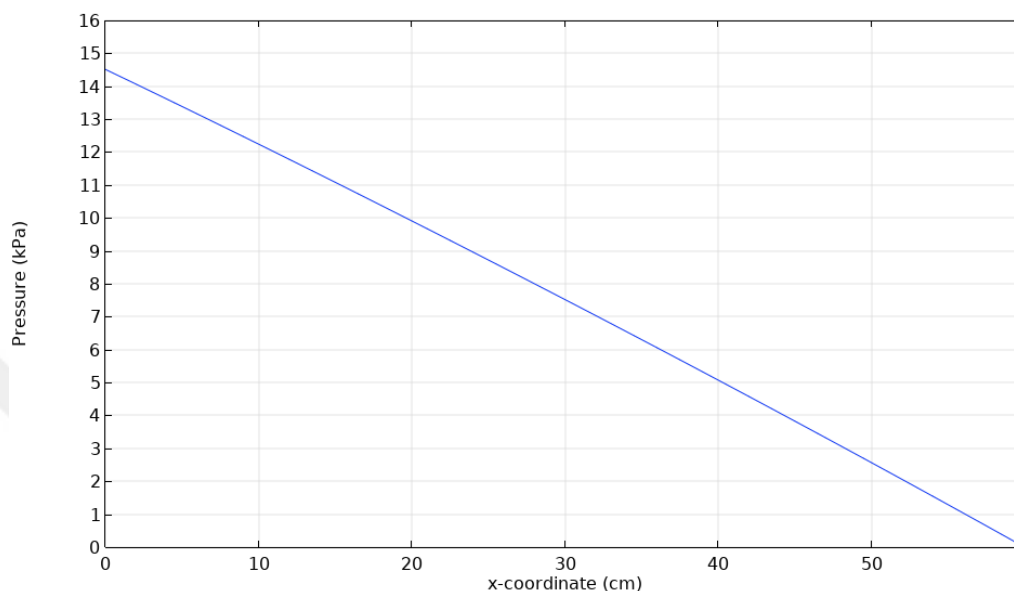
Figure 4.6. Pressure drop along the monolith channel direction for Case 4 (SCR unit diameter: 20 cm, NO conversion target at the end of the channel: 97%)
