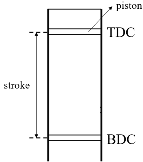
Figure 2.7. Positions of top dead center (TDC) and bottom dead center (BDC) on an engine cylinder
