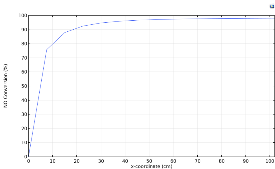
Figure 7.5. NO conversion along the monolith channel direction for Case 3 (SCR unit diameter: 20 cm, NO conversion target at the end of the channel: 98%)
