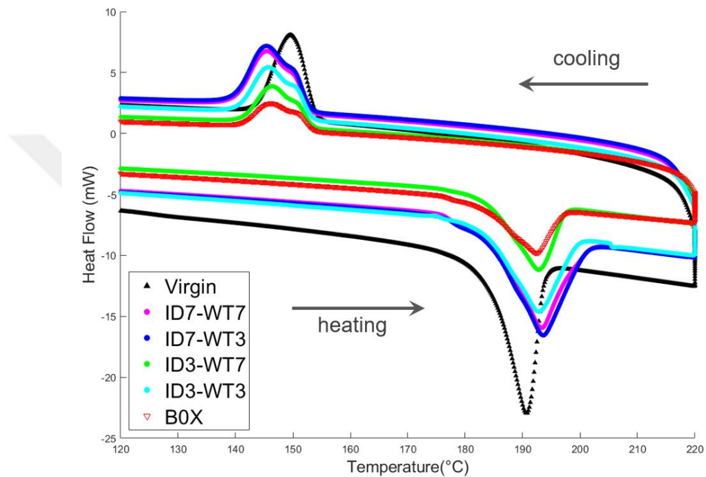
Figure 50 Influence of the nesting parameters on thermal properties of glass filled polyamide 12 powder
