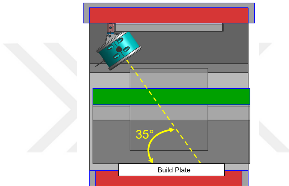
Figure 26 Viewport angle of the LWIR camera
