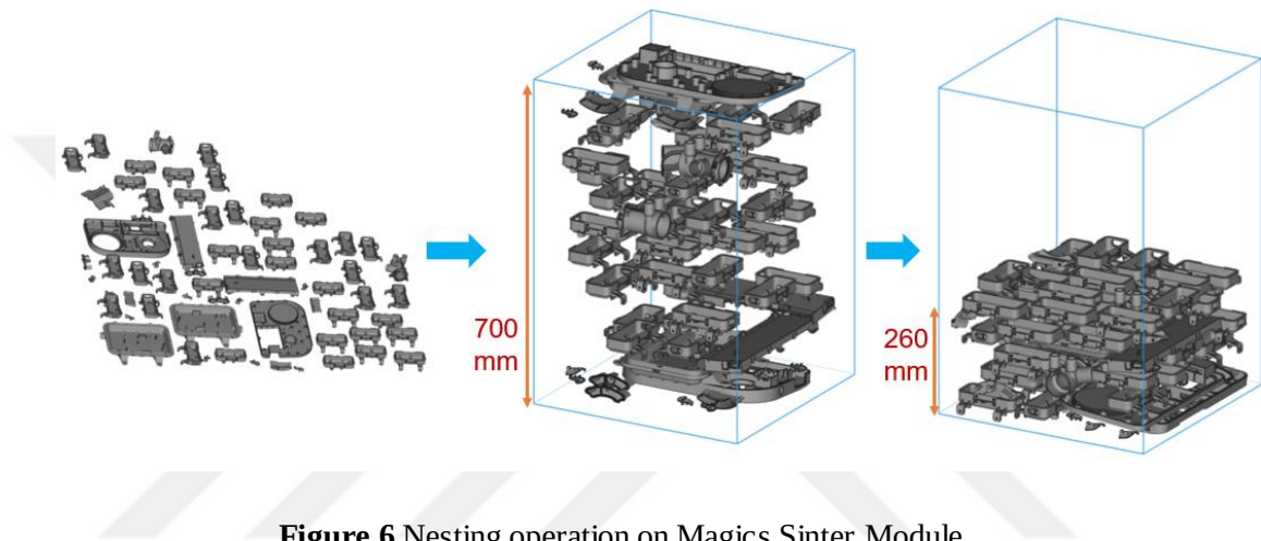
Figure 6 Nesting operation on Magics Sinter Module
