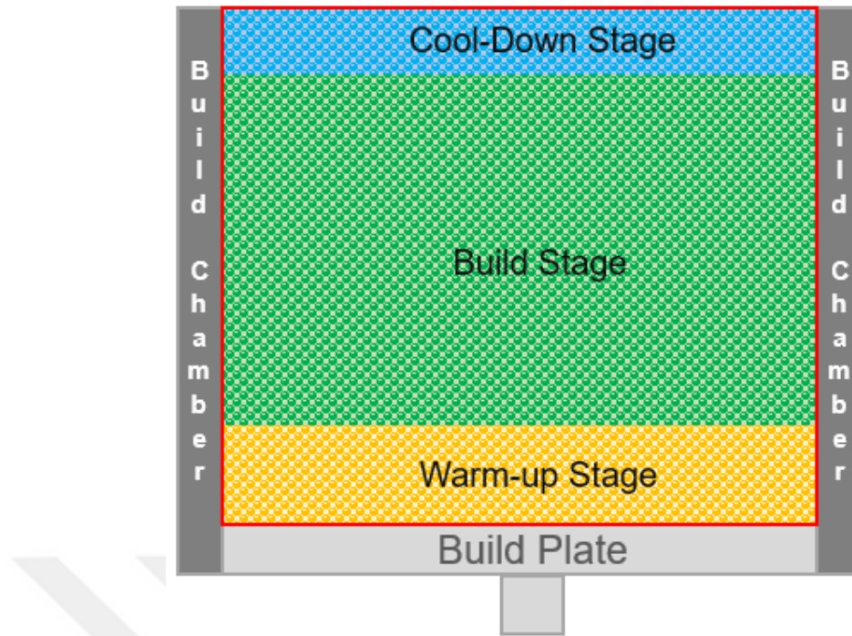
Figure 8 Schematic of stages inside the build space during the SLS process
