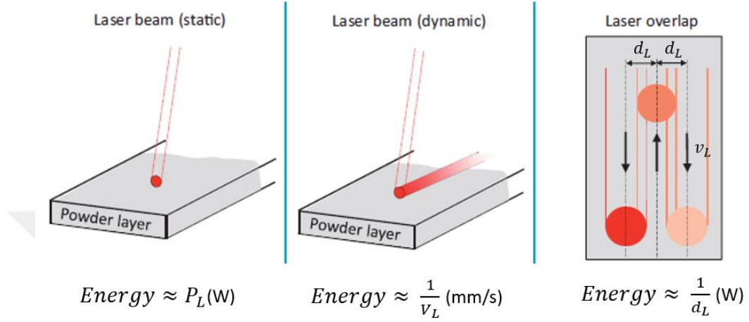
Figure 11 Energy input related with the laser parameters
