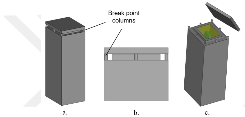
Figure 31 Demonstration for opening the cover. a) Isometric view of the sample b) Side-view of the sample focused on cover c) Sample with the opened cover
