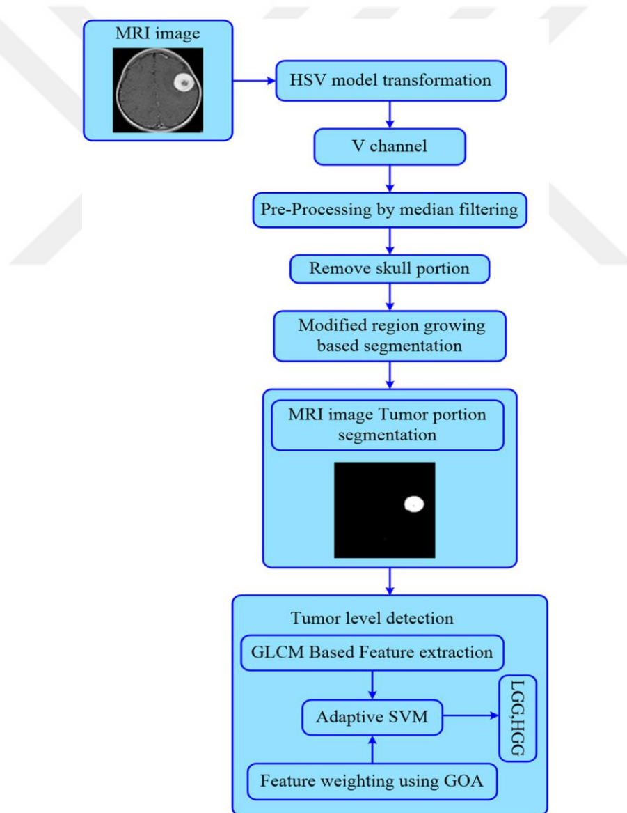
Figure 1.9. A method for modified region growing and adaptive SVM [99]
