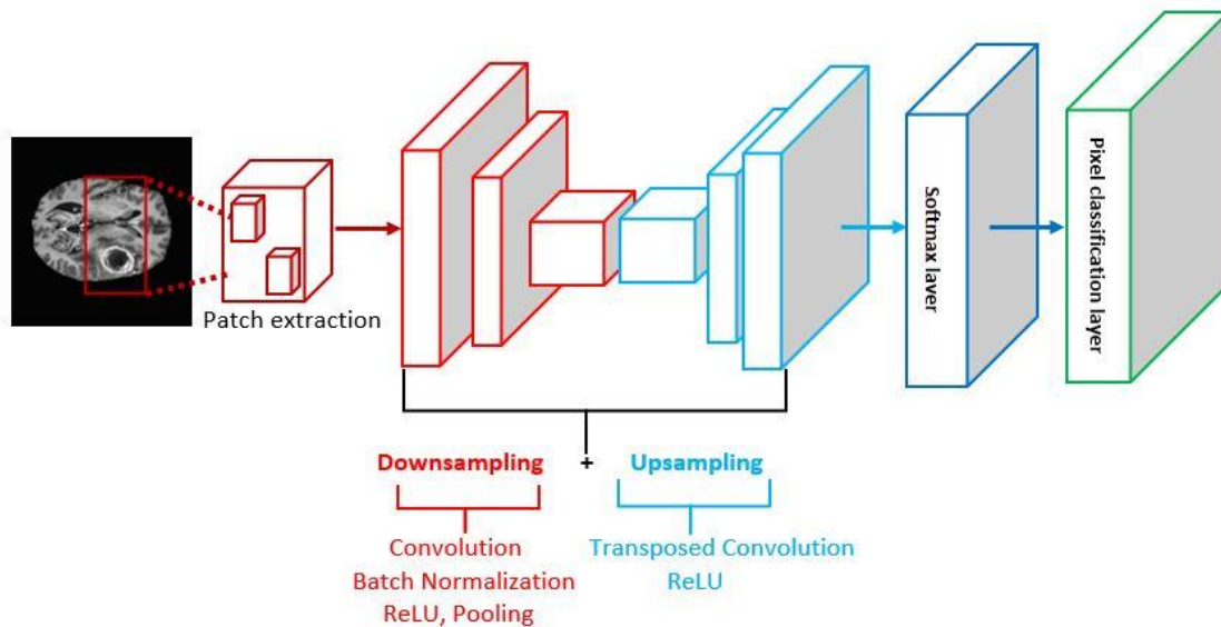
Figure 3.8. Simplified representation of deep learning network for the proposed study.
