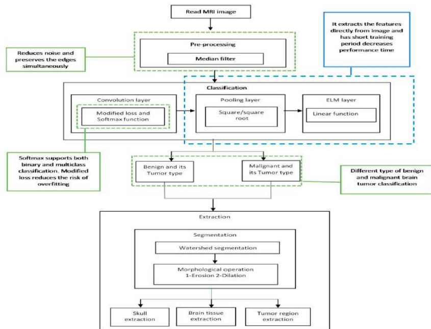
Figure 1.4. Block diagram of the proposed study [36]
