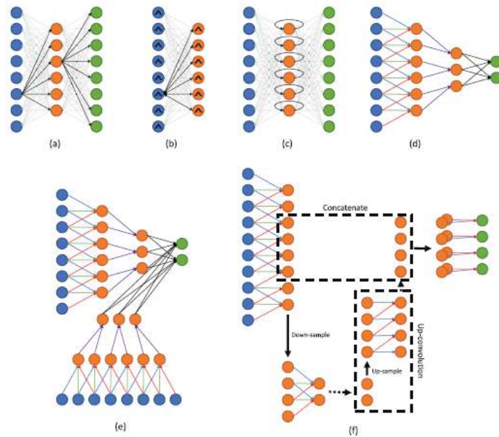
Figure 2.5. Node representation of artificial neural networks used in medical imaging, a) Auto-encoder, b) Constrained Boltzmann model, c) Repetitive neural networks, d) Convolutional neural networks, e) Multi-stream convolutional neural networks, f) U-net [56]
