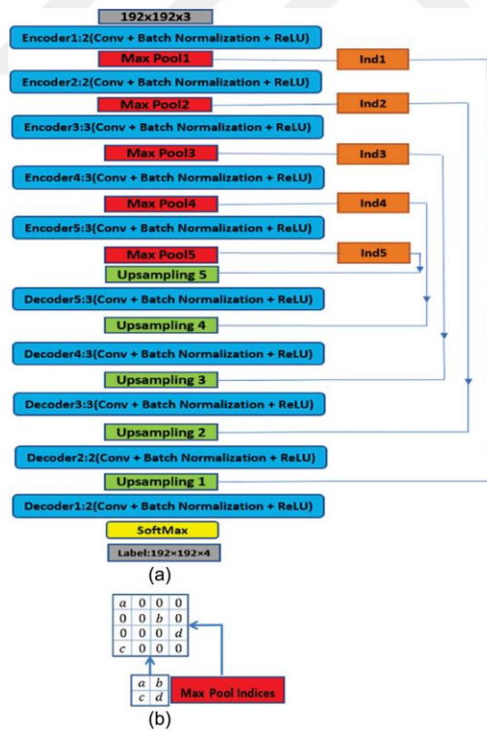
Figure 1.1. Architecture of SegNet [33]
