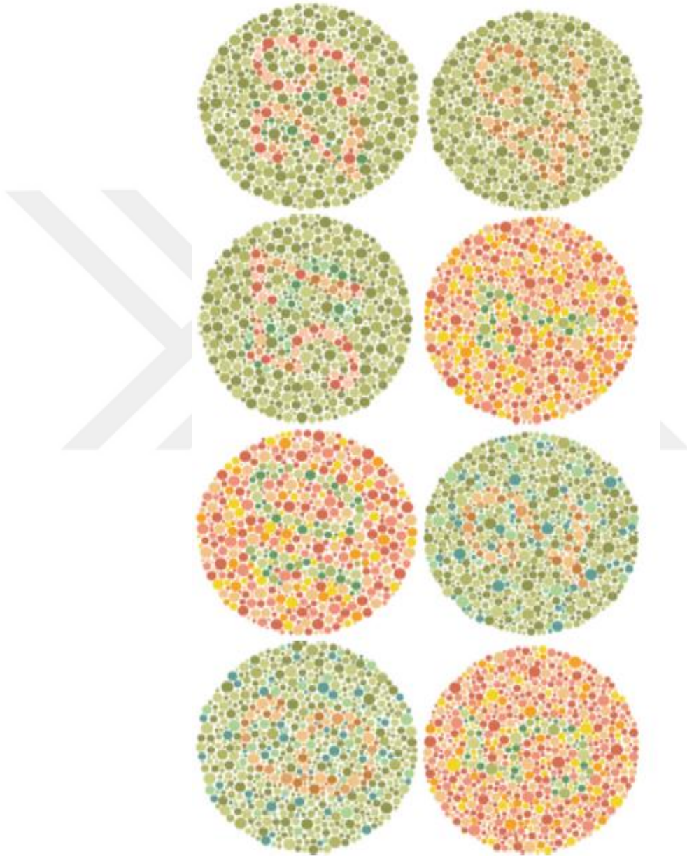
Figure 33. Ishihara's color blindness test.
