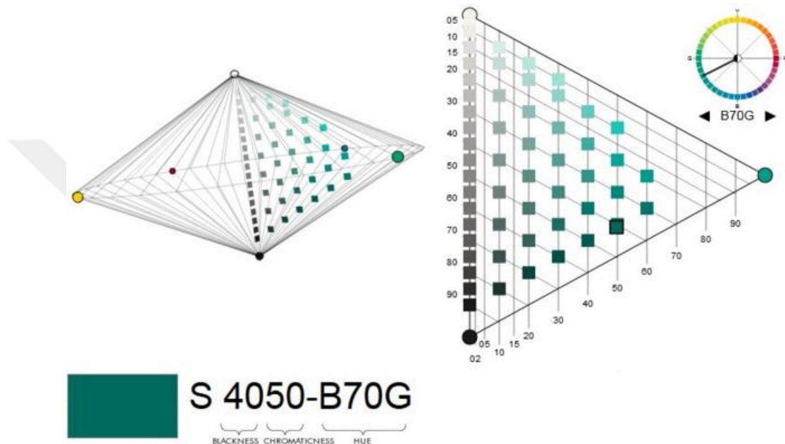
Figure 9. One NCS identification and one NCS hue triangles. (http://www.ncscolour.com/en/design-architecture/work-digitally-with-ncs/ncs-navigator/)
