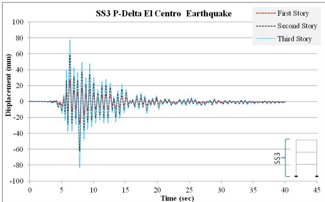
Figure B.14: SS3 P-Delta El Centro earthquake story displacements versus time.
