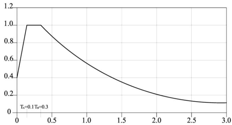
Figure 5.1: Elastic design spectrum.
