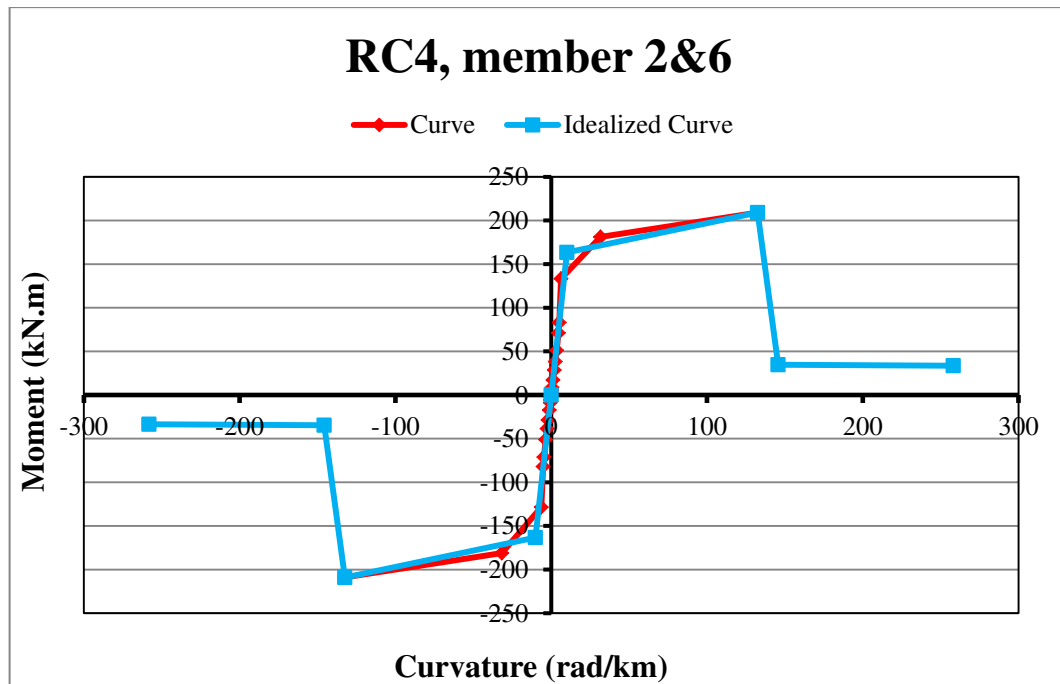
Figure A.5: RC4 Moment-curvature relation of column 2&6 ( N = -150.32 \text{ kN} )
