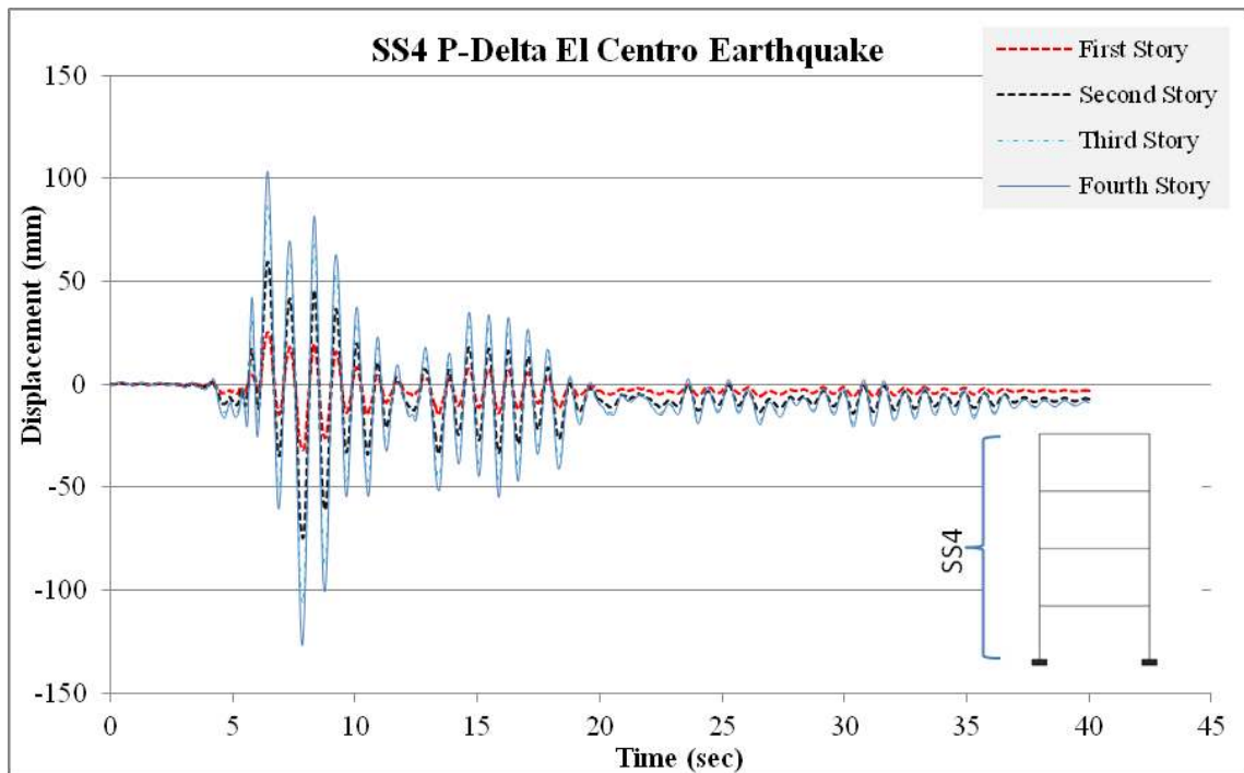
Figure B.32: SS4 P-Delta El Centro earthquake story displacements versus time.
