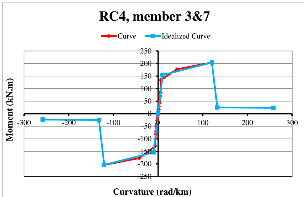
Figure A.6: RC4 Moment-curvature relation of column 3&7 ( N = -100.2 \text{ kN} )
