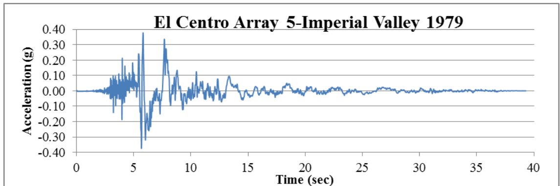
Figure 5.3: El Centro earthquake 1979 ground motion record.
