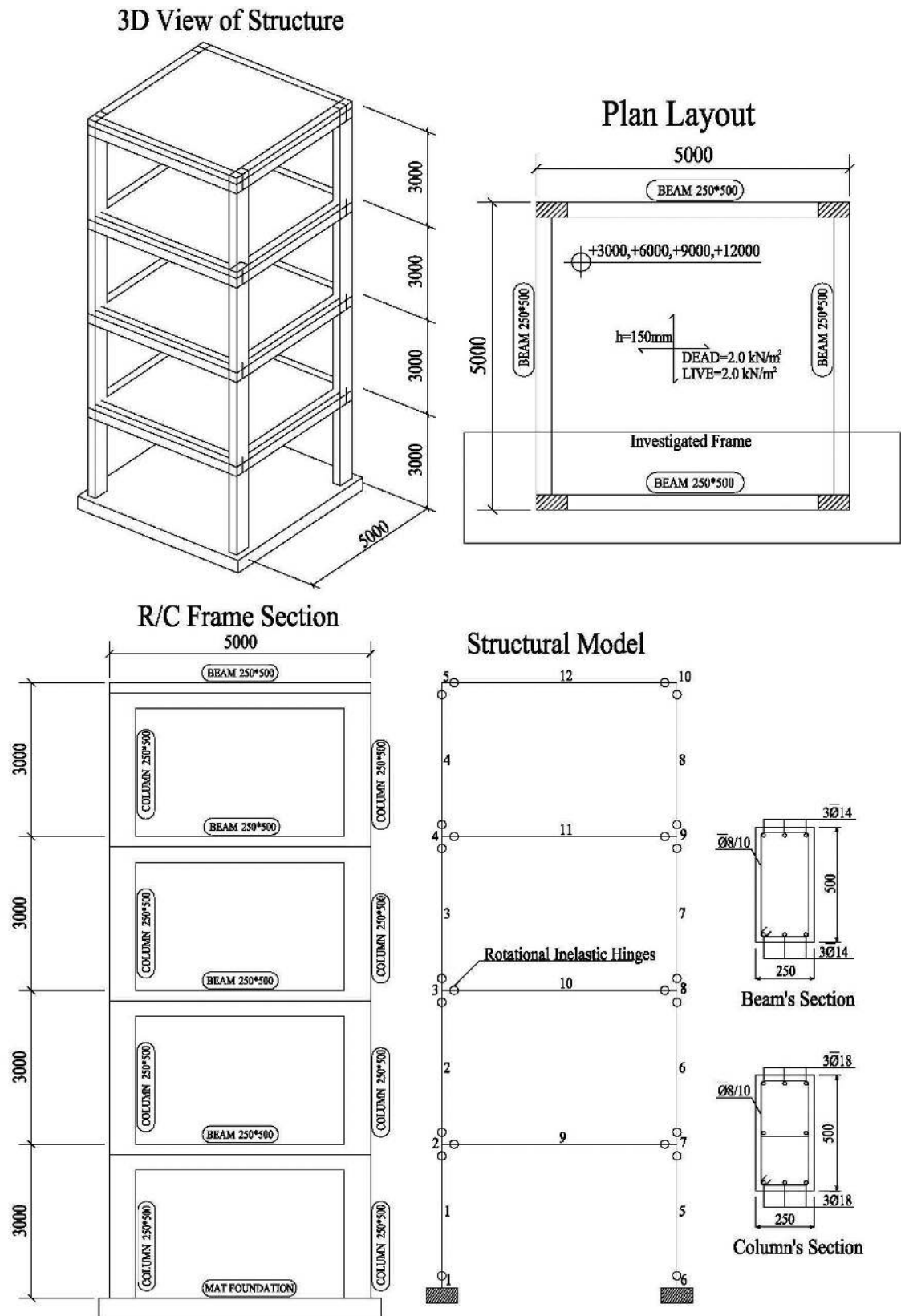
Figure 4.4: Model RC4 details, RC structural frame.
