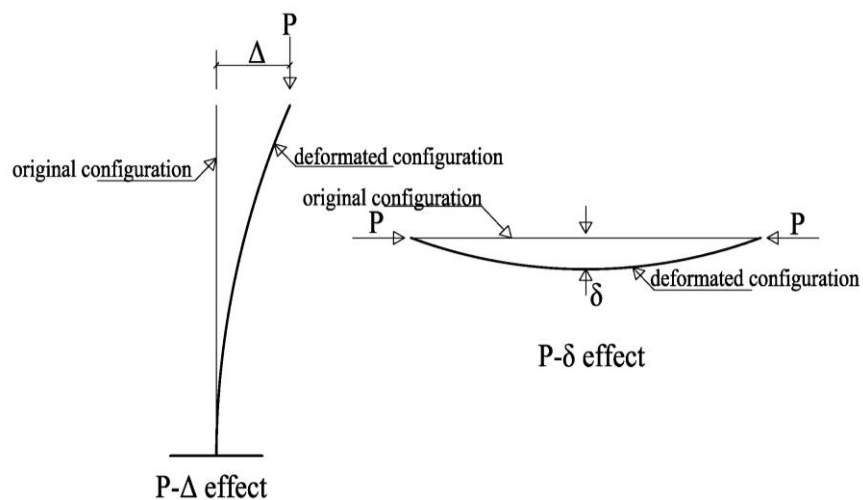
Figure 3.1: P-\Delta and P-\delta effects (Li 1996).
