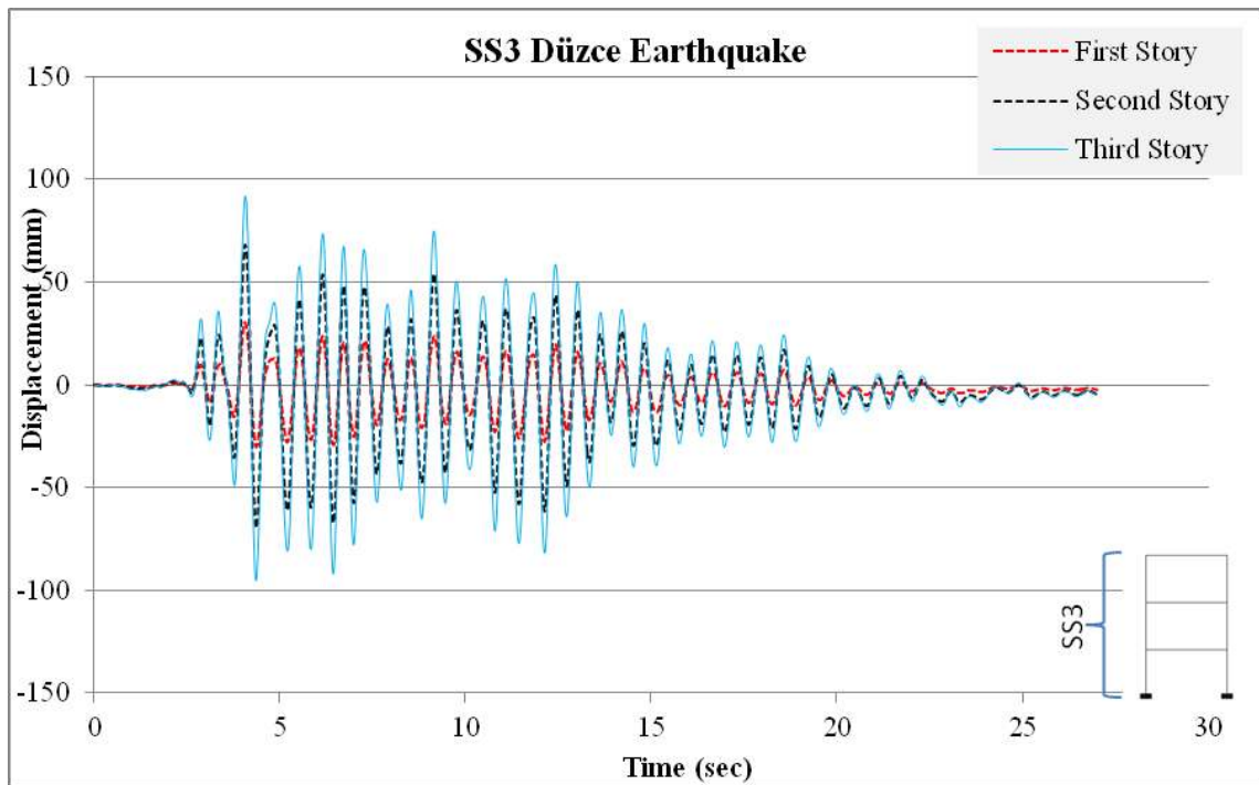
Figure B.4: SS3 Düzce earthquake story displacements versus time.
