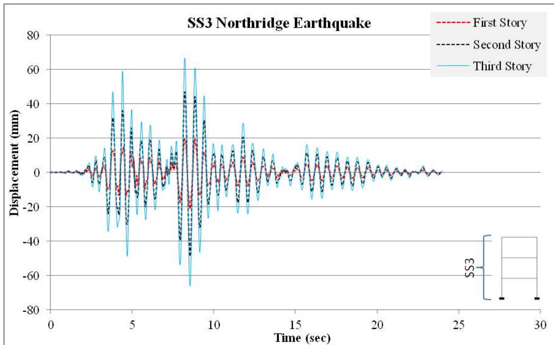
Figure B.6: SS3 Northridge earthquake story displacements versus time.
