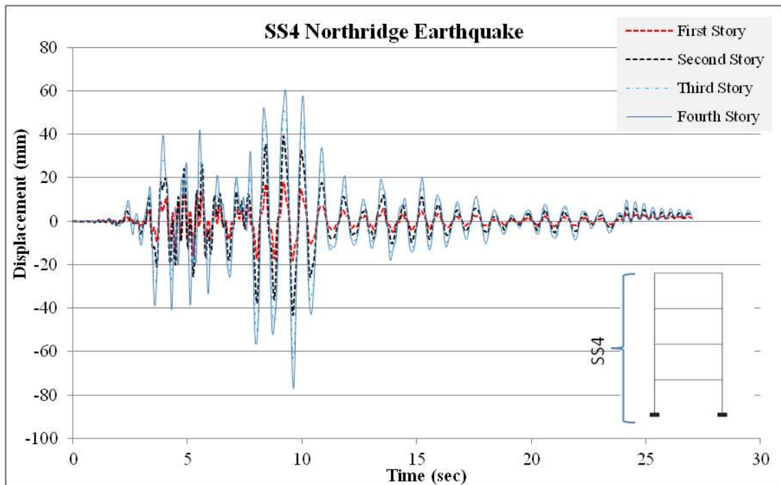
Figure B.24: SS4 Northridge earthquake story displacements versus time.
