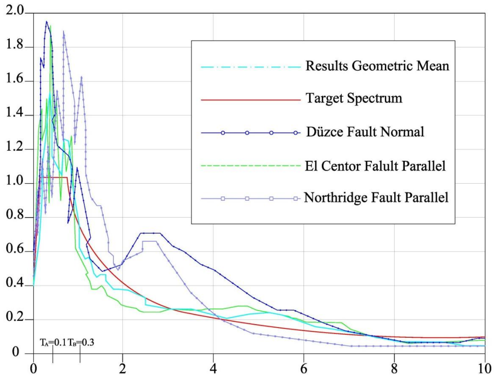
Figure 5.5: Elastic target spectrum and scaled earthquake spectra.
