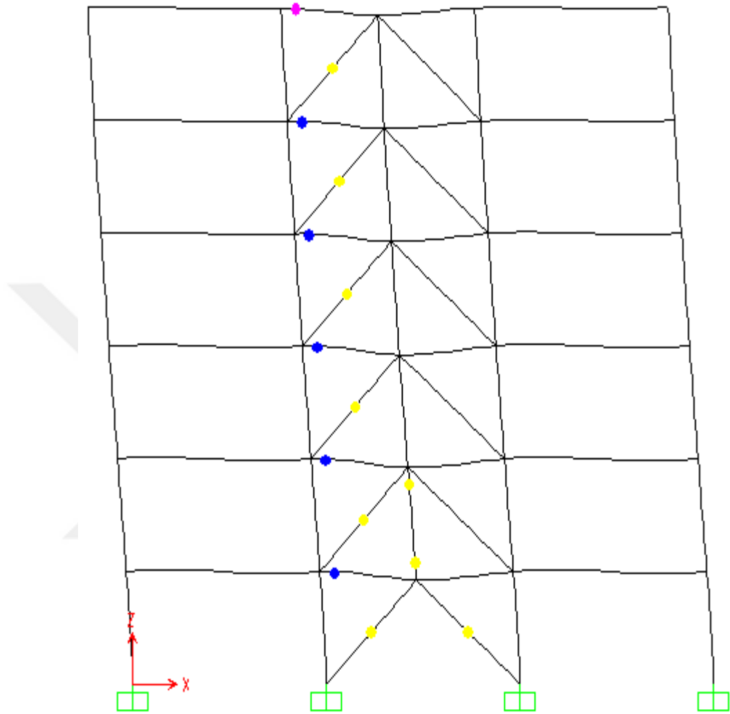
Figure A5 The hinge formation for six story single zipper braced frame under Chi-Chi earthquake
