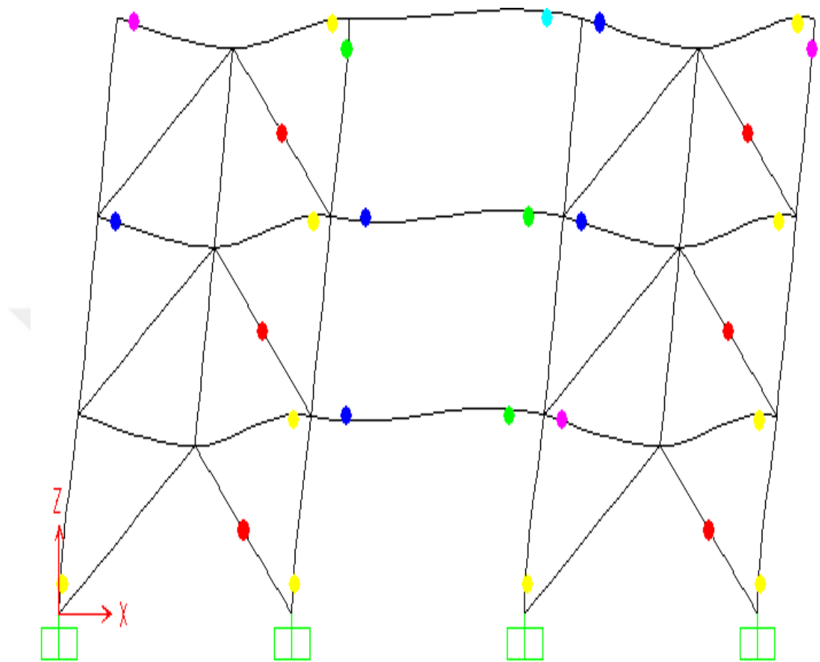
Figure A3 The hinge formation for three story double zipper braced frame under Hector Mine earthquake
