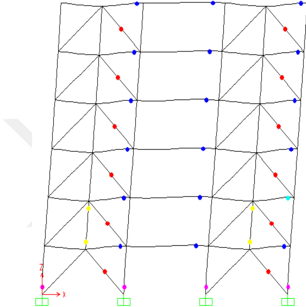
Figure A6 The hinge formation for six story double zipper braced frame under Chi-Chi earthquake
