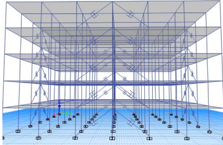
Figure 25: Dampers distribution in the middle of the outer frame
