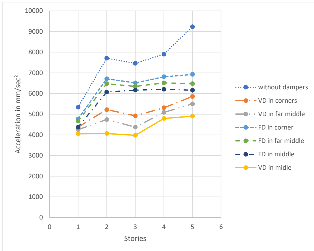
Figure 37: Stories Acceleration for five stories buildings in X direction
