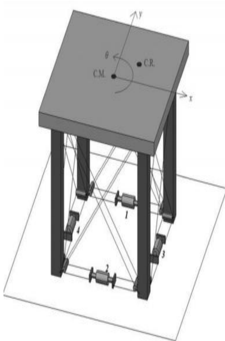
Figure 12: 3D view of ATCS single-story structure (Nigdeli & Boduroğlu, 2013)
