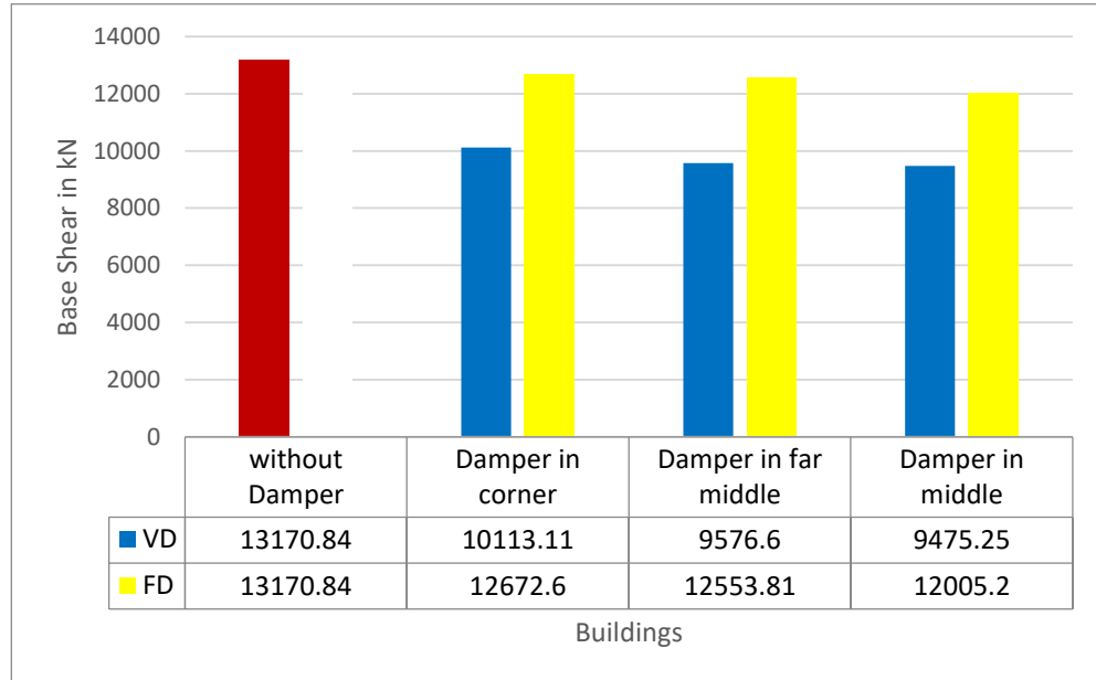
Figure 31: Base Shear for five stories buildings in X direction
