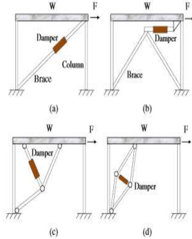
Figure 2: Illustration of dampers implementation ways: (a) diagonal; (b) chevron; (c) toggle; (d) scissor (Guo, Xu, Xu, & Di, 2014).
