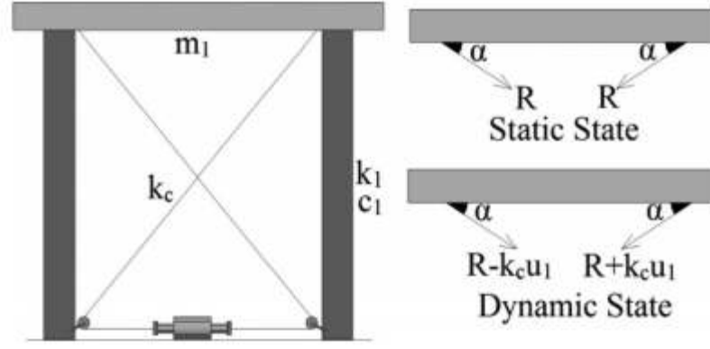
Figure 11: Active tendon control scheme (Nigdeli & Boduroğlu, 2013)
