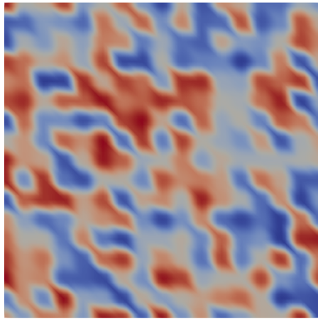
(a) Concentration at t = 0
