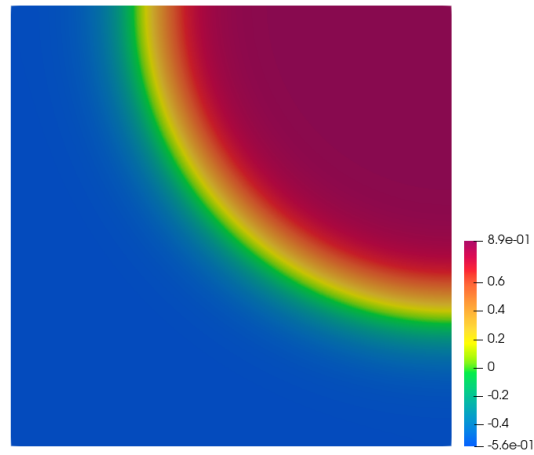
(e) Concentration for f(c) = (c - 0.3)^2(c^2 - 1)
