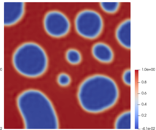
(f) Concentration at t = 0.0025
