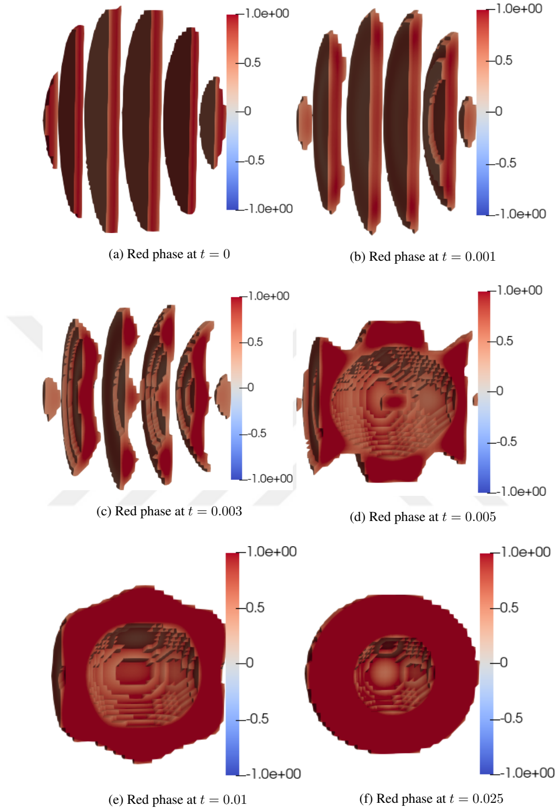
Figure 4.9: Evolution of red phase in the copolymer. The combination of Figures 4.8 and 4.9 gives Figure 4.6. The color indicates the c_2 field.
