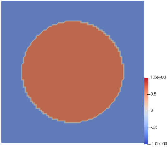
(a) c_1 at t = 0
