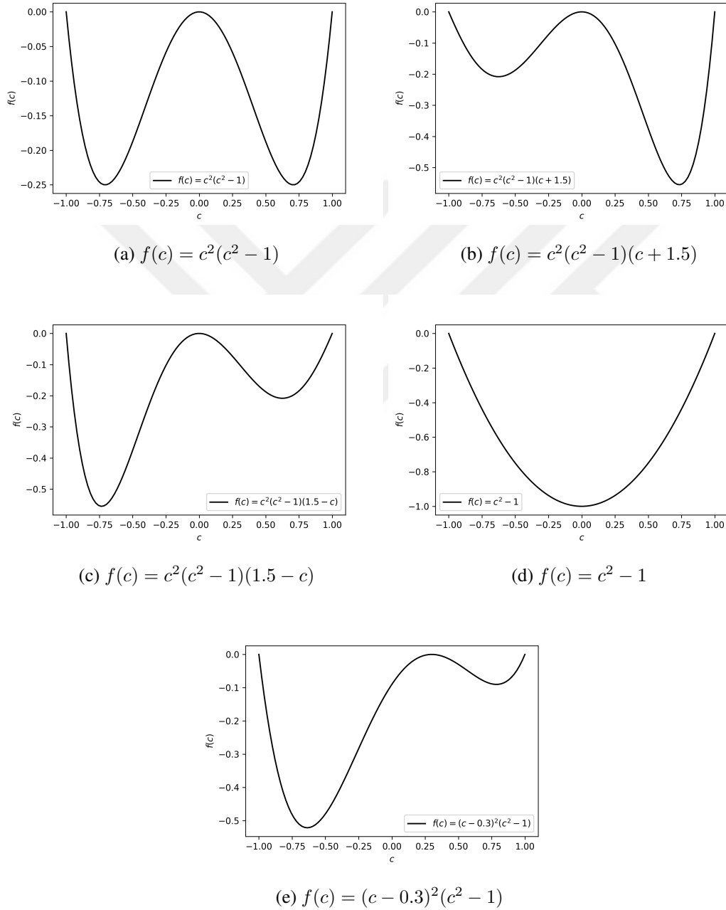
Figure 2.10: Different free energy function functions for the CH problem
