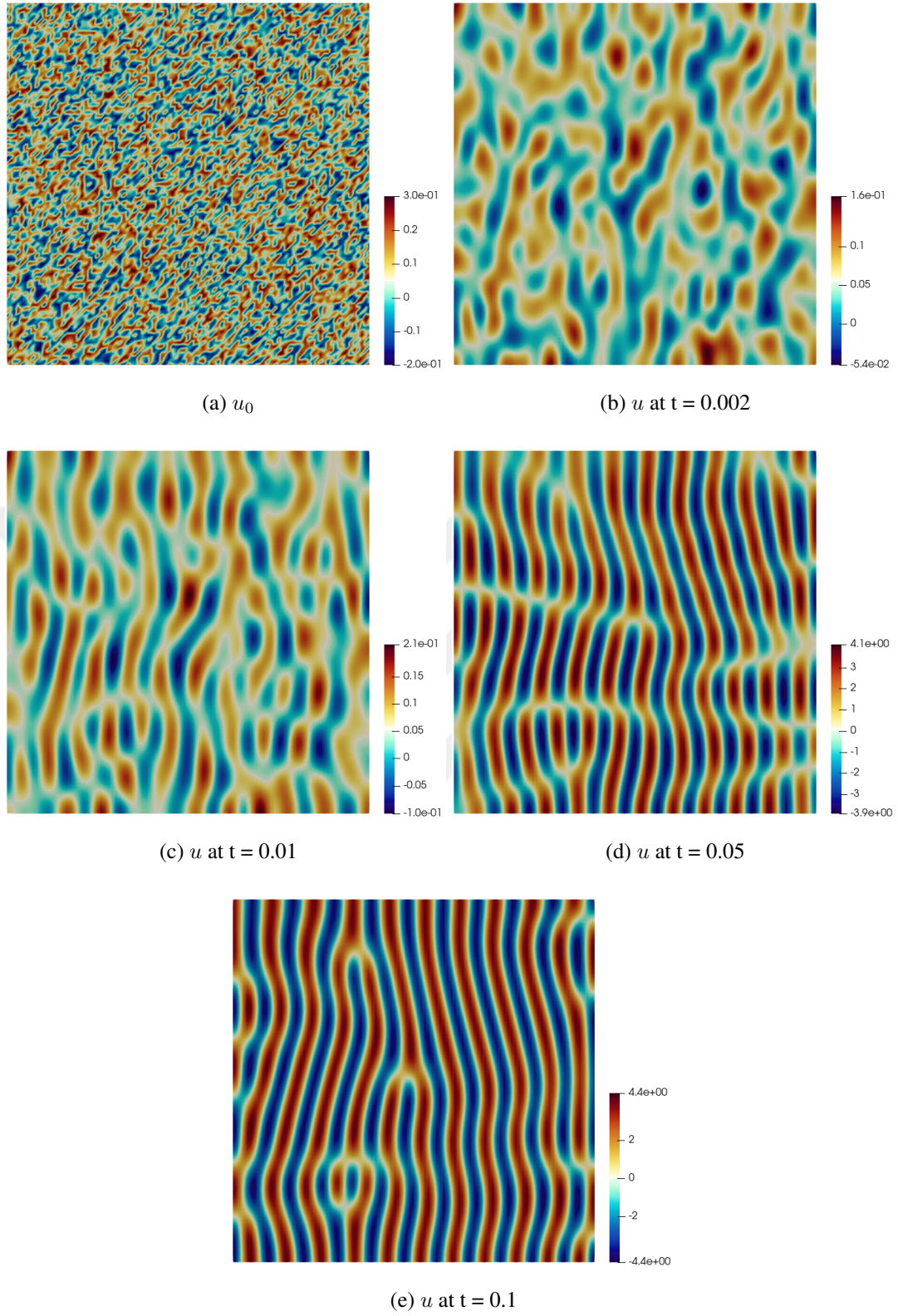
Figure 2.23: Solutions of phase-field crystal example 2. The color indicates the value of u field.
