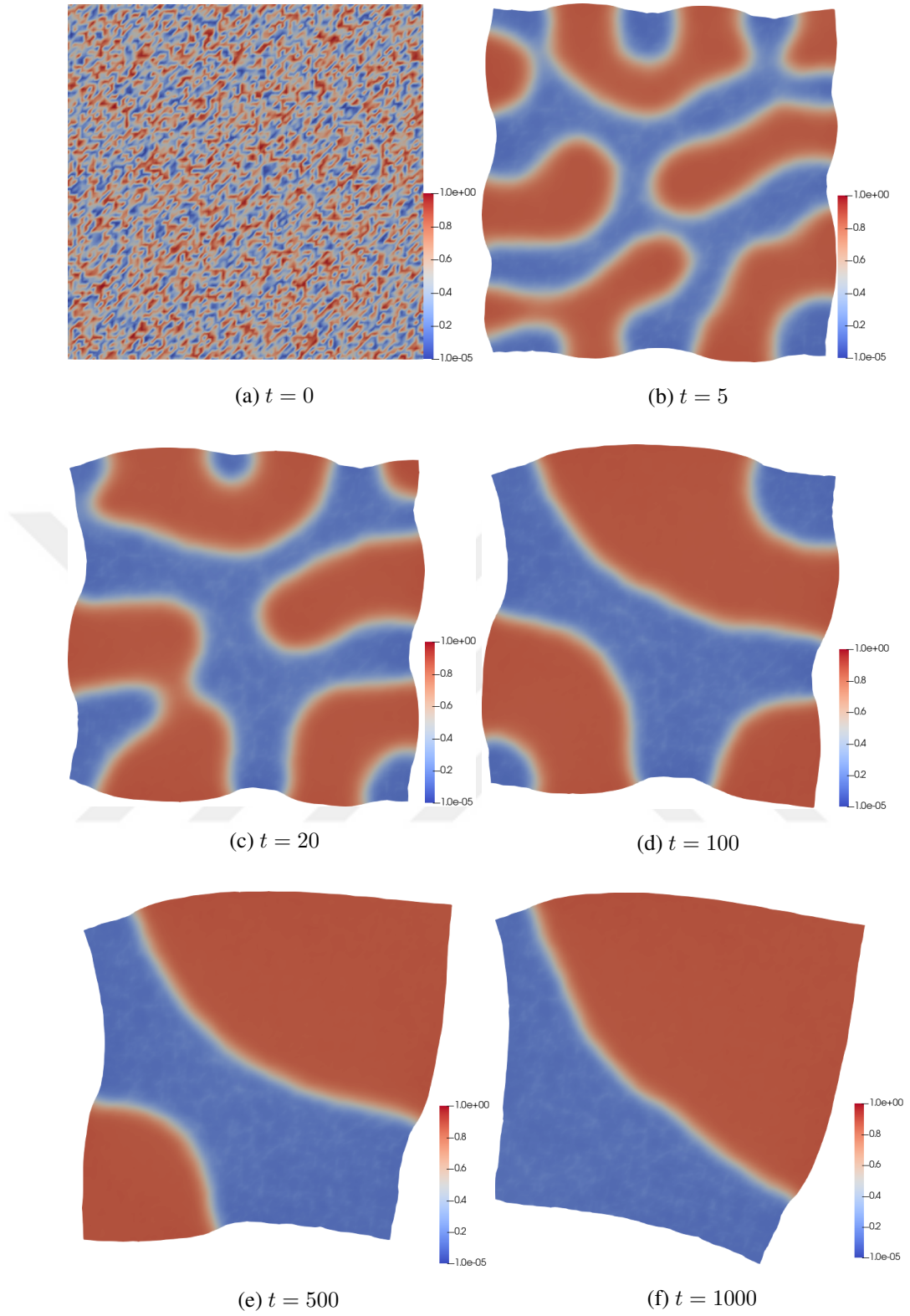
Figure 3.3: Solution of the Cahn-Hilliard problem coupled with finite elasticity in the two-dimensional domain. The color indicates the concentration field, and deformed shapes show the deformation field.
