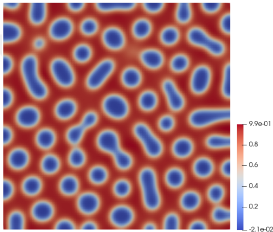
(c) Concentration at t = 0.0001
