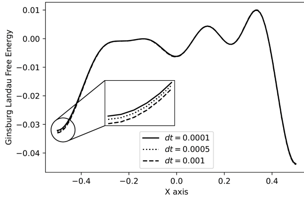
(c) Ginzburg-Landau Free Energy vs x axis for different time steps
