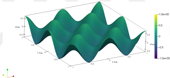
(c) Concentration at t = 5
