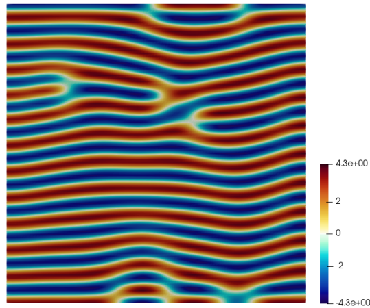
(e) u at t = 0.1
