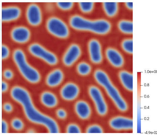
(c) Concentration at t = 0.0001
