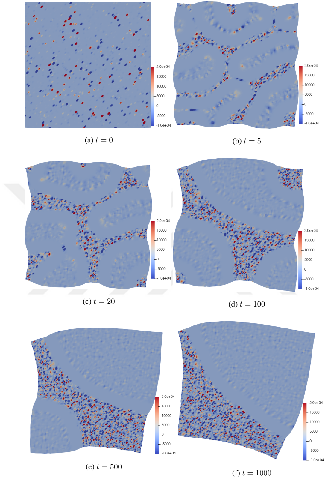
Figure 3.5: Gaussian curvature of the concentration field in Figure 3.3. The color indicates the Gaussian curvature field
