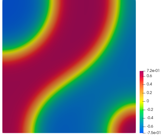
(b) Concentration for f(c) = c^2(c^2 - 1)(c + 1.5)
