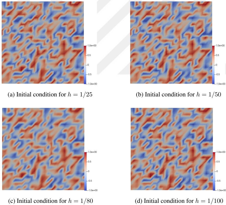
Figure 2.4: Finer meshes have the same pattern as the initial condition of the coarsest mesh. Four uniform meshes ( 50 \times 25 = 1250 , 100 \times 50 = 5000 , 160 \times 80 = 12800 and 200 \times 100 = 20000 T1 elements) are presented
