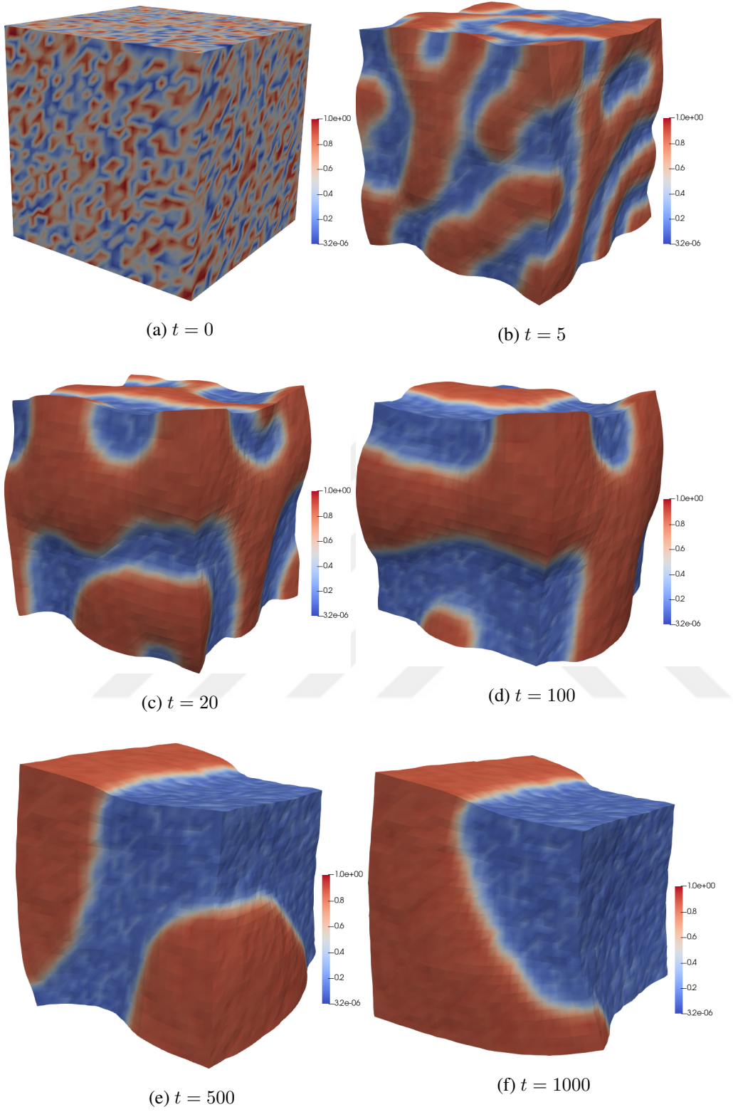
Figure 3.6: Solution of the Cahn-Hilliard problem coupled with finite elasticity in the three-dimensional domain. The color indicates the concentration field, and deformed shapes show the deformation field.
