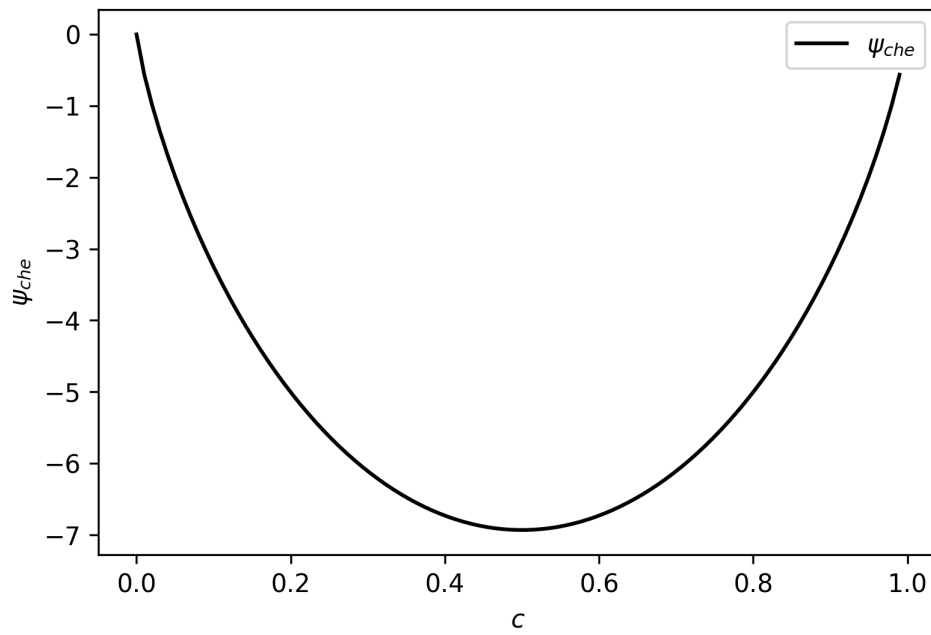
(b) Chemical energy, \psi_{che} for a = 10, b = 0
