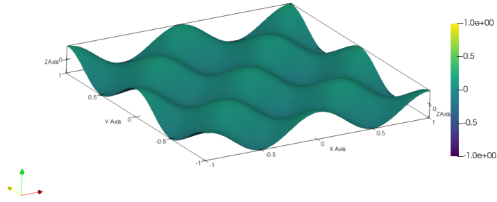
(a) Concentration at t = 0.5
