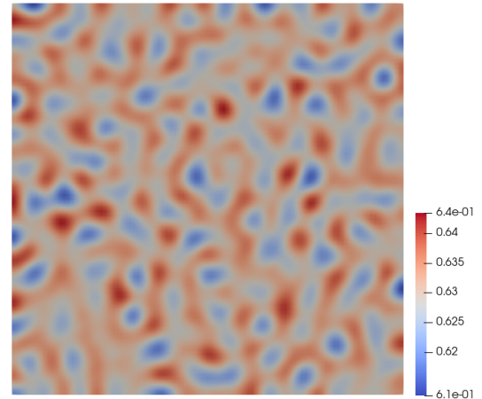
(b) Concentration at t = 0.00001
