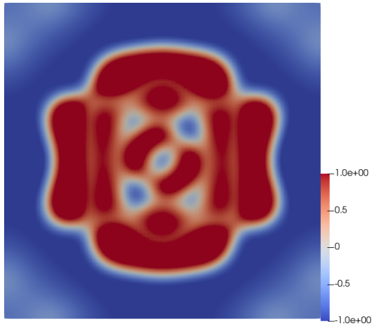
(e) c_1 at t = 0.01
