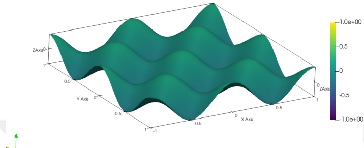
(b) Concentration at t = 2.5
