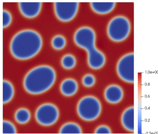
(e) Concentration at t = 0.001
