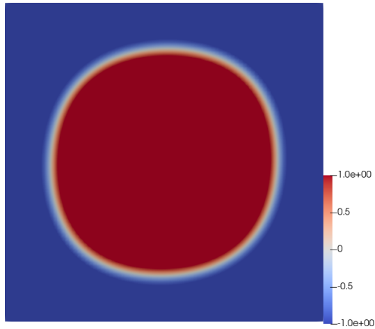
(f) c_1 at t = 1
