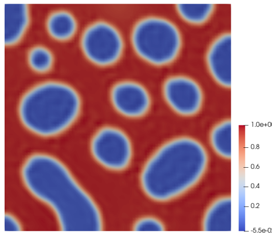
(e) Concentration at t = 0.001
