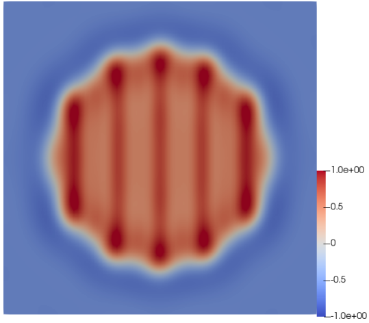
(b) c_1 at t = 0.001
