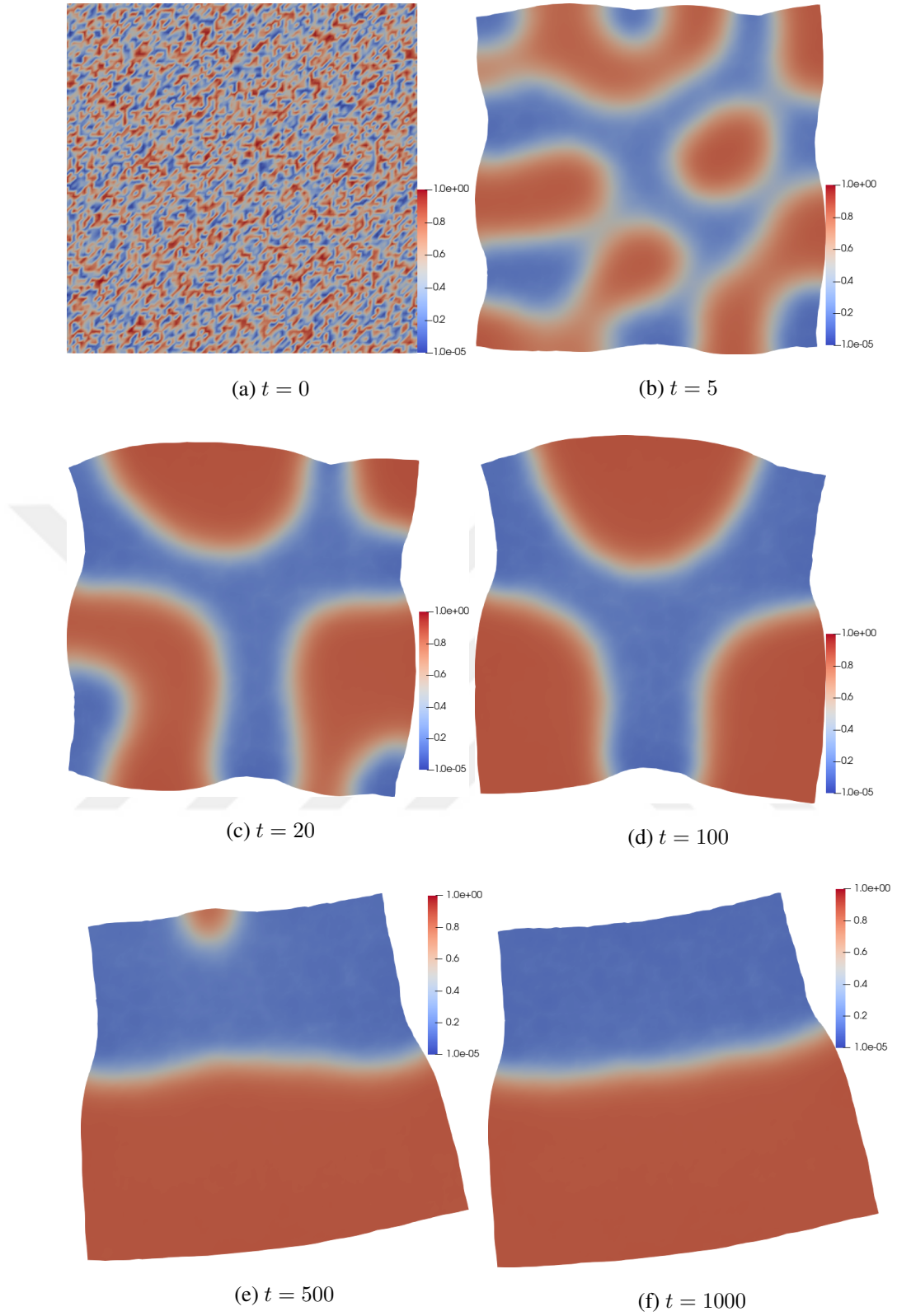
Figure 3.7: Solution of the Cahn-Hilliard problem coupled with the finite elasticity considering the additional interface stretch term in the two-dimensional domain. The color indicates the concentration field, and deformed shapes show the deformation field.
