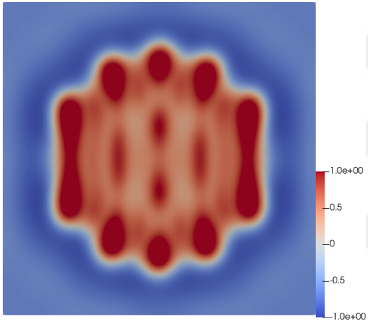
(c) c_1 at t = 0.003
