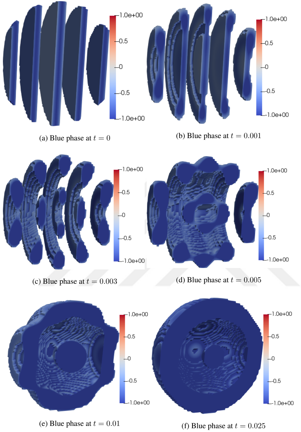
Figure 4.8: Evolution of blue phase in the copolymer. The blue phase and red phase in Figure 4.6 depict the onion shape formation. The color indicates the c_2 field.
