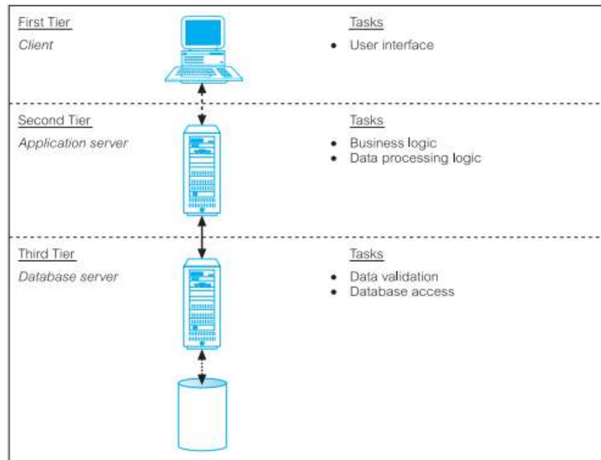
Figure 3 Three-tier architecture
