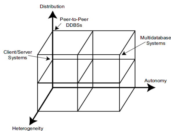
Figure 5 Implementation alternatives
