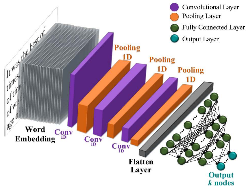
Figure 2: Architecture of CNN Layers
