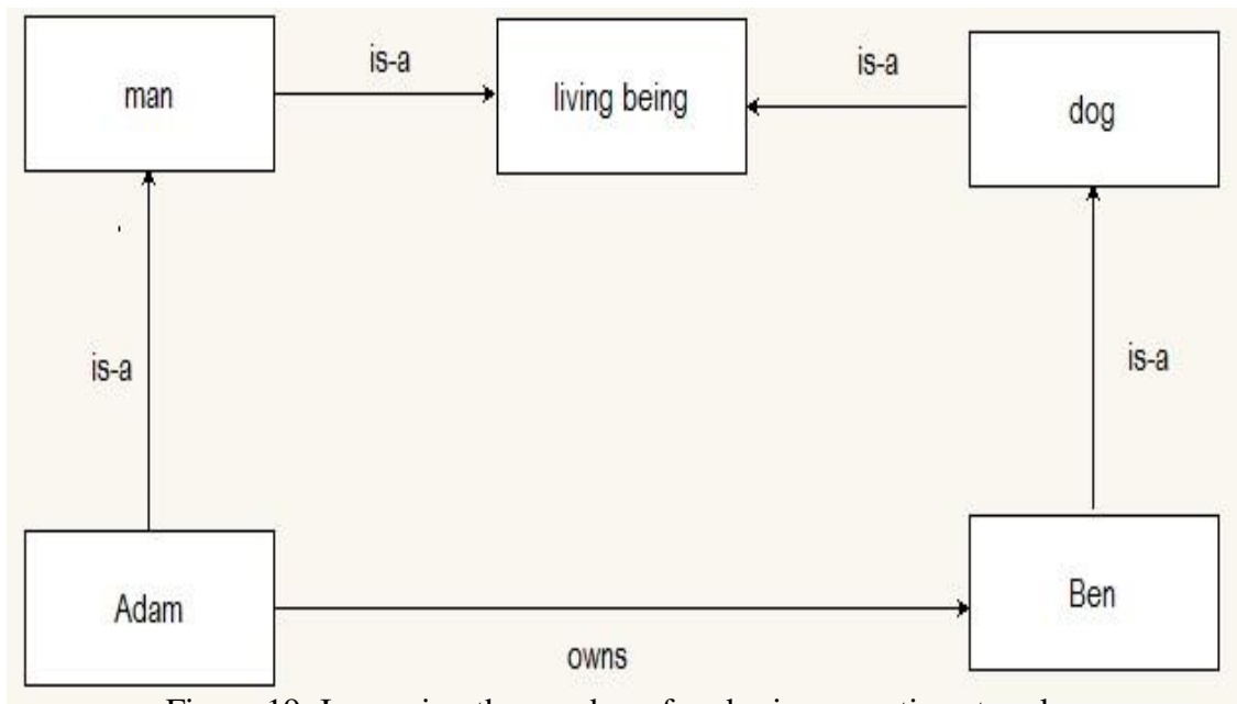
Figure 19: Increasing the number of nodes in semantic network
