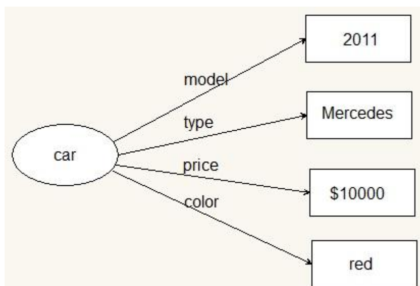
Figure 7: OAV triplets with multiple attribute values
