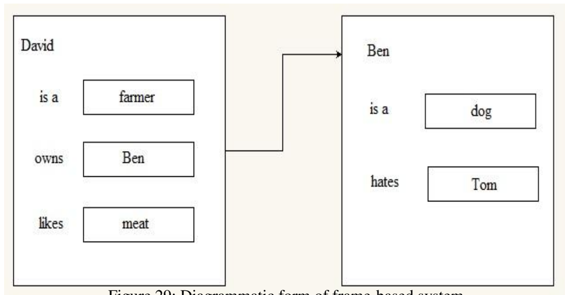
Figure 29: Diagrammatic form of frame-based system
