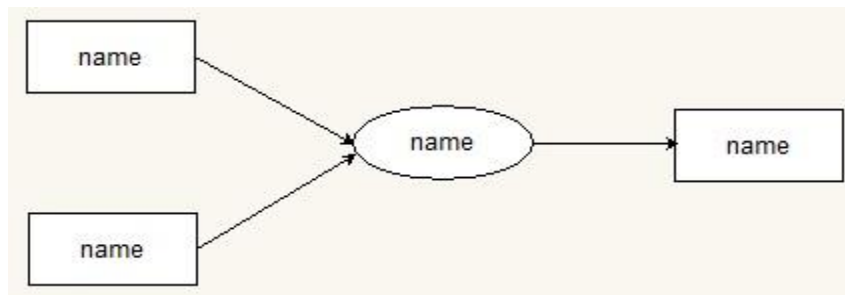
Figure 14. The 3-adic relation
