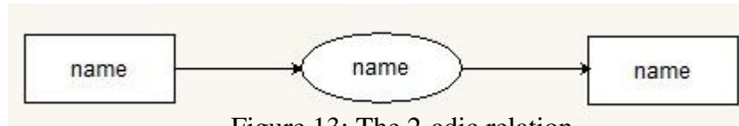
Figure 13: The 2-adic relation
