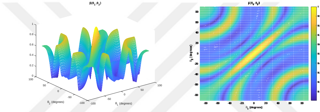
Figure 3.5. Correlation between True and False Array Steering Vectors
