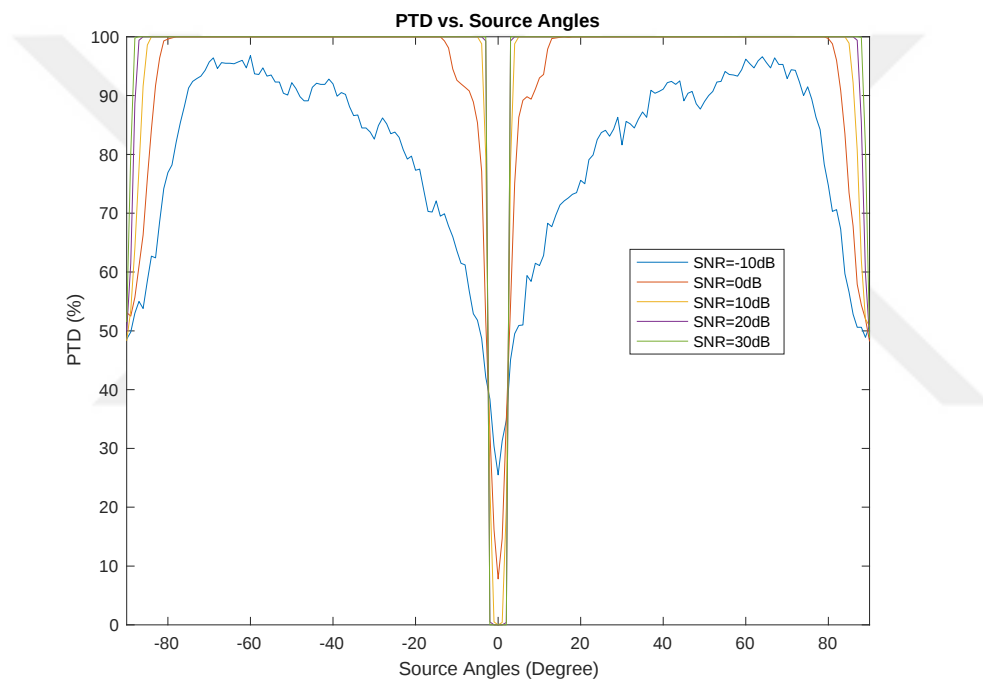
Figure 4.4. PTD of Scenario 1, M = 6 , Case 1
