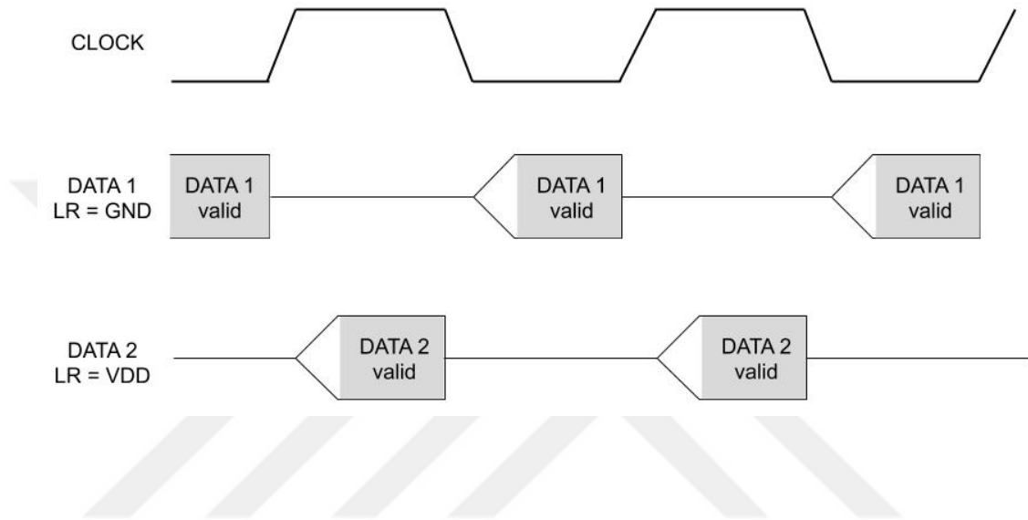
Figure 3.2. Timing Diagram of MEMS microphone
