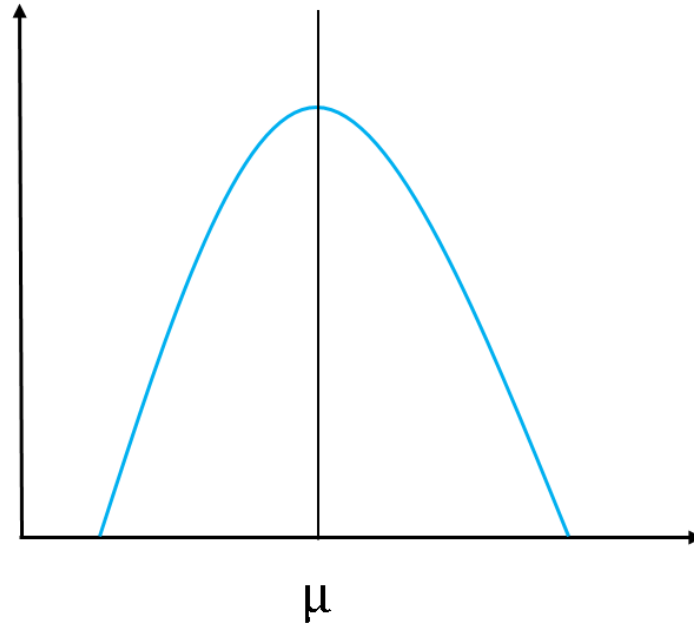
Figure 4.4. The Gaussian distribution
