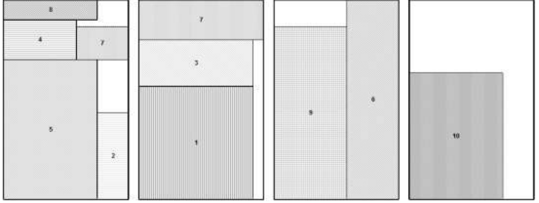
Figure 5.4 A feasible fuzzy SRP solution
