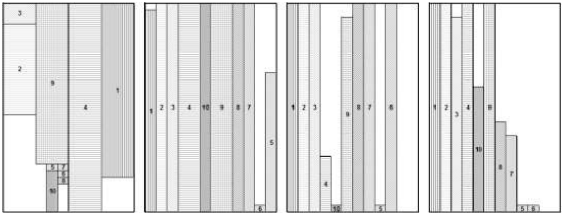
Figure 4.7 SRP-III optimal packing by 40 rectangles of a problem with 10 users over 4 frames with traffic distribution TR1 ; with average user demand of 102 slots
