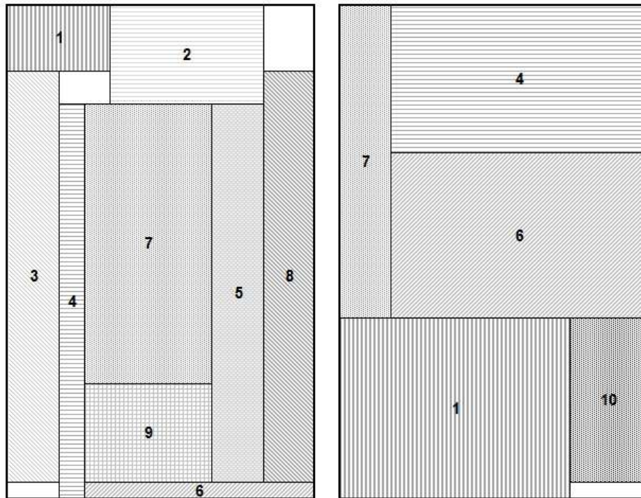
Figure 4.3 SRP-II solution for a problem with 10 users packed over 2 frames
