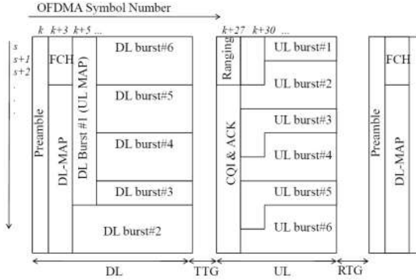
Figure 2.2 A sample OFDMA frame structure in TDD mode (Source: So-In et al., 2009b, pp. 1)
