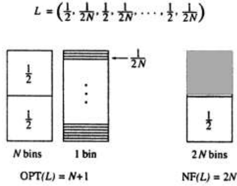
Figure 2.1 Worst-case example for the Next-Fit algorithm (Source: Coffman et al. 1996, p. 49)
