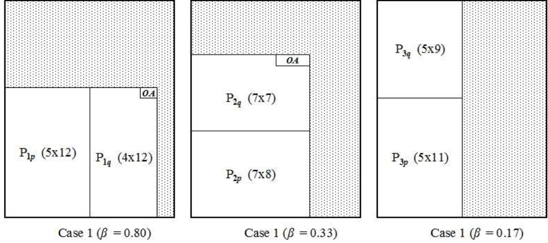
Figure 5.2 Possible placements of two users with fuzzy demands on a frame
