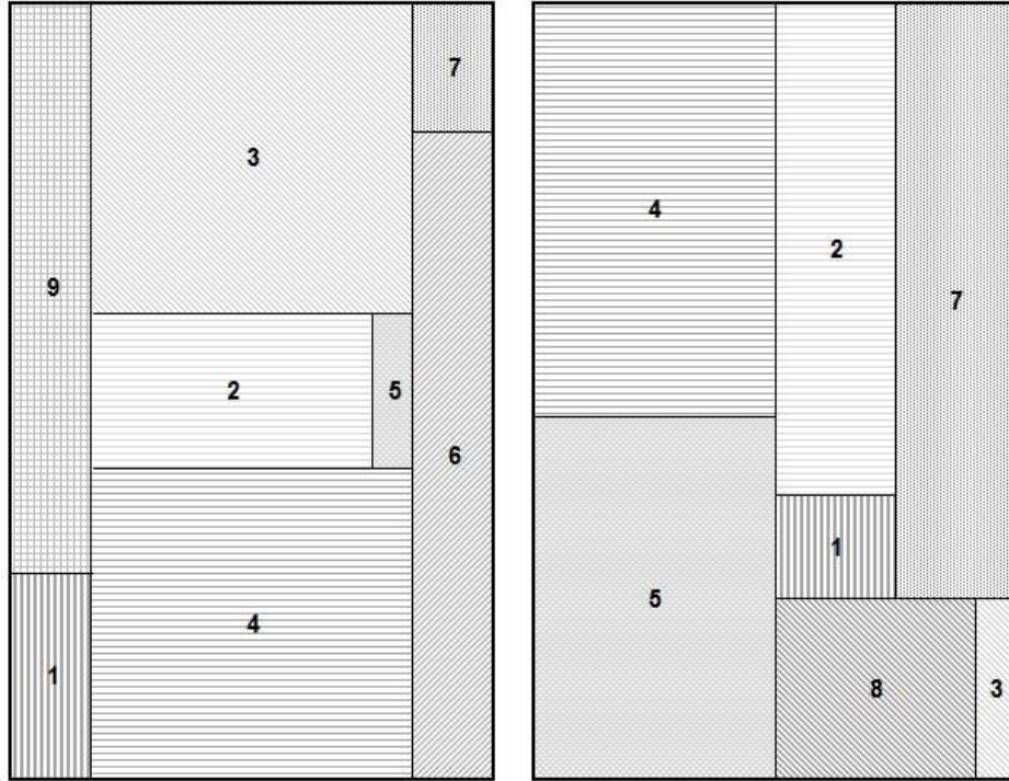
Figure 4.5 SRP-I solution for a problem with 10 users packed over 2 frames with traffic distribution TRI (75% of users with data + 25% voice traffic)
