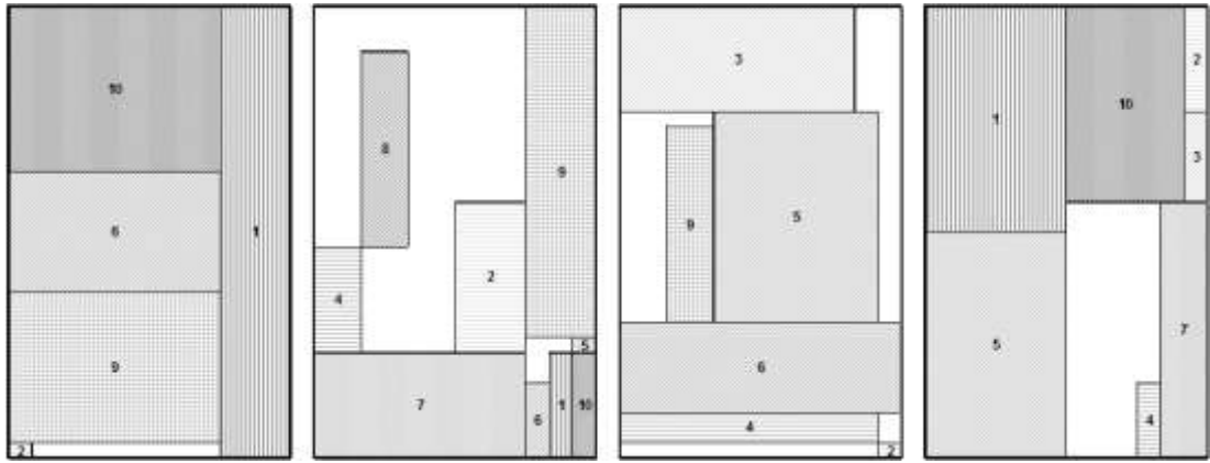
Figure 4.6 SRP-III optimal packing by 27 rectangles of a problem with 10 users over 4 frames with traffic distribution TR1 (75% of users with data + 25% voice traffic); with average user demand of 116 slots
