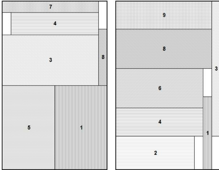
Figure 4.2 SRP-I solution for the same problem employing bounds
