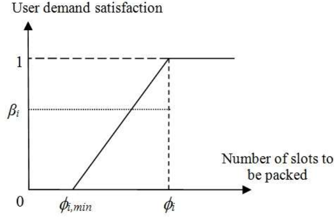
Figure 5.3 Fuzzy demand parameter definition for the SRP-I model
