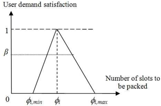
Figure 5.1 A general fuzzy demand parameter definition for SRP models
