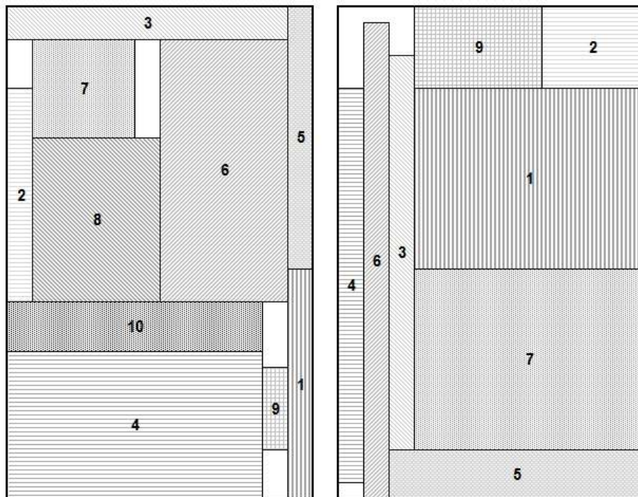
Figure 4.4 SRP-III solution for the same problem with 10 users over 2 frames
