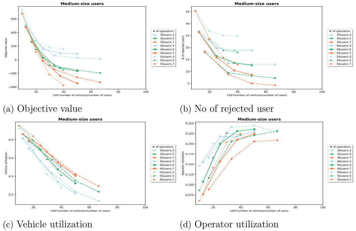
Figure 4.3 Operator-based model plots for medium-size users (Fixed number of operators)
