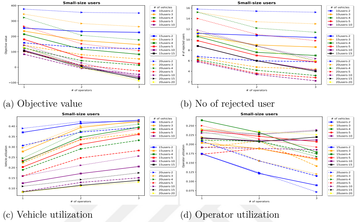
Figure 4.8 Operator-based model plots for small-size users (Fixed number of vehicles)
