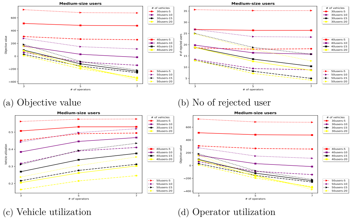
Figure 4.9 Operator-based model plots for medium-size users (Fixed number of vehicles)
