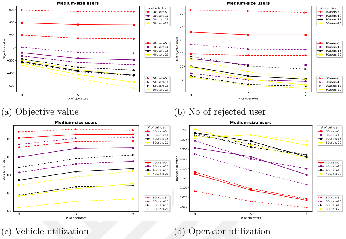
Figure 4.12 Hybrid model plots for medium-size users (Fixed number of vehicles)
