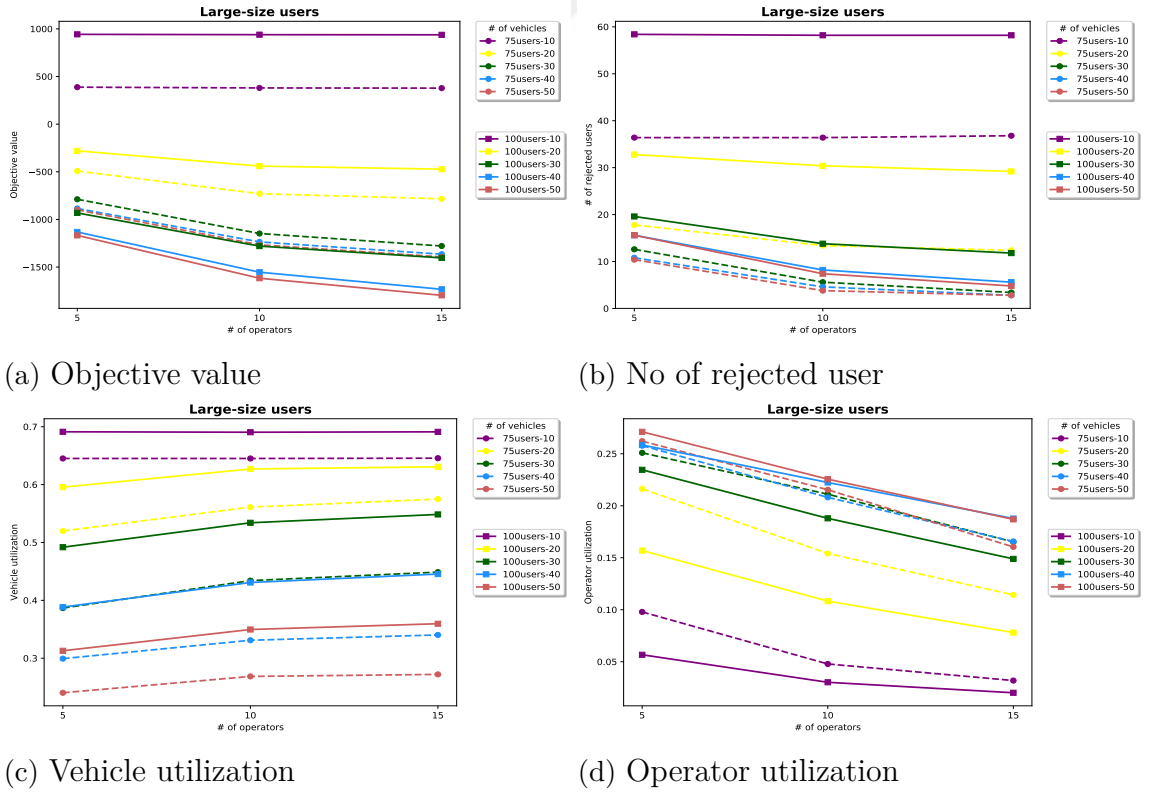
Figure 4.13 Hybrid model plots for large-size users (Fixed number of vehicles)
