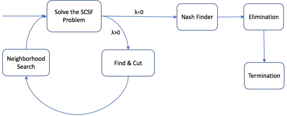
Figure 4.3 SwpN-NS Algorithm
