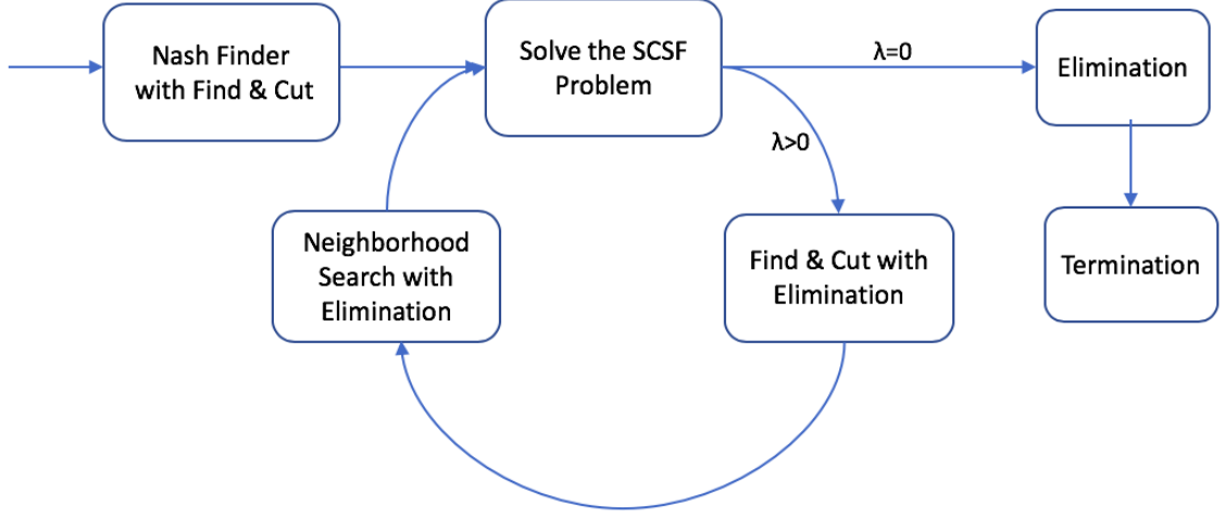
Figure 4.5 pp-SwpN-NS Algorithm
