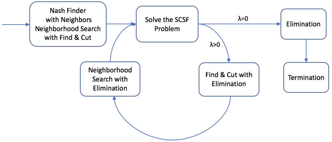
Figure 4.6 pp-SwpN-NoNS Algorithm
