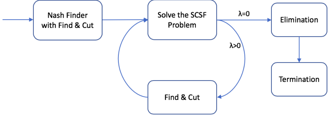
Figure 4.4 pp-SwpN Algorithm
