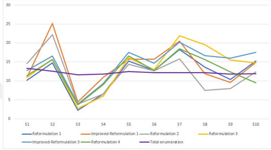
Figure 5.5 CPU time of reformulations for small instance
