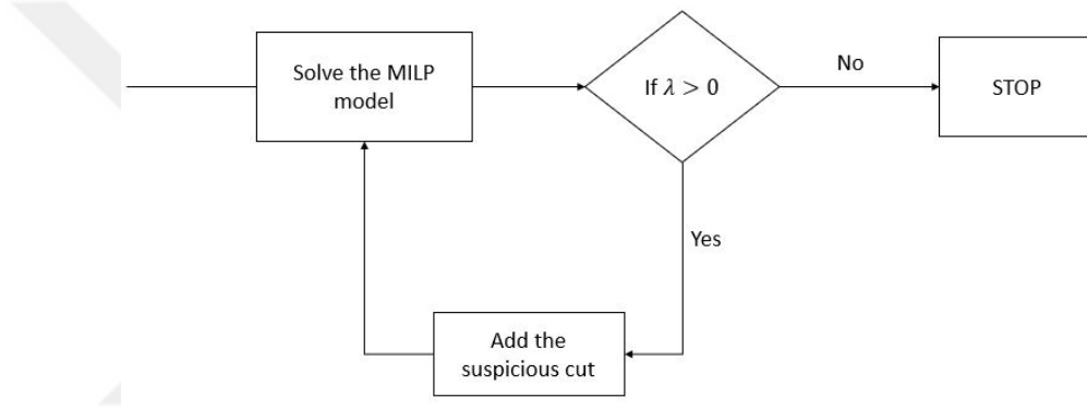
Figure 5.4 Iterative algorithm
