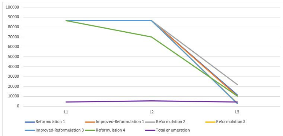
Figure 5.8 CPU time of reformulations for large instances
