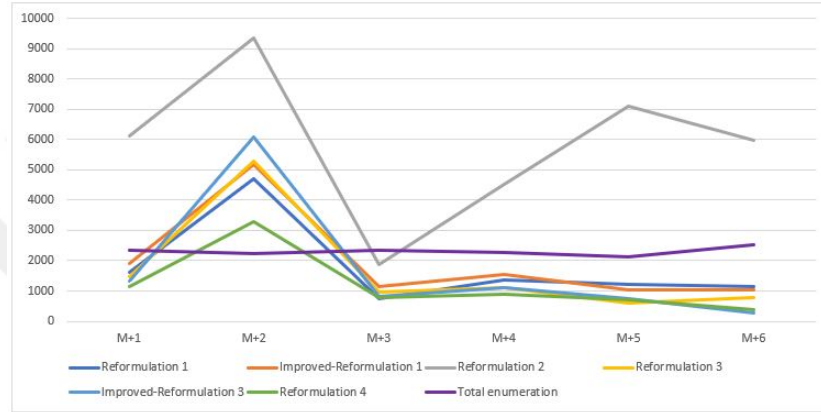
Figure 5.7 CPU time of reformulations for medium-plus instances
