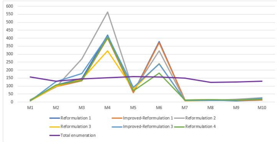
Figure 5.6 CPU time of reformulations for medium instances
