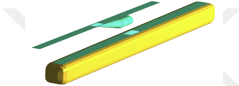
Figure 4.32: Design variable surfaces in blue with and without full body in yellow.
