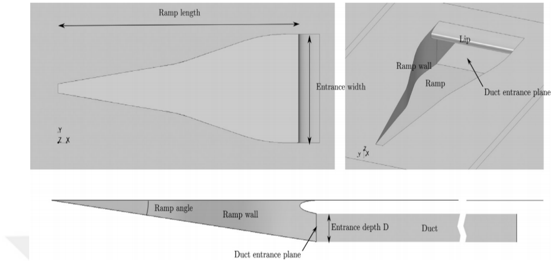
Figure 2.3: Benchmark geometry based on the reference study by Pignier [5].
