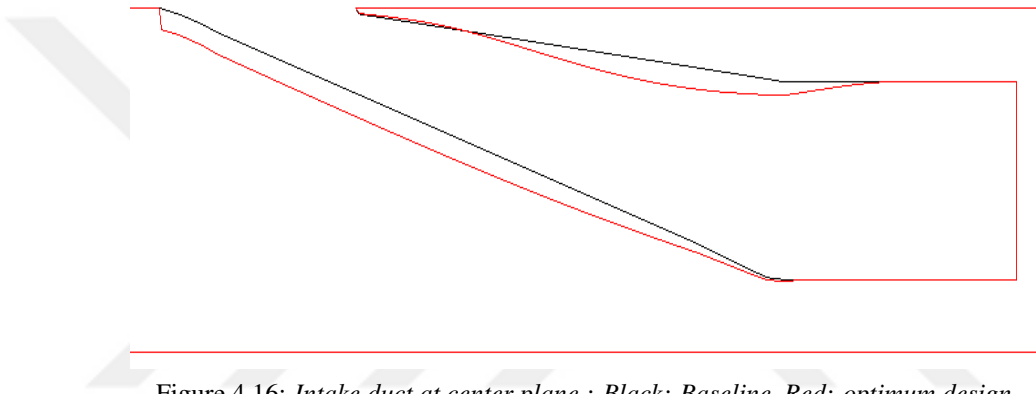
Figure 4.16: Intake duct at center plane : Black: Baseline, Red: optimum design.
