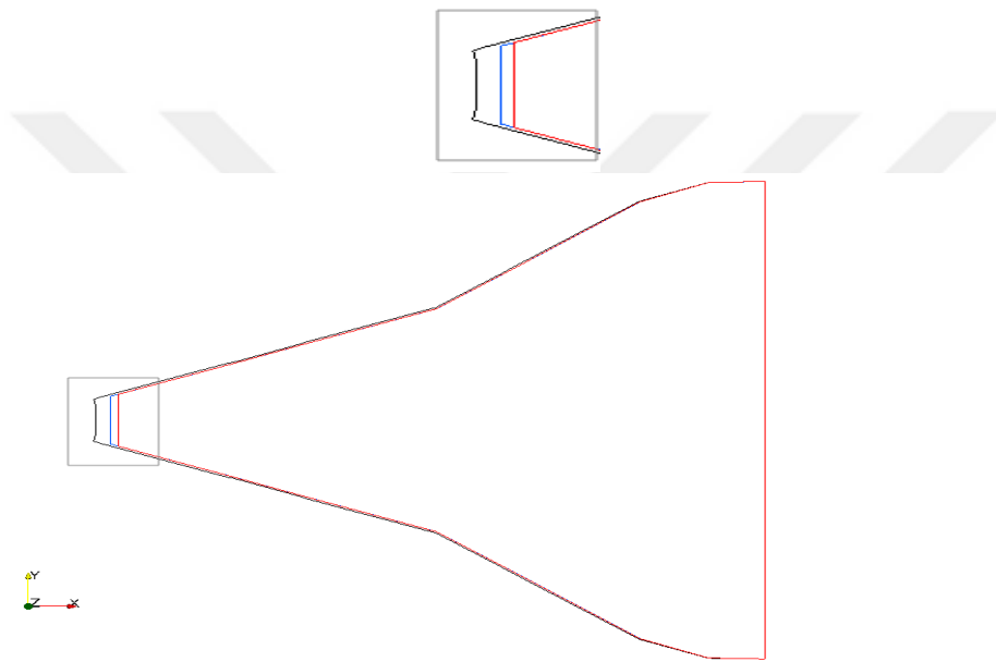
Figure 4.6: NACA intake top view at different optimization steps;
