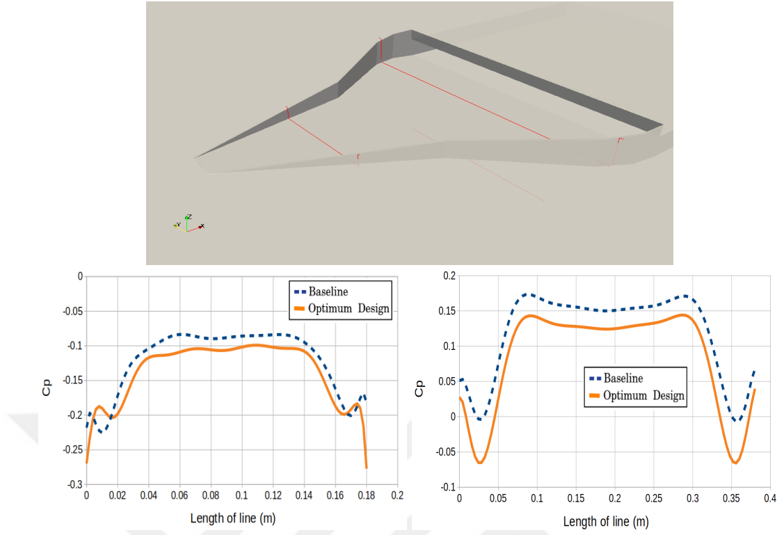
Figure 4.7: C_p distribution along intake ramp sections.
