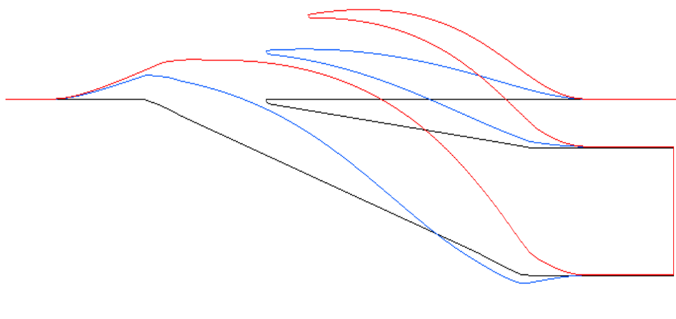
Figure 4.38: Intake duct outlines at center plane ; Black: Baseline, Blue: Intermediate, Red: optimum design.
