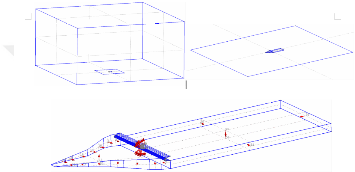
Figure 2.6: Representation of the solid model as imported in GMSH in .stl format.
