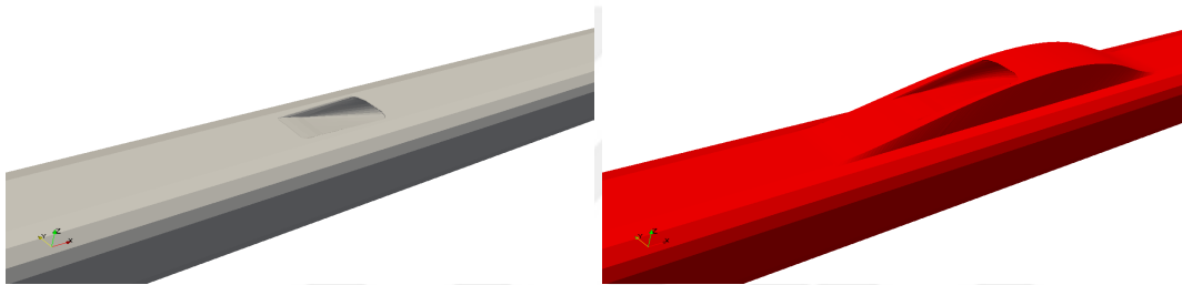
Figure 4.44: Shape deformation for case IV intake; Left: Baseline; Right: Optimum design.
