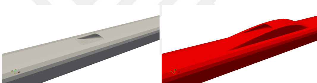
Figure 4.37: 3D view of shape deformation process; Left: Baseline, Right: Optimum design.
