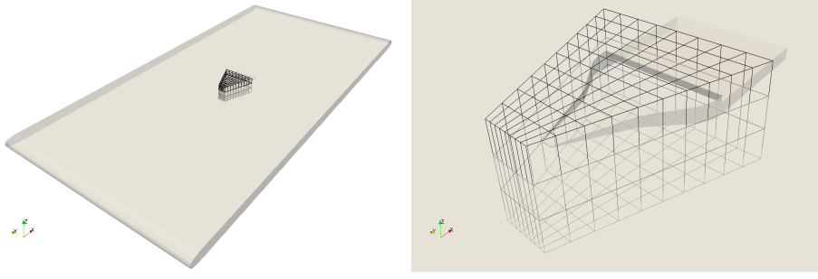
Figure 2.15: FFD box of [11,9,4] configuration for NACA intake on flat plate.
