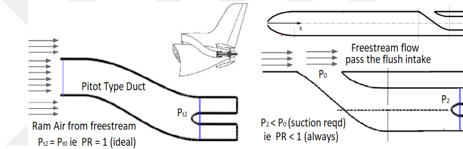
Figure 1.12: Pitot intake vs. submerged intake.
