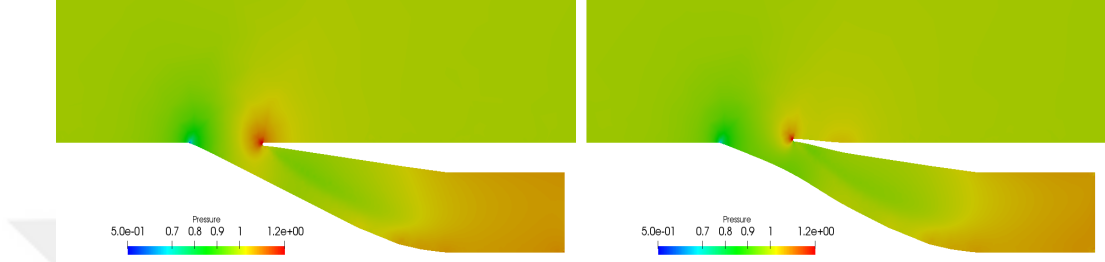
Figure 4.30: Pressure Distribution for Left: Baseline ; Right: Optimum design
