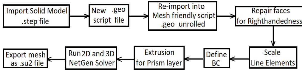
Figure 2.5: Mesh generation flow chart in GMSH
