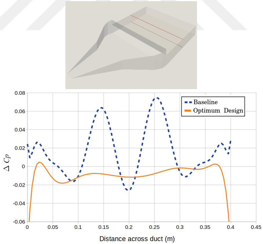
Figure 4.8: \Delta C_p distribution between upper and lower duct walls.
