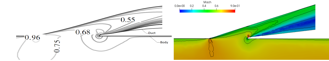
Figure 3.15: Mach contours. left: Reference study [4] Right: Baseline solution.
