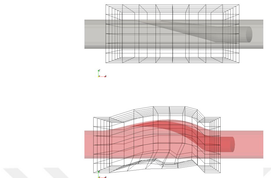
Figure 4.36: FFD Box deformation; Top: Baseline; Bottom: Optimum design.
