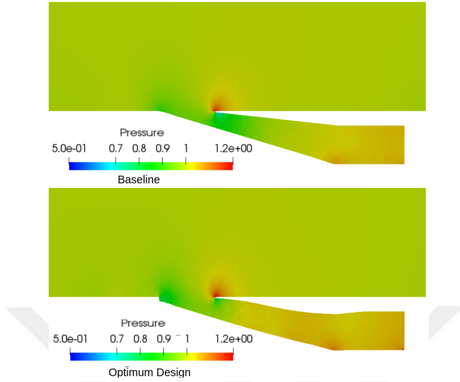
Figure 4.18: Pressure distribution on center-plane - Top: Baseline , Bottom: Optimum design.
