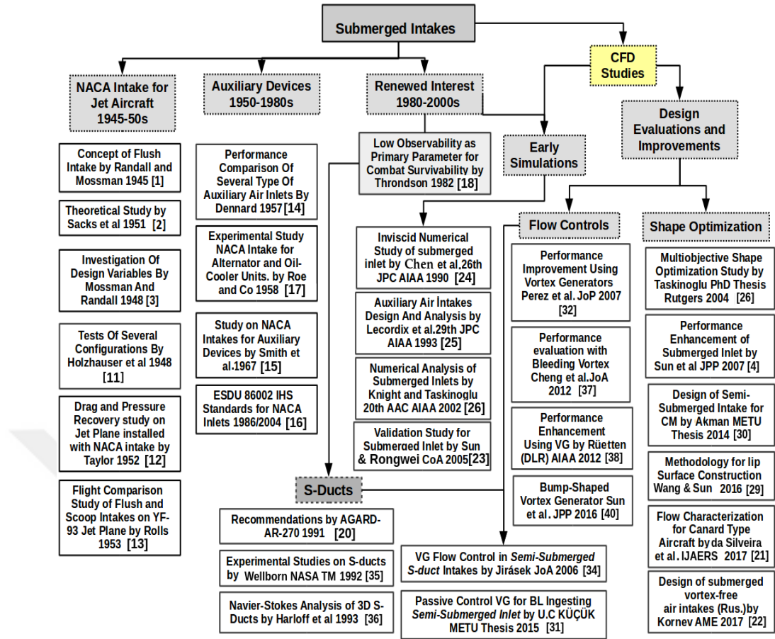
Figure 1.5: A hierarchical representation of salient studies on submerged intake
