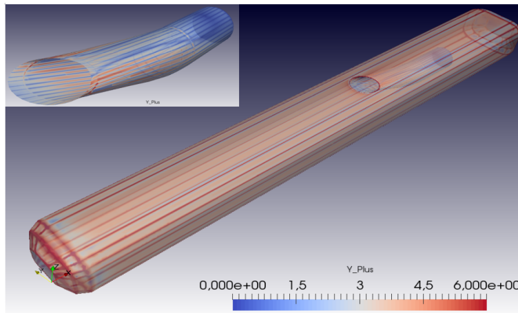
Figure 4.22: Y+ Distribution on surface.
