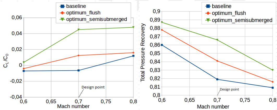
Figure 4.46: Off-design performance at different Mach numbers for fixed \alpha=0^\circ .
