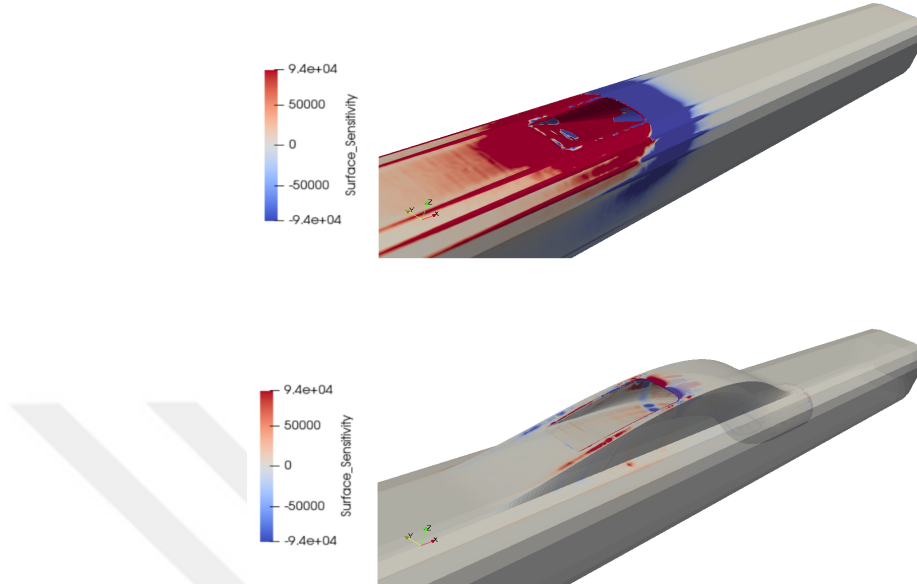
Figure 4.34: Surface sensitivity: Top Baseline; Bottom Optimum design
