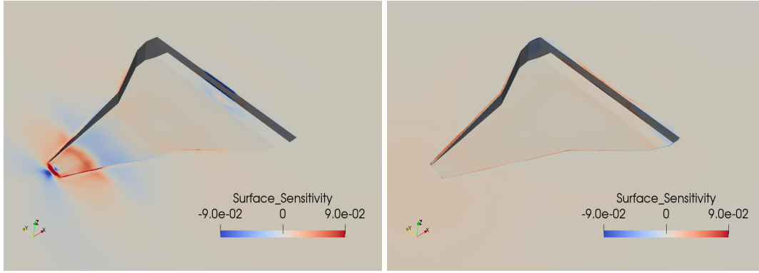
Figure 4.2: Lift calculated surface sensitivity; Left: Baseline; Right: Optimum design.
