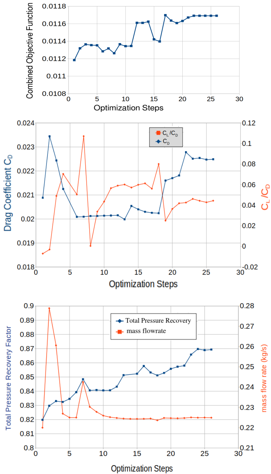
Figure 4.35: Optimization history
