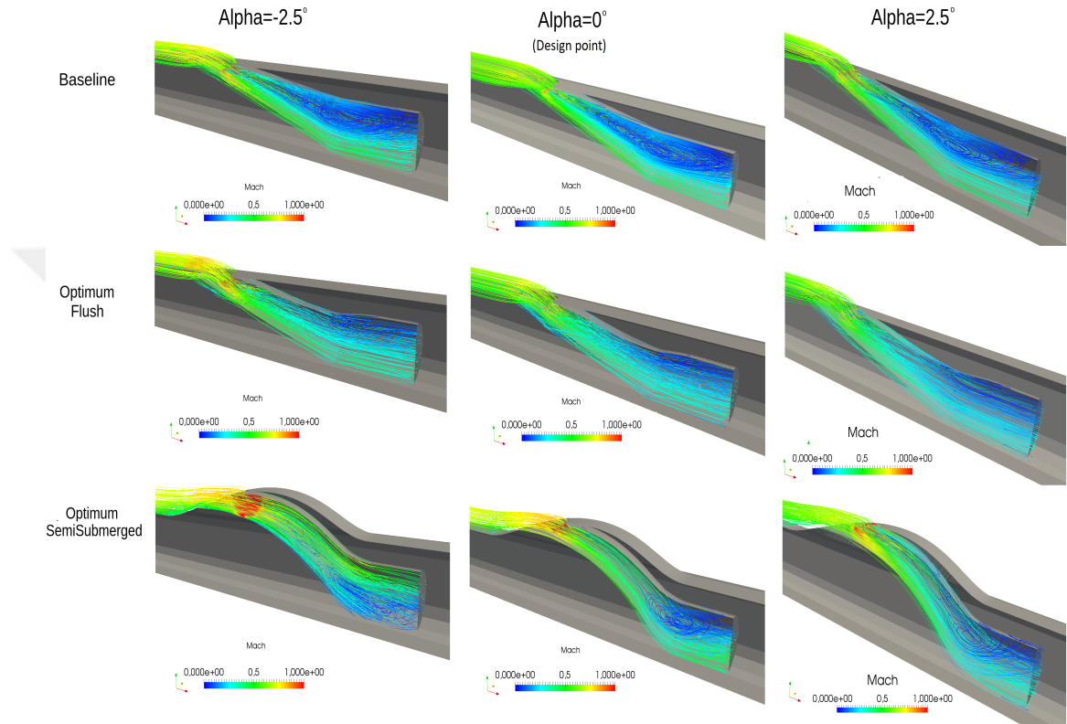
Figure 4.47: Comparison of flow at design and off-design alpha for fixed Mach 0.7.
