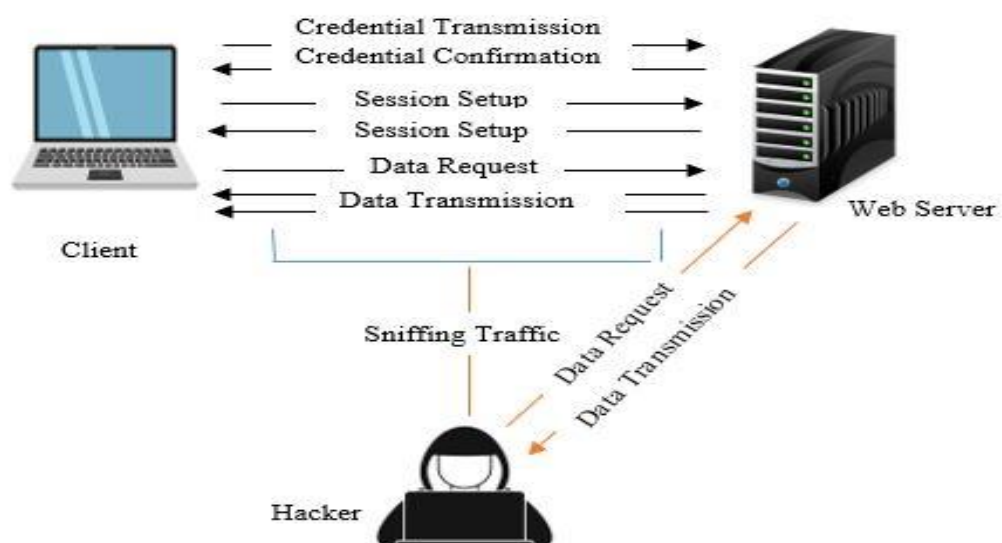
Figure 3.4. Session hijacking.
