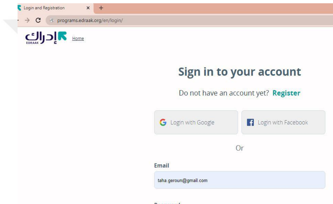
Figure 4.13. After attack redirecting to HTTP.
