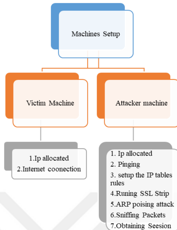
Figure 4.2. Machines setup steps.
