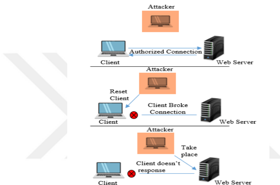
Figure 3.6. Active session hijacking.
