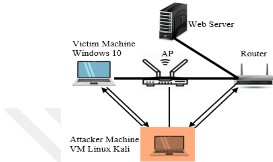
Figure 4.1. Session hijacking simulation system.
