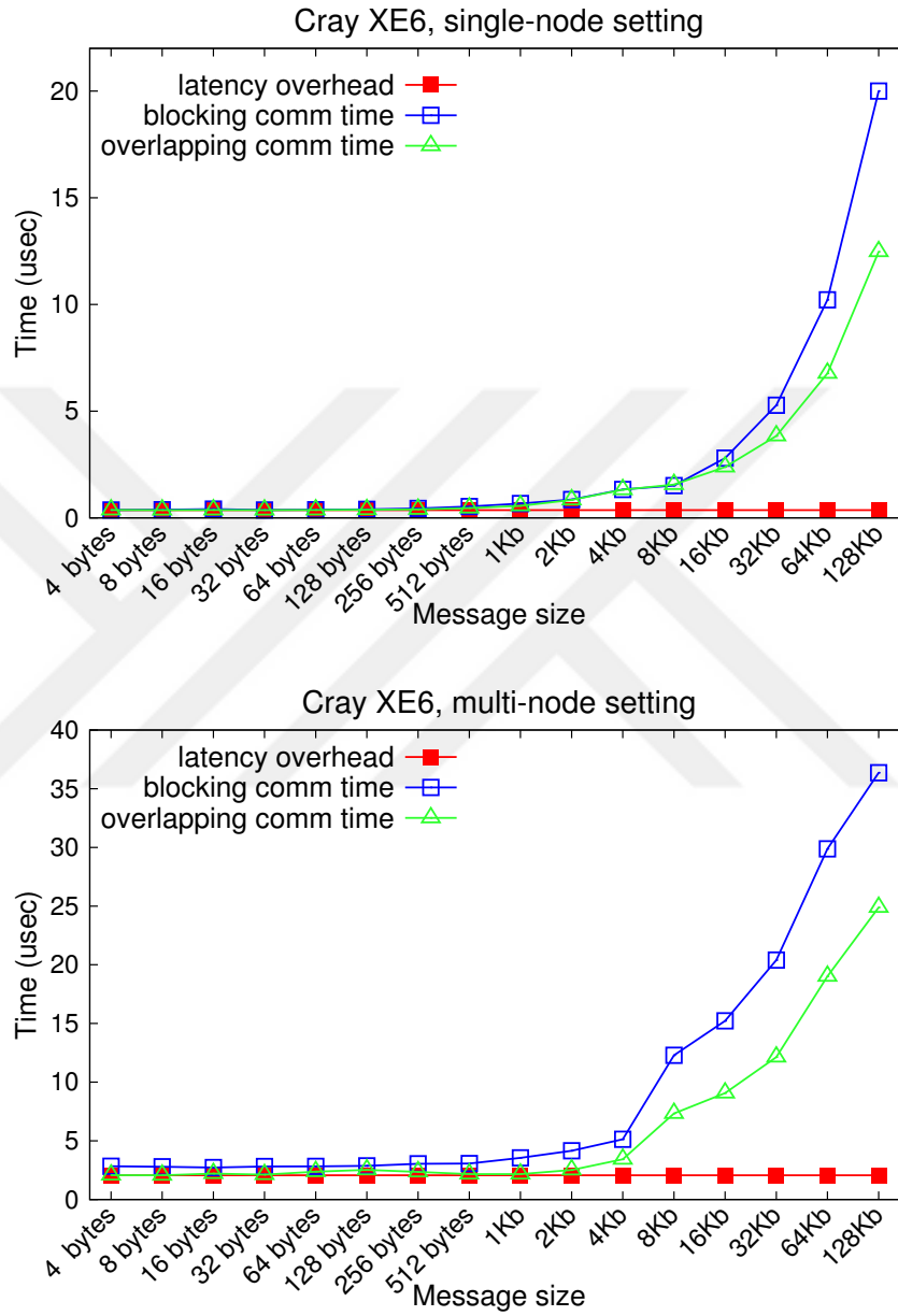
Figure 2.2: Blocking and overlapping communication times vs. latency overhead on Cray XE6.
