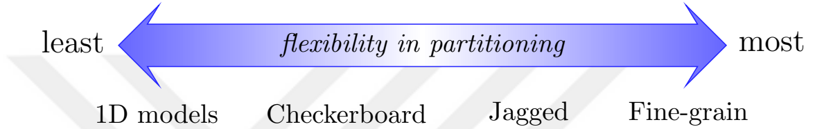
Figure 3.11: Comparison of models in terms of partitioning flexibility.
