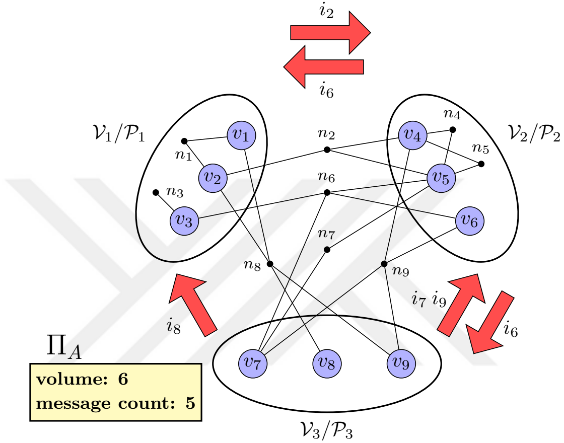
Figure 4.3: 3-way partitioning of hypergraph A_{PRE} . Note that v_j represents both task t_j and input i_j .
