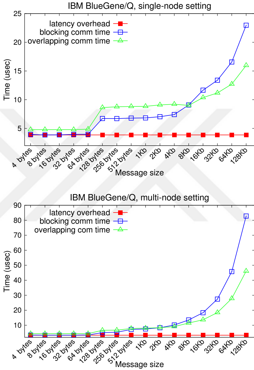
Figure 2.1: Blocking and overlapping communication times vs. latency overhead on IBM BlueGene/Q.
