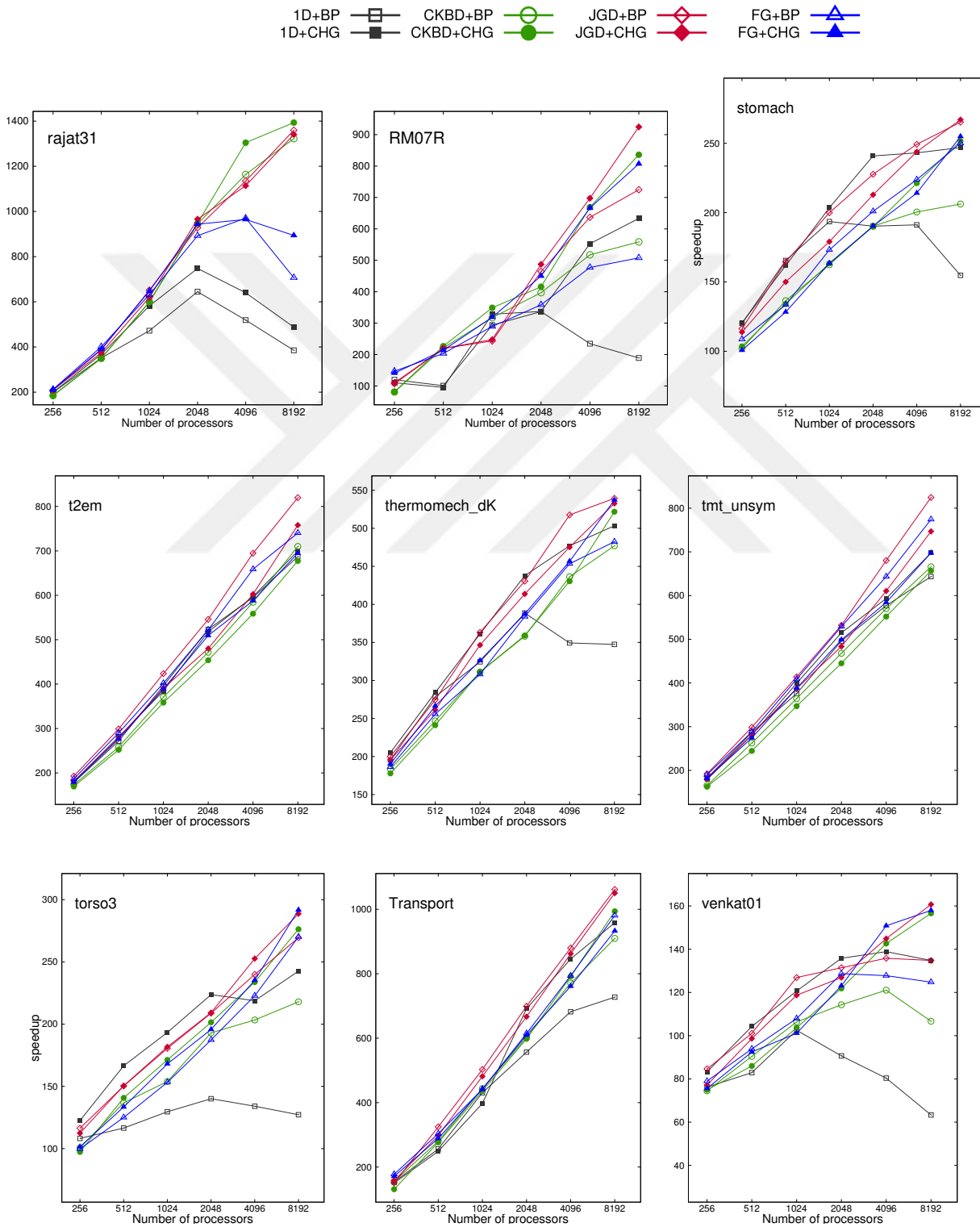
Figure 3.16: Speedup curves for 9 matrices (Part 3 of 3).
