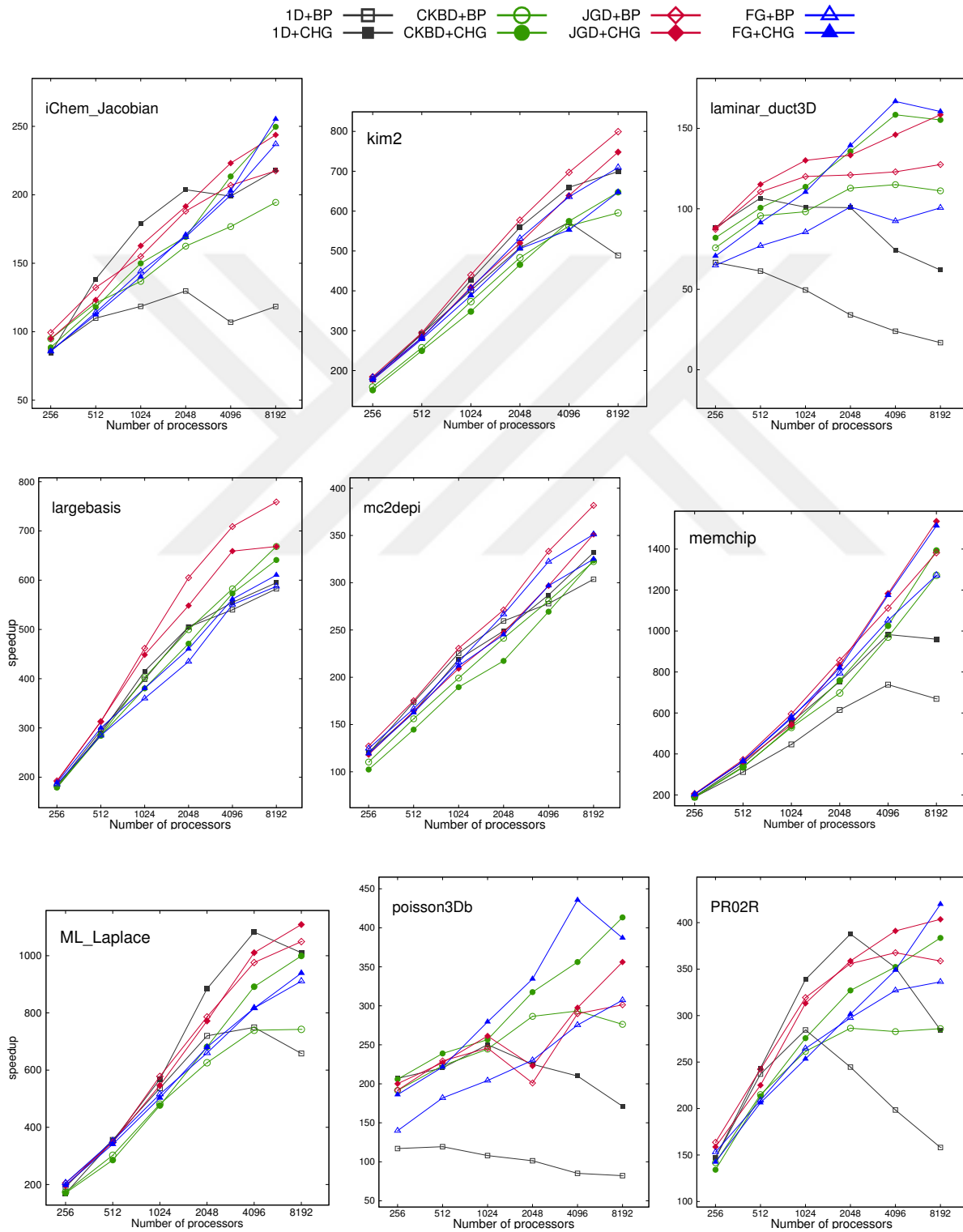
Figure 3.15: Speedup curves for 9 matrices (Part 2 of 3).
