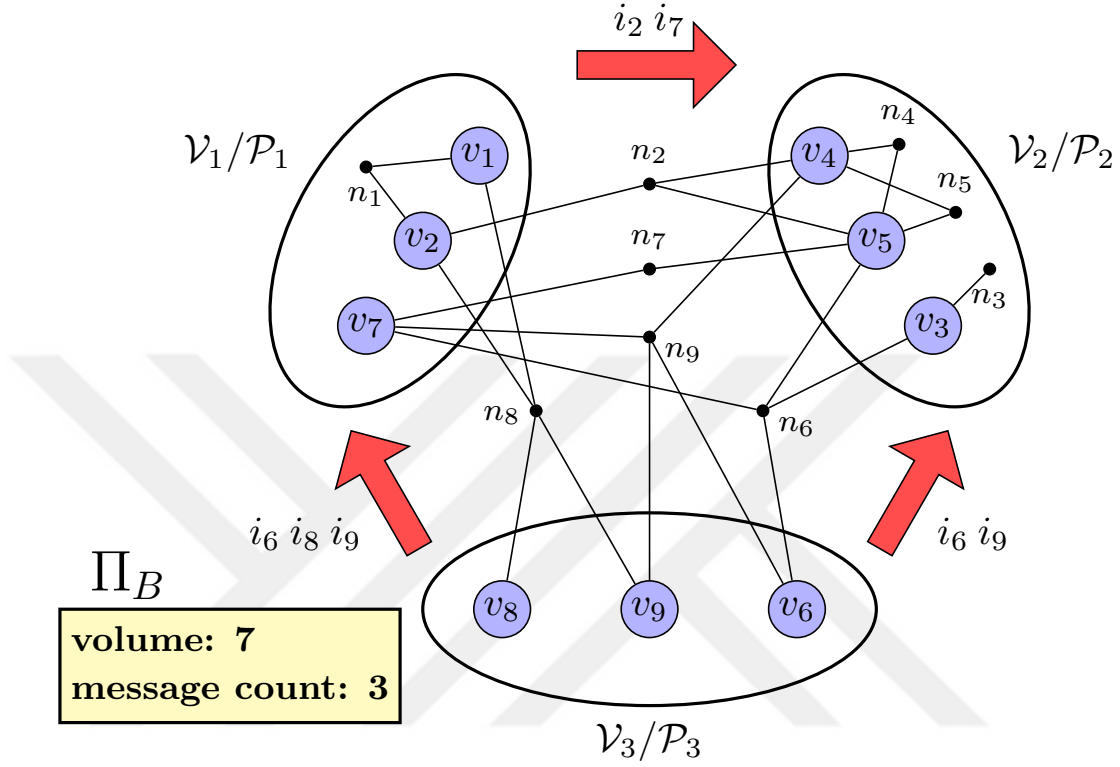
Figure 4.4: Another 3-way partitioning of hypergraph A_{PRE} . Only the parts of v_3 , v_6 and v_7 differ in \Pi_A (see Fig. 4.3) and \Pi_B . \Pi_A incurs less volume but more messages while \Pi_B incurs more volume but less messages.
