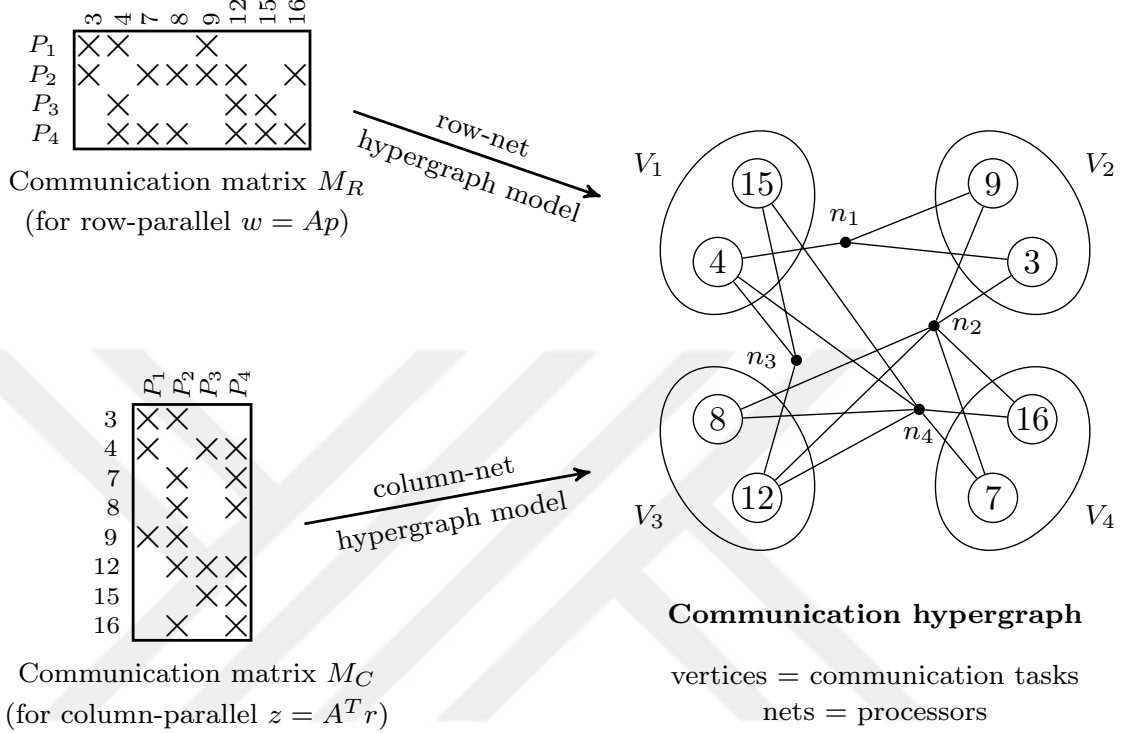
Figure 3.3: Formation of the communication hypergraph from communication matrix, and a four-way partition on this hypergraph. Matrices M_R and M_C summarize the communication requirements of w = Ap and z = A^T r operations illustrated in Figure 3.1.
