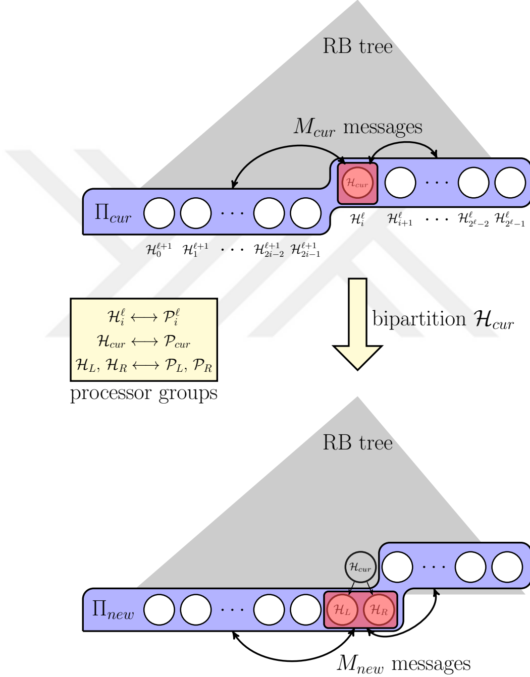
Figure 4.5: The state of the RB tree and the number of messages from/to \mathcal{P}_{cur} and \{\mathcal{P}_L, \mathcal{P}_R\} to/from the other processor groups before and after bipartitioning \mathcal{H}_{cur} . The processor groups corresponding to the vertex sets of the hypergraphs are shown in the box.
