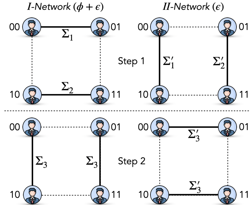
Figure 6.2. Bid aggregations of PMTBS protocol in 2-dimensional hypercube networks.
