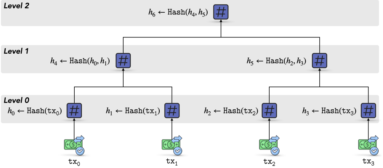
Figure 2.2. Merkle tree for blockchain transactions.
