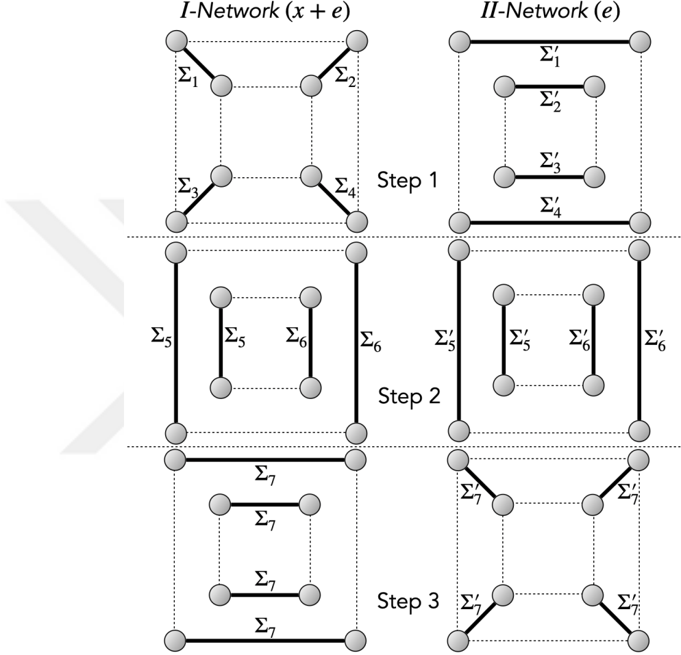
Figure 5.4. Aggregations of PVSS protocol in 3-dimensional hypercube network.
