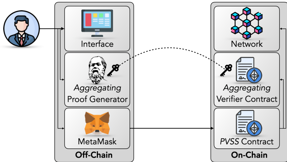
Figure 5.2. Architecture of PVSS protocol.
