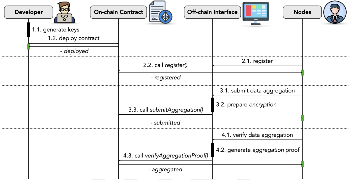
Figure 5.3. Sequence diagram of PVSS protocol.
