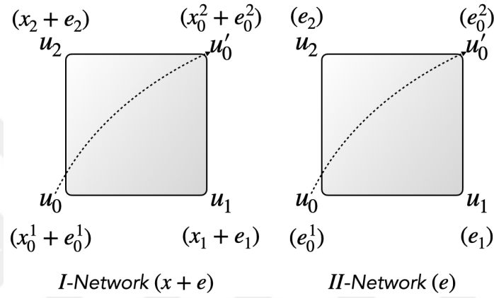
Figure 5.19. Data splitting technique on PVSS protocol.
