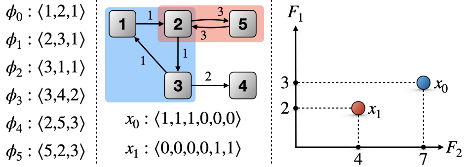
Figure 7.1. A simple illustration for multi-objective bartering with six bids
