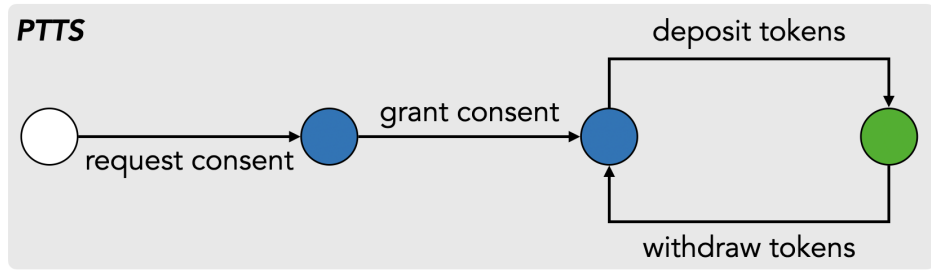
Figure 4.1. State-transition diagram of PTTS protocol.
