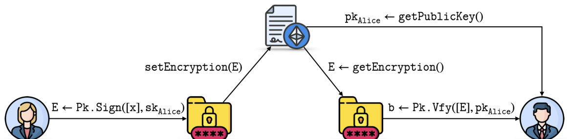
Figure 2.9. Public key cryptography on blockchain: authentication.
