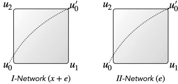
Figure 5.15. Node multiplexing technique on PVSS protocol.
