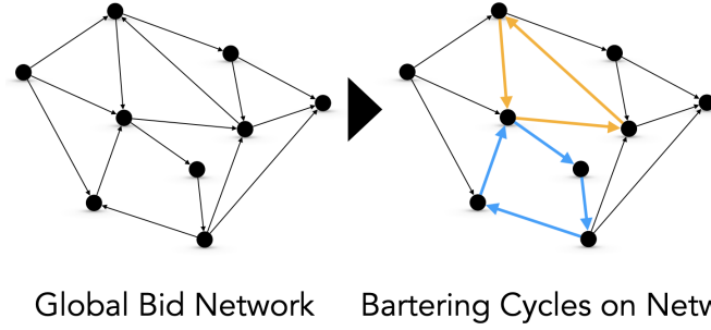
Figure 7.3. Negative cycle detection with Bellman-Ford
