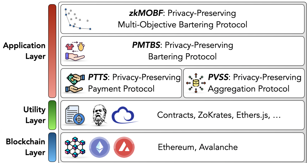
Figure 1.1. Layered architecture of our protocols.
