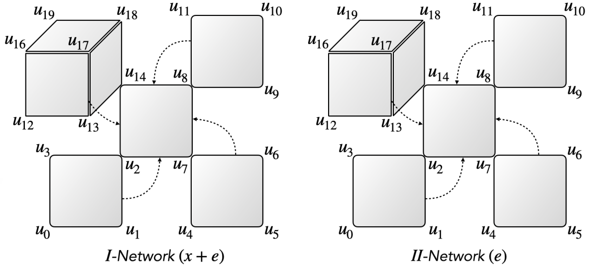
Figure 5.17. Topological recursing technique on PVSS protocol.
