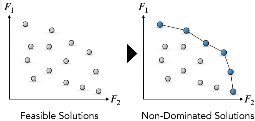
Figure 7.5. Non-dominated ranking of solutions for POS
