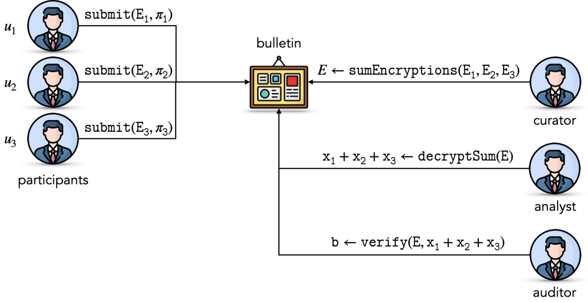
Figure 3.1. Architecture of Masquerade [75] with trusted parties.
