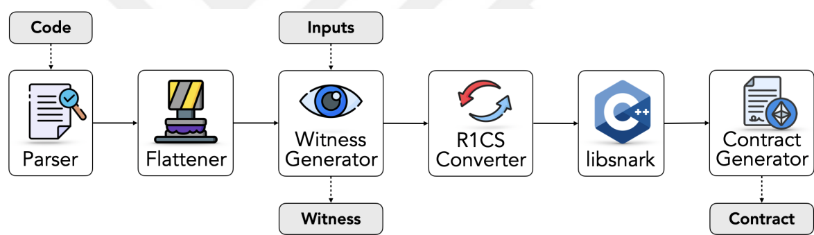
Figure 2.11. Architecture of ZoKrates framework [27].
