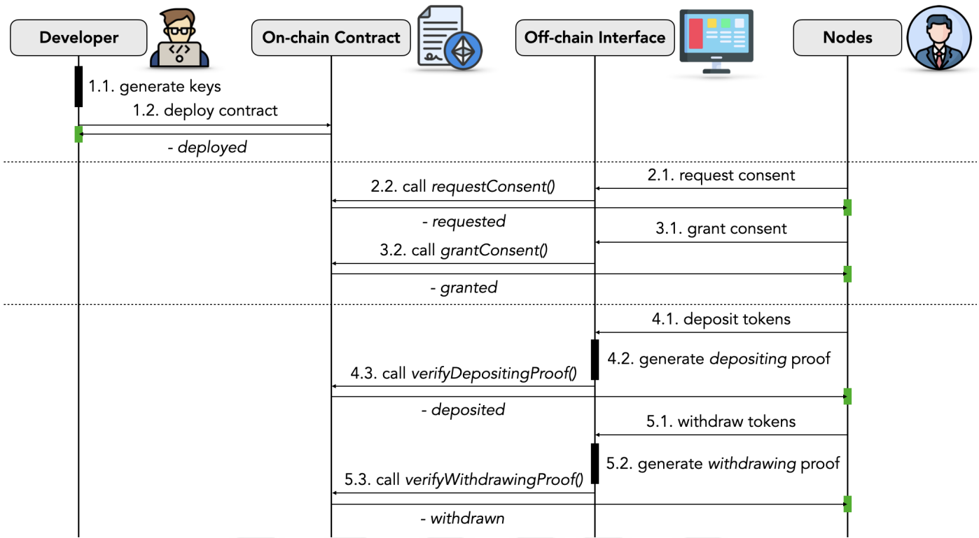
Figure 4.3. Sequence diagram of PTTS protocol.
