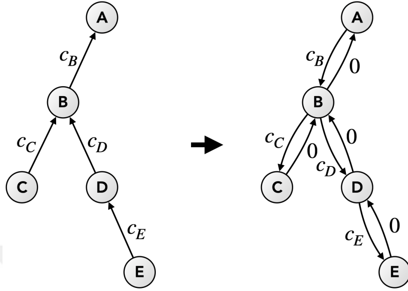
Figure 5.23. Transformation of global directed graph with Euler Tour Technique.
