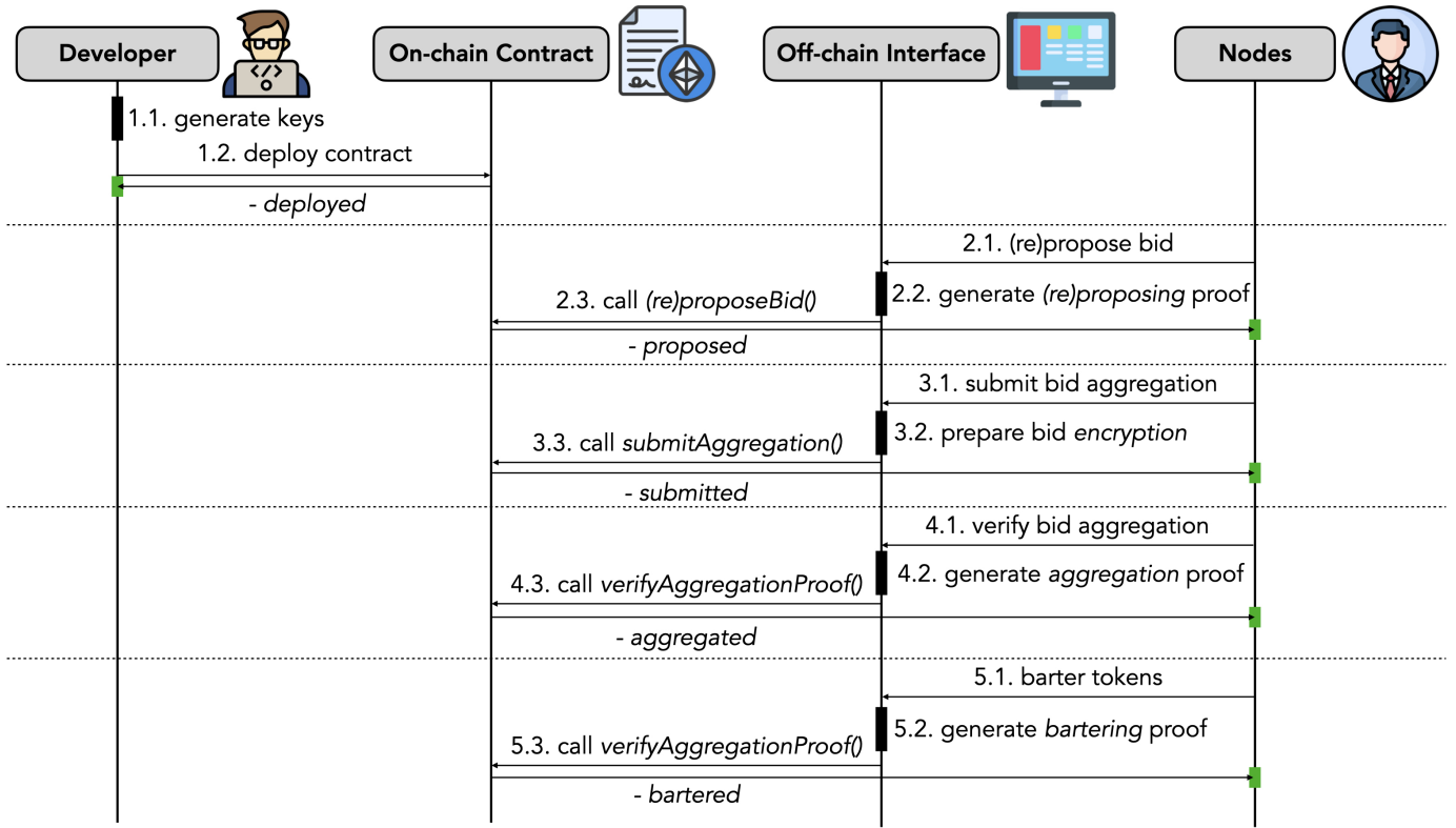
Figure 6.6. Sequence diagram of PMTBS protocol.
