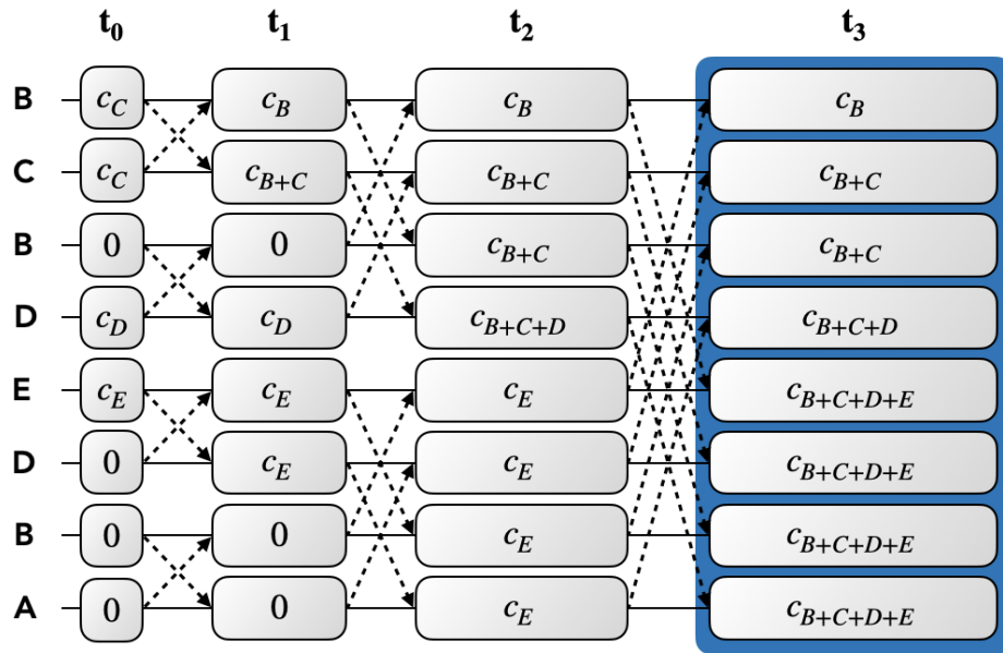
Figure 5.25. Privacy-preserving prefix summation with PRFX protocol.
