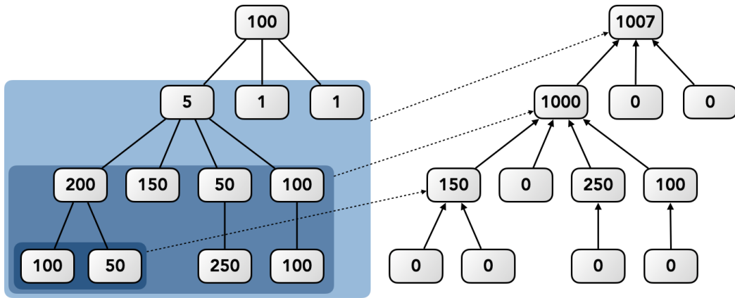
Figure 5.22. Delegation of tokens in PRFX protocol.
