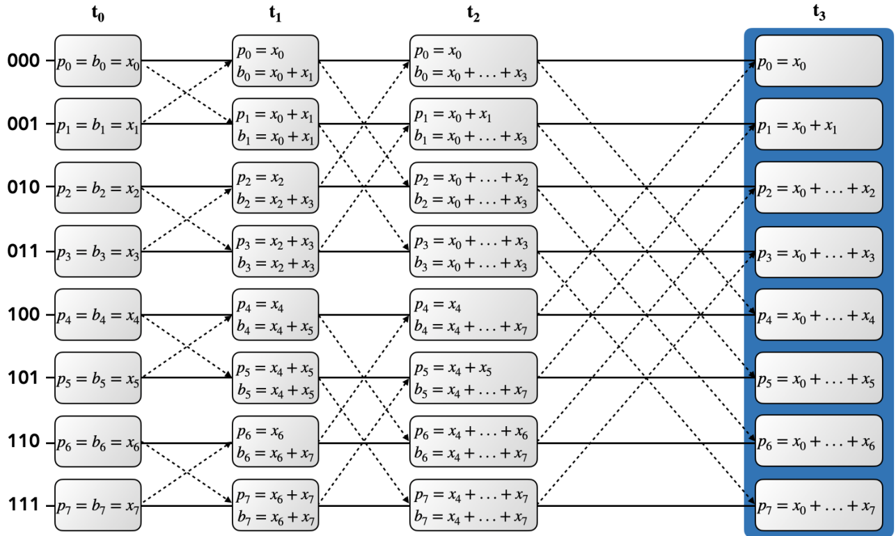
Figure 5.21. Communication of aggregators in PRFX protocol.
