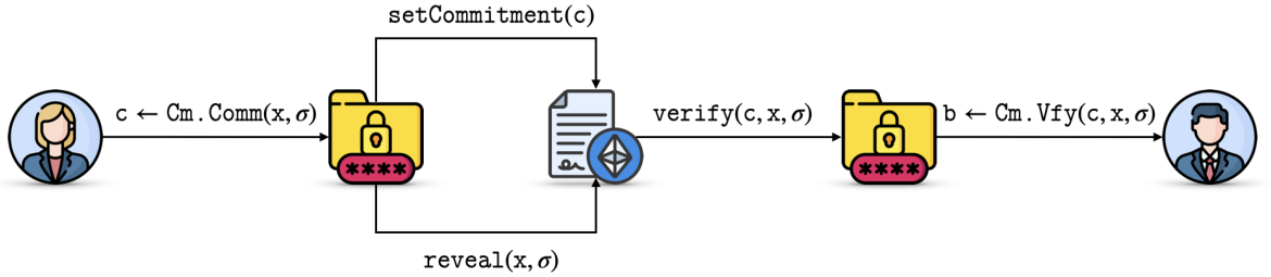
Figure 2.6. Commitment scheme on blockchain.
