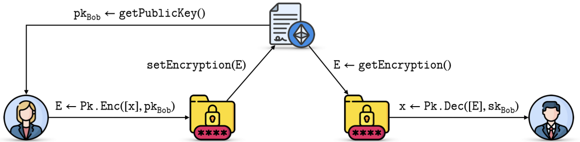
Figure 2.8. Public key cryptography on blockchain: confidentiality.
