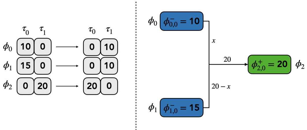
Figure 6.15. Ambiguity of bid satisfaction in PMTBS protocol.
