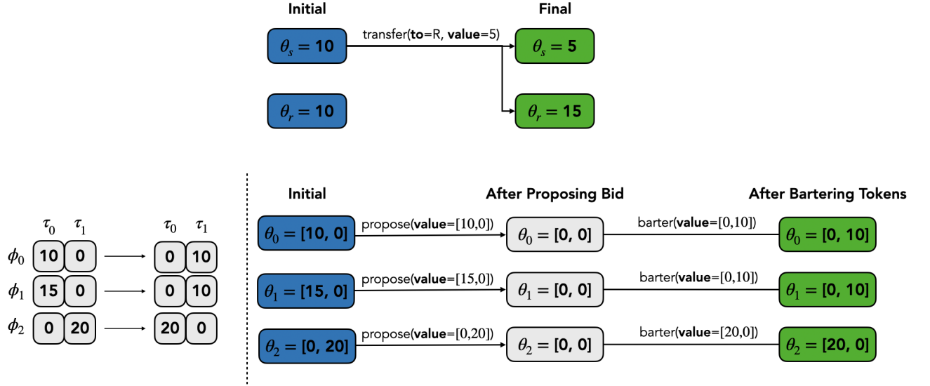
Figure 6.16. Comparison of ERC-20 token transfer with PMTBS token transfer.
