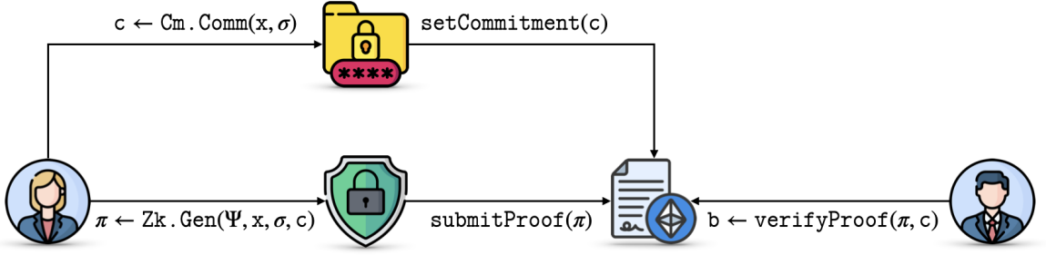
Figure 2.10. Zero-Knowledge proof on blockchain.
