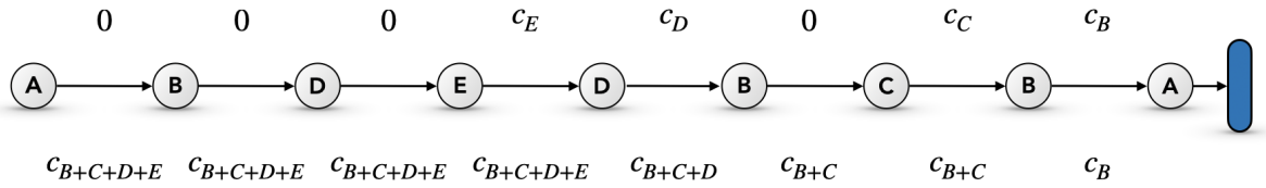
Figure 5.24. Linearization of global directed graph with Euler Tour Technique.
