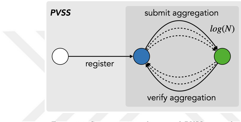
Figure 5.1. State-transition diagram of PVSS protocol.
