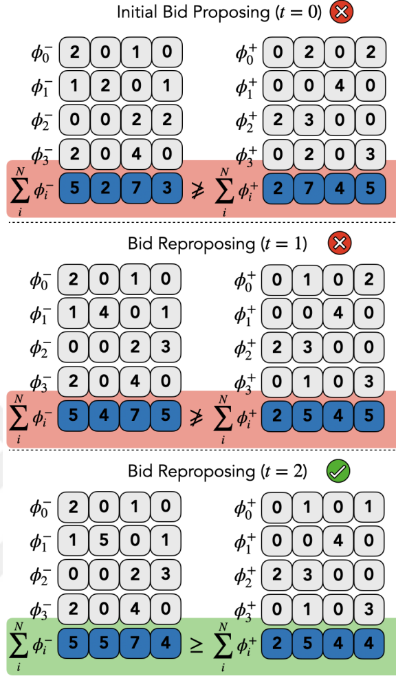
Figure 6.1. Illustration for ascending auction bartering (with four bids (\phi_0, \phi_1, \phi_2, \phi_3) and four tokens (\tau_0, \tau_1, \tau_2, \tau_3) ).
