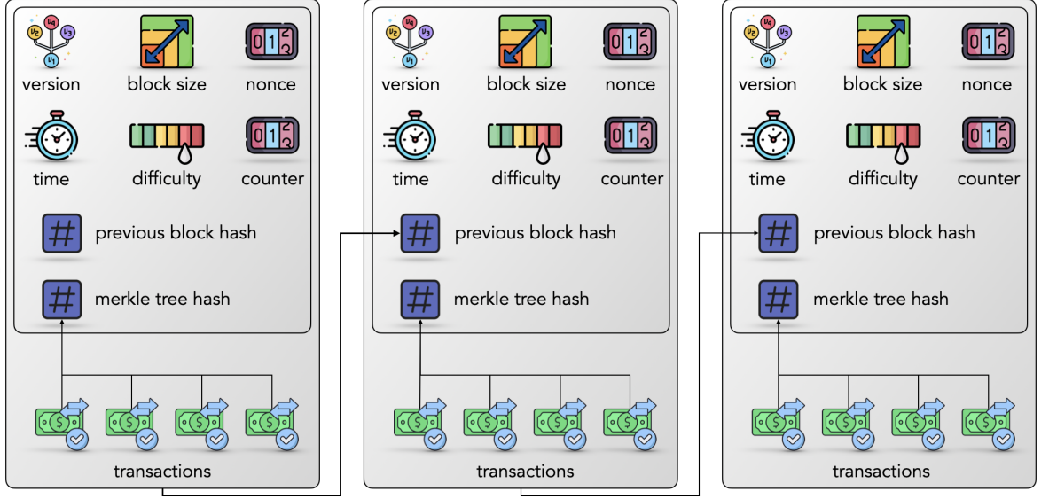
Figure 2.1. Blockchain as a chain of blocks.
