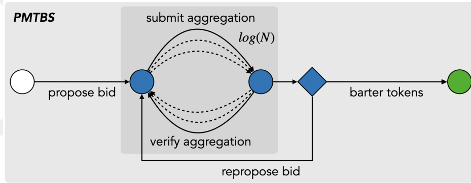
Figure 6.3. State-transition diagram of PMTBS protocol.
