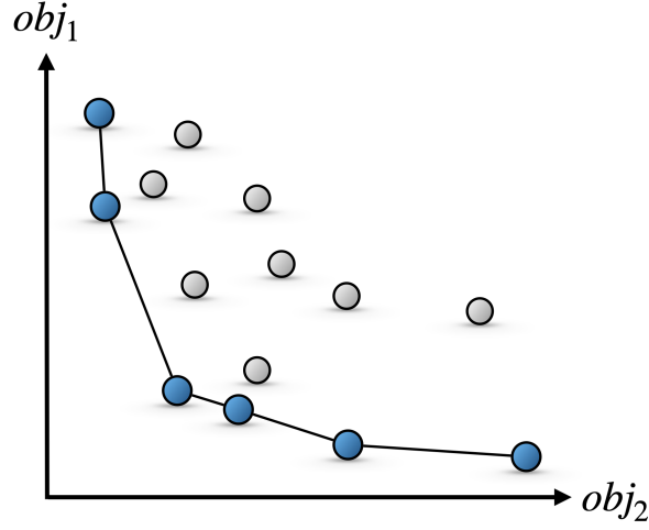
Figure 2.5. Multi-objective optimization with two objectives: (blue): optimal solutions (gray): non-optimal solutions.
