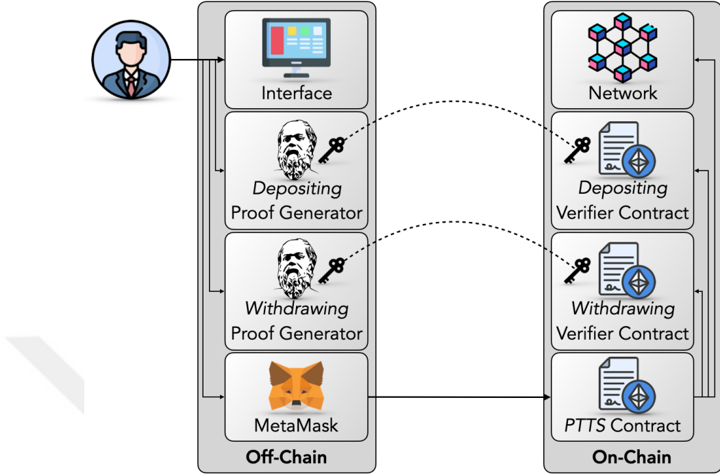
Figure 4.2. Architecture of PTTS protocol.
