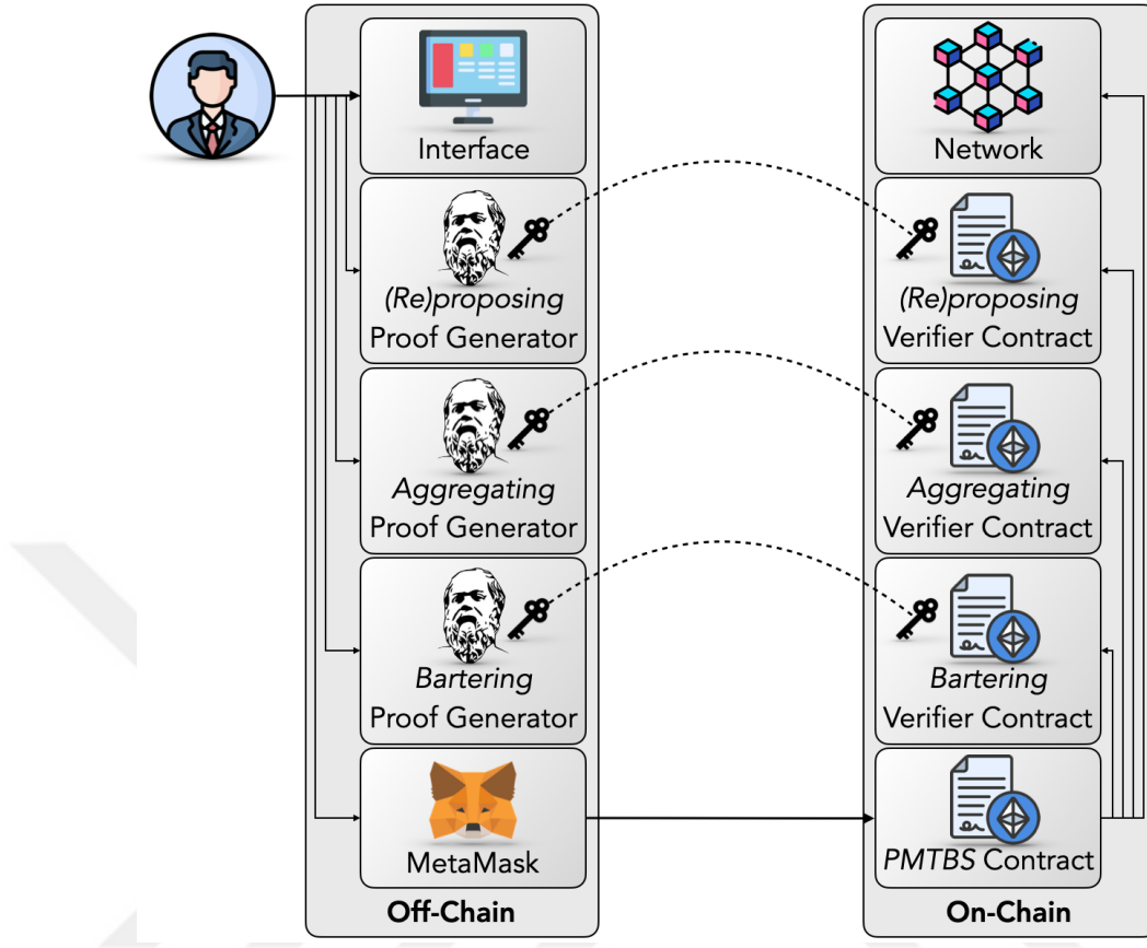
Figure 6.4. Architecture of PMTBS protocol.
