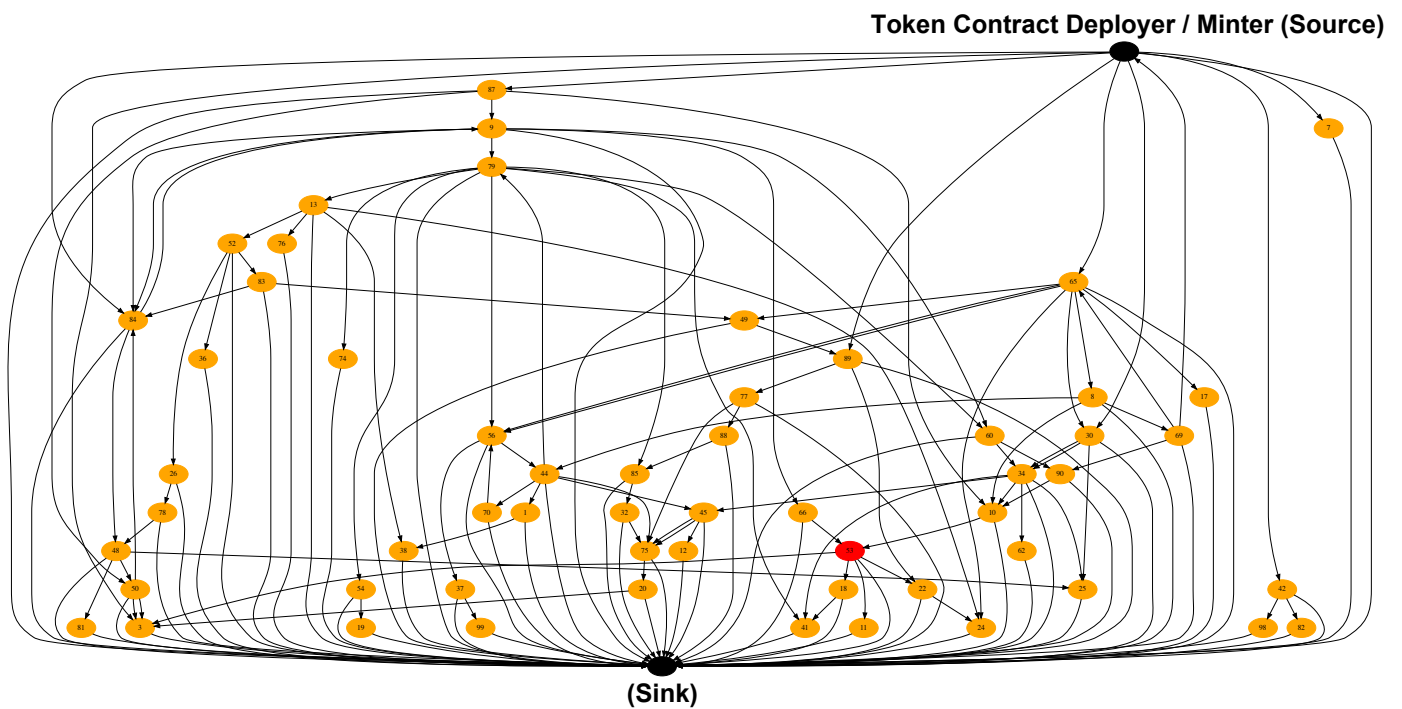
Figure 4.17. The minimum cost flow network: (black) source and sink addresses, (orange) ordinary addresses, (red) address to be attacked.
