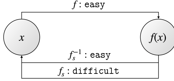
Figure 2.7. One-way functions with trapdoors.
