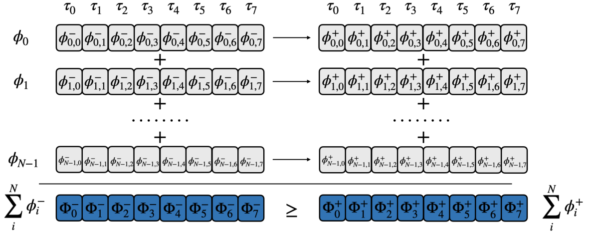
Figure 6.5. Bid aggregation with vector summation in PMTBS protocol.
