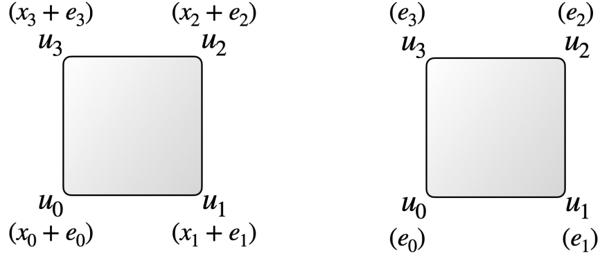
Figure 5.13. Undeterminacy on PVSS protocol.
