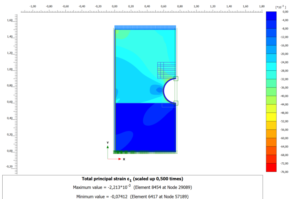
Figure D.10. Principal strain ( \epsilon_1 ) at 200 kPa
