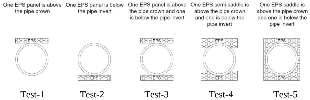
Figure 4.1. Pipe – EPS geofoam combinations from laboratory test [taken from Kılıç & Akinay (2019)]
