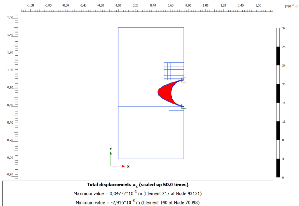
Figure D.5. Horizontal displacements of pipe ( u_x ) at 200 kPa
