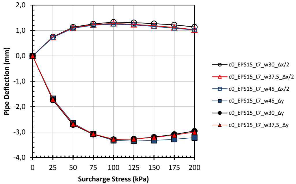
Figure 5.43. Effect of EPS width while density=15 kg/m 3 & thickness=7 cm
