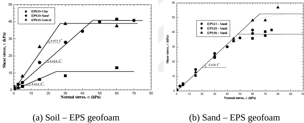
Figure 3.9. Applied normal stress (kPa) vs. shear stress (kPa)
