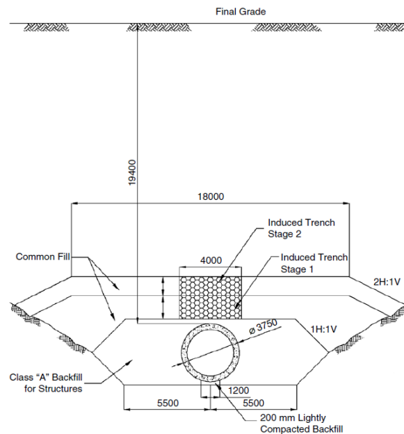
Figure 2.12. Installation of the imperfect trench application (Parker et al., 2008)
