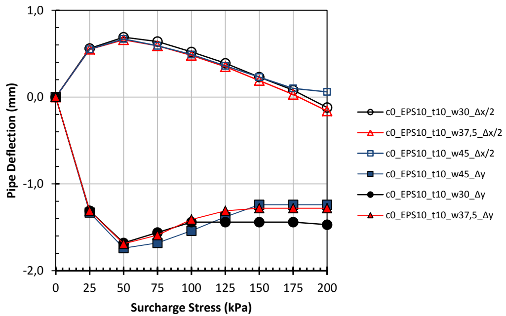
Figure 5.40. Effect of EPS width while density=10 kg/m³ & thickness=10 cm
