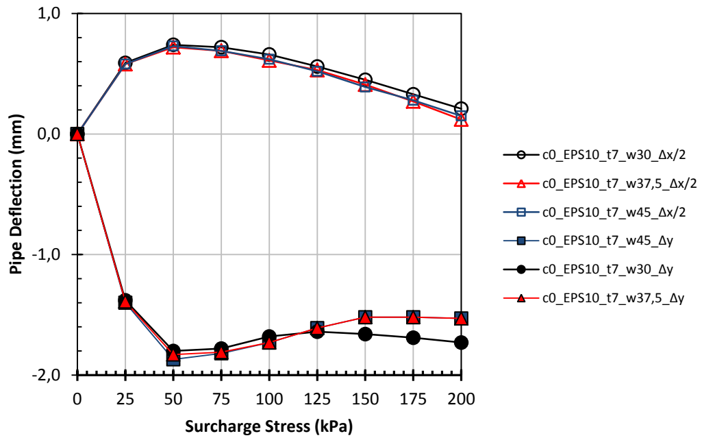
Figure 5.39. Effect of EPS width while density=10 kg/m³ & thickness=7 cm
