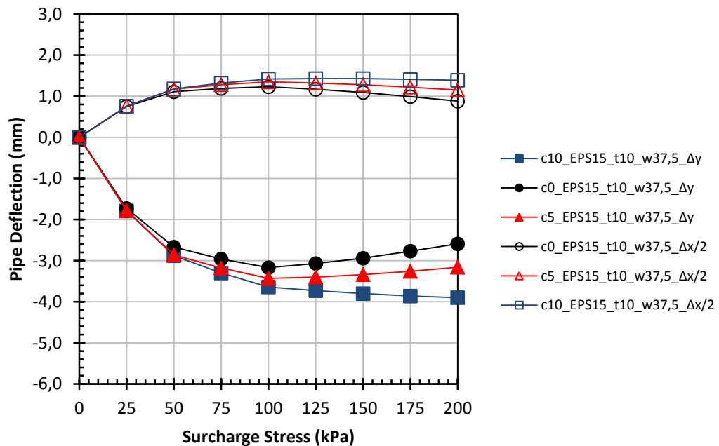
Figure 5.13. Effect of EPS-15 location while thickness=10 cm and width=37.5 cm
