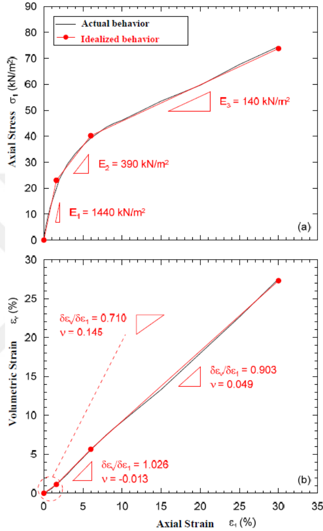
Figure 3.3. Stress-strain behavior of EPS-10 a) Axial strain – axial stress b) Axial strain – volumetric – strain [taken from Akınay (2017)]
