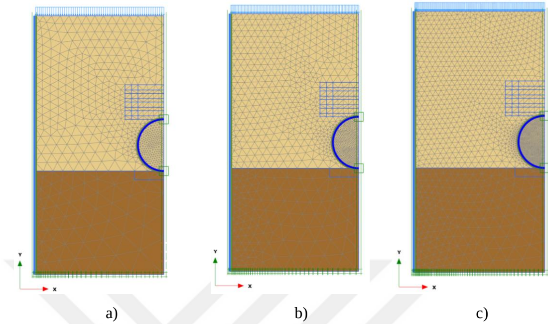
Figure 3.16. Finite element meshes for a) very coarse mesh density b) coarse mesh density c) medium mesh density
