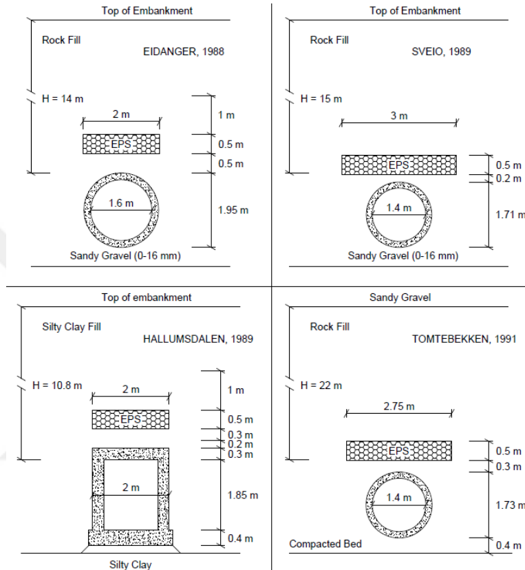
Figure 2.21. Placement of field installations of Vaslestad et al. (2011) [taken from Akinay (2017)]
