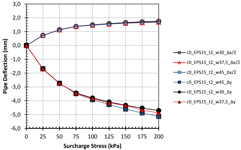
Figure 5.41. Effect of EPS width while density=15 kg/m 3 & thickness=2 cm
