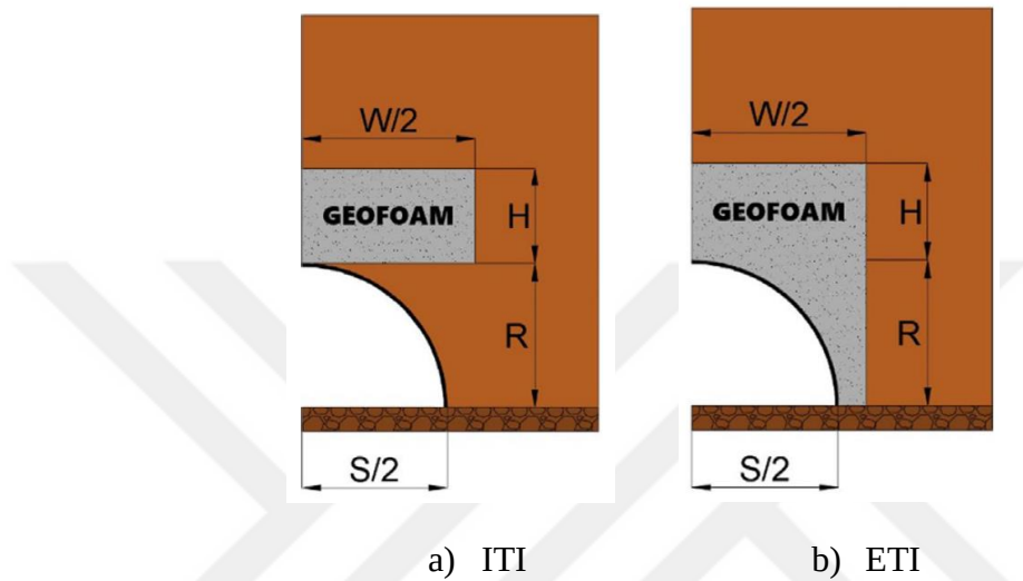
Figure 2.28. Configuration of EPS geofoam placement for ITI and ETI methods [taken from Santos et al. (2020)]
