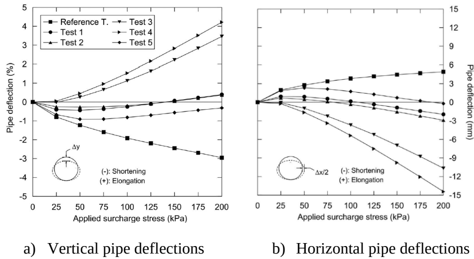
Figure 2.33. Comparison of vertical and horizontal deflections [taken from Kılıç and Akınay (2019)]
