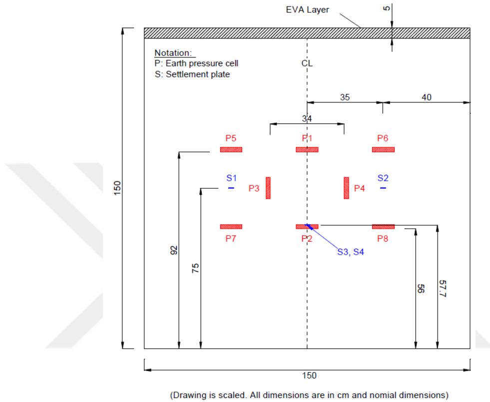
Figure 3.7. The layout of earth pressure sensors and settlement plates in laboratory test with no pipe and EPS geofoam [taken from Akinay (2017)]
