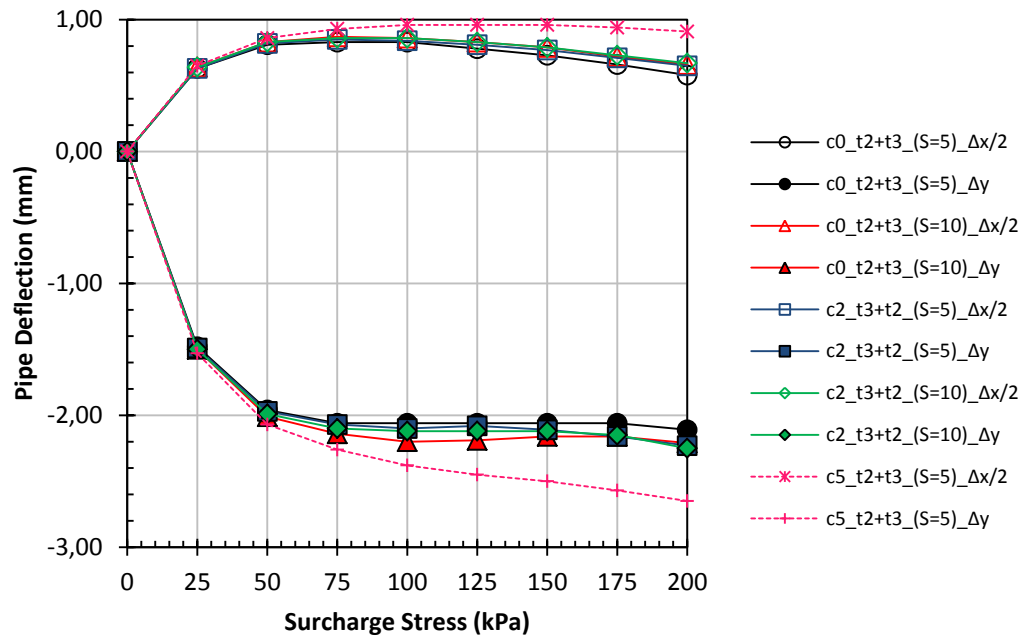
Figure 5.53. Two layers comparison of EPS geofoam for 5 cm thick in total for all combinations
