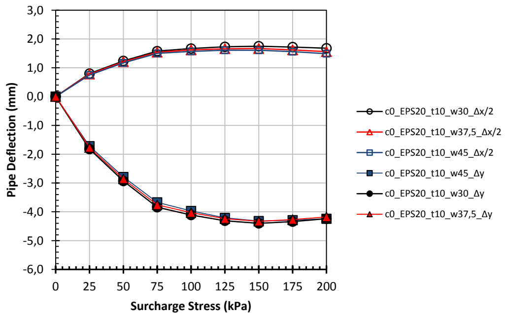
Figure 5.48. Effect of EPS width while density=20 kg/m 3 & thickness=10 cm
