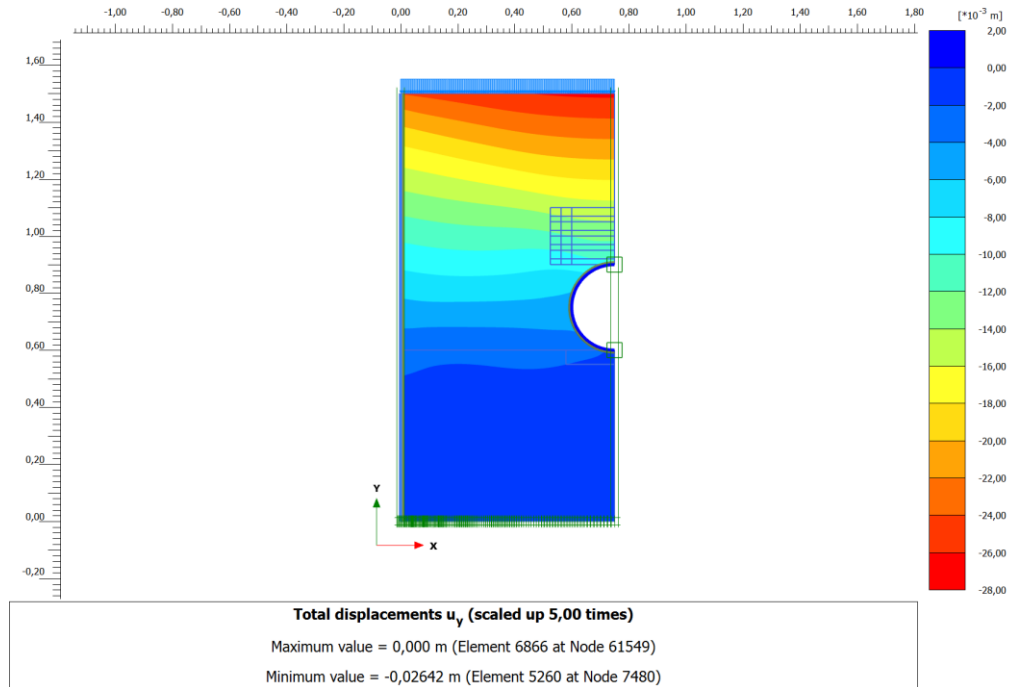
Figure D.4. Vertical displacements ( u_y ) at 200 kPa
