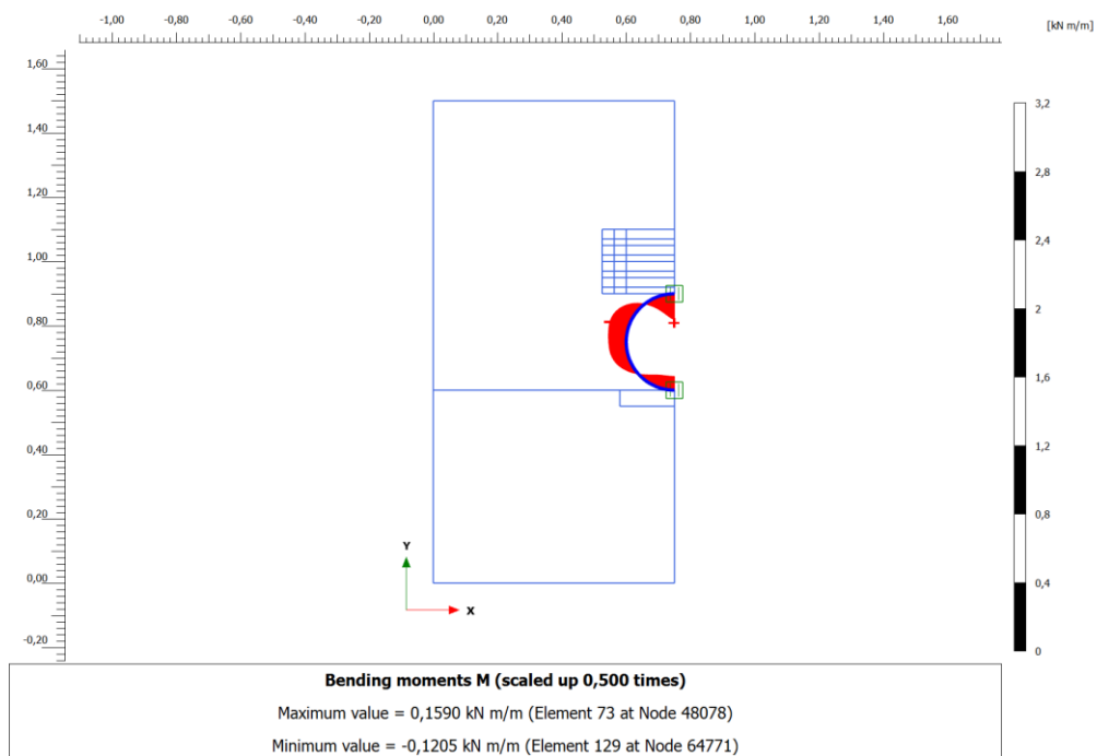
Figure D.9. Bending moments at pipe wall (M) at 200 kPa
