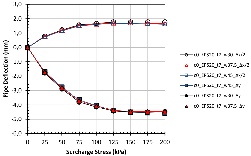
Figure 5.47. Effect of EPS width while density=20 kg/m 3 & thickness=7 cm
