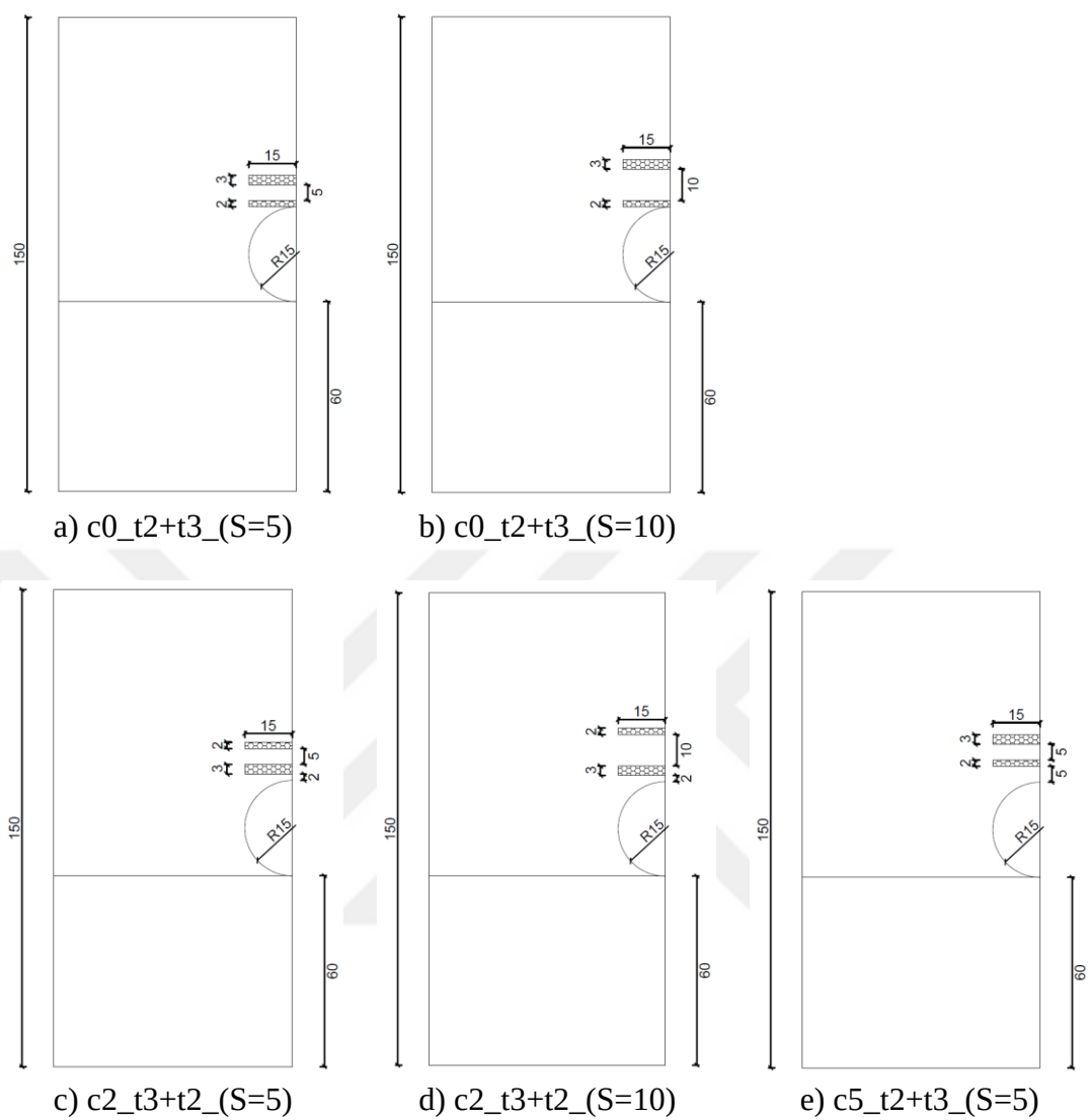
Figure 5.49. Two layers EPS combinations for total thickness of 5 cm
