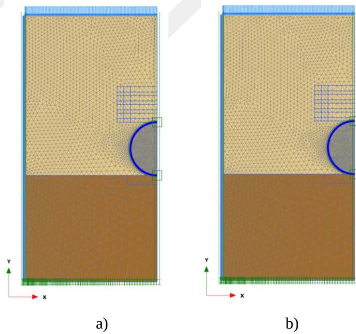
Figure 3.17. Finite element meshes for a) fine mesh density b) very fine mesh density
