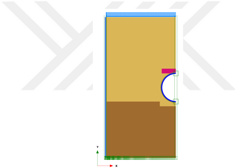
Figure 4.6. General overview of numerical model for configuration-1
