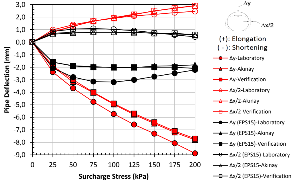
Figure 4.10. Comparison of deflections with EPS-15 (bilinear elastic parameters) in Test-1 Configuration
