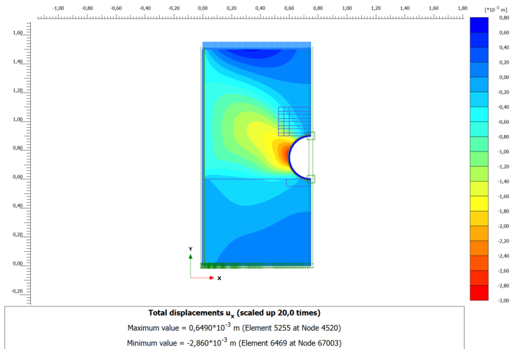
Figure D.3. Horizontal displacements ( u_x ) at 200 kPa
