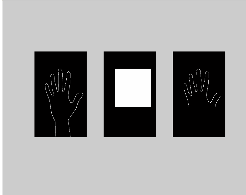
Figure 4.15: AND operation
