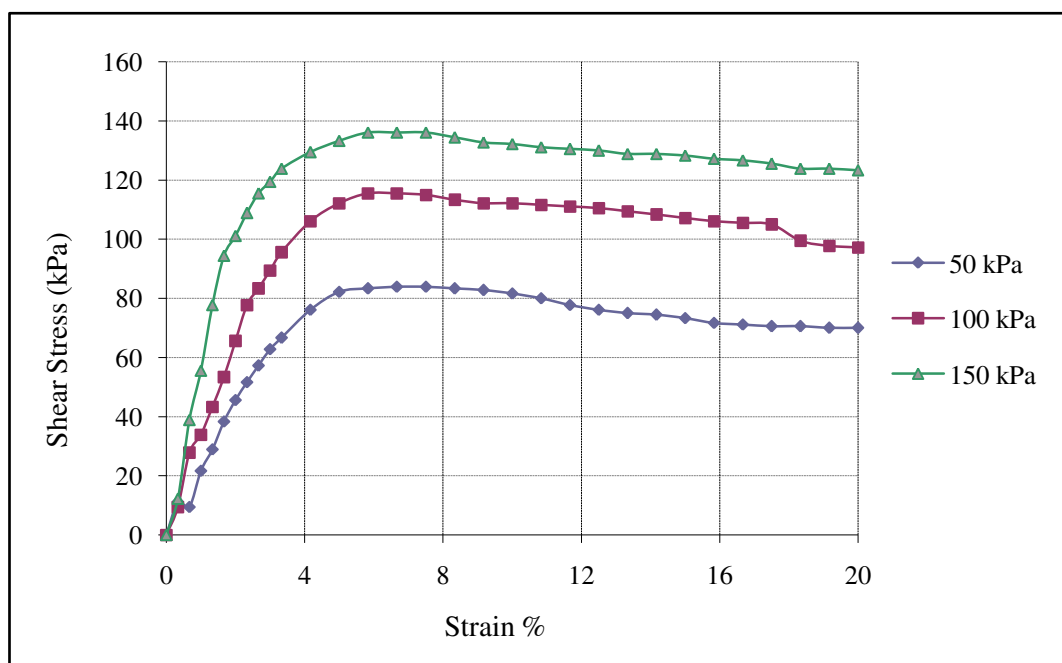
Figure 5.1. Plot of shear stress vs. strain for pure clay soil
