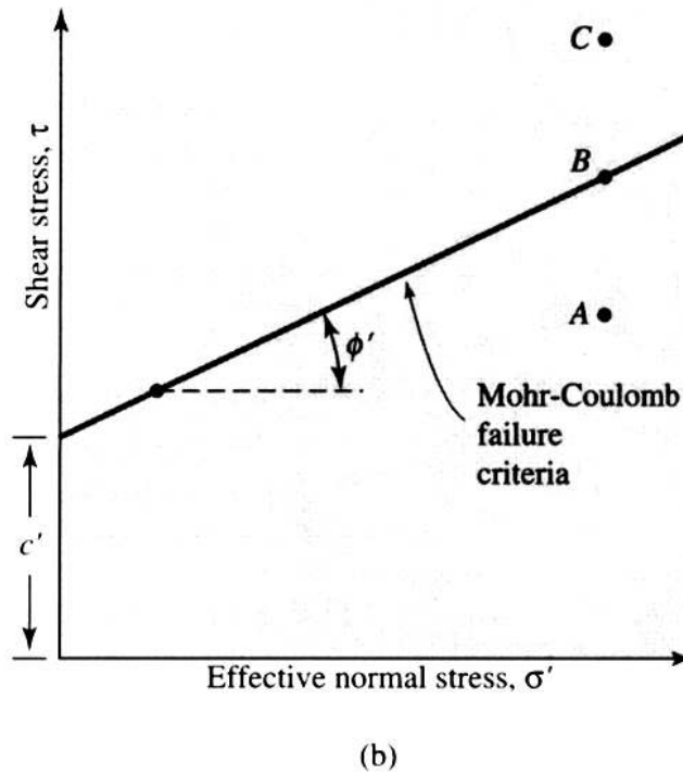
Figure 3.1. Mohr-Coulomb failure criterion (Das, 2008)
