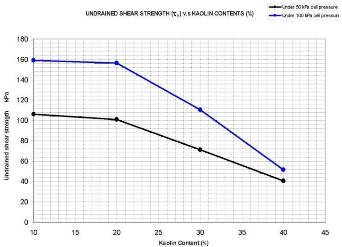
Figure 2.7. Relations between undrained shear strength and kaolin contents, in series 2 (Ölmez, 2008)
