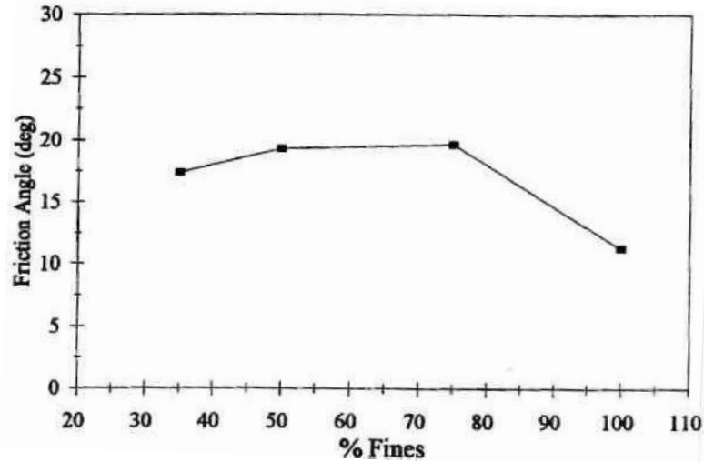
Figure 2.5. Undrained friction angle plotted against % fines (Bayoğlu, 1995)
