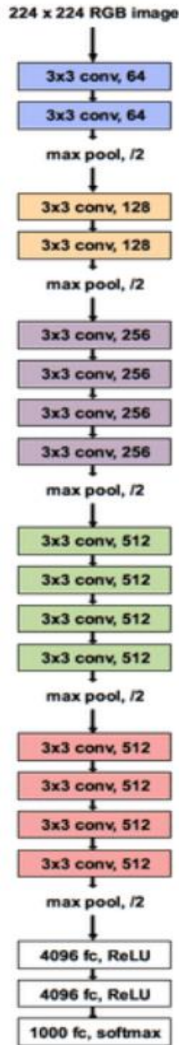
Figure 7 VGG19 Architecture [77]
