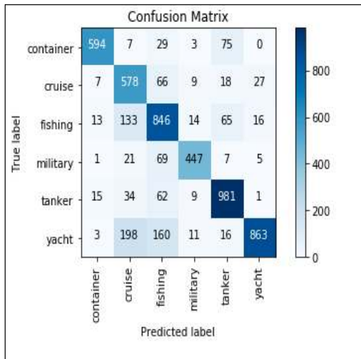
DensetNet121
