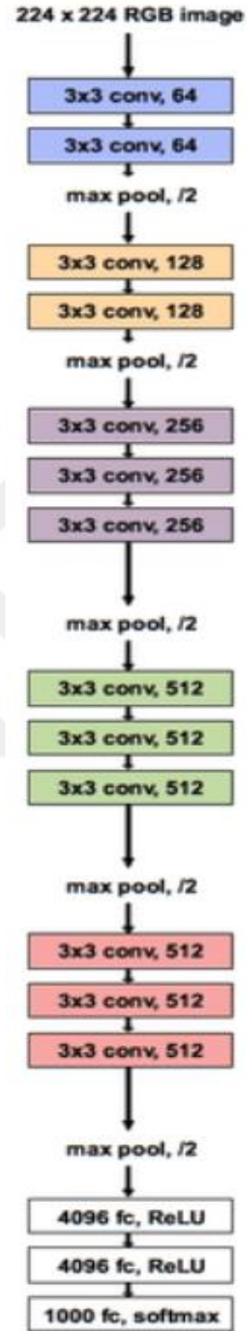
Figure 8 VGG16 Architecture [77]
