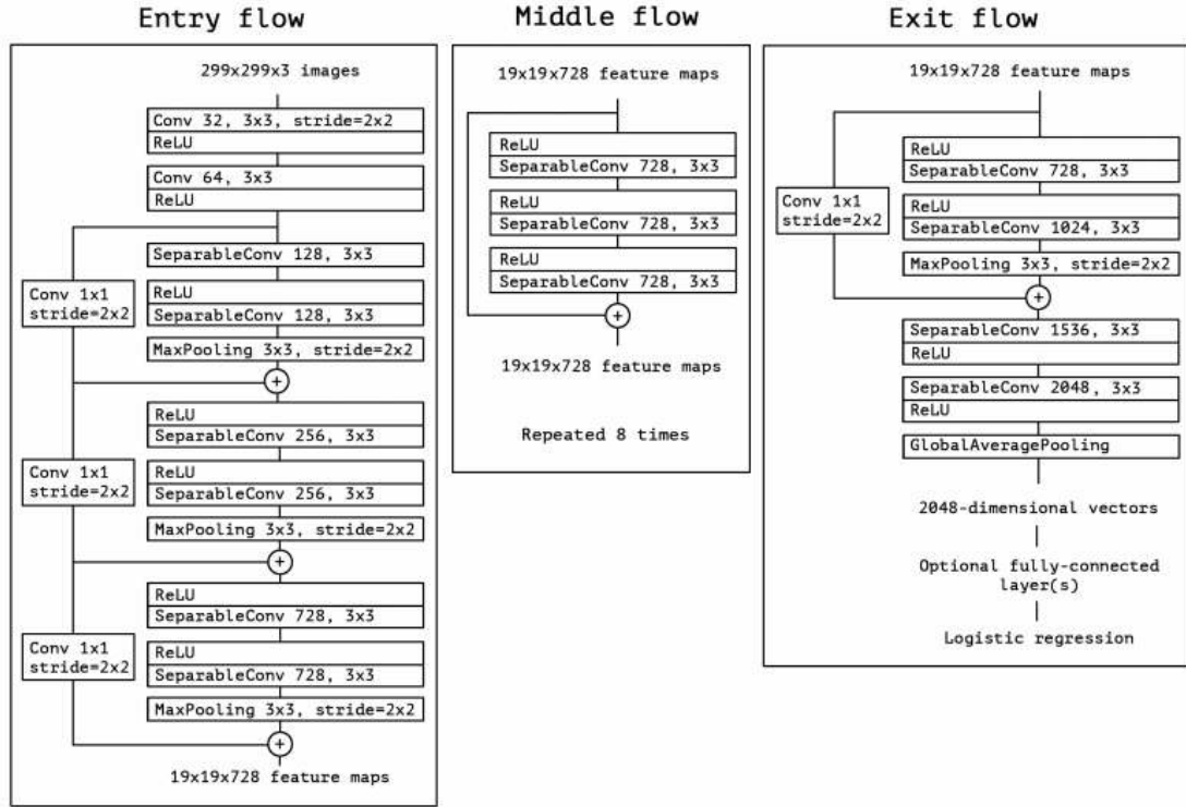
Figure 11 Xception Workflow [80]
