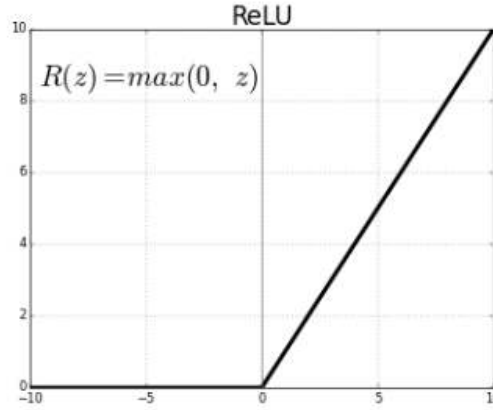
Figure 16 ReLu Graph
