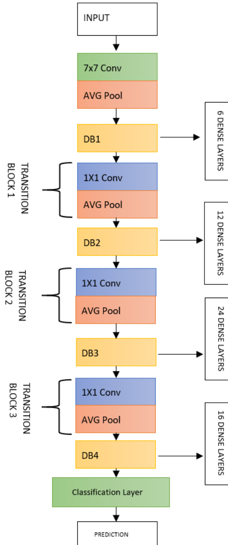
Figure 10 DenseNet Architecture
