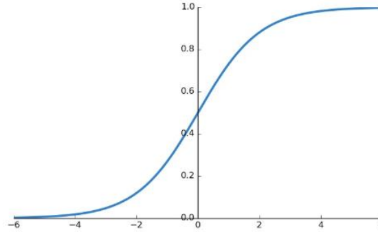
Figure 17 Sigmoid Function
