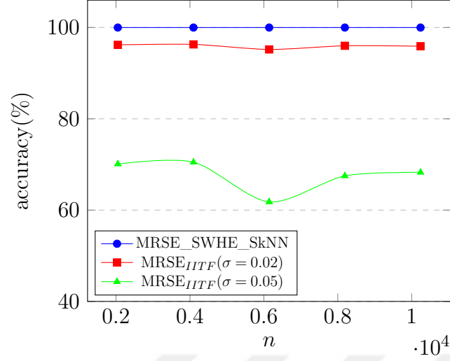
Figure 6.1 Accuracy of \text{MRSE}_{ITF} and \text{MRSE\_SWHE\_SkNN} with varying values of n and w
