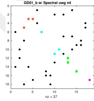
(f) Unweighted, nproc = 4, spy rep.
