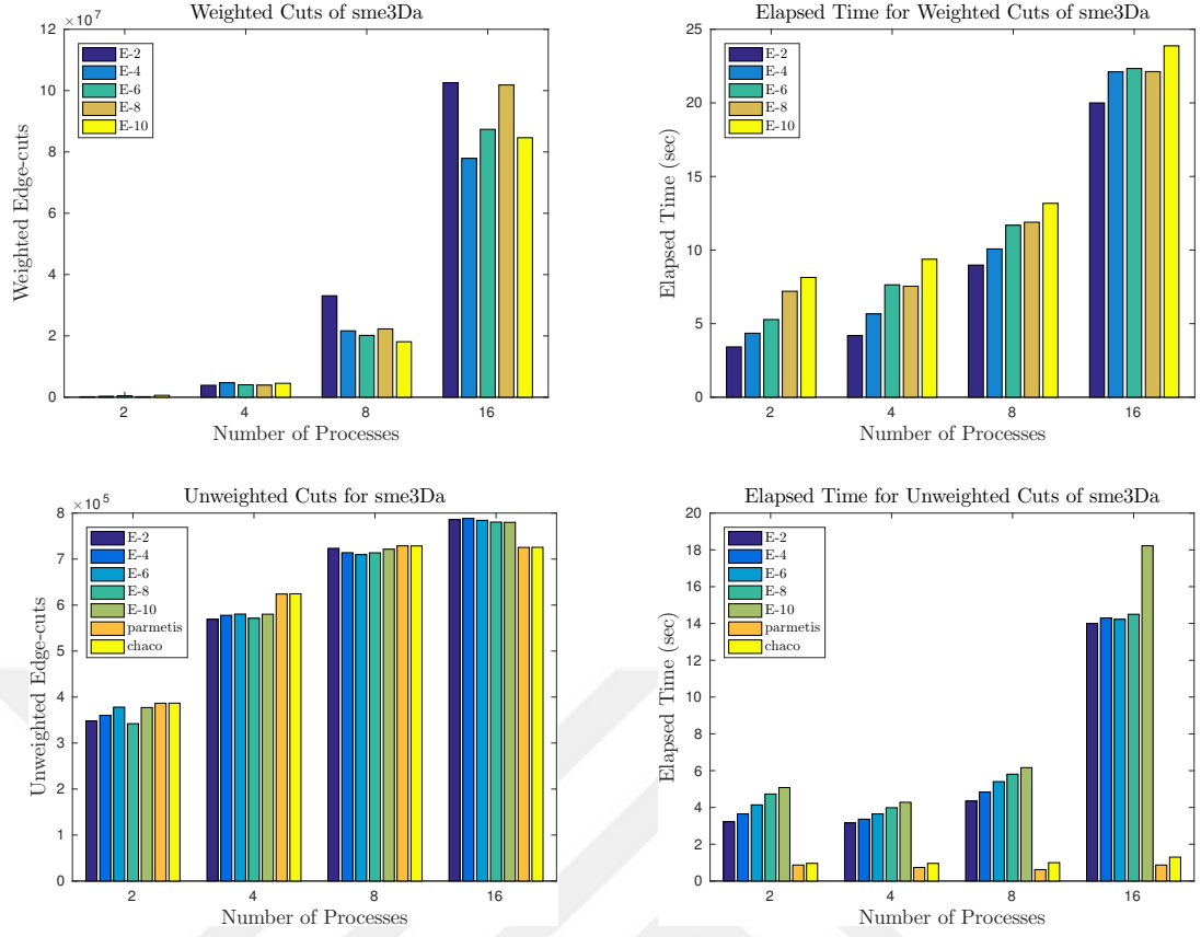
Figure 4.17: Results obtained from the partitioning of sme3Da
