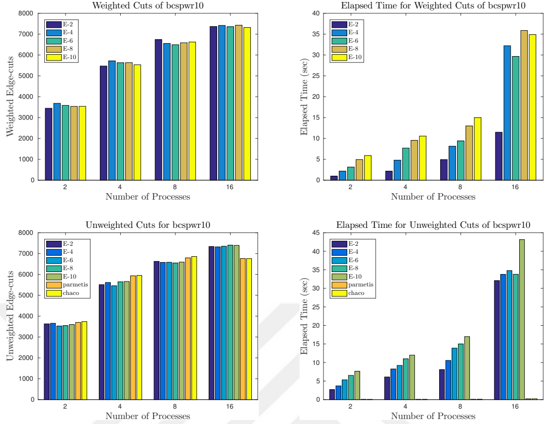
Figure 4.9: Results obtained from the partitioning of bcspwr10
