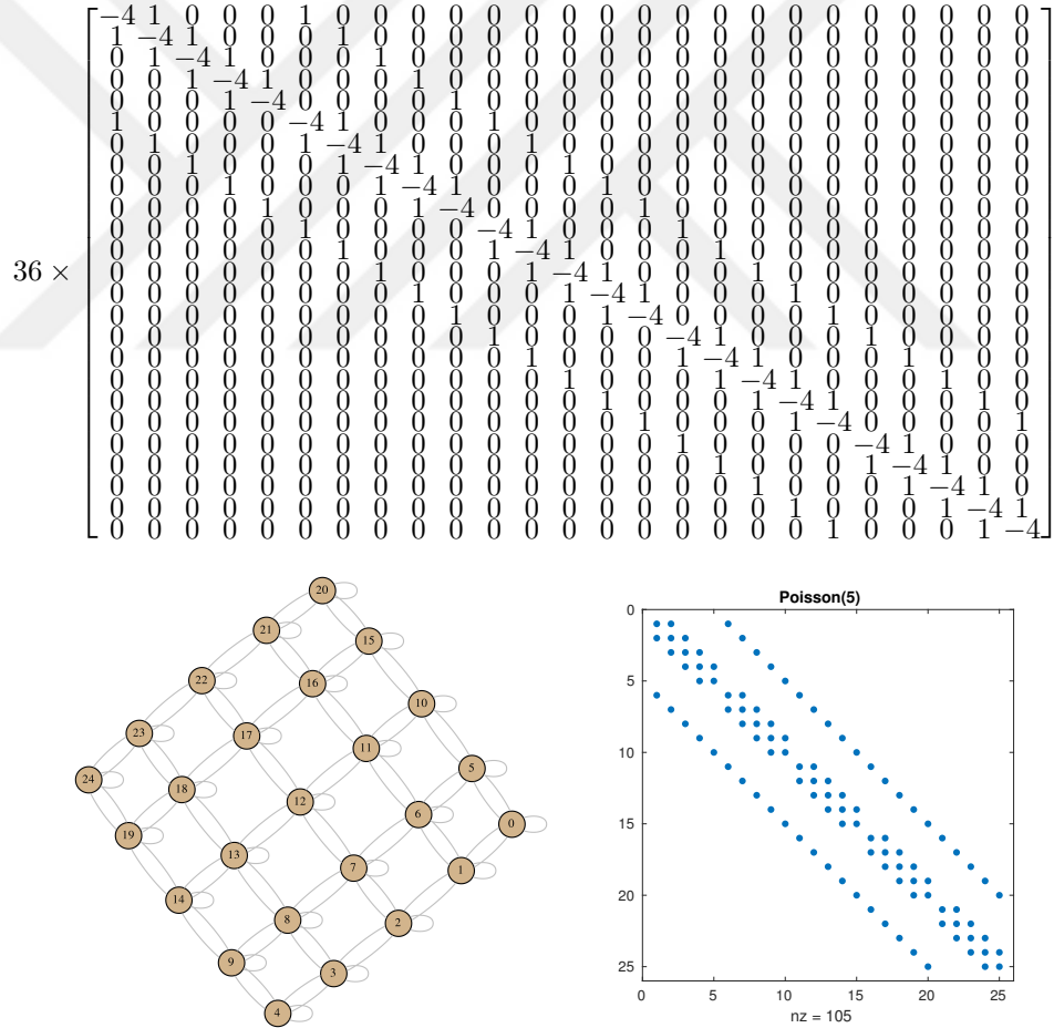
Figure 3.1: Matrix, graph, and spy representations of Poisson(5)
