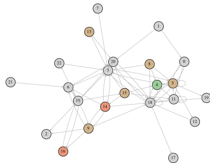
(g) Weighted, nproc = 4, graph rep.
