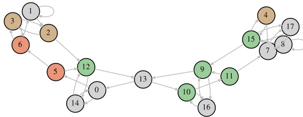
(g) Weighted, nproc = 4, graph rep.
