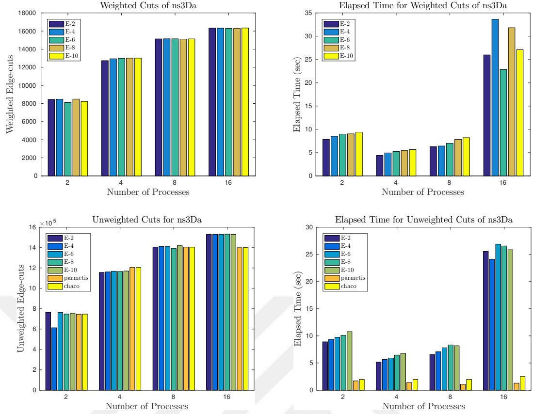
Figure 4.15: Results obtained from the partitioning of ns3Da
