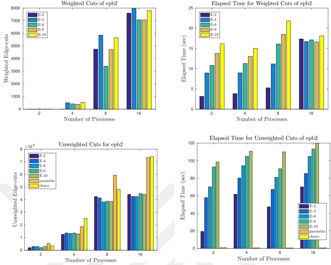
Figure 4.13: Results obtained from the partitioning of epb2
