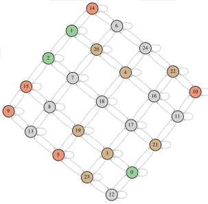
(e) Unweighted, nproc = 4 , graph rep.
