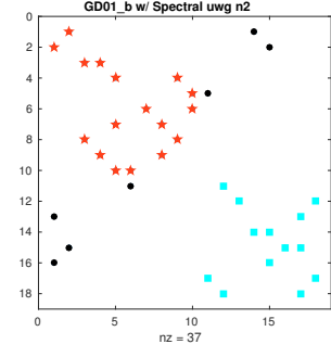
(b) Unweighted, nproc = 2, spy rep.
