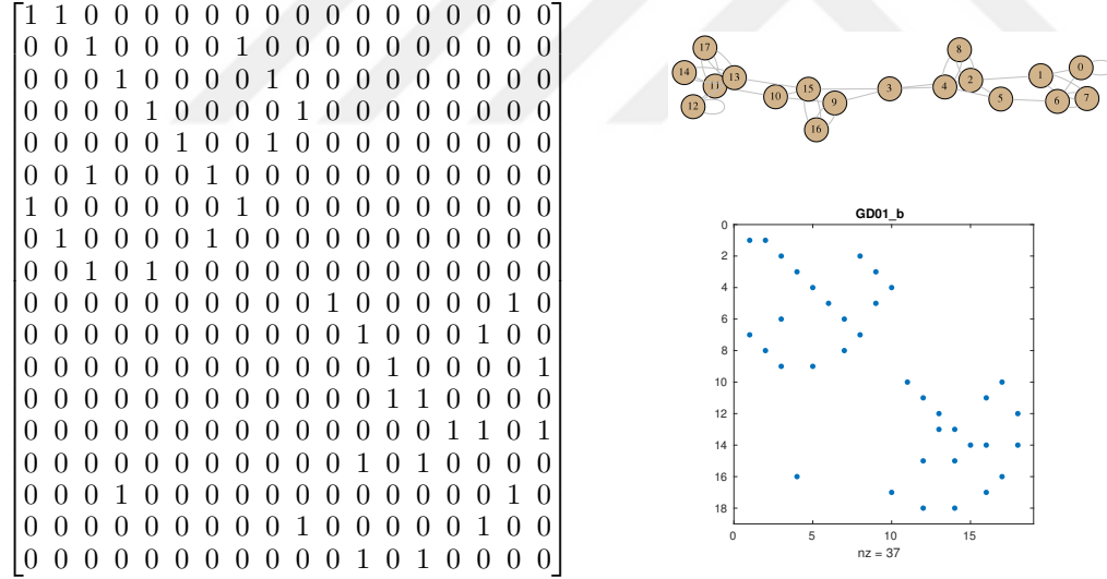
Figure 3.3: Matrix, graph, and spy representations of GD01_b
