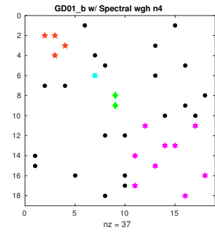
(h) Weighted, nproc = 4, spy rep.
