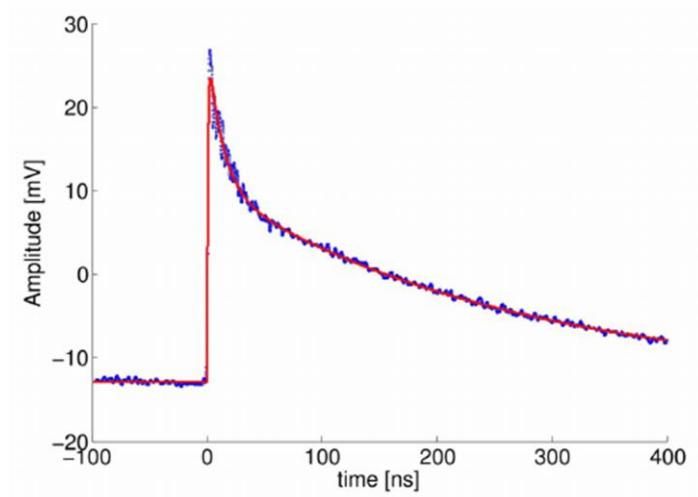
Figure 4.4 A SiPM Signal waveform.[21]
