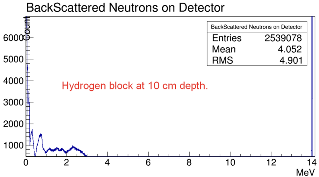
Figure 3.12 BSN on the detector, hydrogen block at 10 cm depth
