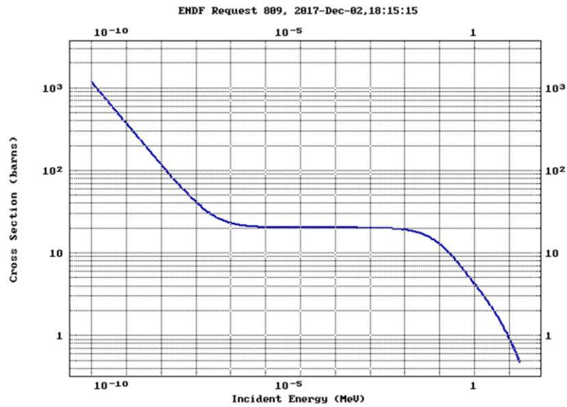
Figure 3.1 Neutron cross section for H-1 (ENDF/B-VII.1)
