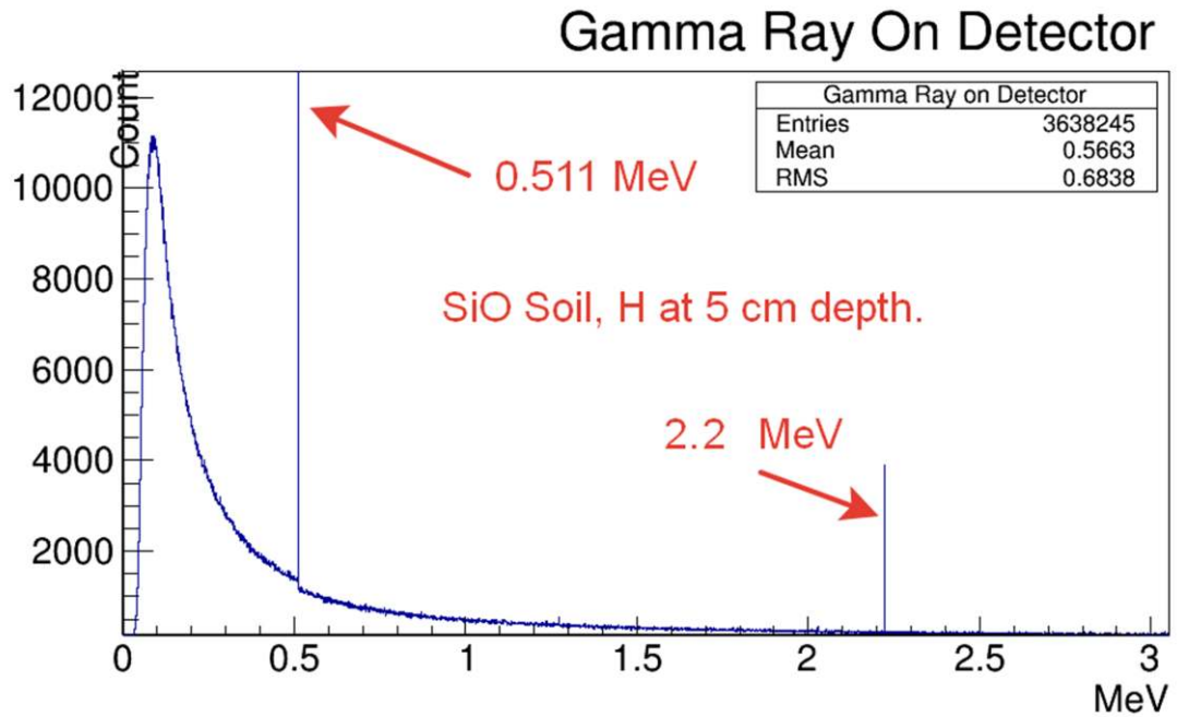
Figure 3.10 Gamma spectrum on the detector, hydrogen block at 5 cm depth.
