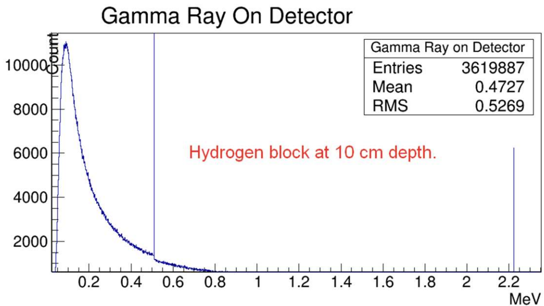
Figure 3.13 Gamma spectrum on the detector, hydrogen block at 10 cm depth.
