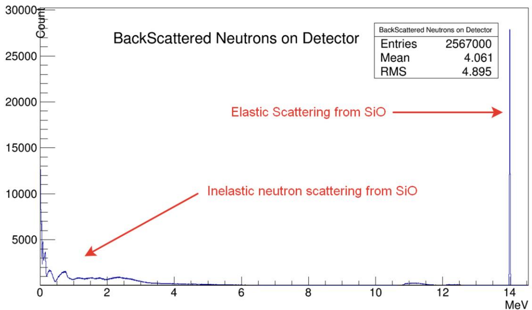
Figure 3.5 Back Scattered Neutrons energy from SiO.
