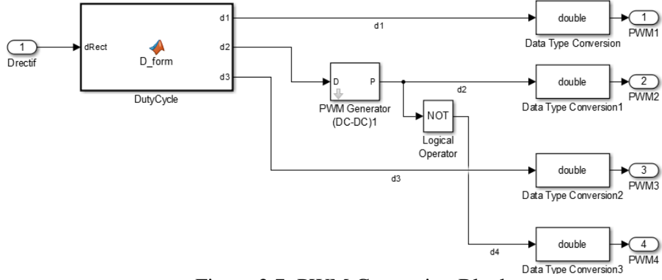
Figure 3.7: PWM Generating Block
