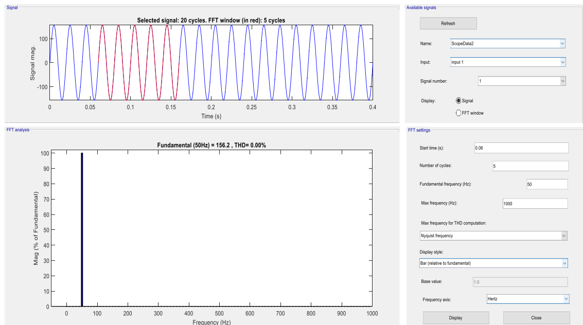
Figure5.6: Fourier analysis for grid voltage I_g
