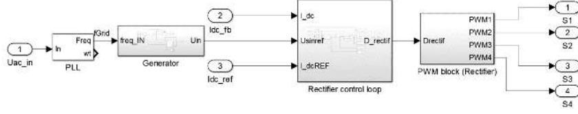
Figure 3.6: Rectifier Controller
