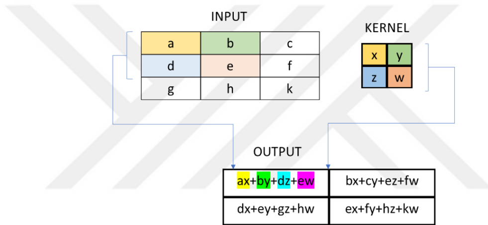
Figure 3.3. An example of 2D Convolution Operation
