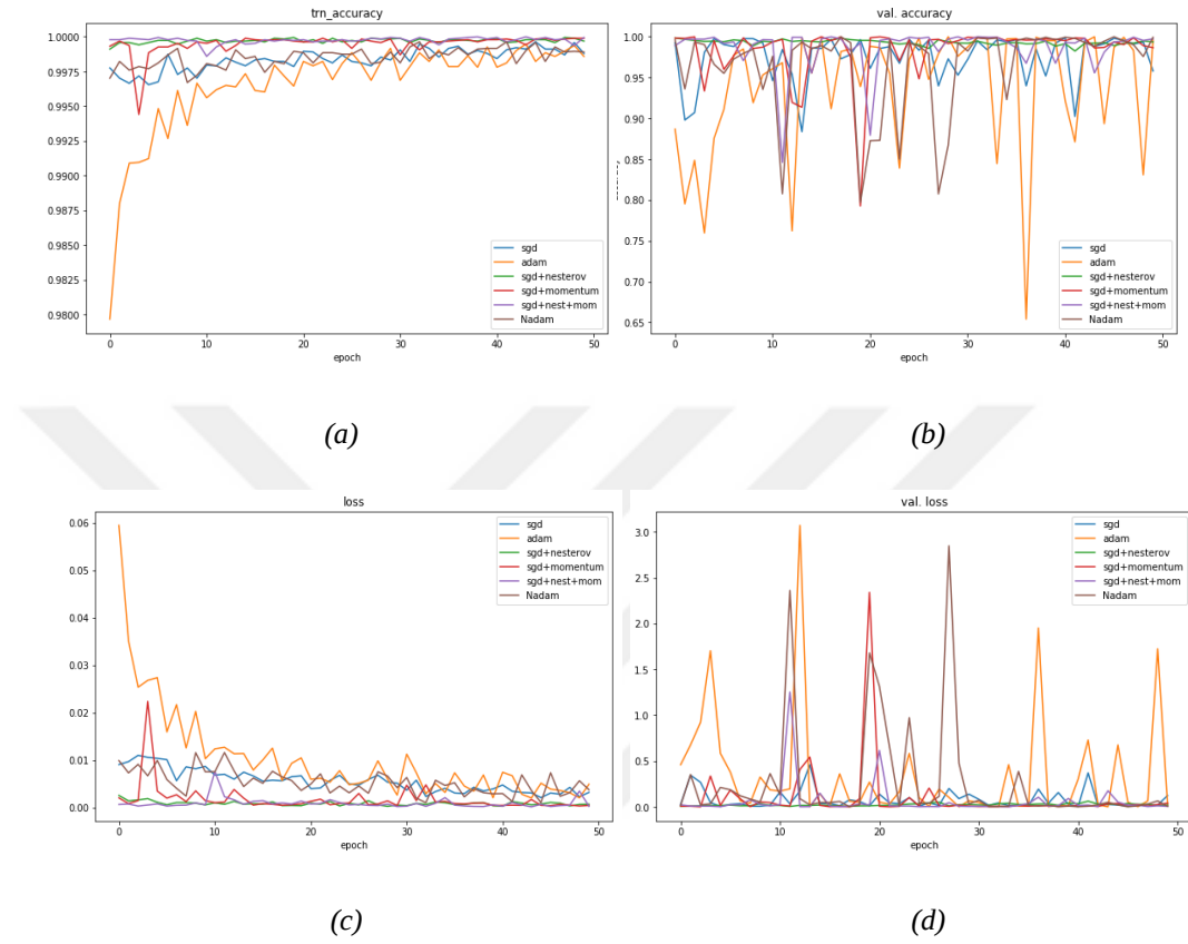
Figure 4.19. (a) Train accuracy (b) Validation accuracy (c) Train loss (d) Validation loss for 40x40 Images of the X-axis of the vibration data classification after 50 epochs with different optimizers
