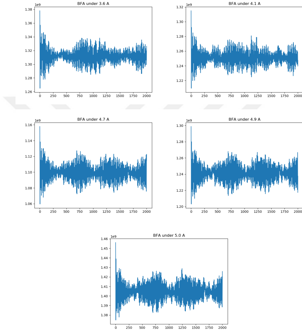
Figure 4.8. Autocorrelation sequences of the vibration data recorded for BFA under different loading conditions
