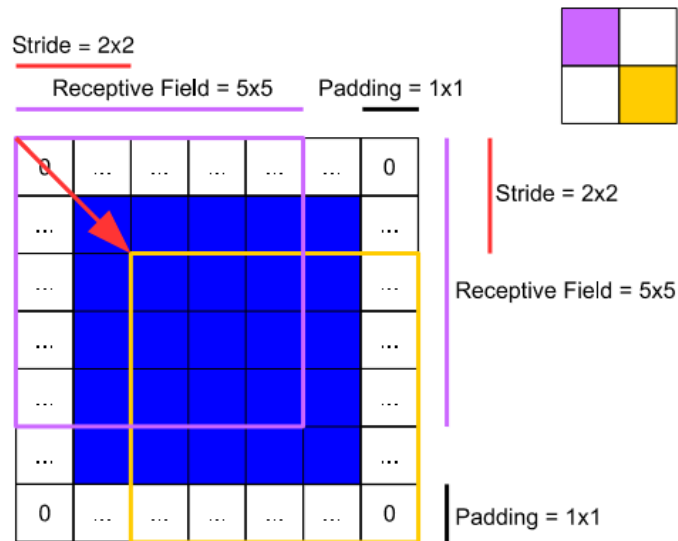
Figure 3.7. A visualization of the different hyperparameters of convolutional layers: receptive field, stride and padding (Altenberger and Lenz, 2018)
