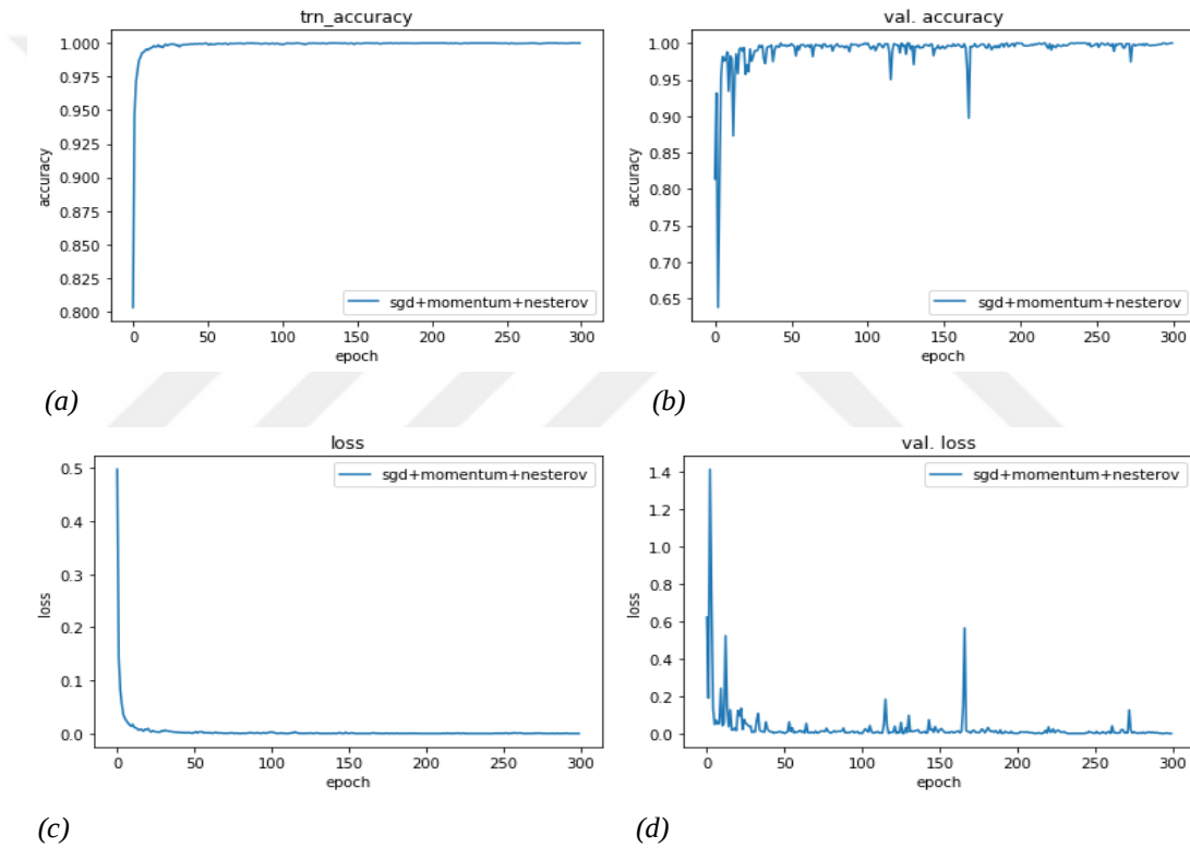
Figure 4.28. (a) Train accuracy (b) Validation accuracy (c) Train loss (d) Validation loss for 50x50 Color Images of the vibration data classification after 300 epochs using different optimizers
